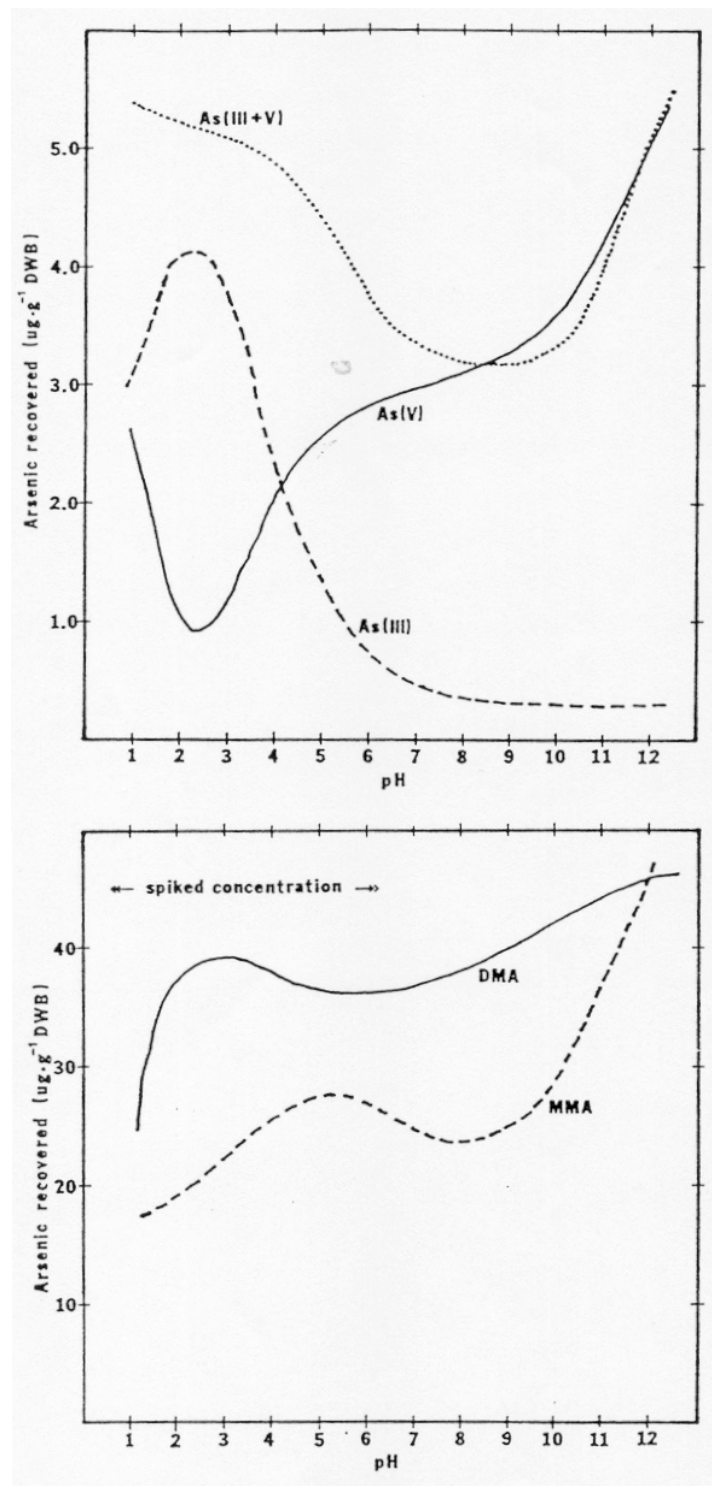
Figure 2-6. Arsenic species released from sediments as a function of solution pH. Plot of arsenic in sediment leached, \mu\text{g}\cdot\text{g}^{-1} dry weight basis (DWB), versus pH of leachate.
