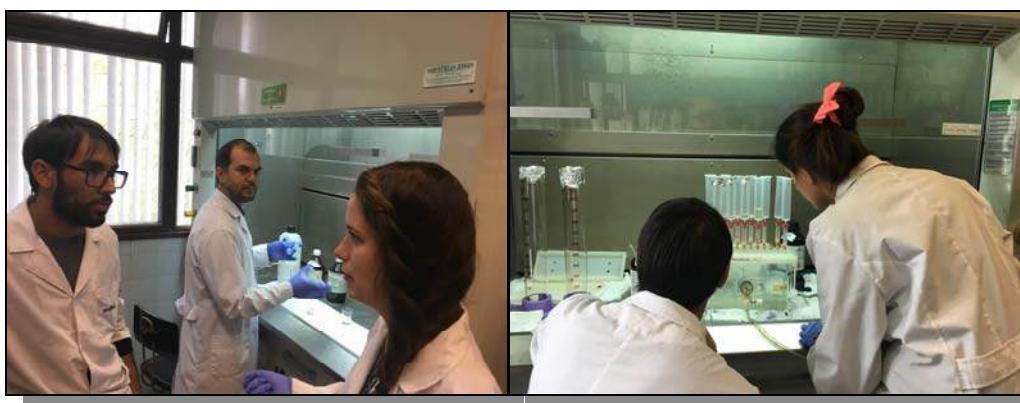
Figure 5. Analysis of PFAS in real samples: sample preparation.
