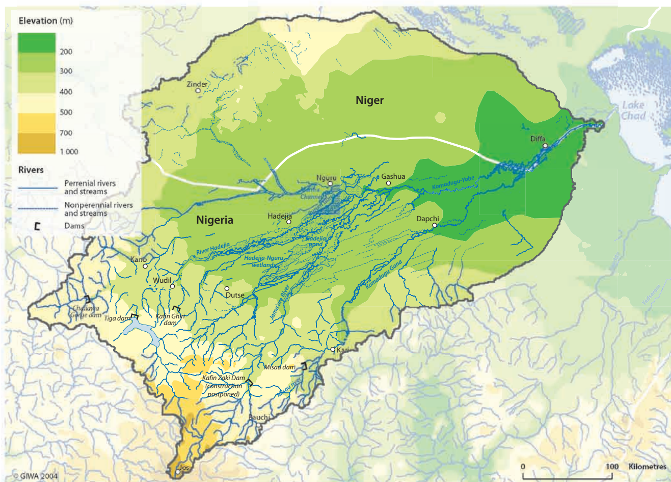
Figure 49 Komadugu-Yobe sub-system.
