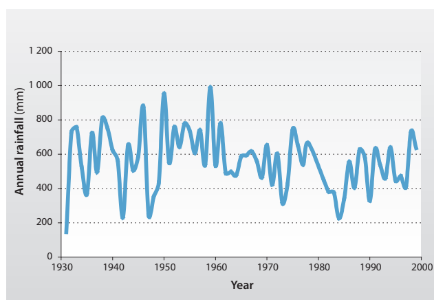
Figure 31 Annual rainfall at N'Djamena. (Source: Meteorological station at N'Djamena airport)
