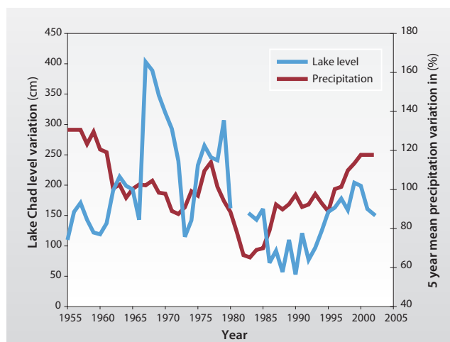
Figure 33 Lake Chad level variation and yearly precipitation at Bol. (Source: Tschierschke 2002)
