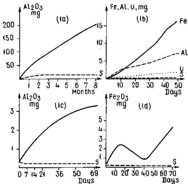
Fig. 1. General aspects of the kinetics of heterotrophic microbial solubilization of elements from rocks:
