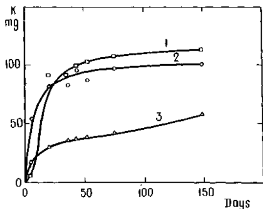
Fig. 2. Potassium solubilization of leucite vs. time
