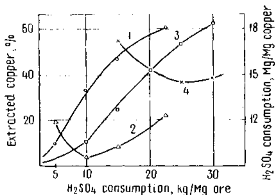
Fig. 5. Influence of the sulphuric acid concentration on the rate of bacterial and chemical extraction of copper from sulphide-oxide ores:
