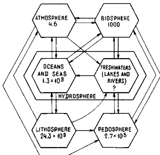
Fig. A simplified version of the biogeochemical cycle of sulfur
