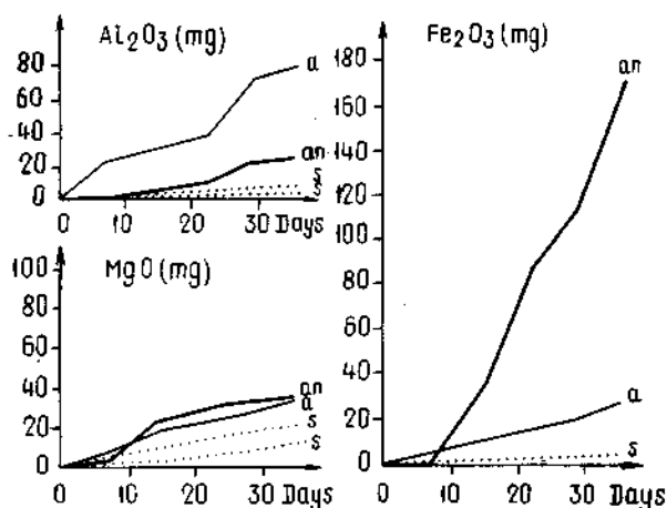
Fig. 4. Solubilization of aluminium, iron and magnesium by aerobic and anaerobic microflora during percolation of 50 g of a granite sand:
