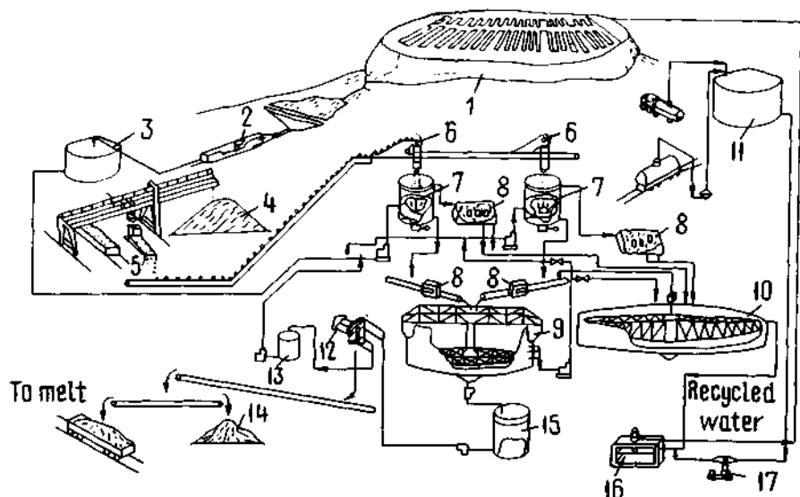
Fig. 2. Copper precipitation shop at "Utah" plant of Bingham Canyon Works, Kennecott Copper Corp.:
