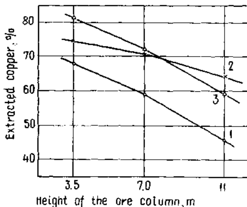
Fig. 4. Influence of the ore column height on the extraction of copper (sulphuric acid consumption 35 kg/t ore):
