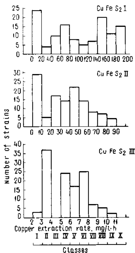
Fig. 2. Histograms of the ferrobacilli strains distribution in accordance with their copper extraction rates during the leaching of chalcopyrite specimens
