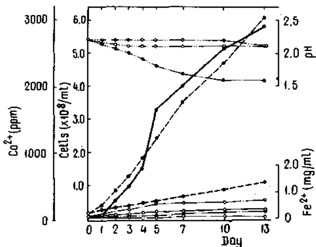
Fig. 6. Leaching of CoS with T. ferrooxidans in 9K medium. (trace amounts of Fe): — Cells, — \text{Fe}^{2+} , ..... \text{Co}^{2+} (leached), — pH a) 0 - 9K medium (trace Fe), inoculated; b) 9K medium (trace Fe) + CoS (1 %) inoculated; c) 9K medium (trace Fe) + CoS (1 %), not inoculated
