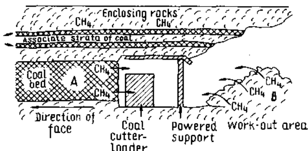
Fig. 7. Sources of methane emission into the atmosphere of a coal mine (scheme):
