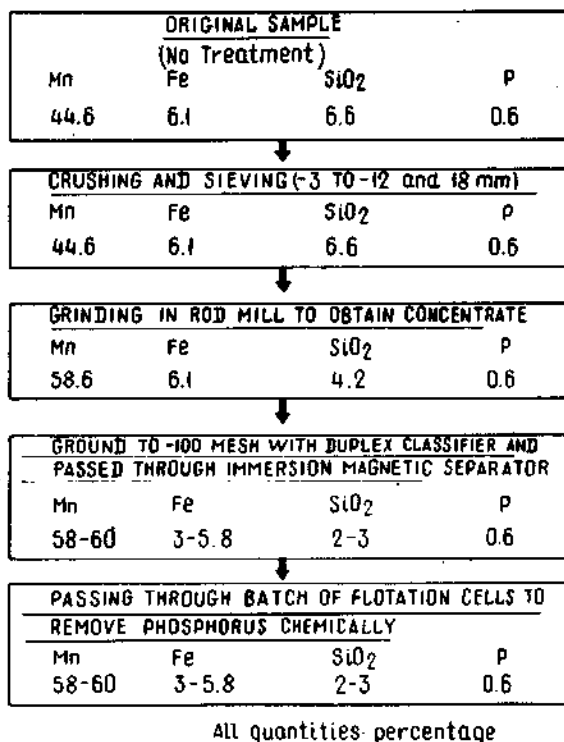
Fig. 3. Physical and Chemical Treatments Used for Removal of Phosphorus from Manganese Ores
