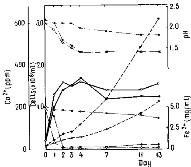
Fig. 5. Leaching of CoS with T. ferrooxidans in 9K medium: — Cells, — \text{Fe}^{2+} , ..... \text{Co}^{2+} (leached), — pH a) 0 - 9K medium ( \text{Fe}^{2+} , 5 mg/ml), inoculated; b) 9K medium ( \text{Fe}^{2+} , 5 mg/ml) + CoS (1 %), inoculated; c) 9K medium ( \text{Fe}^{2+} , 5 mg/ml) + CoS (1 %), not inoculated
