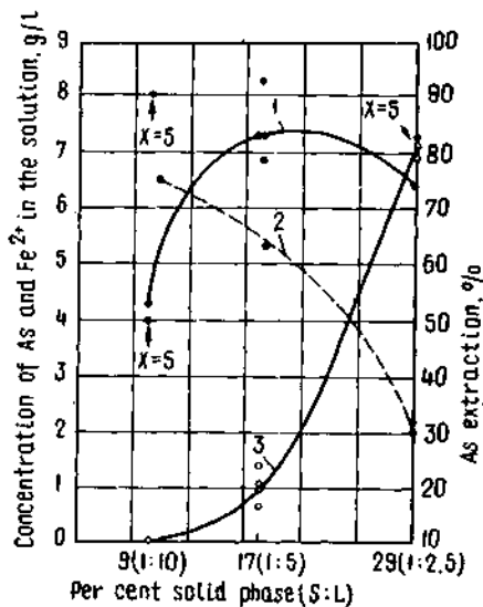
Fig. 3. Effect of pulp density (per cent solid) on the rate of arsenic leaching (1) and variation in Fe 2+ concentration in the solution (2):
