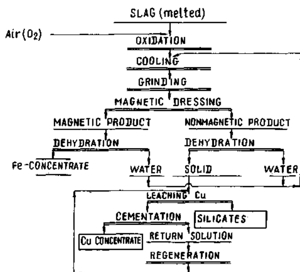
Fig. 1. Basic flowsheet for copper slag processing
