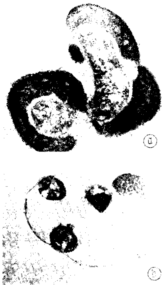
Fig. 6. Deposition of \text{Fe}^{3+} on the outer surface of L. ferrooxidans cells
