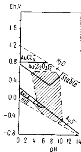
Fig. Correlations of stability between some gold compounds in water at 25 °C and 1 atm of undirect pressure. The sum total of dissolved chloride components is 10^{-6} ; the sum total of dissolved sulfur is 10^{-1} . The cross-hatching indicates the field of stable gold-organic complexes in natural waters
