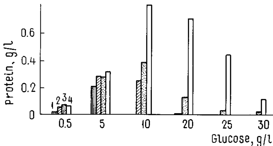
Fig. 1. Dependence of the stimulating effect of Mn^{2+} and Mn^{4+} on the growth of Leptothrix pseudoochraceae upon glucose content of the medium:
