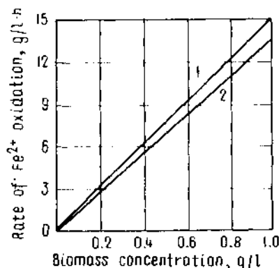
Fig. 1. Effect of T. ferrooxidans biomass concentration on the rate of \text{Fe}^{2+} oxidation in the solution:
