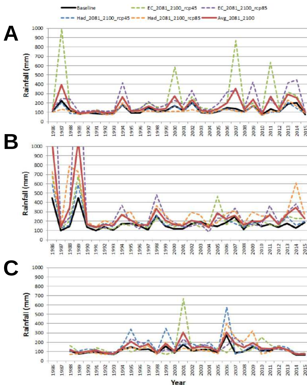
Figure 12. Annual maximum daily rainfall for the period 2081—2100. A = Pakse city; B = Paksan city; C = Savannakhet city. The graph depicts a time series of the maximum daily rainfall event for each year of the observed rainfall time series. Solid black lines represent the baseline climate conditions, solid red lines represent the average of all model projections, and dashed lines represent individual model projections under either RCP 4.5 (blue, green) or RCP 8.5 (orange, purple).
