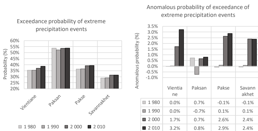
Figure 2.6: Exceedance probability of high precipitation events (left) and the shifted anomaly in probability (right)
