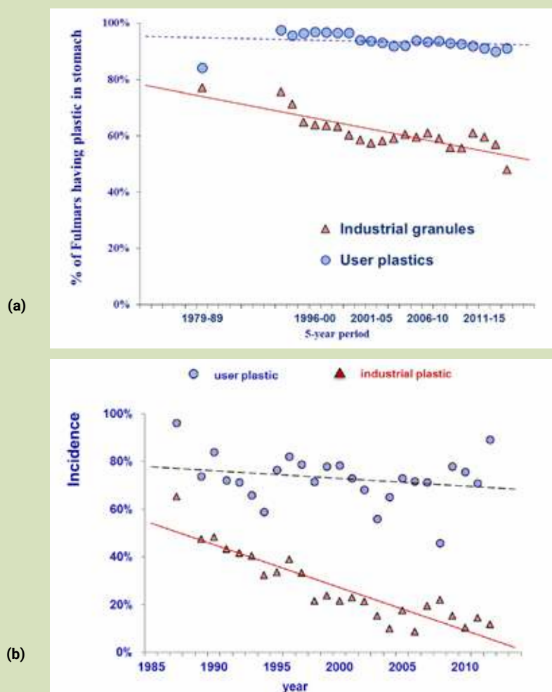
Figure 7.6 Long term time trends in the plastic composition in a) the gut contents of the northern fulmar in the North Sea (graph derived from Table 3.B in Van Franeker and Kühn 2018) , and b) surface net samples in the North Atlantic Gyre (image used under the Creative Commons Licence, ©van Franeker and Law 2015) showing a very small decline in 'user' plastic but a much greater decline in 'industrial' plastic.
