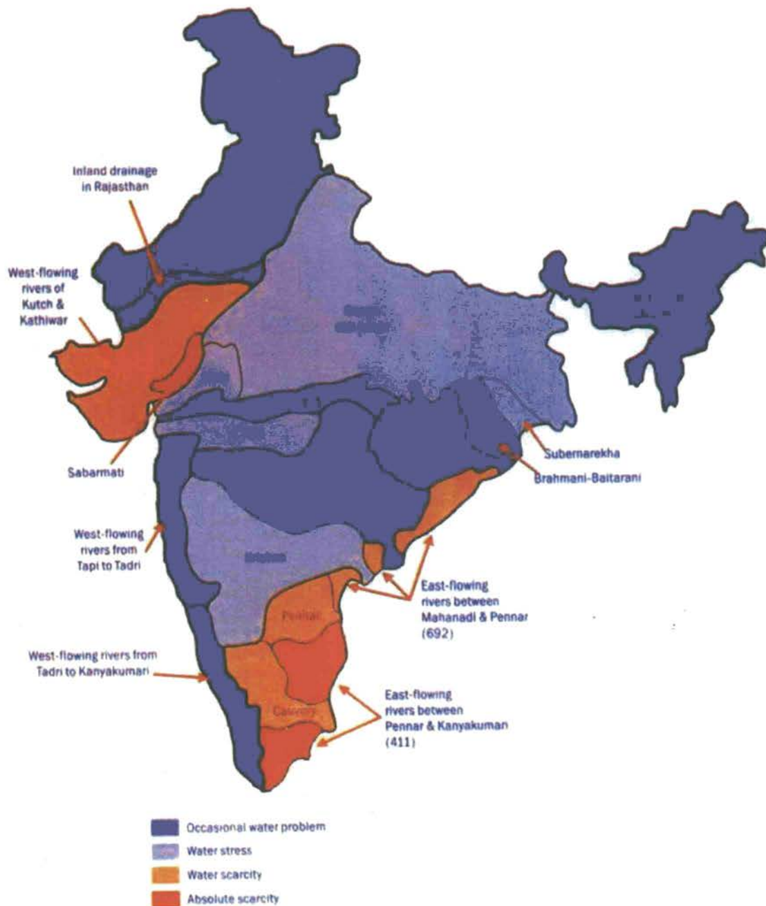
Map 11.1 Per capita resource availability in the country's river basins (Chitale 1992)
