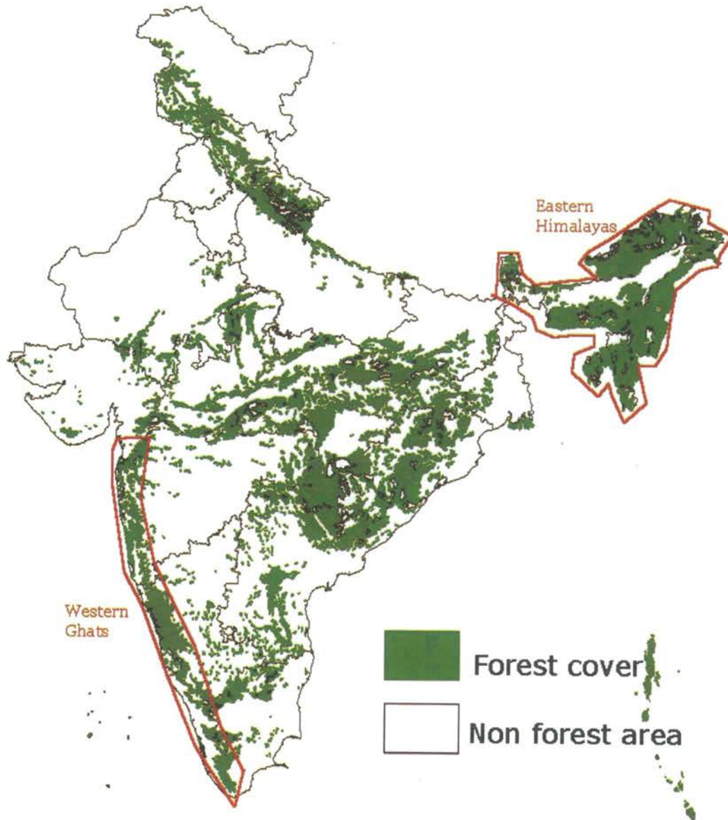
Map 9.1 National forest vegetation map of India with biodiversity hotspots
