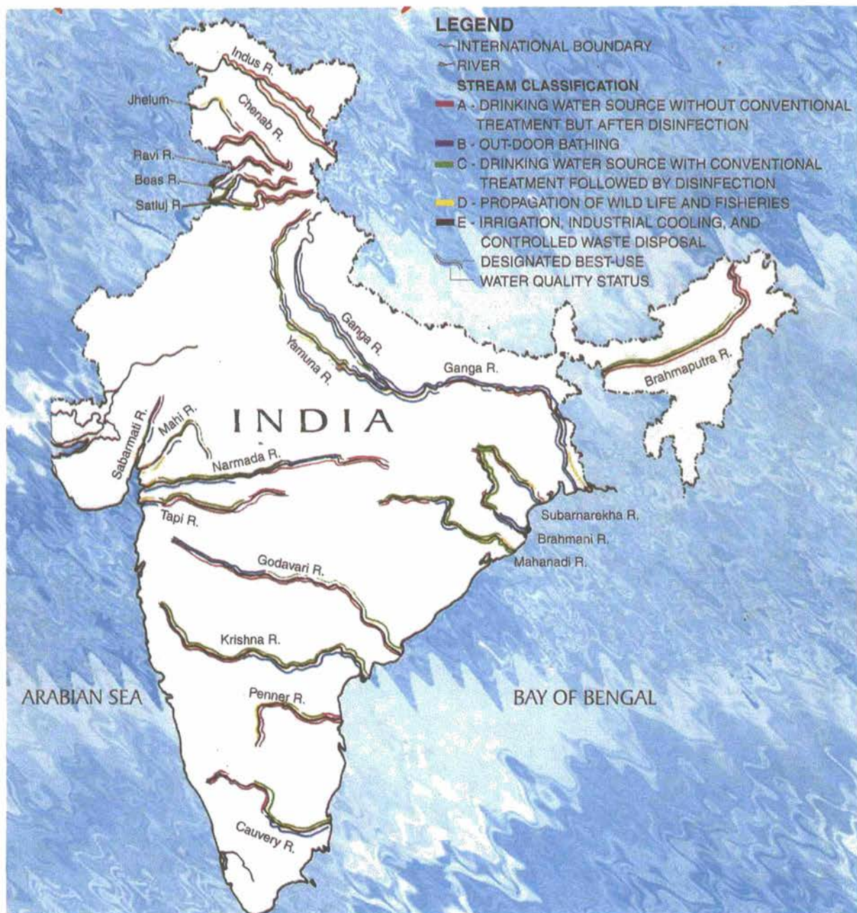
Map 11.2 Water quality profile of major Indian rivers
