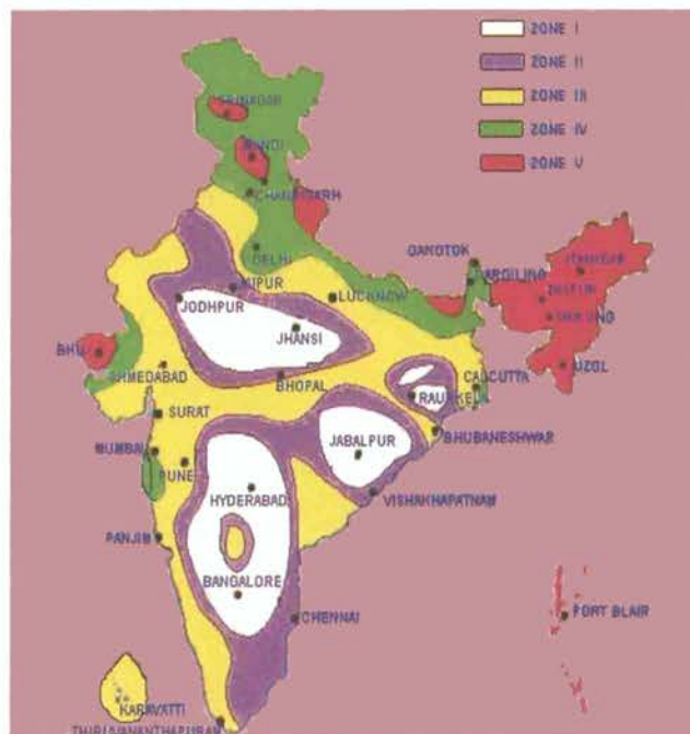
Map 6.1 Earthquake Zoning Map
