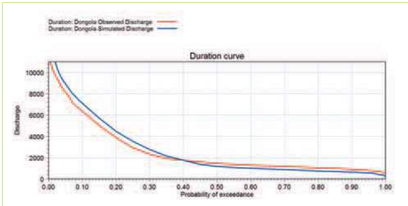
Figure 5.91 Comparison of the observed (red) & simulated (blue) flow duration curves at the Abay station for the period 1960-1980
