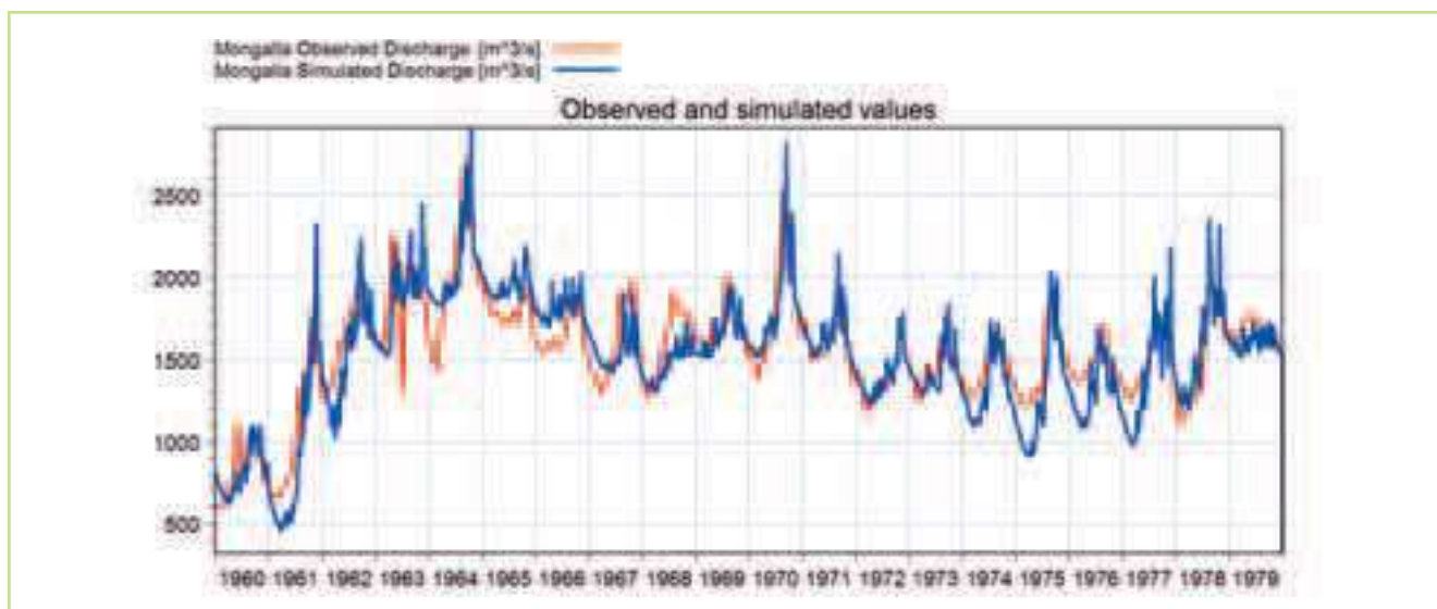
Figure 5.23 Comparison between observed (red) & simulated (blue) discharge at Mongalla for the modelling period 1960-80
