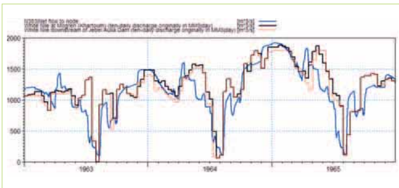
Figure 5.38 Observed flow at Mogren (black line), simulated flow at Mogren (blue line) & observed flow at Jebel Aulia (red line)
