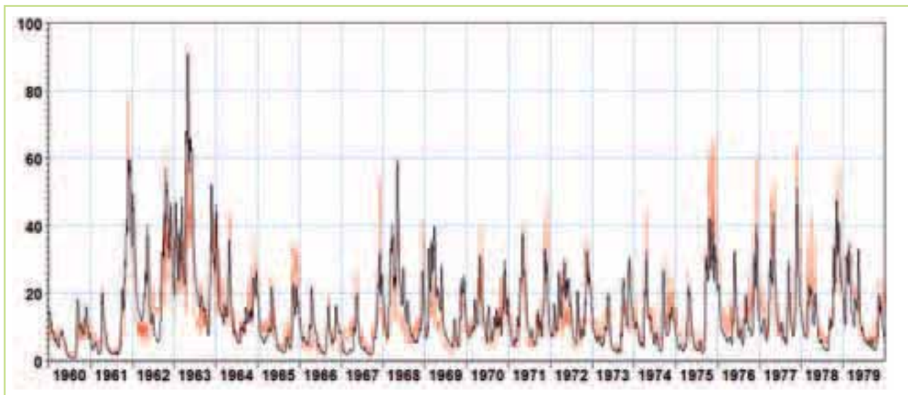
Figure 5.15 Comparison between simulated (black) & observed discharge (red) for UG20_84267_Mitano for the period 1960-1980. It has been possible to obtain a reasonable & realistic representation throughout the 20 years period, indicating good data quality as well as the RR-models ability to reproduce the flow regime
