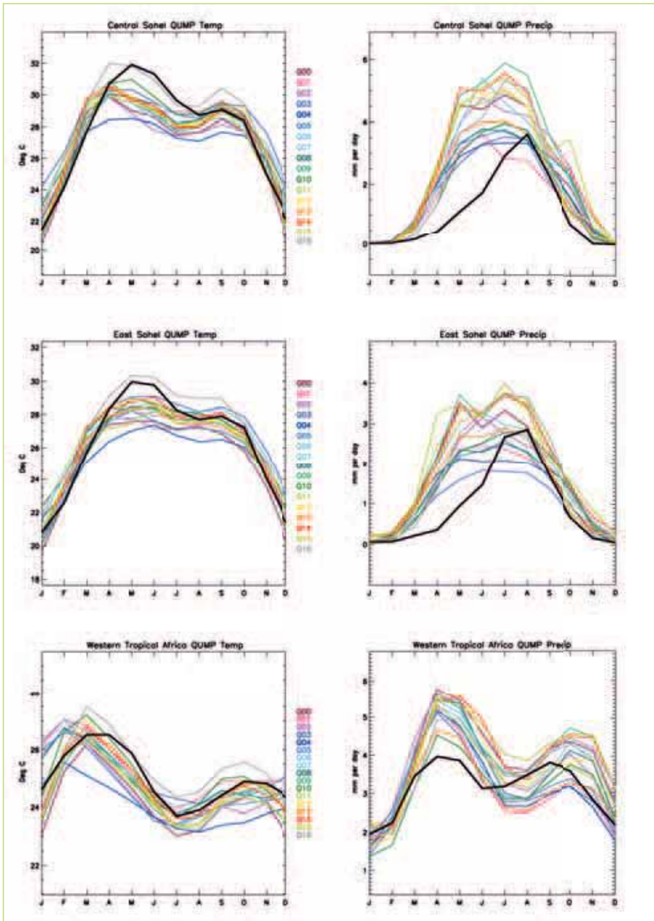
Figure 3.7 The annual variation in temperature (left) & precipitation (right) for Central Sahel, East Sahel & Western Tropical Africa. The black line shows the observed values of temperature & precipitation from CRU 3.0 & CMAP, respectively, while the coloured lines show the model outcomes
