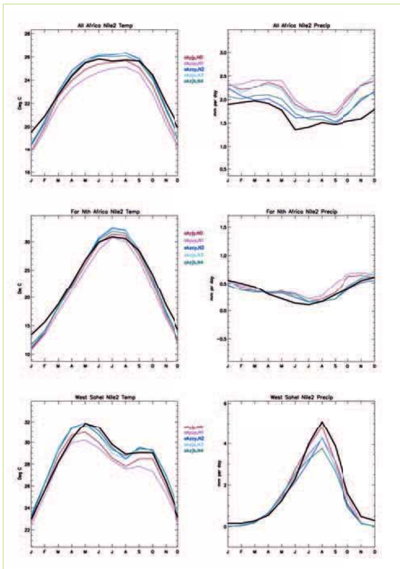
Figure 3.15 The annual variation in temperature (left) & precipitation (right) for Africa, North Africa & West Sahel. The black lines show the observed values of temperature & precipitation from CRU 3.0 & CMAP, respectively, while the coloured lines show the selected RCM ensemble member simulations
