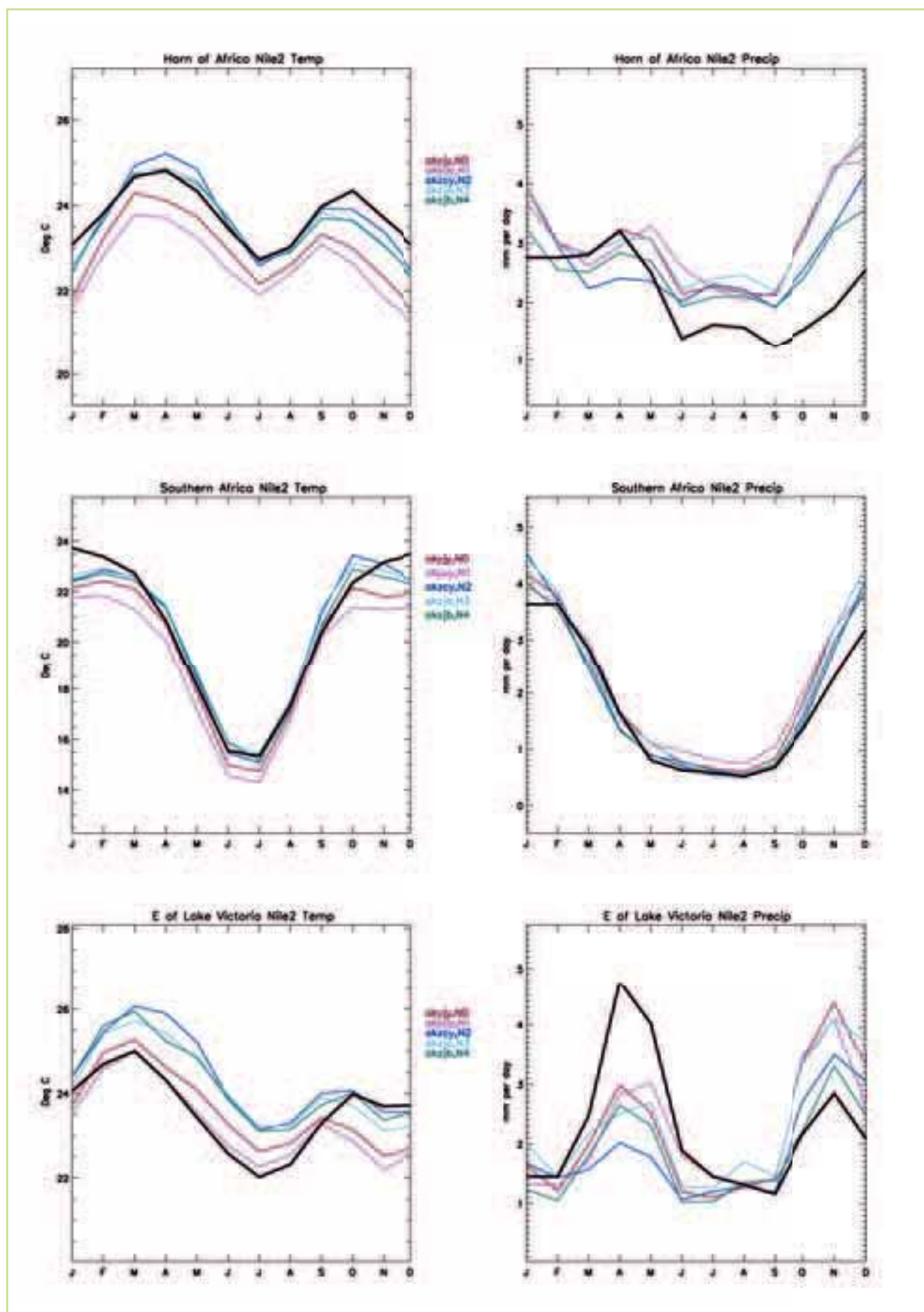
Figure 3.17 The annual variation in temperature (left) & precipitation (right) for the Horn of Africa, Southern Africa & East of Lake Victoria. The black lines show the observed values of temperature & precipitation from CRU 3.0 & CMAP, respectively, while the coloured lines show the selected RCM ensemble member simulations
