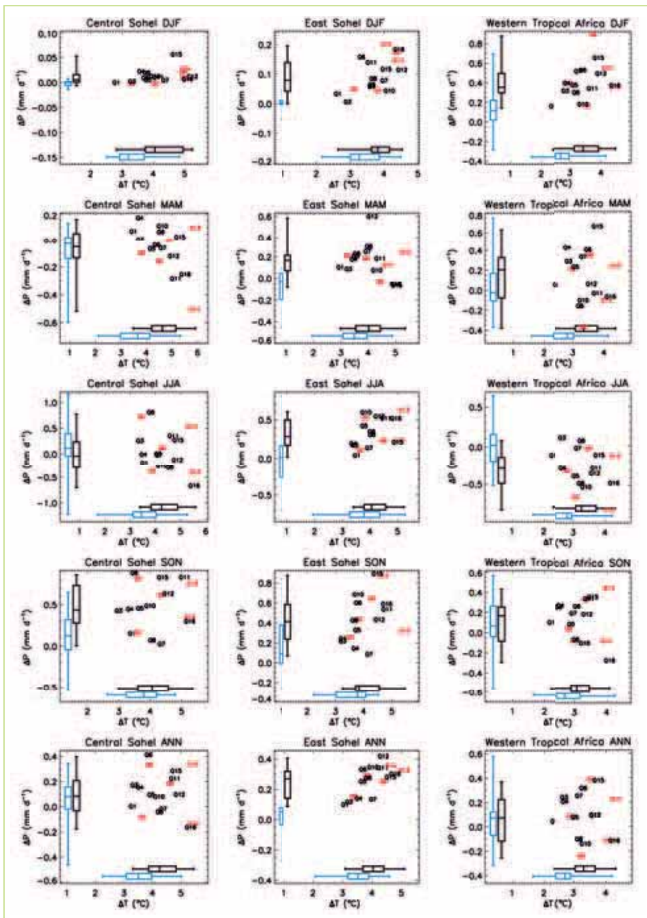
Figure 3.14 Plots for the QUMP ensemble showing projected change in precipitation versus change in the temperature for Central Sahel, East Sahel & Western tropical Africa. The panels show the spread in projected outcomes during DJF, MAM, JJA, SON & annual (ANN). The data point labels (Q#) identify the models & the red data points indicate the selected sample
