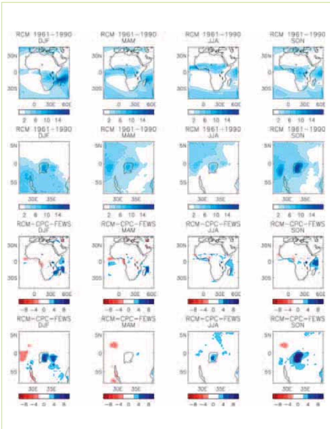
Figure 3.21 Average daily rainfall in mm/day for each season for the African continent (top) & the Lake Victoria region (second row) from the baseline model runs (average over 5 ensemble members) & model bias (bottom rows) when compared to CPC-FEWS
