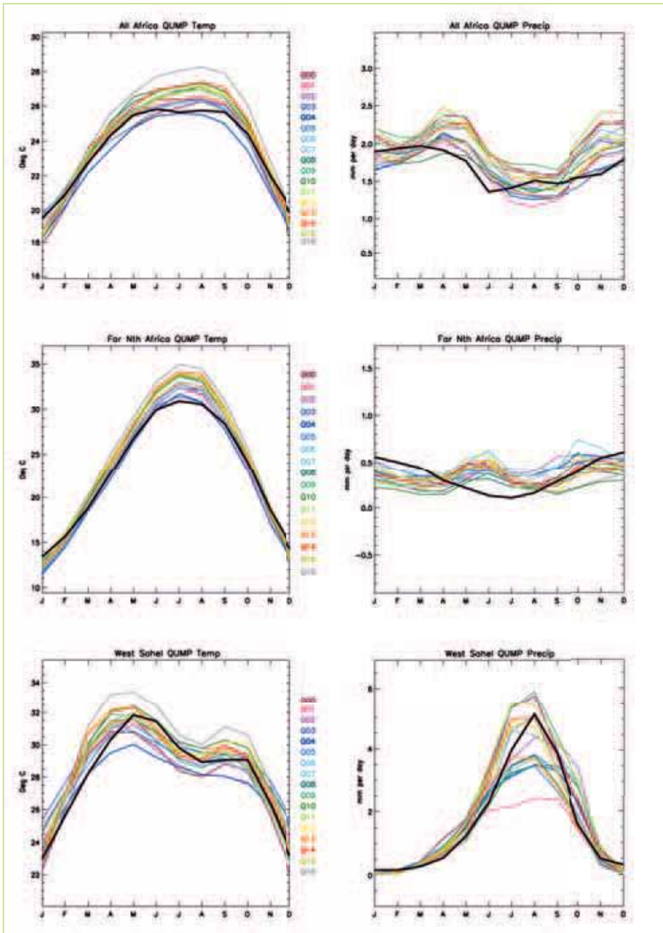
Figure 3.5 The annual variation of temperature (left) & precipitation (right) for Africa, North Africa & West Sahel. The black line shows the observed values of temperature & precipitation from CRU 3.0 & CMAP, respectively, while the coloured lines show the model outcomes. Note the differences in y-axis scaling, especially for precipitation
