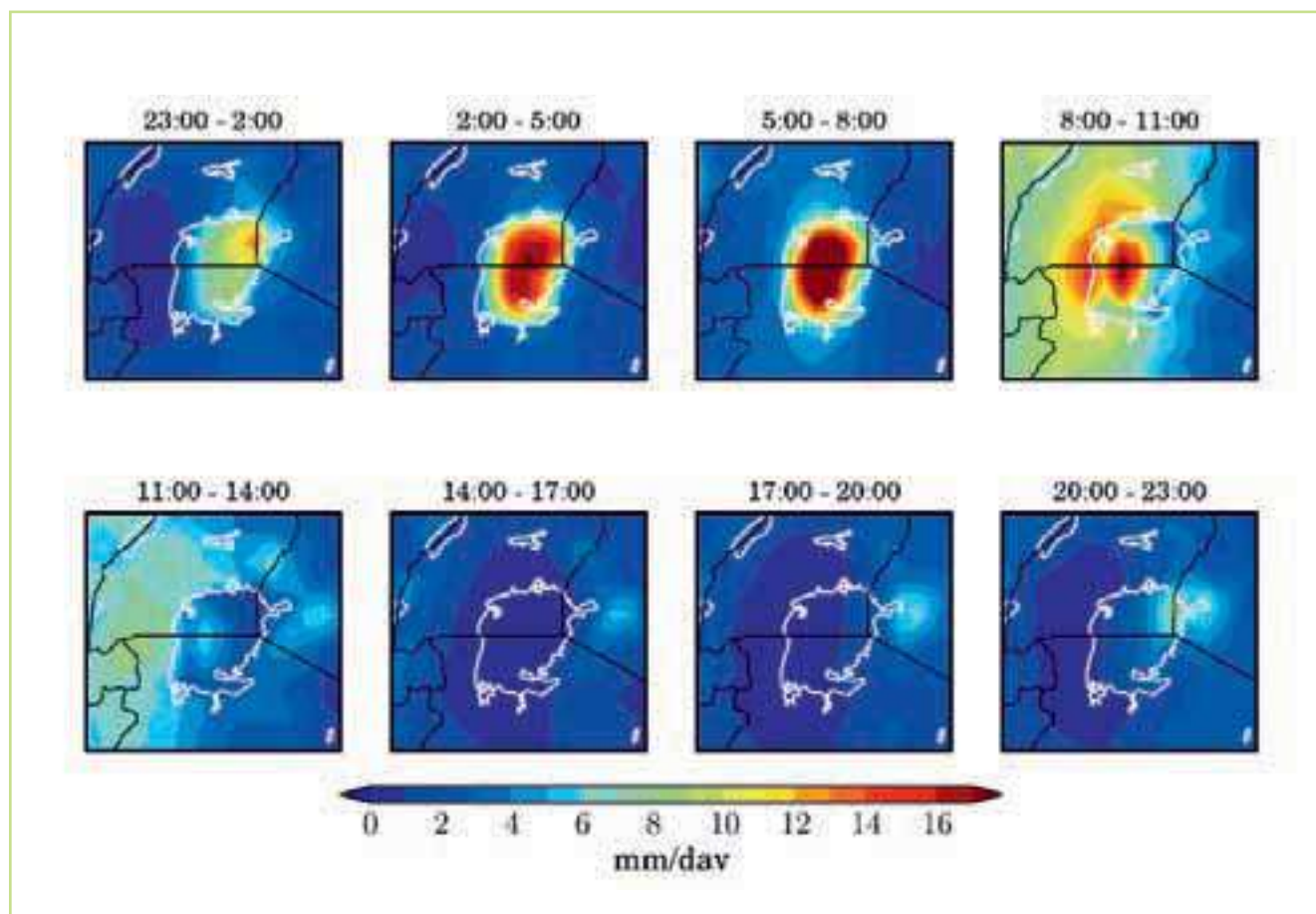
Figure 3.22 Convective rainfall in the model, averaged over each day in a baseline period of 1961-1990 & averaged over the RCM ensemble
