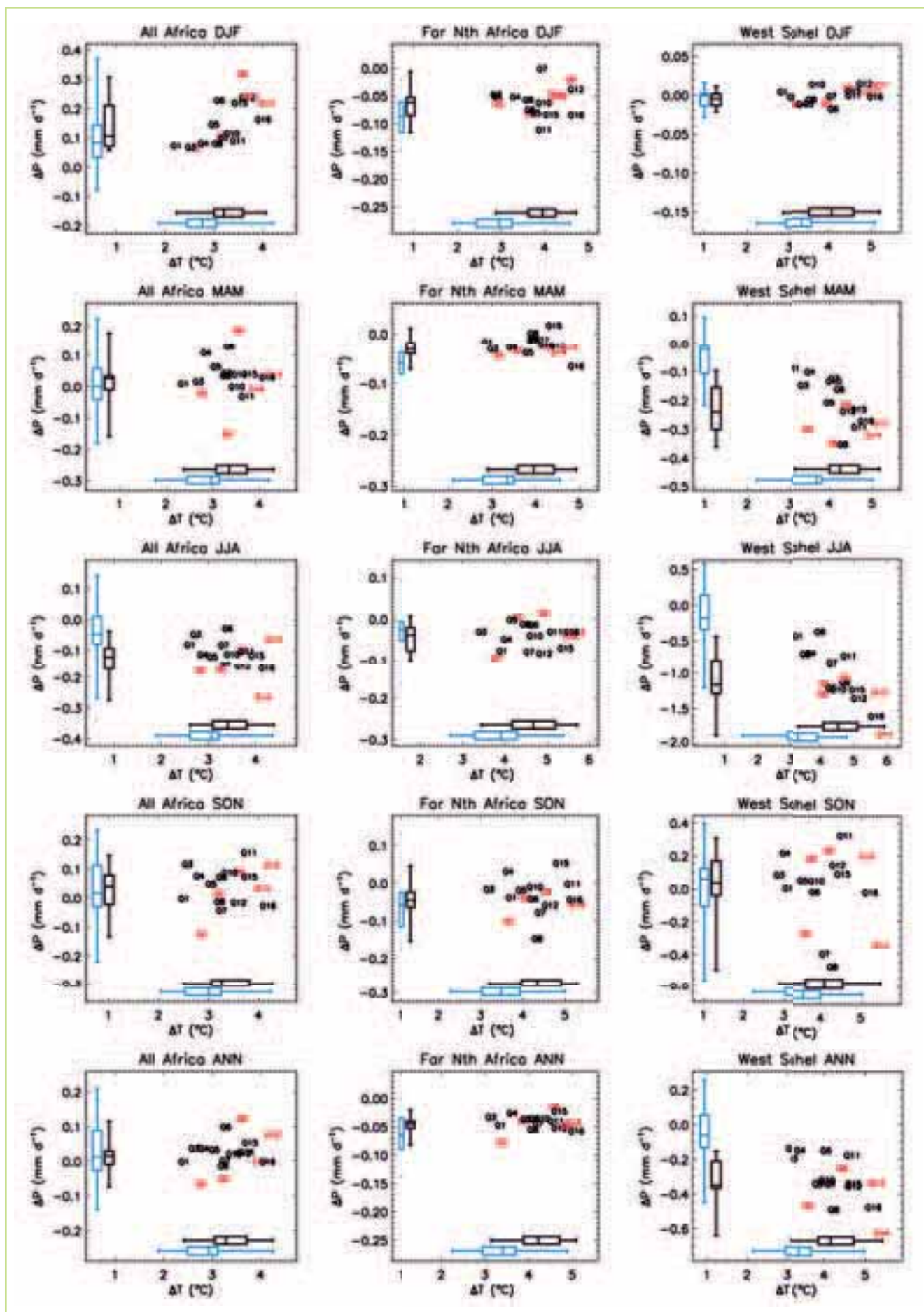
Figure 3.12 Plots for the QUMP ensemble showing projected change in precipitation versus change in the temperature for all Africa, North Africa & West Sahel. The panels show the spread in projected outcomes during DJF, MAM, JJA, SON & annual (ANN). The data point labels (Q#) identify the GCM models & the red data points indicate the selected sample
