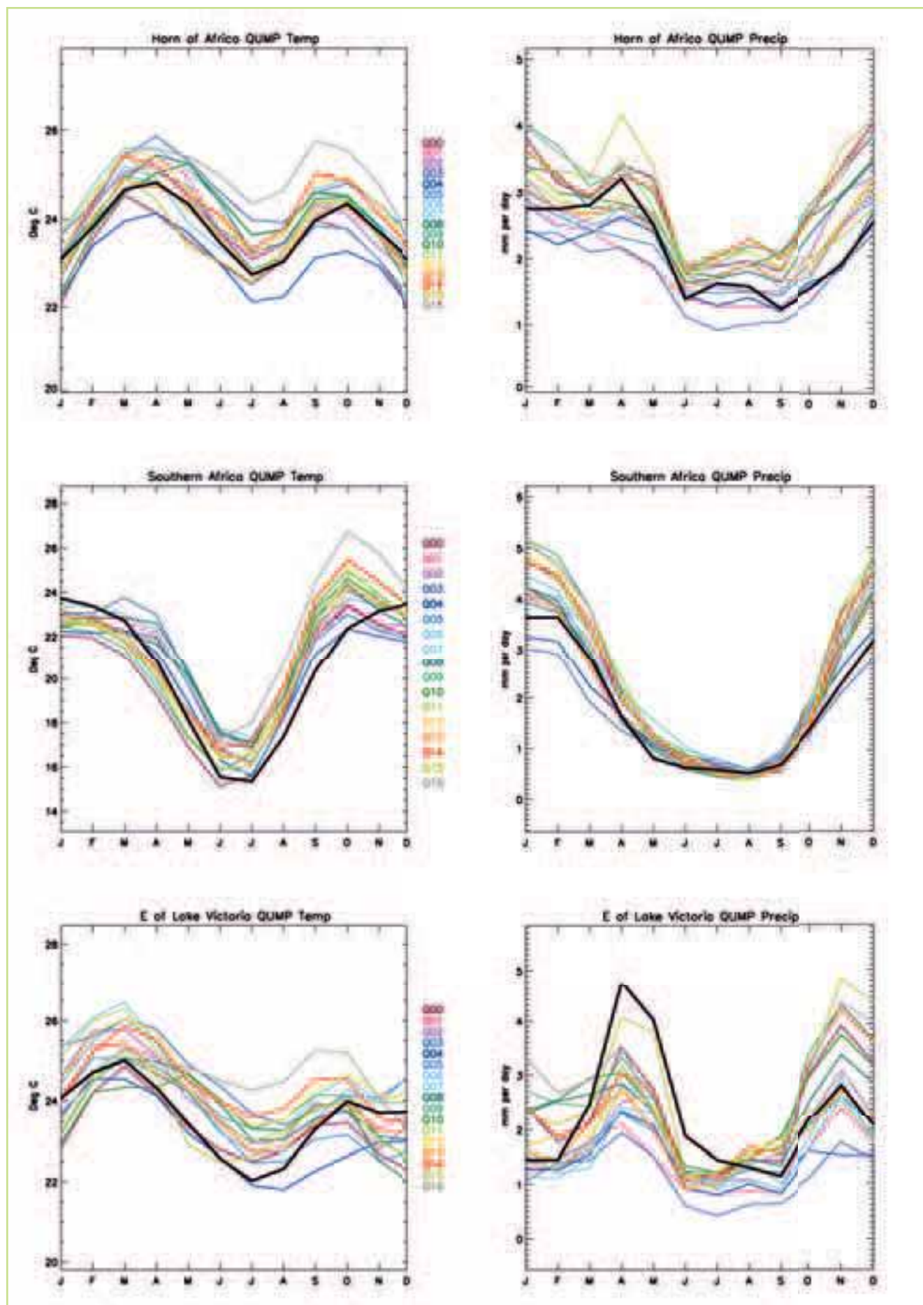
Figure 3.6 The annual variation of temperature (left) & precipitation (right) for Horn of Africa, Southern Africa & East of Lake Victoria. The black line shows the observed values of temperature & precipitation from CRU 3.0 & CMAP, respectively, while the coloured lines show the model outcomes
