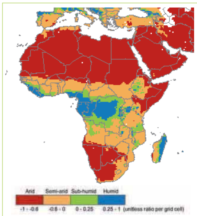
Figure 6.4 CMI Annual Mean for Africa from GWSP Digital Water Atlas (2008). Map 40: Climate Moisture Index (V1.0). Available online at http://atlas.gwsp.org
