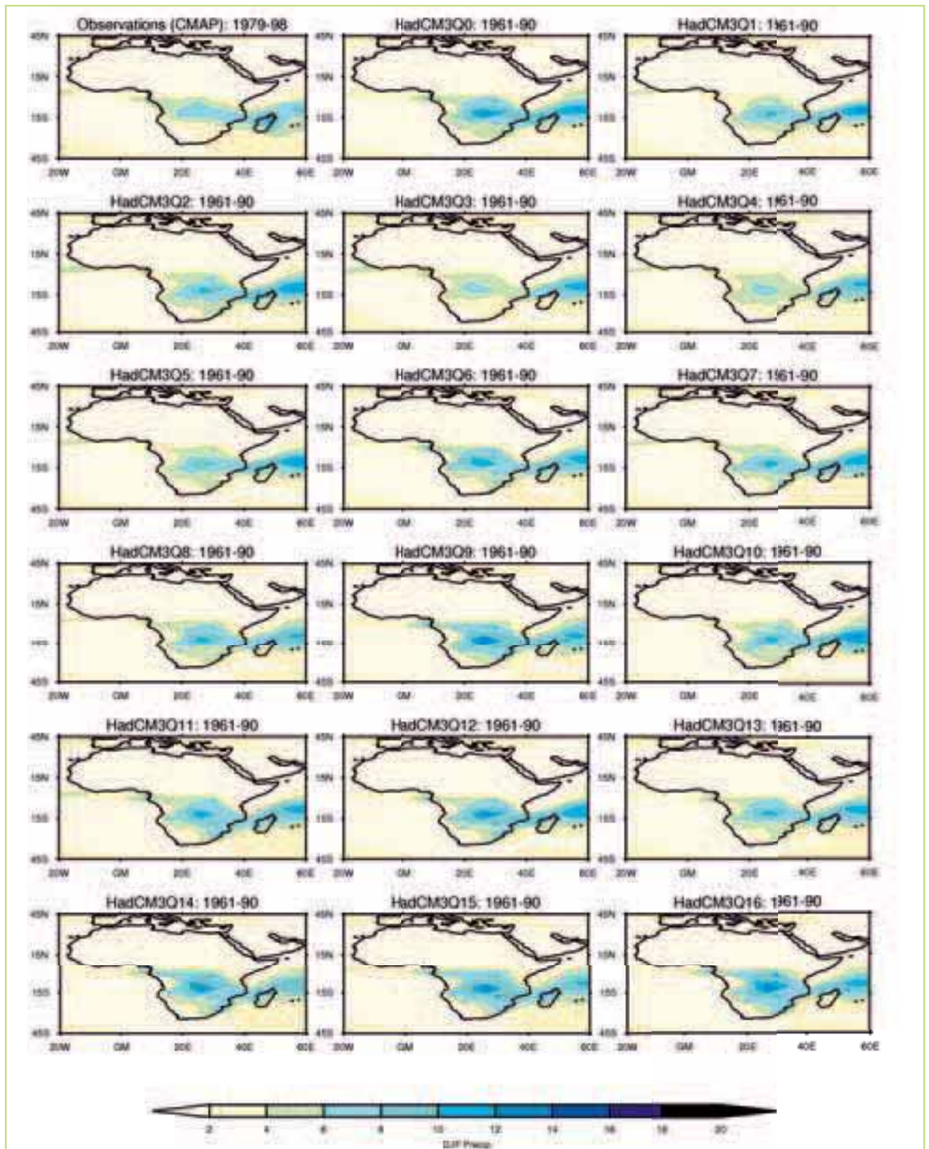
Figure 3.9 A comparison of observed & simulated precipitation for Africa during DJF. The observations were taken during the period 1979-1998 & the simulation data during the period 1961-1990. All values are in mm/d
