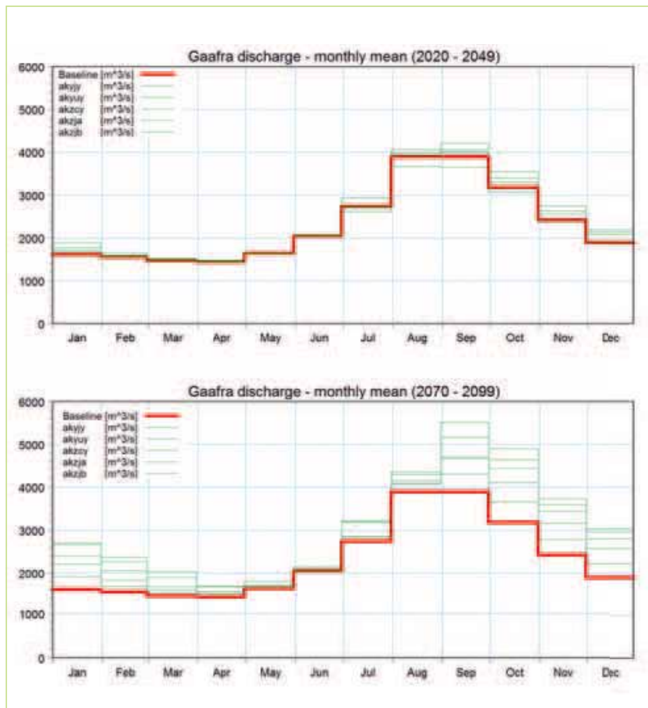
Figure 4. Projected changes in the average monthly flows for the Nile at Gafra (El-Ga'afra). Projections are shown for two periods; 2020-2049 (top) & 2070-2099 (bottom). The solid (red) line shows the baseline levels (1961-1990) & the thin green lines the different RCM ensemble member projections
