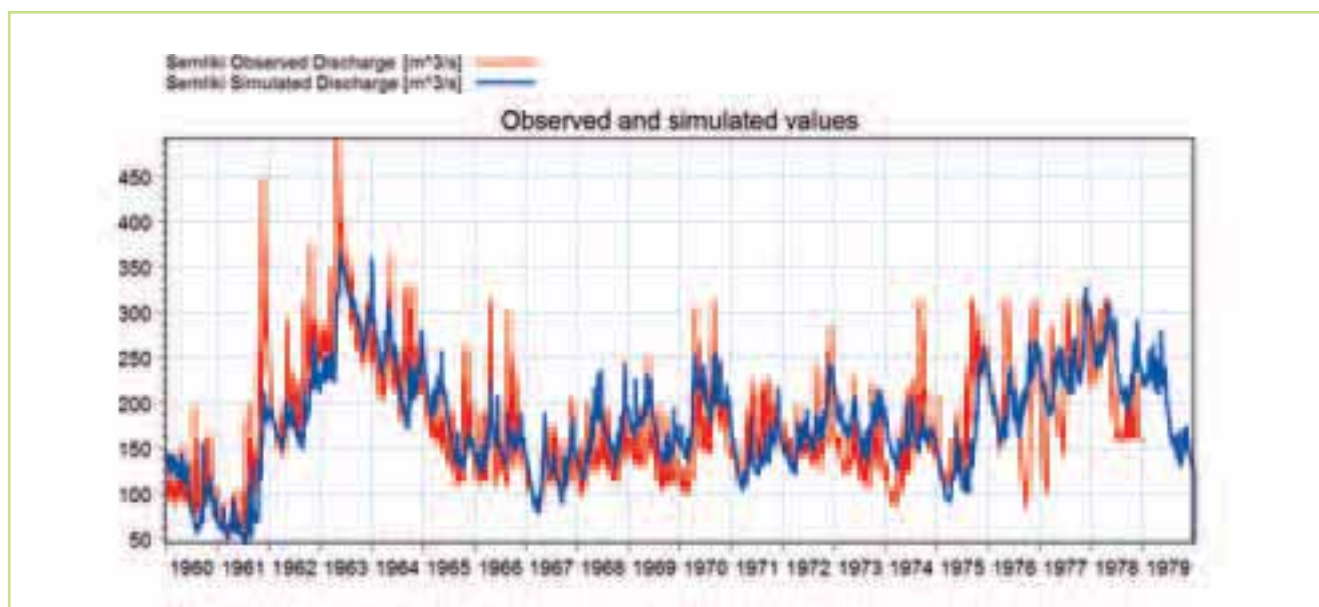
Figure 5.51 Comparison of the observed (red) & simulated (blue) flow hydrographs at the Semliki station for the period 1960-1980
