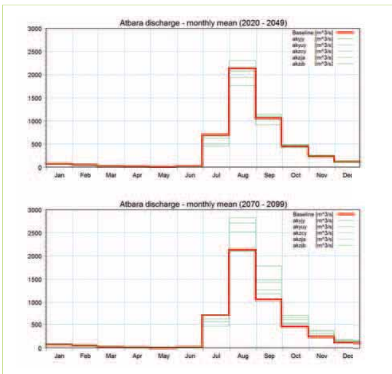
Figure 7.8 Projected changes in the average monthly flows for the Atbara station for the two periods; 2020-2049 & 2070-2099. The solid (red) line shows the baseline levels (1961-1990) & the thin green lines the different RCM ensemble members
