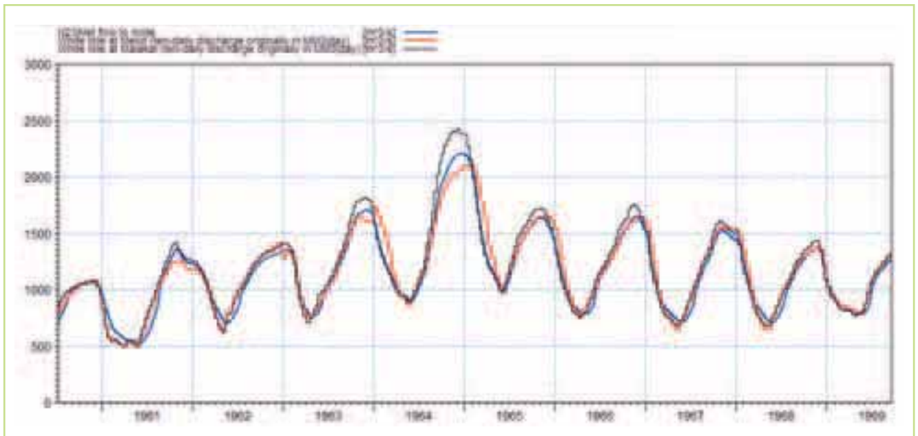
Figure 5.36 Observed flow at Malakal (black line), observed flow at Melut (red line) & simulated flow at Melut (blue line)
