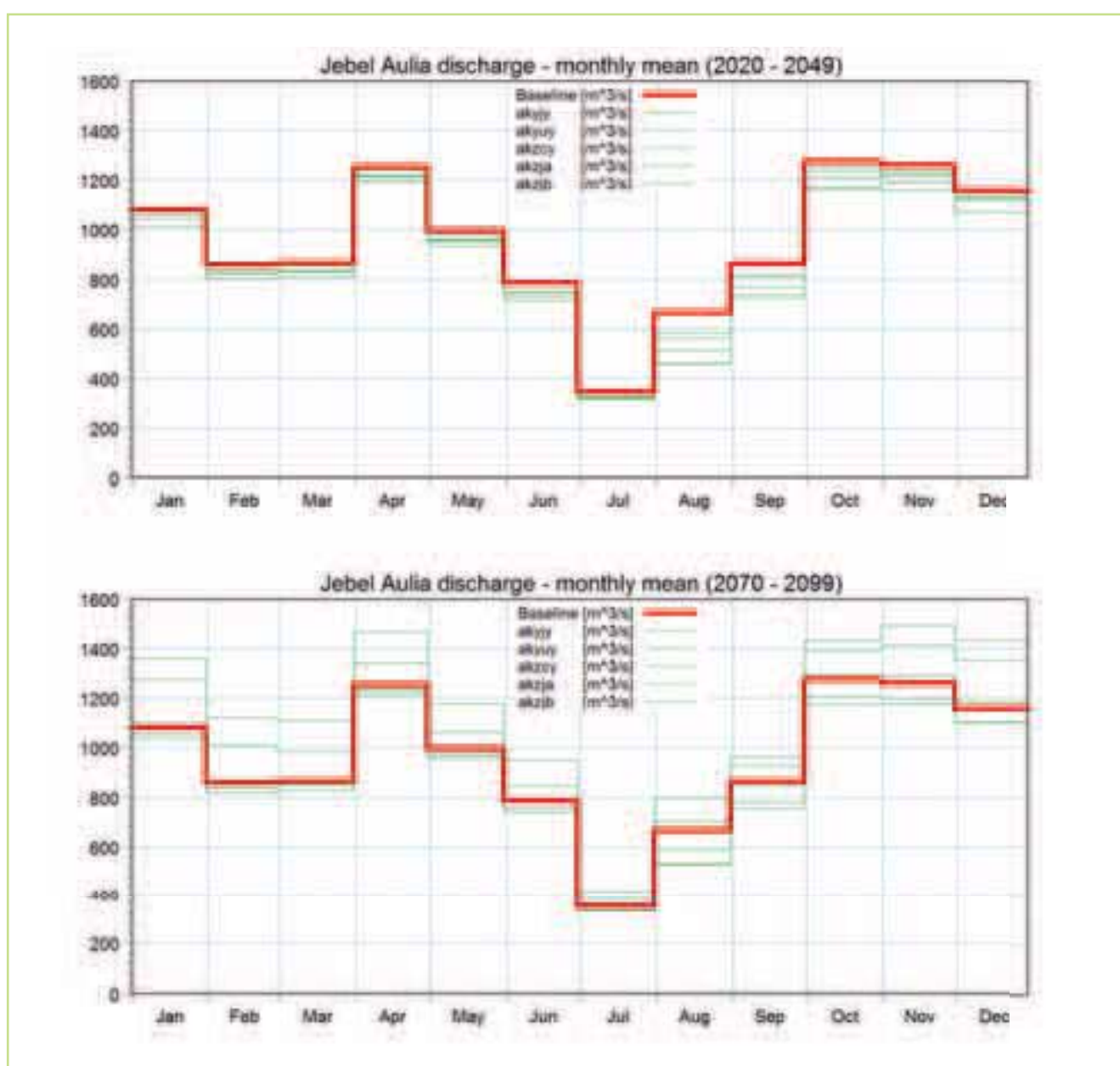
Figure 7.4 Projected changes in the average monthly flows for the Jebel Aulia station for the two periods; 2020-2049 & 2070-2099. The solid (red) line shows the baseline levels (1961-1990) & the thin green lines the different RCM ensemble members
