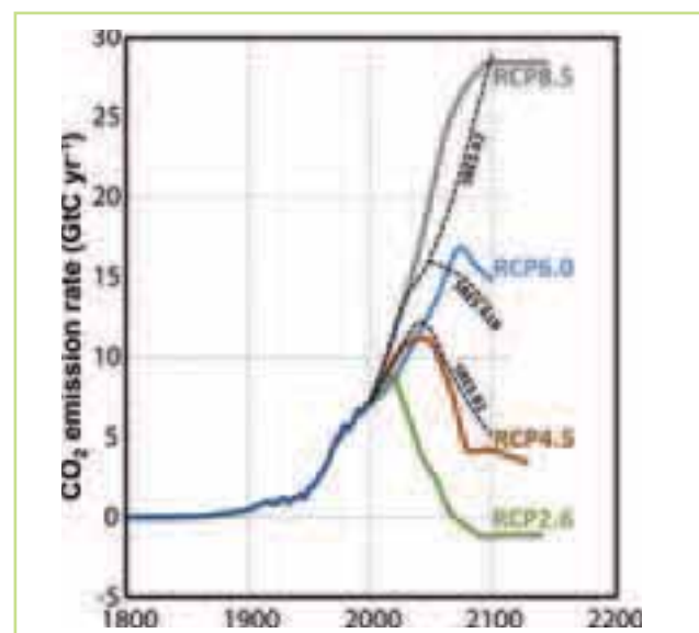
Figure 3.2 Comparison of CO 2 emissions for SRES & RCP scenarios (van Vuuren et al., 2011)
