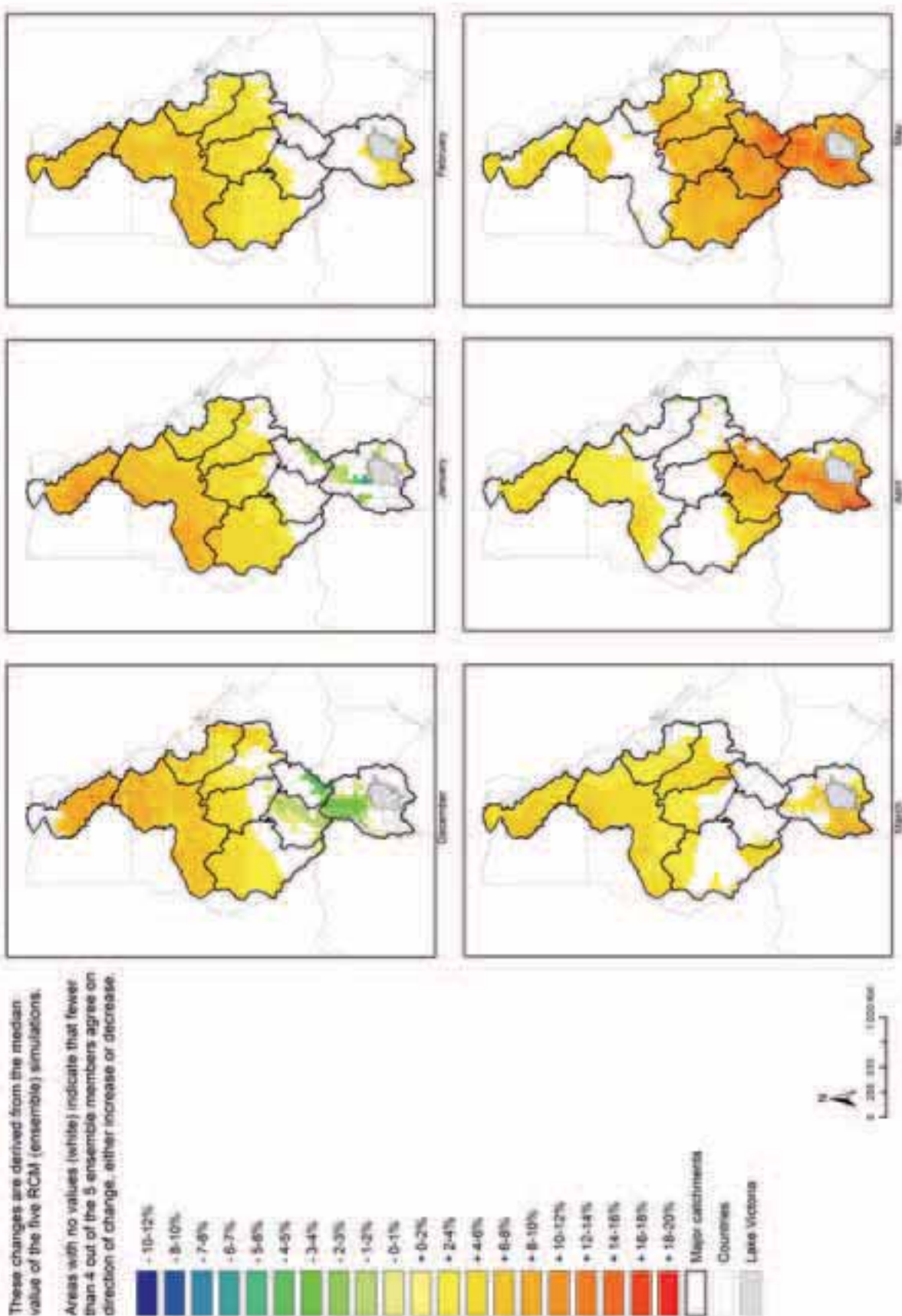
Figure 6.20 Relative change in monthly PET: 2020-2049, December to May
