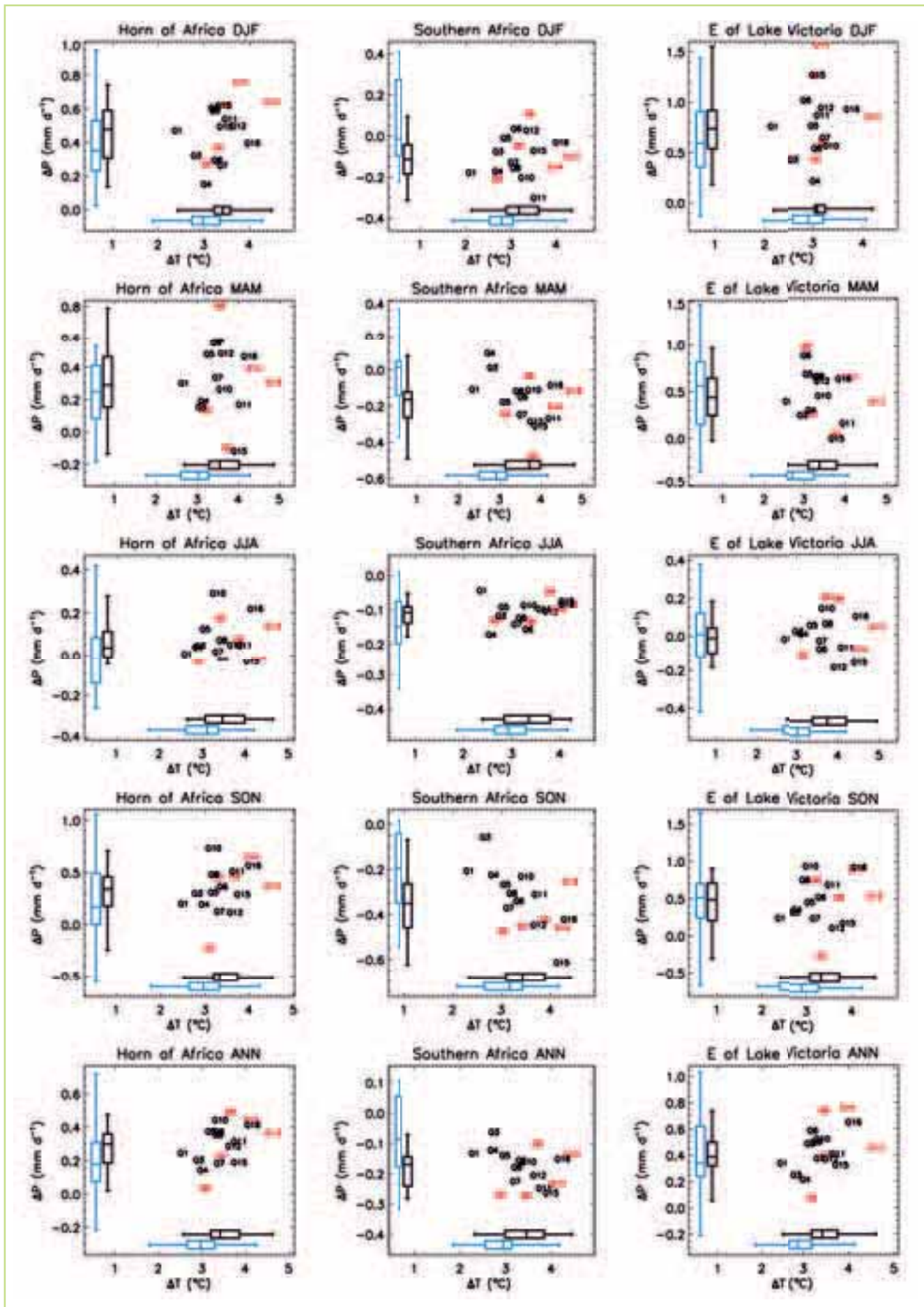
Figure 3.13 Plots for the QUMP ensemble showing projected change in precipitation versus change in the temperature for Horn of Africa, Southern Africa & East of Lake Victoria. The panels show the spread in projected outcomes during DJF, MAM, JJA, SON & annual (ANN). The data point labels (Q#) identify the models & the red data points indicate the selected sample
