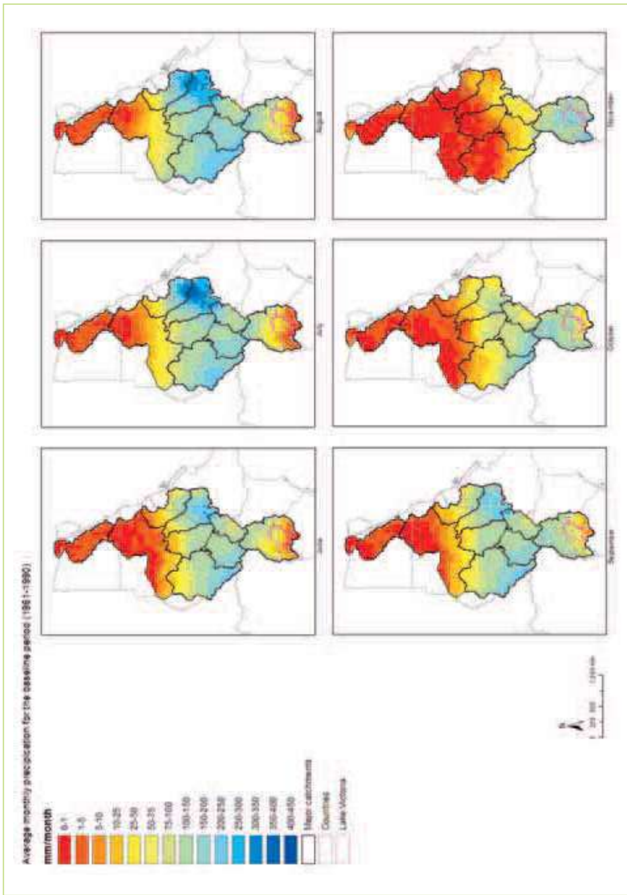
Figure 6.11 Average monthly precipitation for baseline period: 1961-1990, from CRU, June to November
