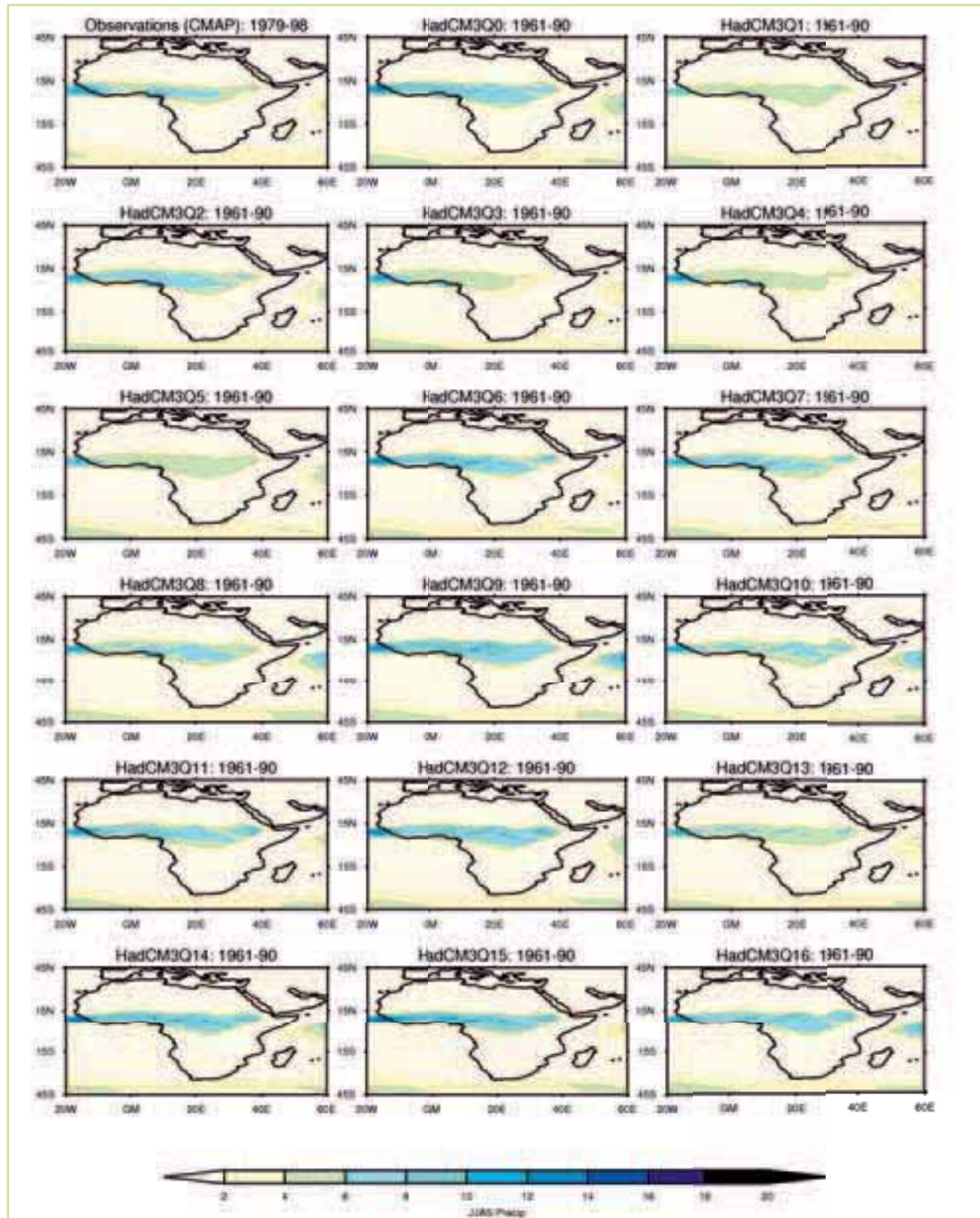
Figure 3.8 Comparison of the observed (CMAP) & simulated precipitation for Africa during JJAS. The observations were taken during the period 1979-1998 & the simulation data during the period 1961-1990. All values are in mm/d
