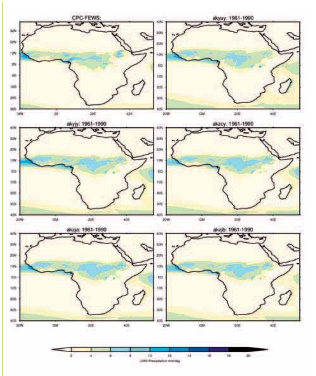
Figure 3.18 Comparison of the observed & simulated precipitation for Africa during JJAS. The observations cover the period 1983-2012 (CPC-FEWS) while the simulations cover the 1961-1990 period. All values are in mm/day
