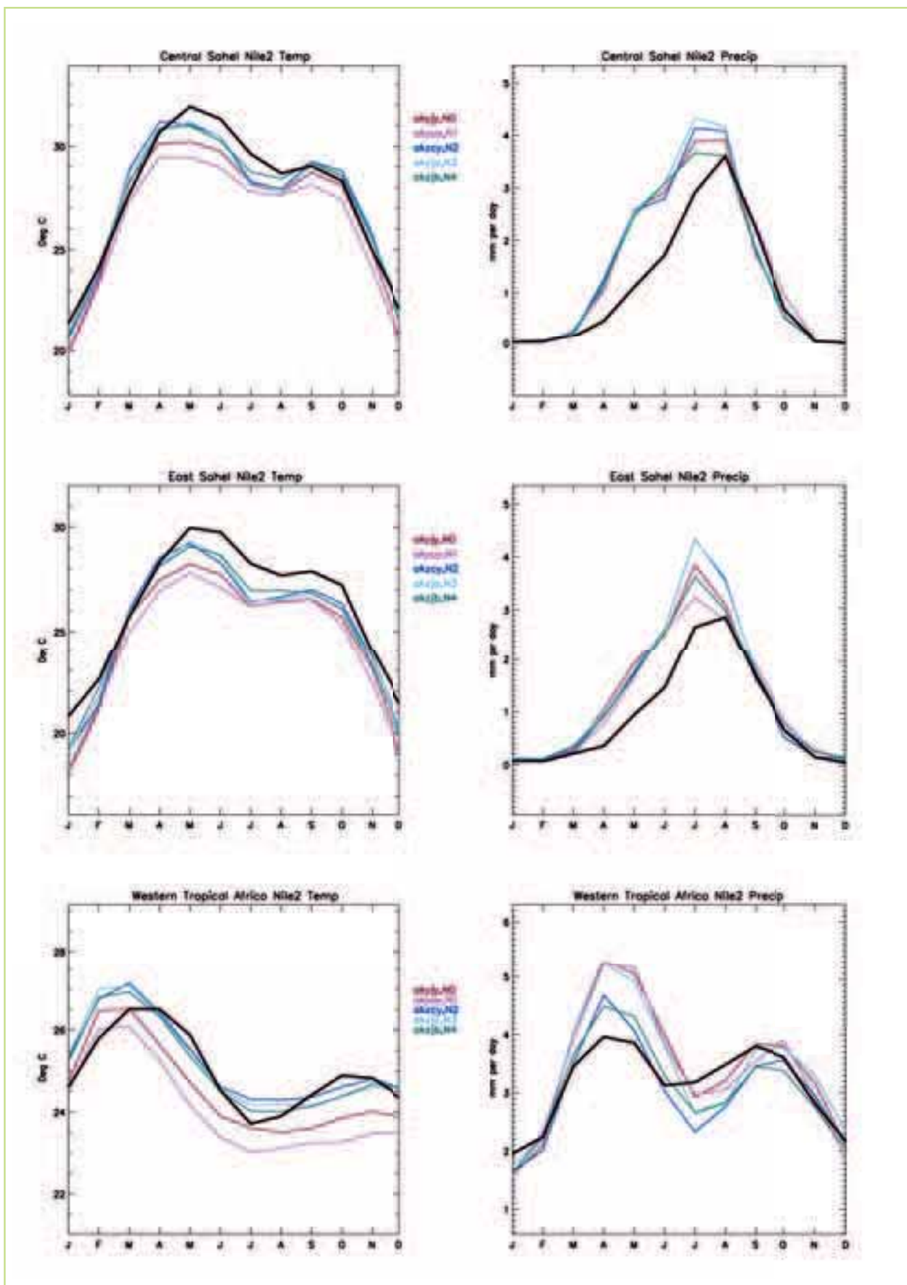
Figure 3.16 The annual variation in temperature (left) & precipitation (right) for central Sahel, East Sahel & Western Tropical Africa. The black lines show the observed values of temperature & precipitation from CRU 3.0 & CMAP, respectively, while the coloured lines show the selected RCM ensemble member simulations
