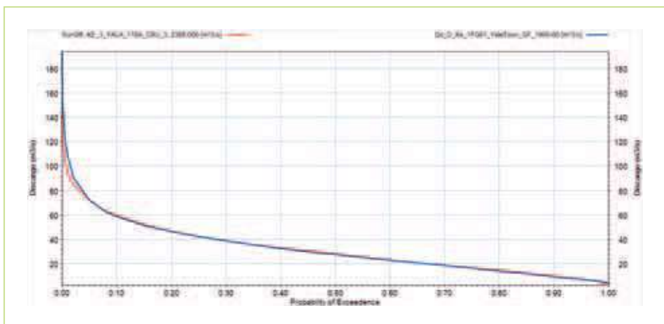
Figure 5.13 Comparison between flow duration curves for simulated (red) & observed discharge (blue) for KE03 – Yala for the period 1960-80. It has been possible to obtain a reasonable reproduction of the flows throughout the flow regime except for some minor differences for the very high flows where the uncertainty related to the observed flows are substantial
