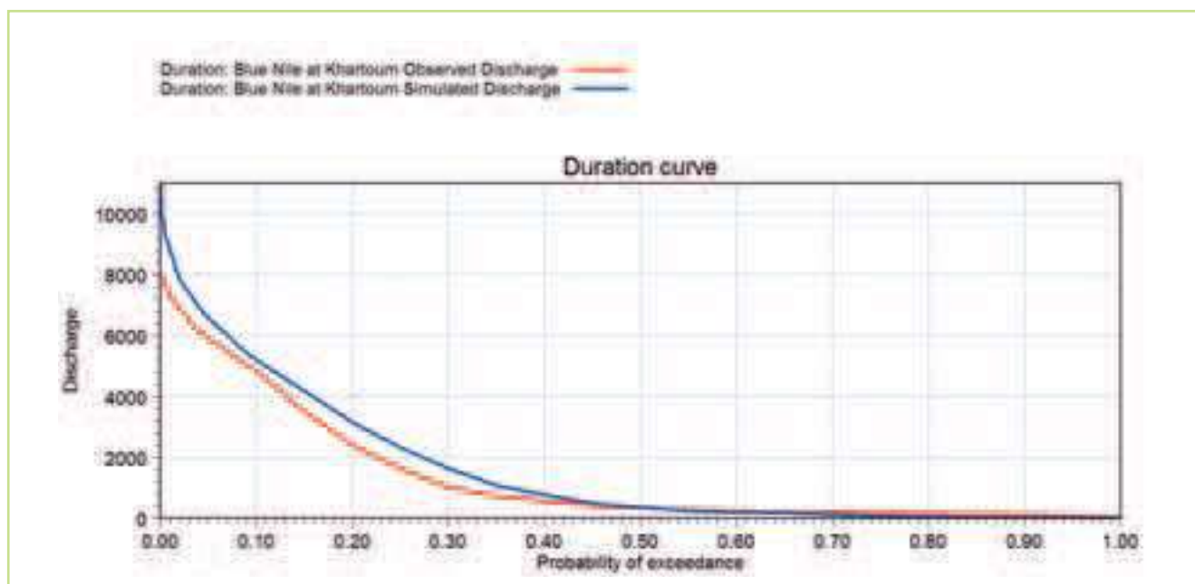
Figure 5.85 Comparison of the observed (red) & simulated (blue) flow duration curves at the Khartoum station for the period 1960-1980.
