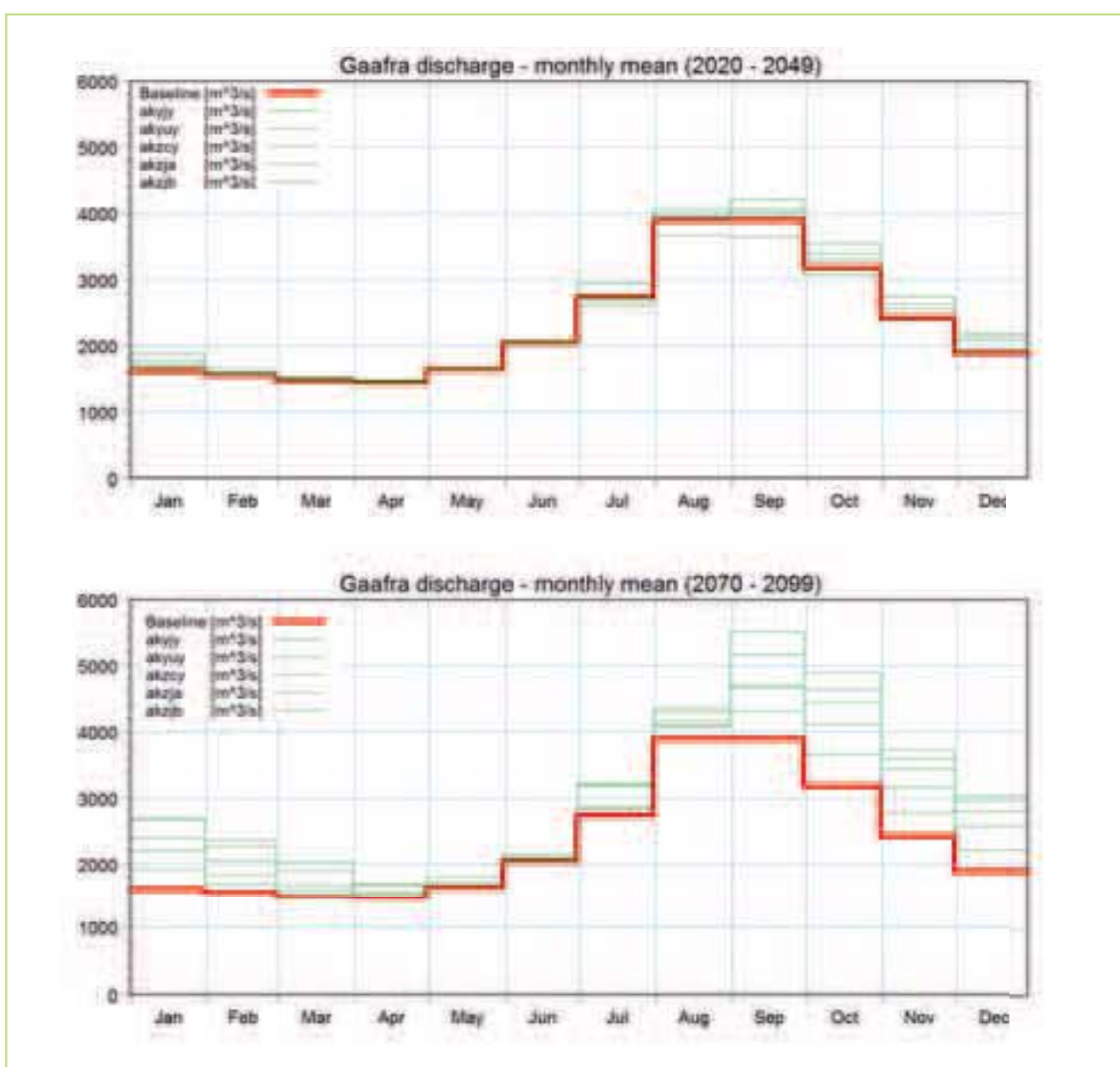
Figure 7.12 Projected changes in the average monthly flows for the Gaafra (El-Ga'Afra) station for the two periods; 2020-2049 & 2070-2099. The solid (red) line shows the baseline levels (1961-1990) & the thin green lines the different RCM ensemble members
