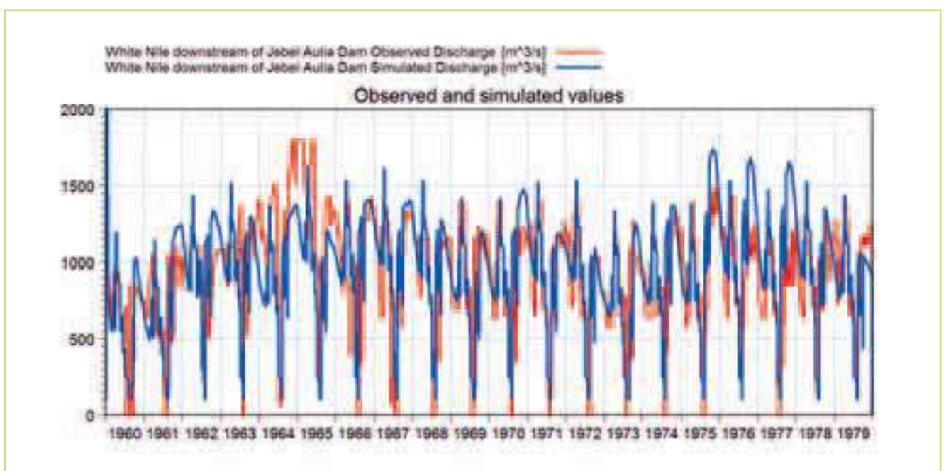
Figure 5.77 Comparison of the observed (red) & simulated (blue) flow hydrographs at the Jebel Aulia station for the period 1960-1980
