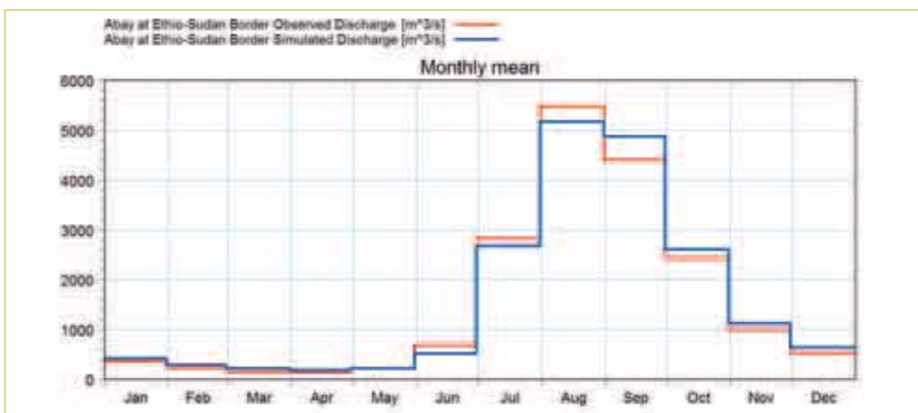
Figure 5.81 Comparison of the observed (red) & simulated (blue) mean monthly flows at the Abay station for the period 1960-1980
