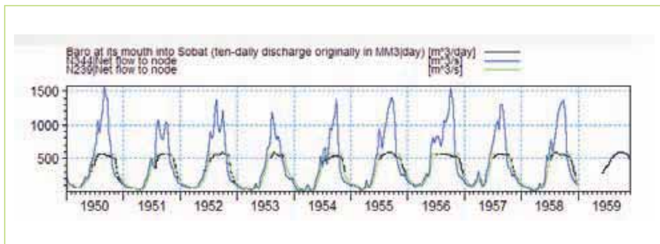
Figure 5.34 Observed flow at Gambeila (blue line), observed flow at the outlet to the Sobat river (black line) & the simulated flow at the outlet to the Sobat (green line)
