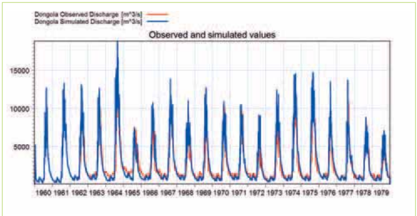
Figure 5.89 Comparison of the observed (red) & simulated (blue) flow hydrographs at the Dongola station for the period 1960-1980
