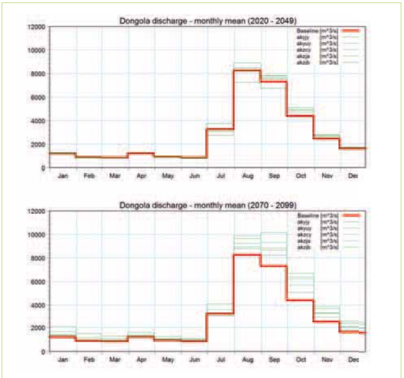
Figure 8.4 Projected changes in the average monthly flows for the Dongola station for the two periods; 2020-2049 & 2070-2099. The solid (red) line shows the baseline levels (1961-1990) & the thin green lines the different RCM ensemble members
