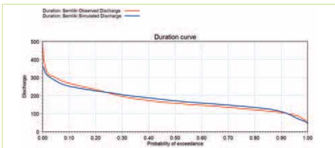
Figure 5.53 Comparison of the observed (red) & simulated (blue) flow duration curves at the Semliki station for the period 1960-1980
