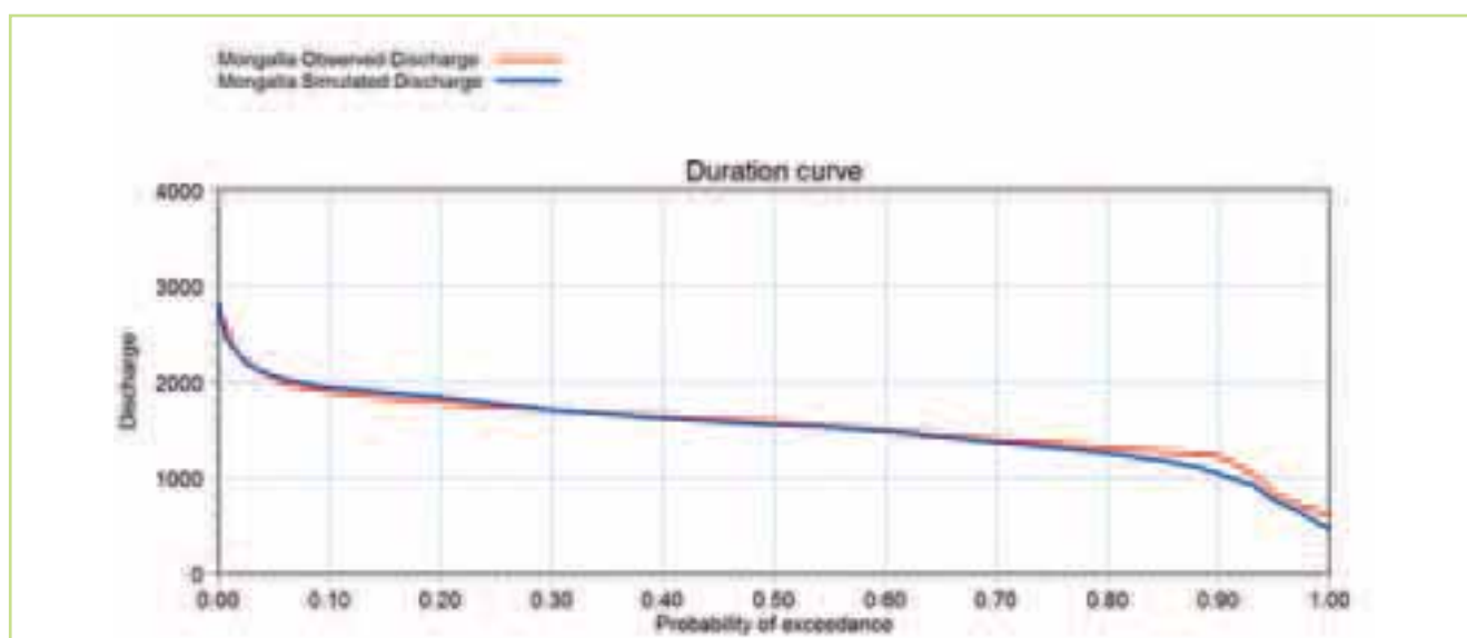
Figure 5.66 Comparison of the observed (red) & simulated (blue) flow duration curves at the Mongalla station for the period 1960-1980
