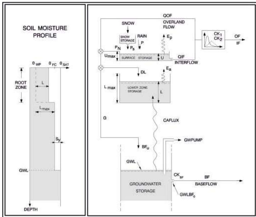
Figure 5.2 The conceptual model structure of the NAM model
