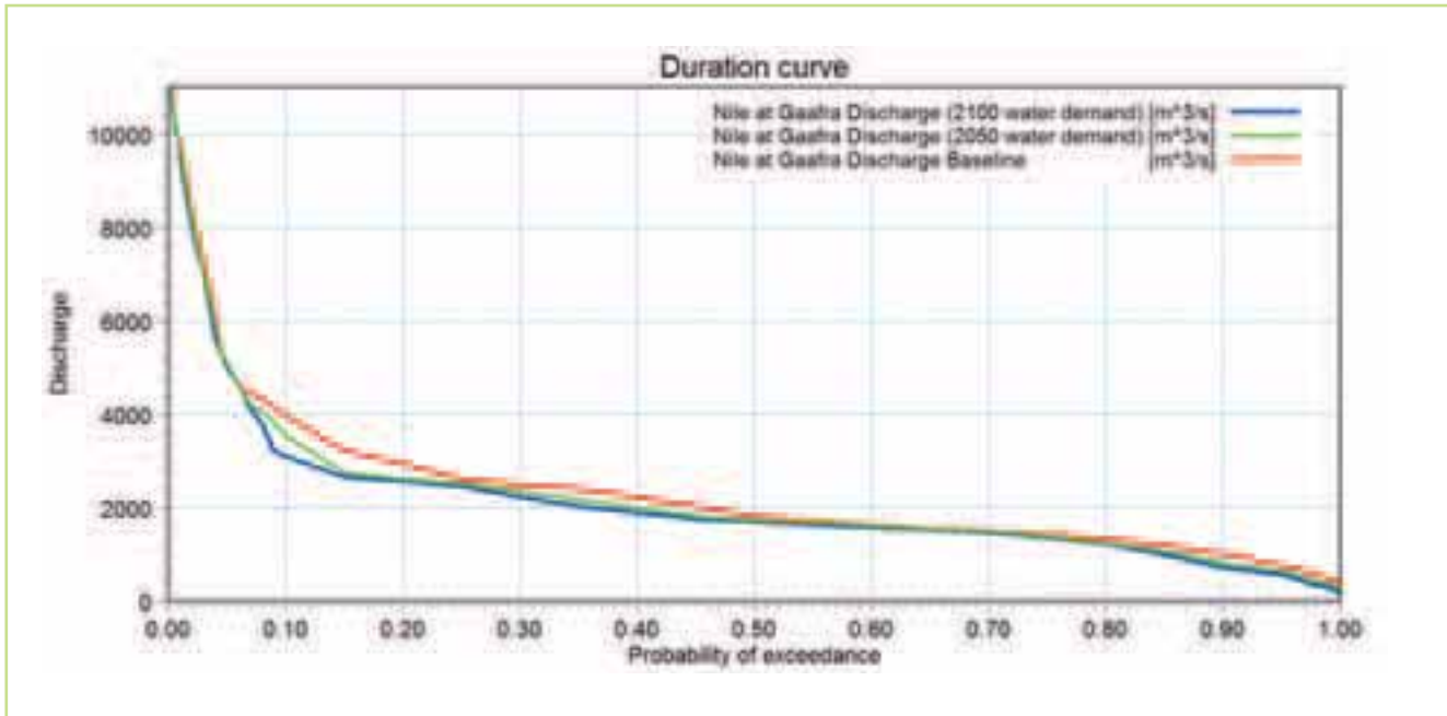
Figure 7.14 Changes in the flow duration curve for the Nile at Gafra (El-Ga'afra) from baseline (red), 2050 (green) & 2100 (blue)
