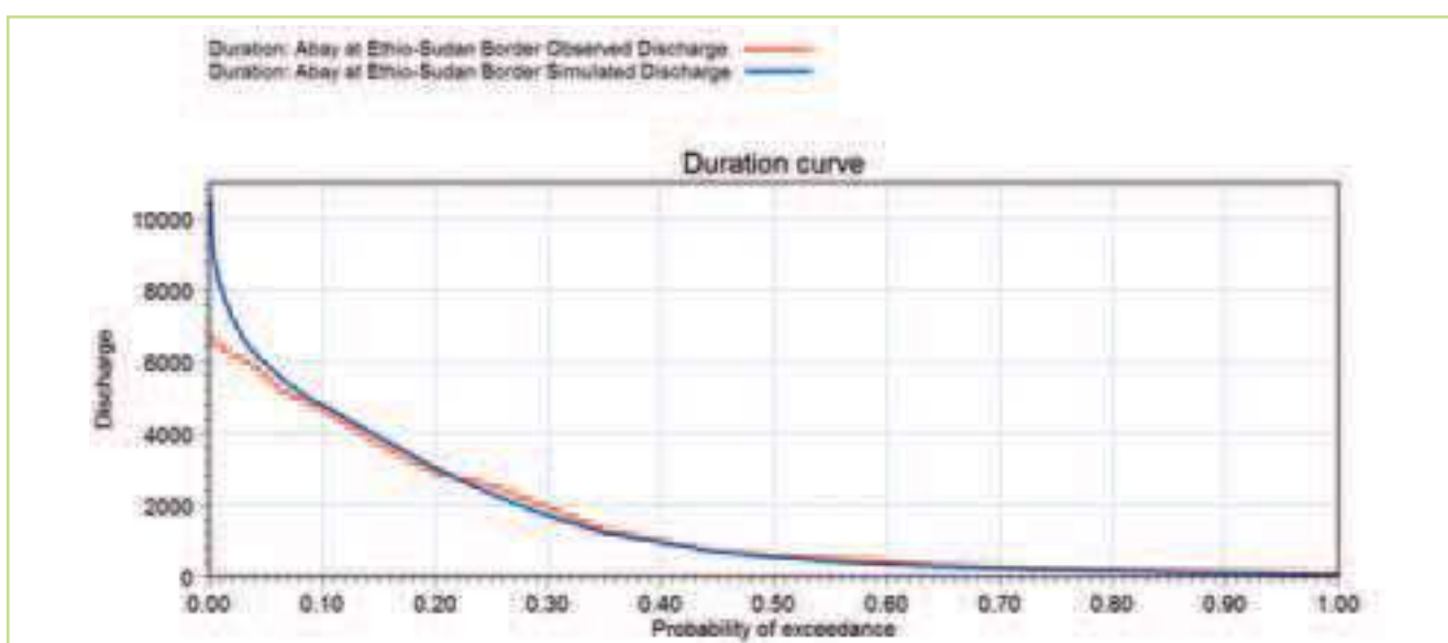
Figure 5.82 Comparison of the observed (red) & simulated (blue) flow duration curves at the Abay station for the period 1960-1980
