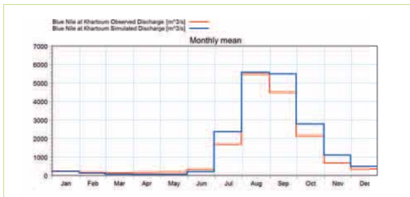
Figure 5.84 Comparison of the observed (red) & simulated (blue) mean monthly flows at the Khartoum station for the period 1960-1980
