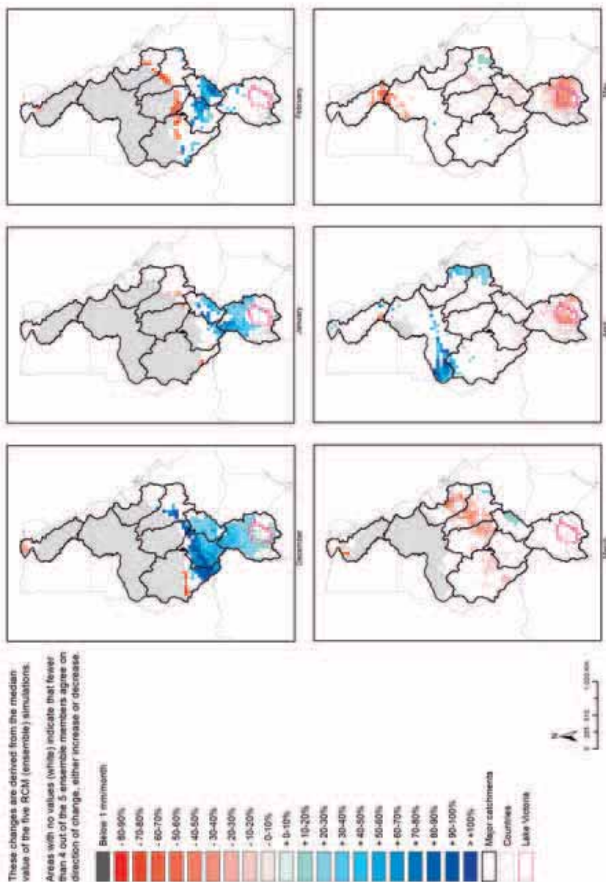
Figure 6.16 Relative change in monthly precipitation: 2020-2049, December to May
