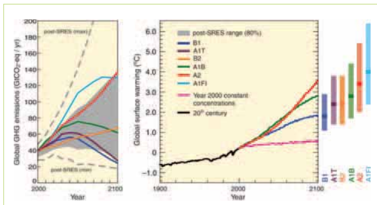
Figure 3.1 The range of global greenhouse gas emissions (left) & corresponding global warming (right) for different SRES scenarios. The bars on the right show the likely range of temperature increase in 2100 (relative to the period 1980-1999). Source: IPCC AR 4 report ( http://www.ipcc.ch/publications_and_data/ar4/syr/en/contents.html )
