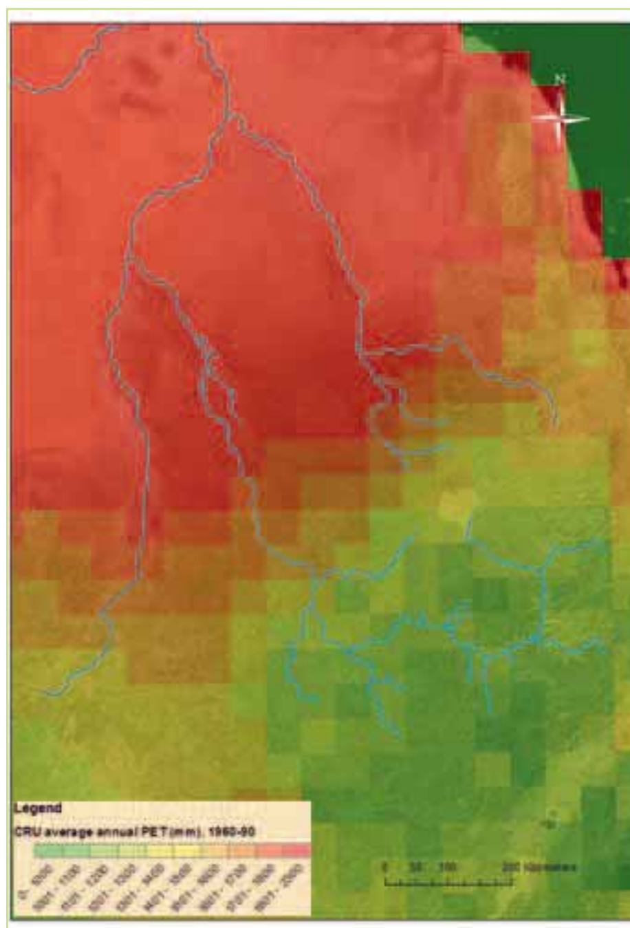
Figure 5.40 Spatial distribution of average annual PET (1960-90) for the Blue Nile & Atbara sub-basins from the CRU gridded dataset
