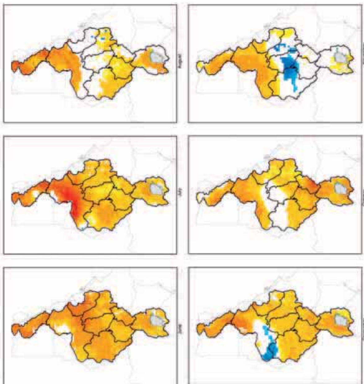
Figure 6.23 Absolute change in monthly PET: 2020-2049, June to November. Note that CRU baseline PET values are given as zero over Lake Victoria.
