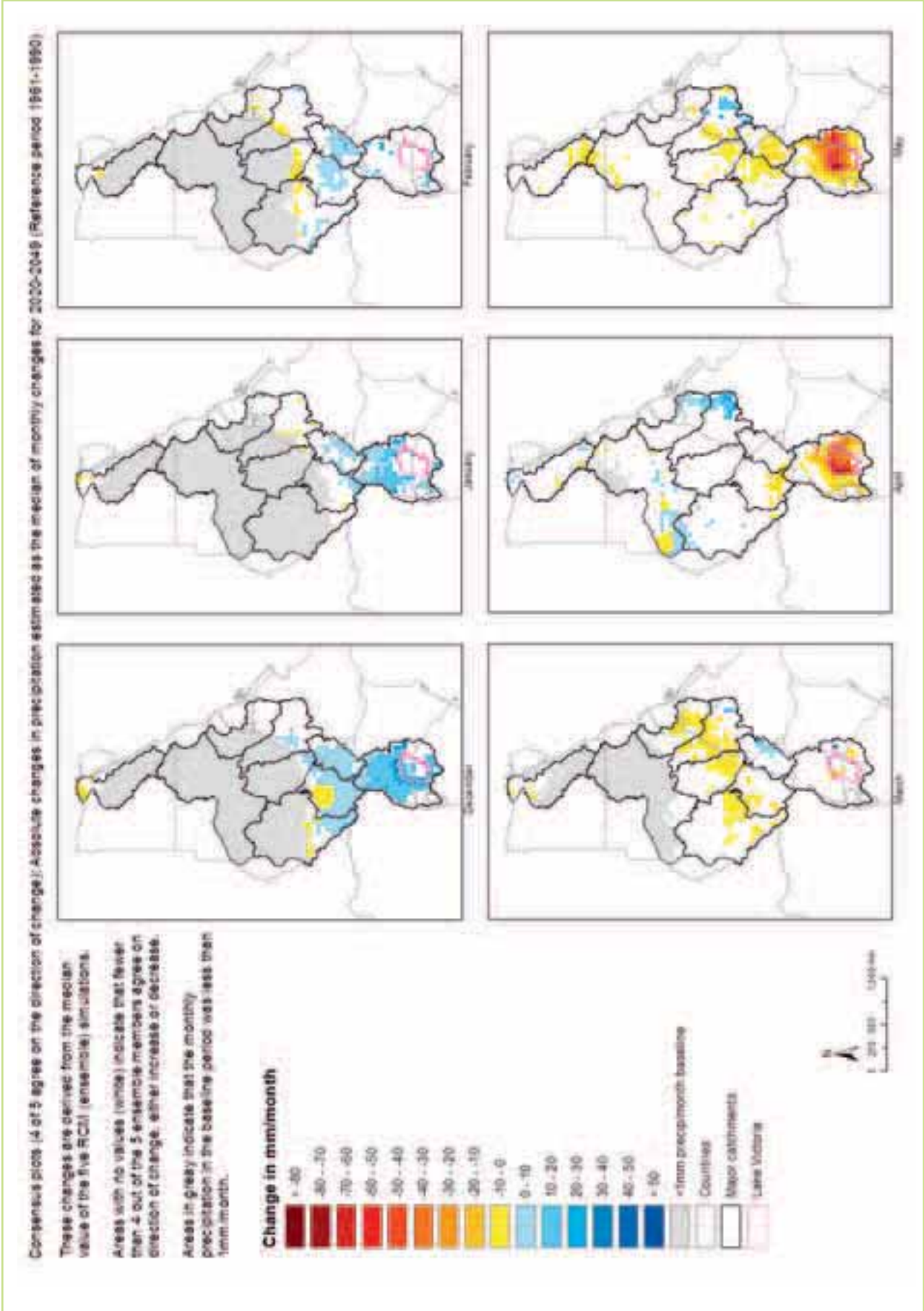
Figure 6.18 Absolute changes in monthly precipitation: 2020-2049, December to May
