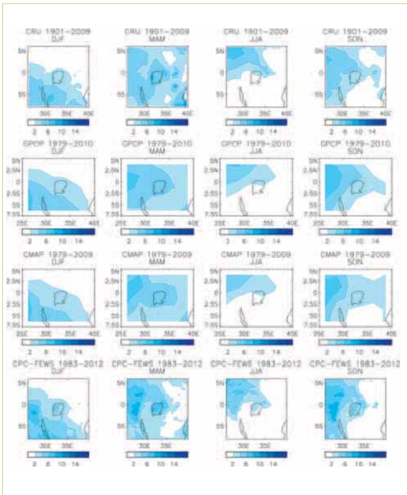
Figure 3.20 Daily precipitation averaged over each season over Africa (mm/day) for four observational datasets 1) CRU, 2) GPCP, 3) CMAP & 4) CPC-FEWS
