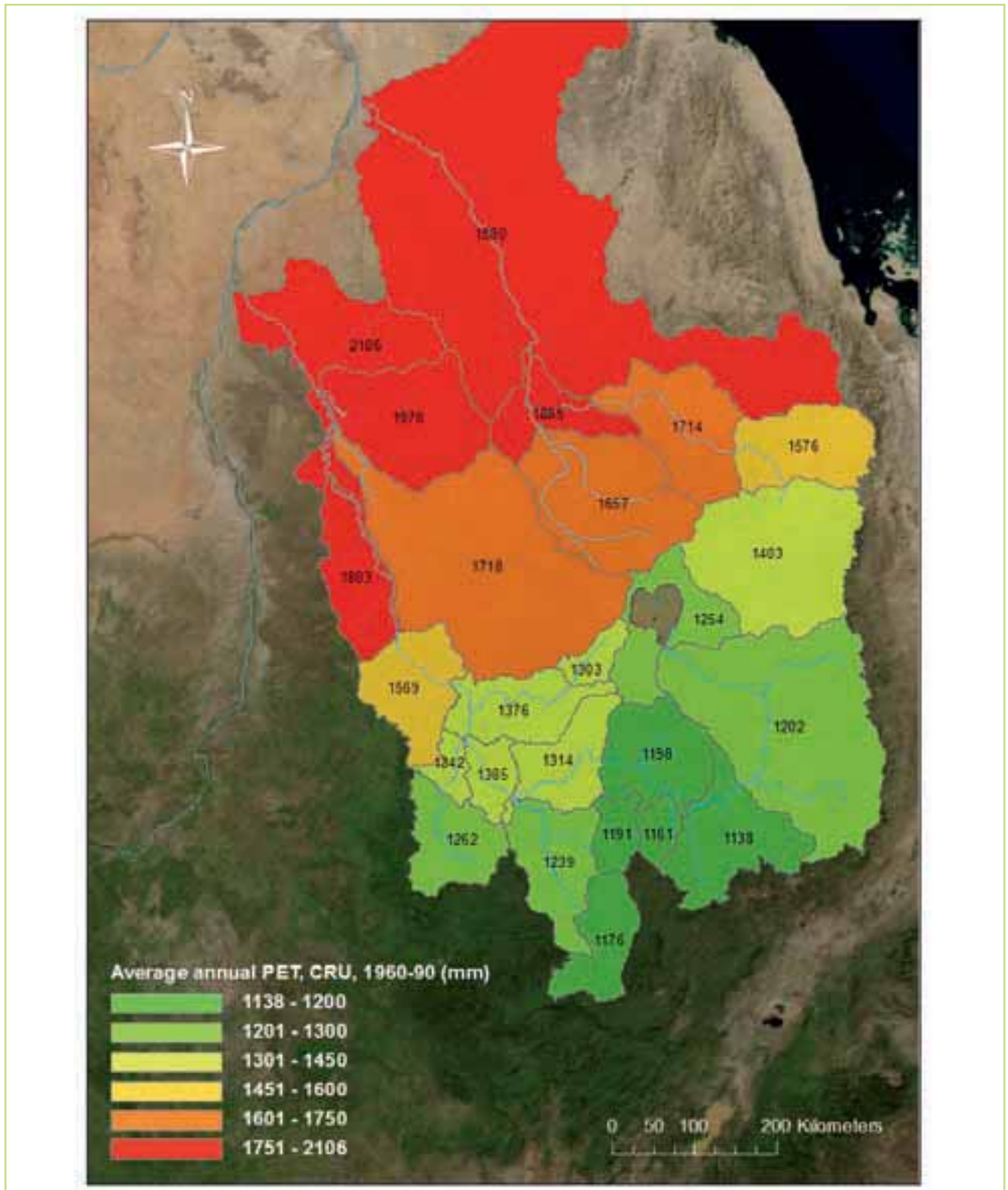
Figure 5.43 Average annual PET estimated from CRU data set, 1960-90
