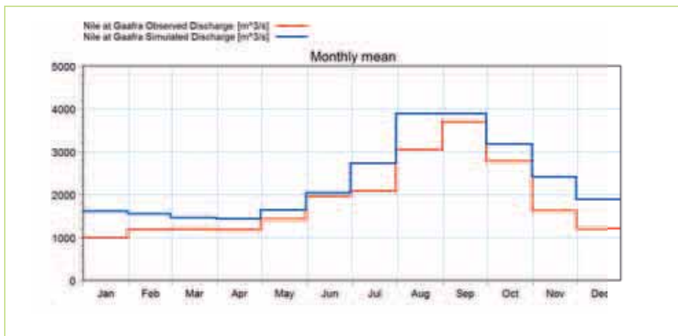
Figure 5.93 Comparison of the observed (red) & simulated (blue) mean monthly flows at the Abay station for the period 1960-1980
