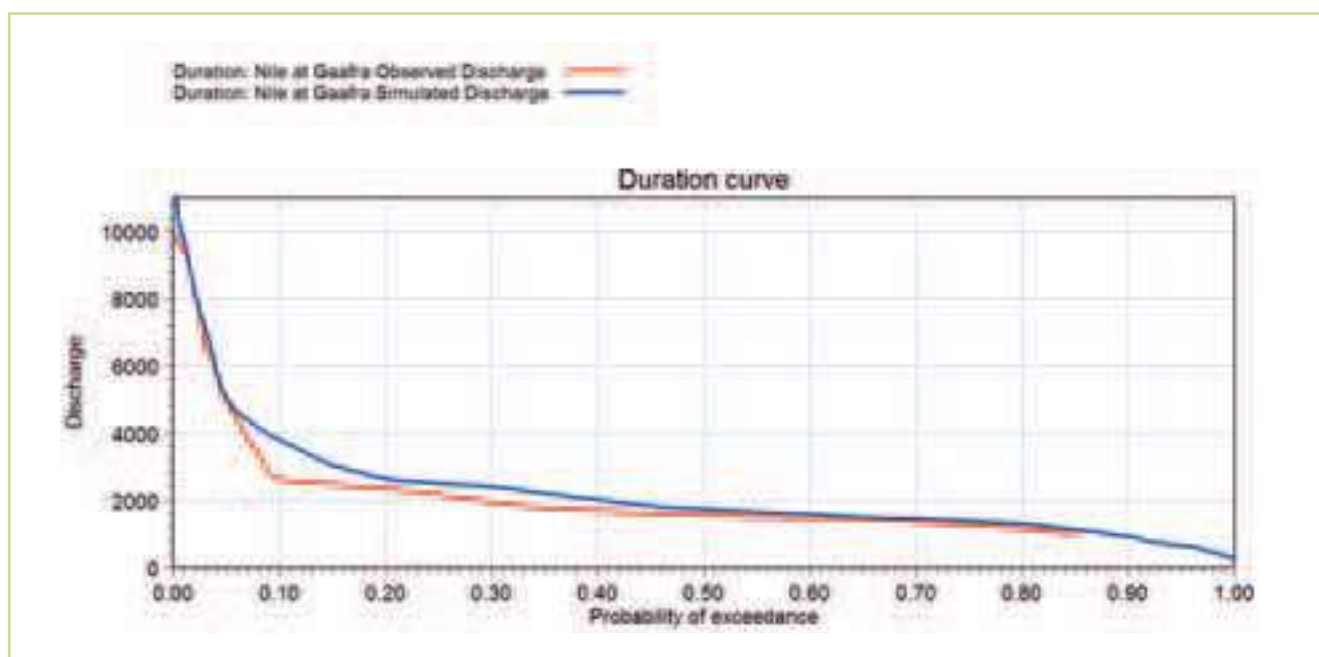
Figure 5.94 Comparison of the observed (red) & simulated (blue) flow duration curves at the Abay station for the period 1960-1980
