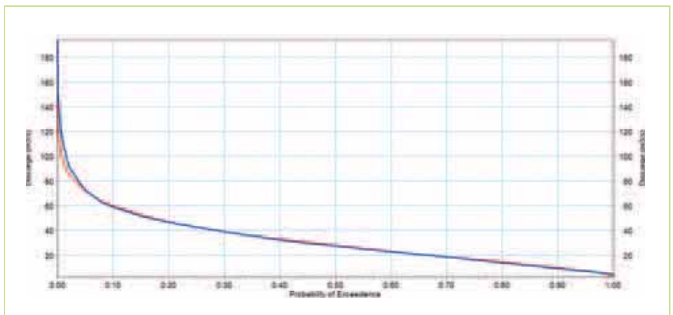
Figure 5.9 Example of calibration plot with duration curve from the Yala catchment in the Lake Victoria basin. Comparison of flow duration curves for the observed (blue) & simulated (red) discharge for KE03 – Yala for the period 1960-1979. There is reasonable reproduction of flows throughout the flow regime except for minor differences for very high flows where the uncertainty in observed flows is expected to be high
