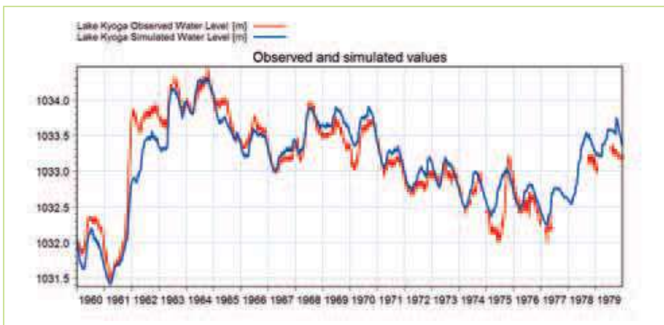
Figure 5.56 Comparison of the observed (red) & simulated (blue) water level hydrographs at the Lake Kyoga station for the period 1960-1980
