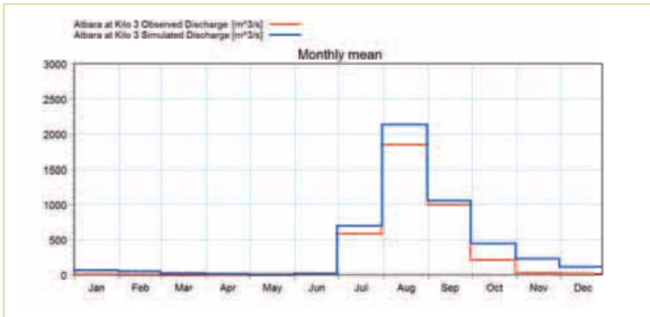
Figure 5.87 Comparison of the observed (red) & simulated (blue) mean monthly flows at the Atbara station for the period 1960-1980
