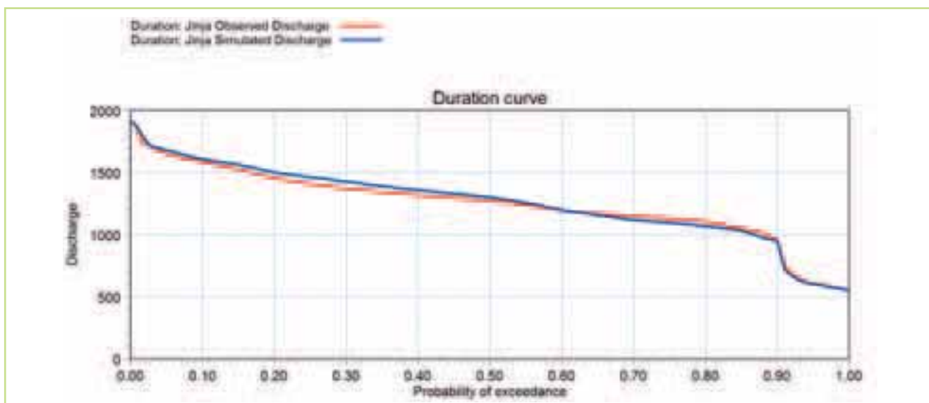
Figure 5.60 Comparison of the observed (red) & simulated (blue) flow duration curves at the Jinja station for the period 1960-1980
