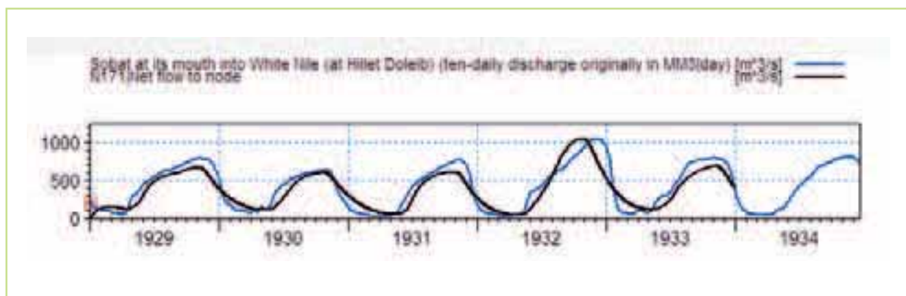
Figure 5.35 Simulated (black line) & observed (blue line) from Sobat river (at the outlet to the White Nile)
