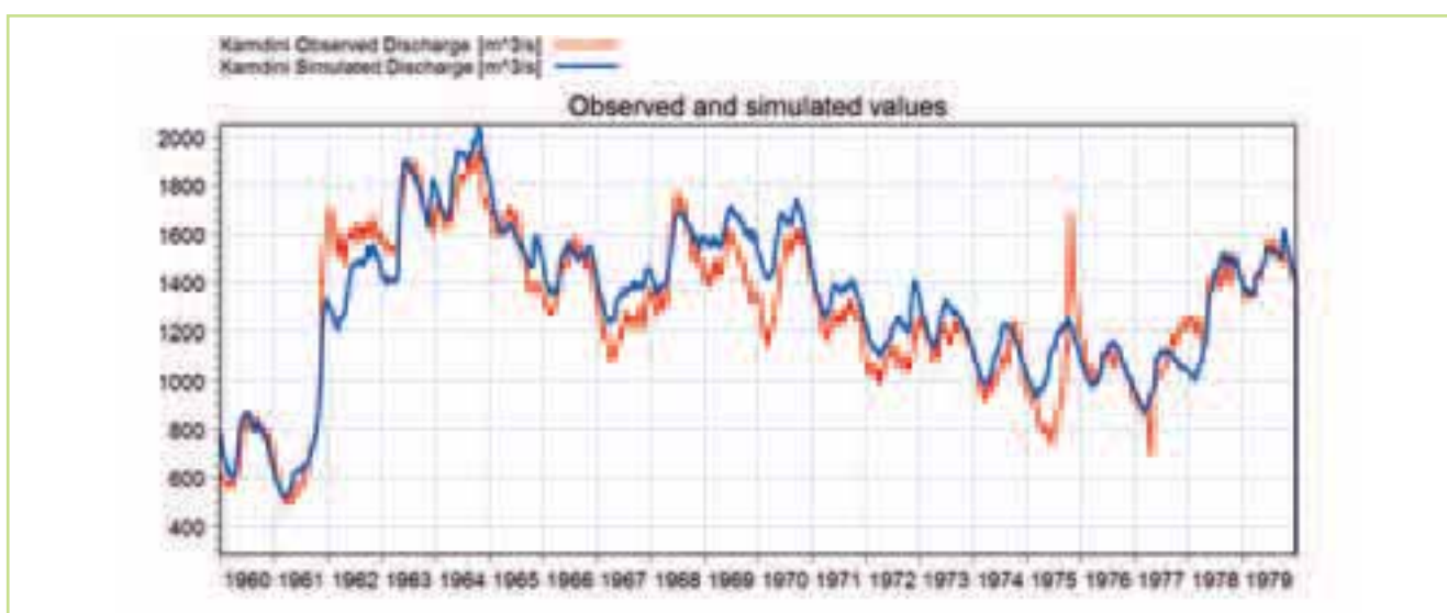
Figure 5.61 Comparison of the observed (red) and simulated (blue) flow hydrographs at the Kamdini station for the period 1960-1980
