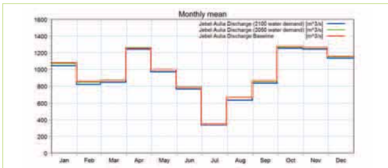
Figure 7.3 Mean monthly discharges for the Jebel Aulia gauge for baseline, 2050 & 2100 water demands
