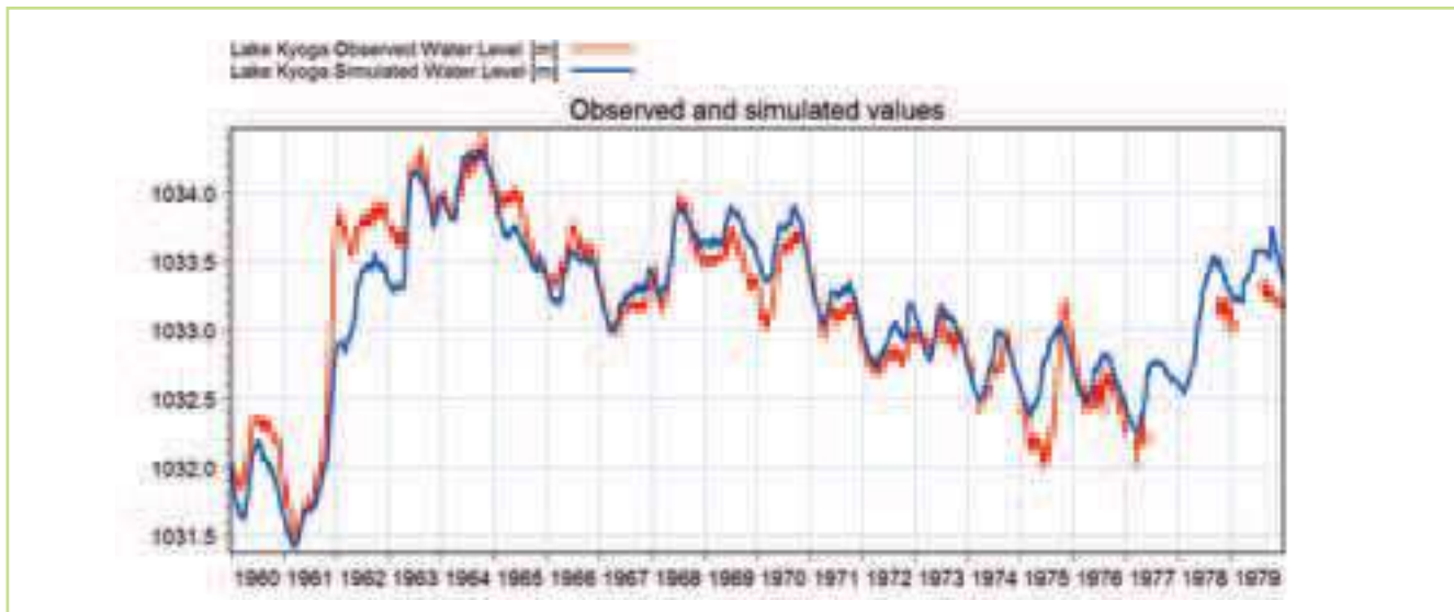
Figure 5.20 Comparison between observed (red) & simulated (blue) water levels at Lake Kyoga for the modelling period 1960-80
