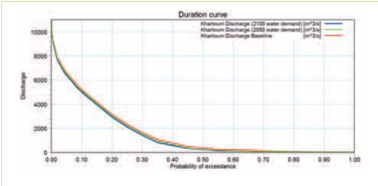
Figure 7.13 Changes in the flow duration curve at Khartoum from baseline (red), 2050 (green) & 2100 (blue)
