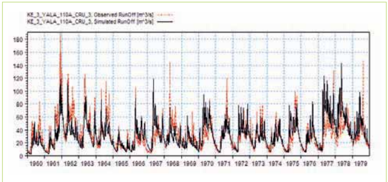
Figure 5.8 Example of calibration plot from the Yala catchment in the Lake Victoria Basin. Comparison of the observed (red) & simulated (black) discharge for the KE03 - Yala catchment for the period 1960-1979. It is possible to obtain a consistent calibration throughout the 20 year period indicating good data quality
