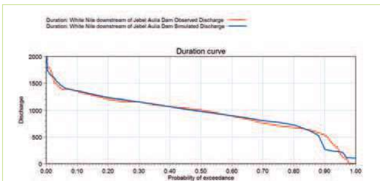
Figure 5.79 Comparison of the observed (red) & simulated (blue) flow duration curves at the Jebel Aulia station for the period 1960-1980
