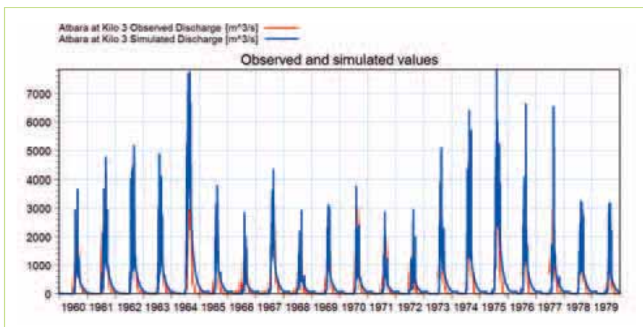
Figure 5.86 Comparison of the observed (red) & simulated (blue) flow hydrographs at the Atbara station for the period 1960-1980
