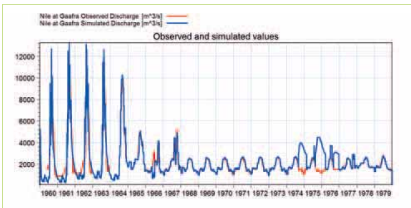
Figure 5.92 Comparison of the observed (red) & simulated (blue) flow hydrographs at the Gaafra station for the period 1960-1980
