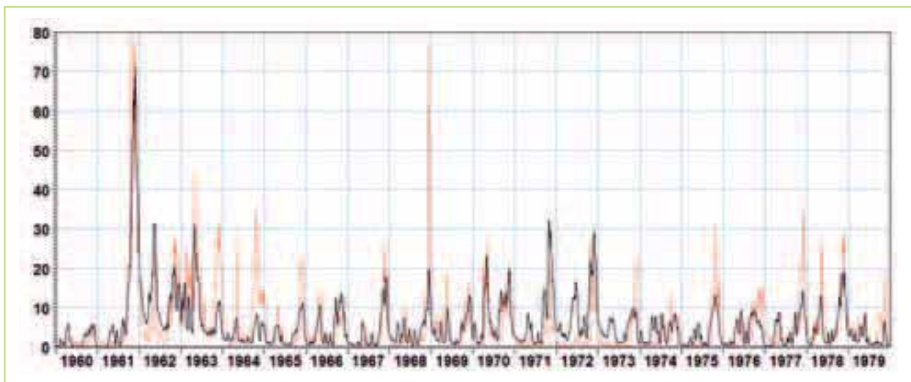
Figure 5.16 Comparison between simulated (black) & observed discharge (red) for UG13_85211_Muzizi for the period 1960-1980
