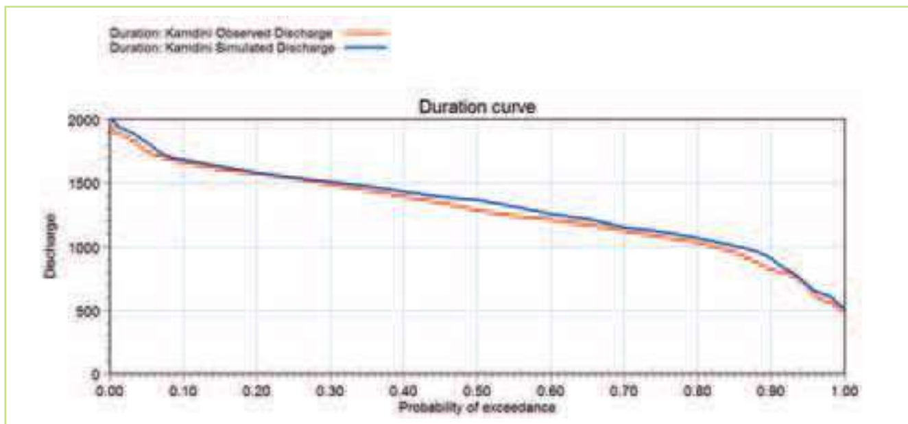
Figure 5.63 Comparison of the observed (red) & simulated (blue) flow duration curves at the Kamdini station for the period 1960-1980
