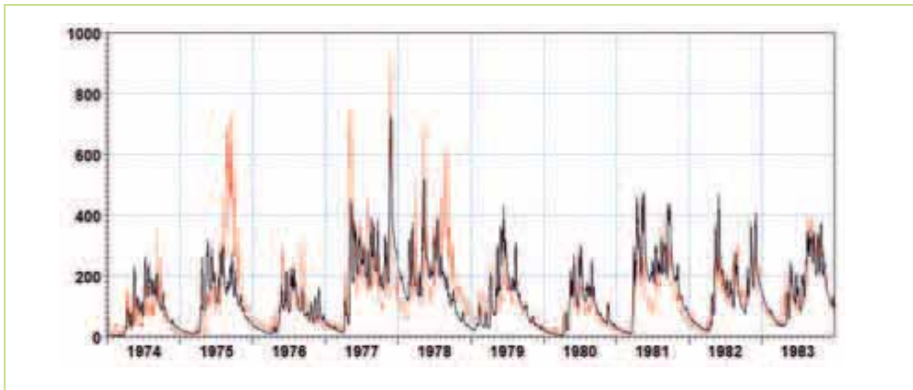
Figure 5.14 Comparison between simulated (black) & observed discharge (red) for KE02 – Nzoia for the period 1974-1983. Due to lack of observed discharge for other periods, 1974-83 was selected as the calibration period
