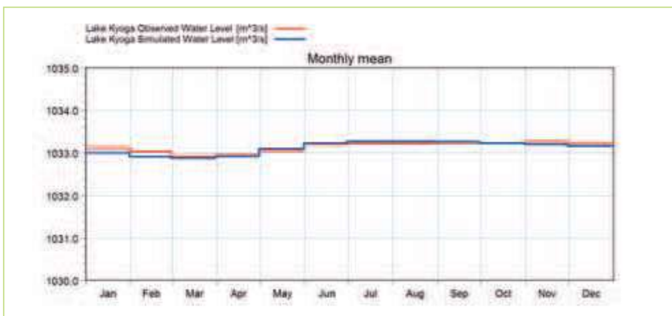
Figure 5.57 Comparison of the observed (red) & simulated (blue) mean monthly water levels at the Lake Kyoga station for the period 1960-1980
