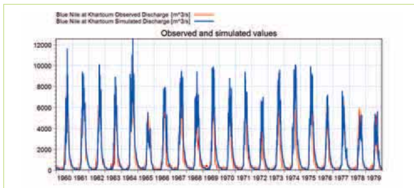
Figure 5.83 Comparison of the observed (red) & simulated (blue) flow hydrographs at the Khartoum station for the period 1960-1980
