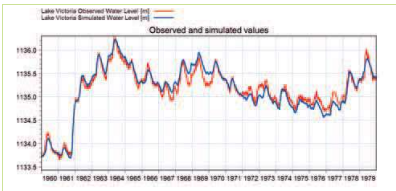
Figure 5.54 Comparison of the observed (red) & simulated (blue) water level hydrographs at the Lake Victoria station for the period 1960-1980
