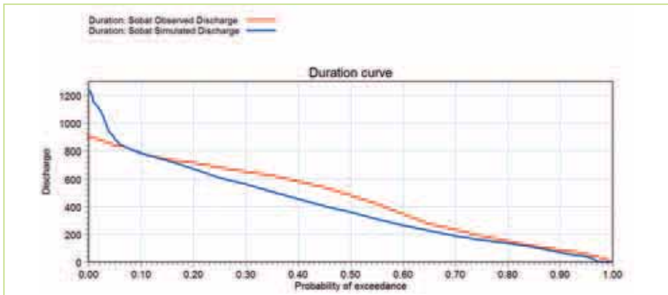
Figure 5.72 Comparison of the observed (red) & simulated (blue) flow duration curves at the Sobat station for the period 1960-1980
