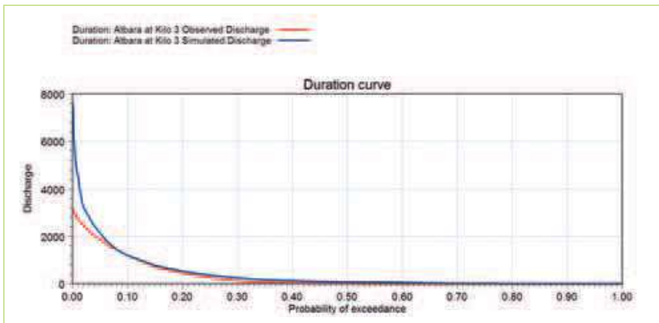
Figure 5.88 Comparison of the observed (red) & simulated (blue) flow duration curves at the Atbara station for the period 1960-1980
