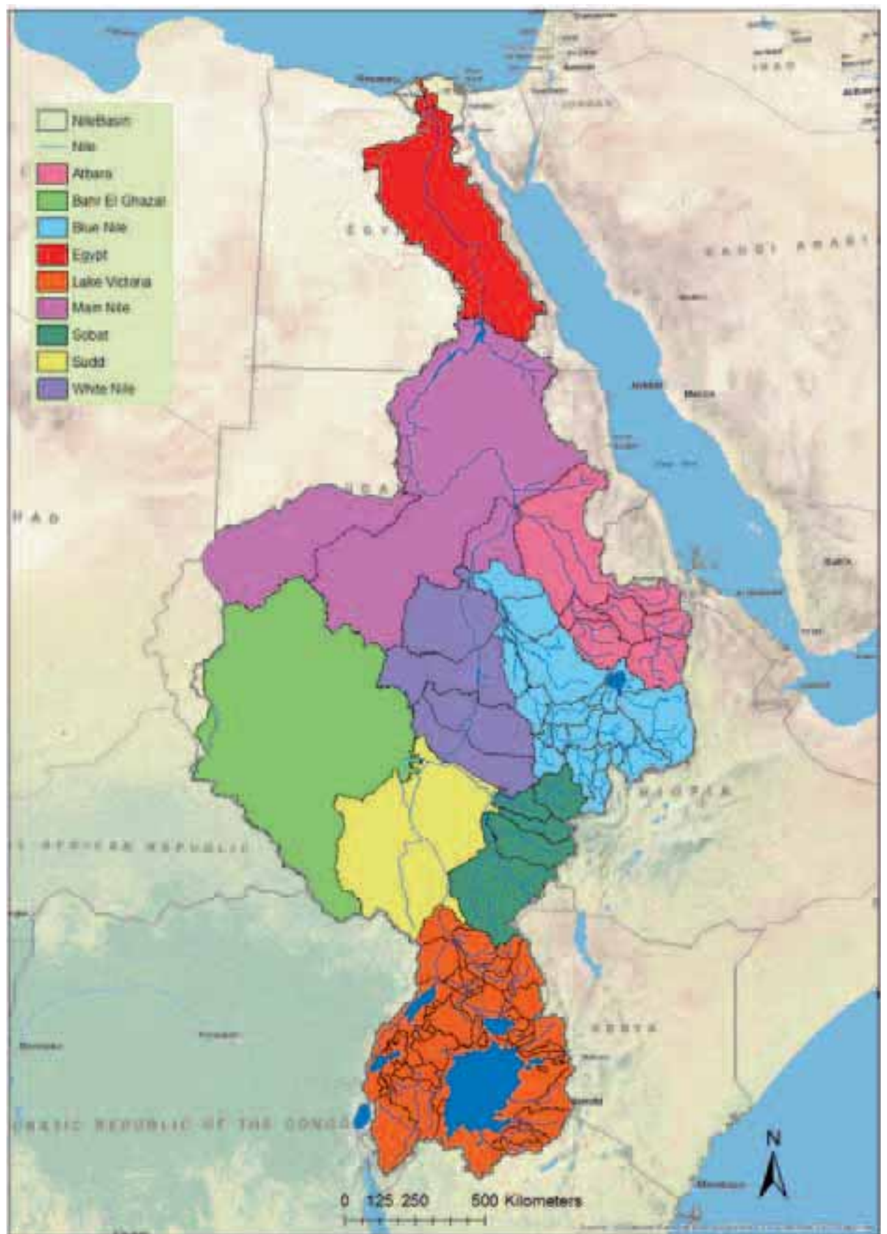
Figure 5.1 The Nile River Basin showing the major sub-basins, the minor sub-basins within each these sub-basins & showing the model river network linking the sub-basins that was used to represent the Nile river system
