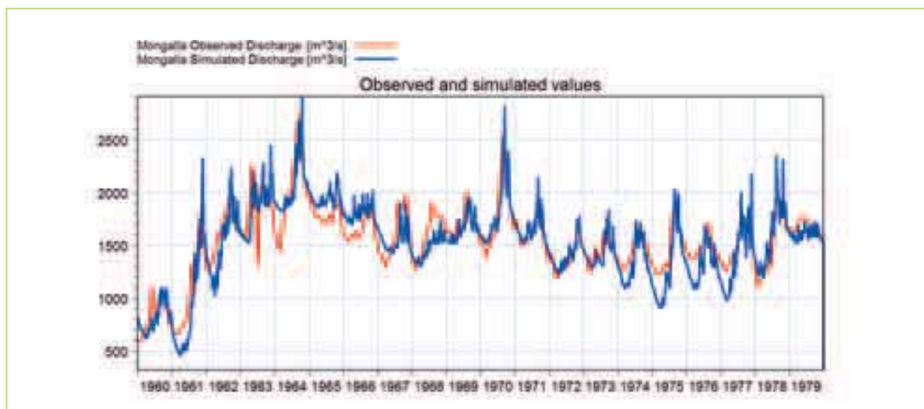
Figure 5.64 Comparison of the observed (red) & simulated (blue) flow hydrographs at the Mongalla station for the period 1960-1980
