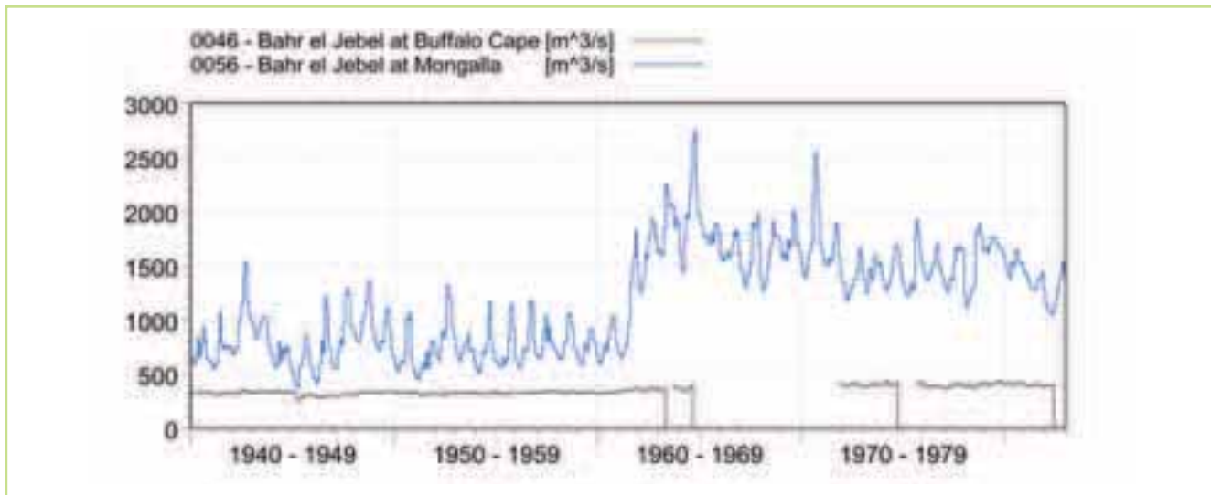
Figure 5.25 Observed discharge at Mongalla & Buffalo Cape
