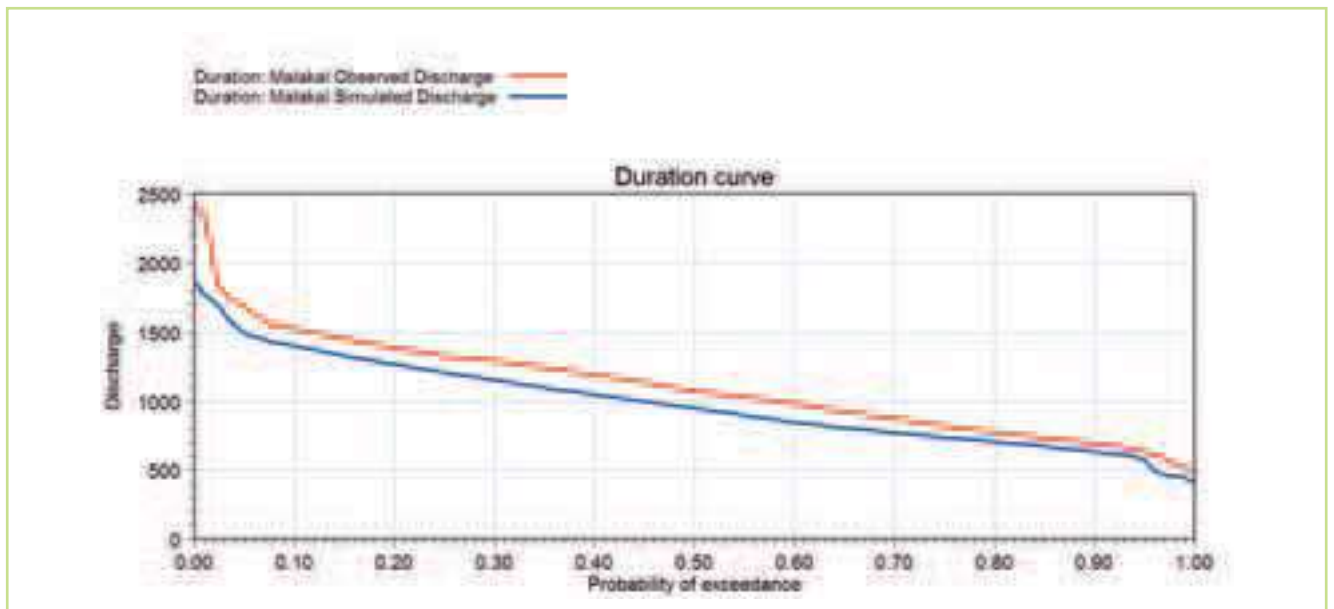
Figure 5.76 Comparison of the observed (red) & simulated (blue) flow duration curves at the Malakal station for the period 1960-1980
