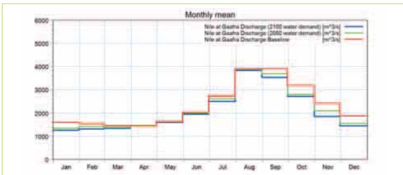
Figure 7.11 Mean monthly discharges for the Gaafra (El-Ga'Afra) gauge for baseline, 2050 & 2100 water demands
