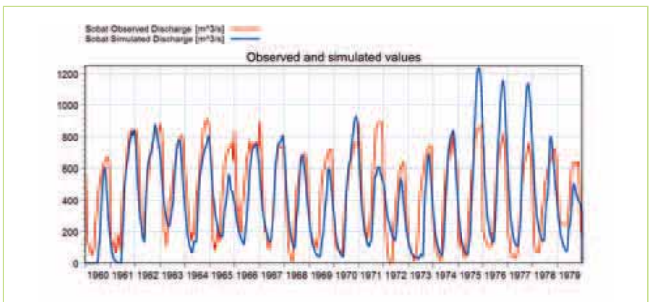
Figure 5.70 Comparison of the observed (red) & simulated (blue) flow hydrographs at the Sobat station for the period 1960-1980
