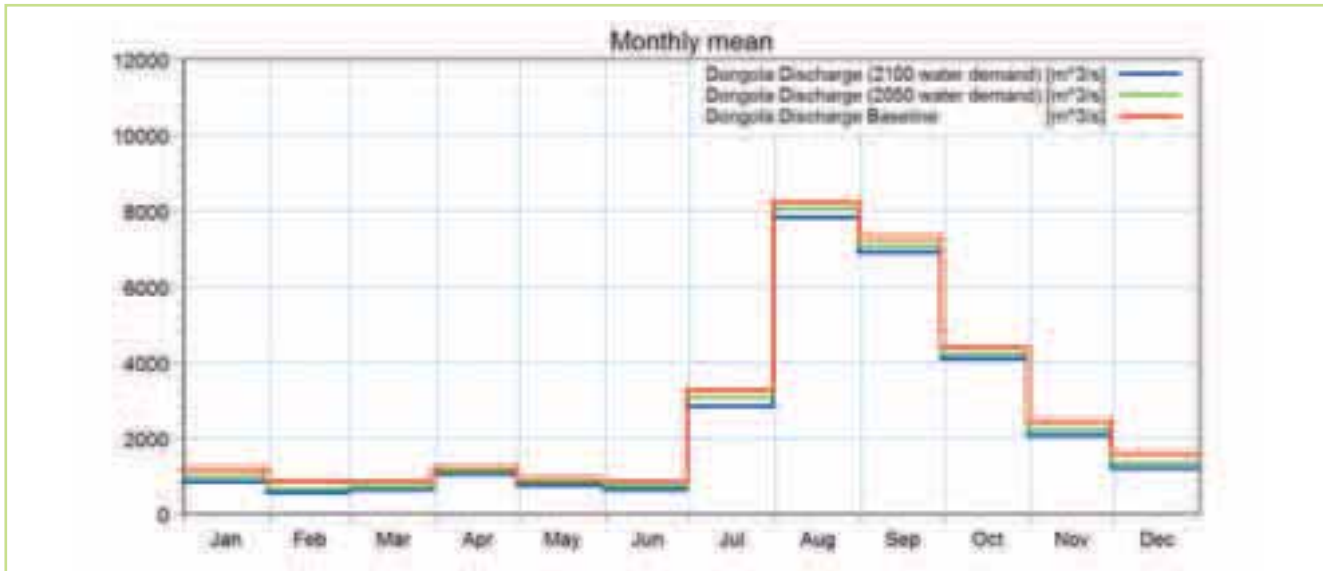
Figure 7.9 Mean monthly discharges for the Dongola gauge for baseline, 2050 & 2100 water demands
