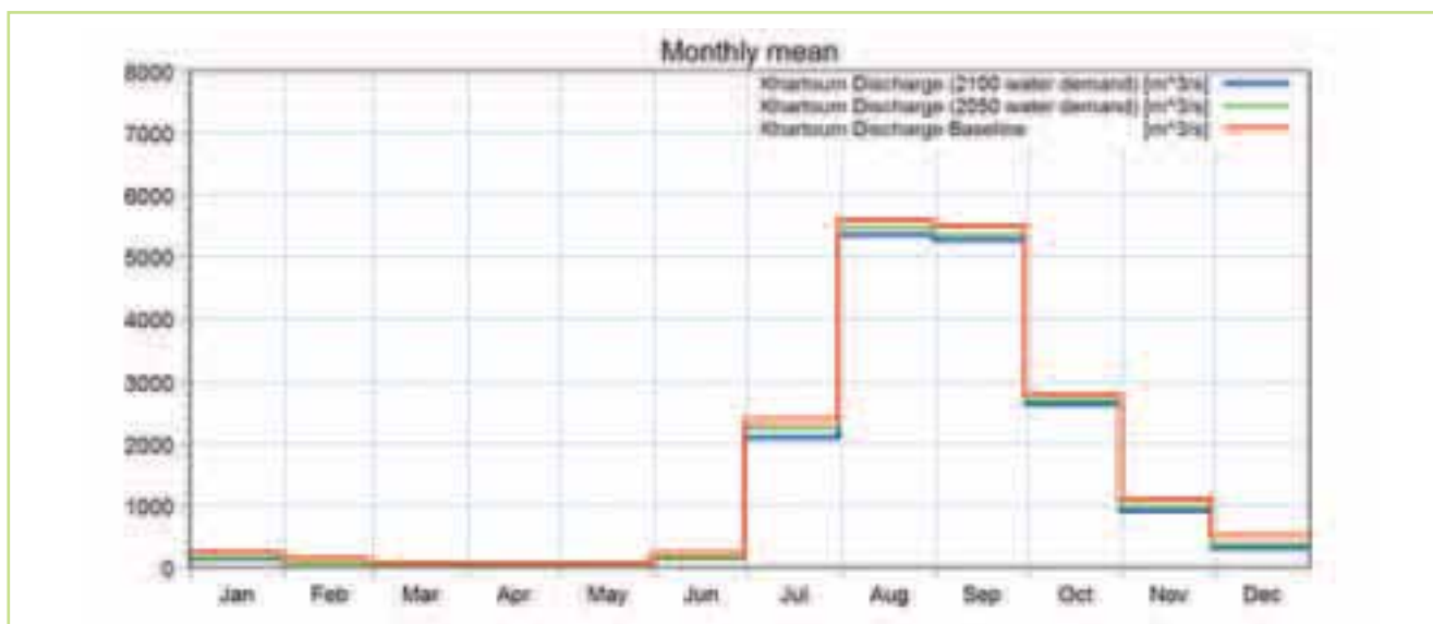
Figure 7.5 Mean monthly discharges for the Khartoum gauge for baseline, 2050 & 2100 water demands
