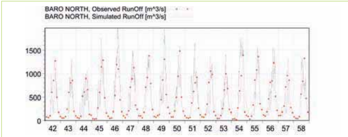
Figure 5.32 Simulated & observed runoff
