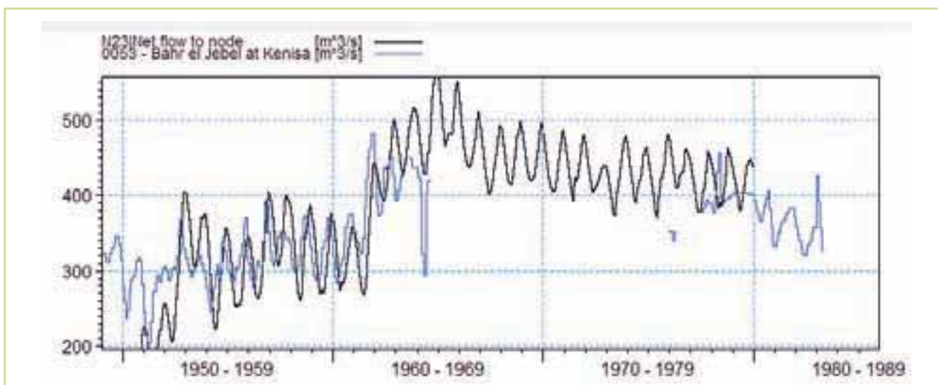
Figure 5.27 Simulated (black line) & observed (blue line) discharge at Kenisa
