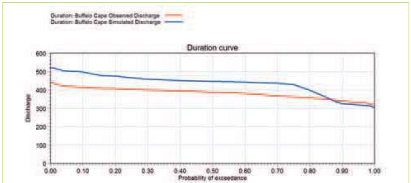
Figure 5.69 Comparison of the observed (red) & simulated (blue) flow duration curves at the Semliki station for the period 1960-1980
