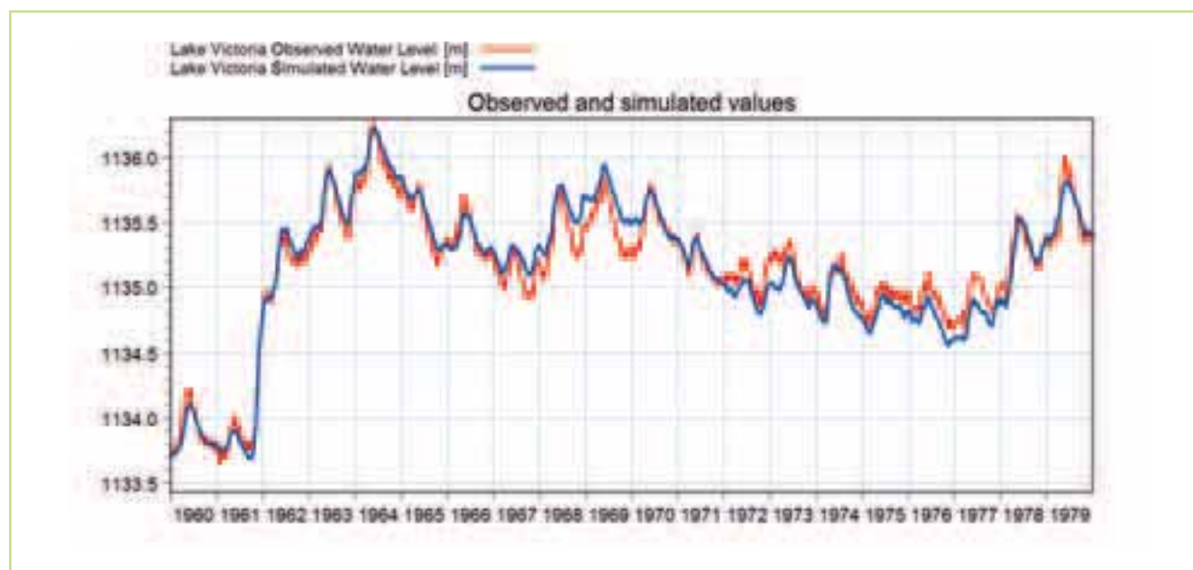
Figure 5.19 Comparison between observed (red) & simulated (blue) water levels at Lake Victoria for the modelling period 1960-80
