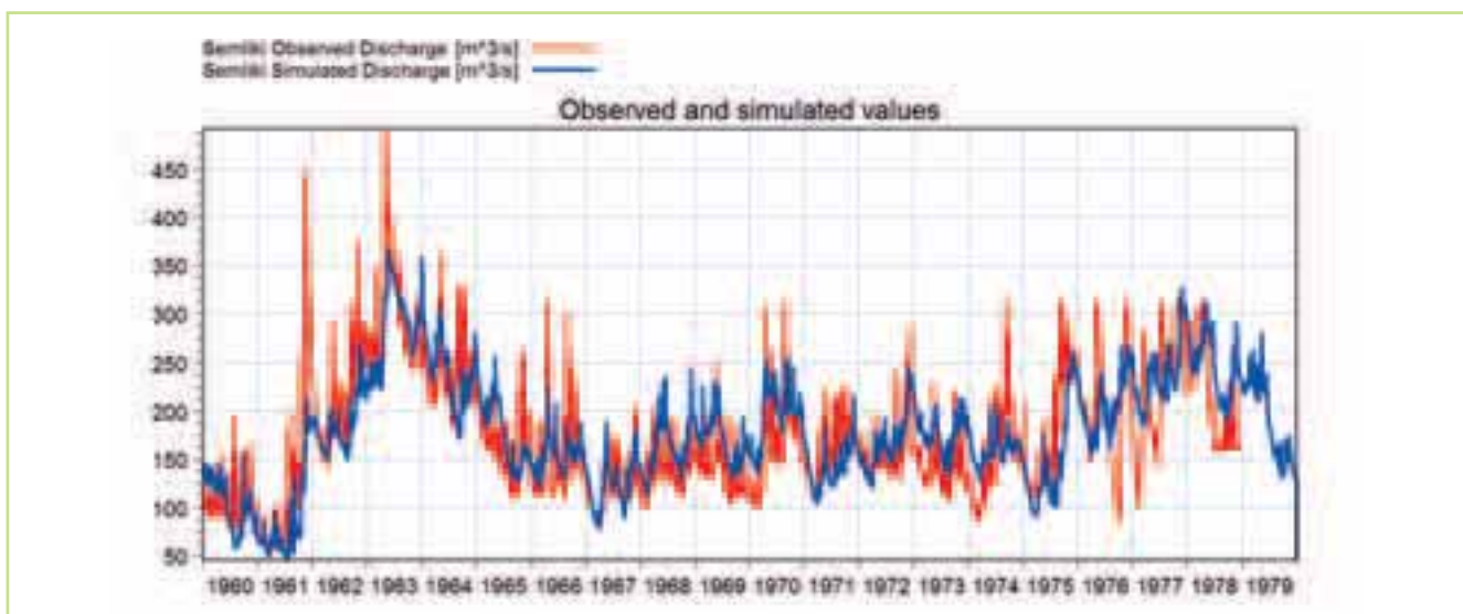
Figure 5.22 Comparison between observed (red) & simulated (blue) discharge at Semliki for the modelling period 1960-80
