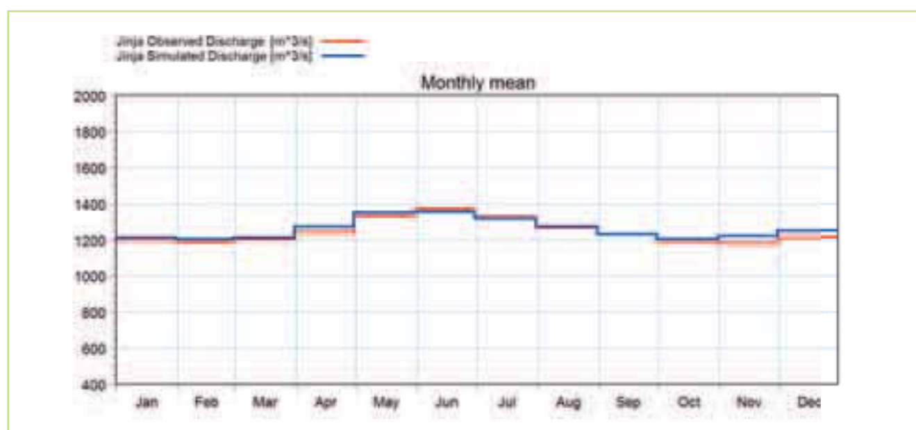
Figure 5.59 Comparison of the observed (red) & simulated (blue) mean monthly flows at the Jinja station for the period 1960-1980.
