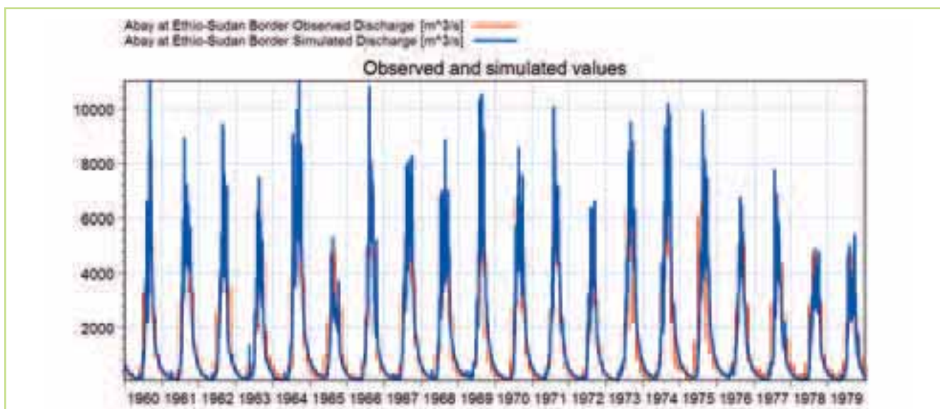
Figure 5.80 Comparison of the observed (red) & simulated (blue) flow hydrographs at the Abay station for the period 1960-1980
