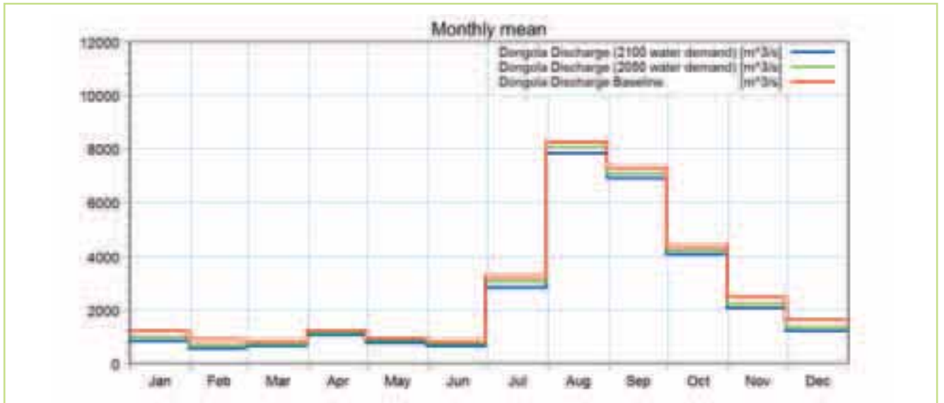
Figure 8.3 Mean monthly discharges for the Dongola gauge for baseline, 2050 & 2100 water demands
