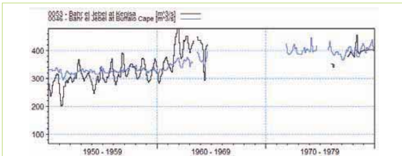
Figure 5.28 Observed discharge at Kenisa (black line) & Buffalo Cape (blue line)
