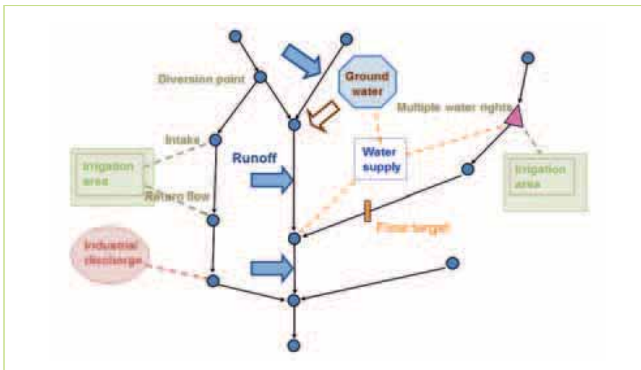
Figure 5.6 Schematic of the MIKE BASIN network model including different water activities
