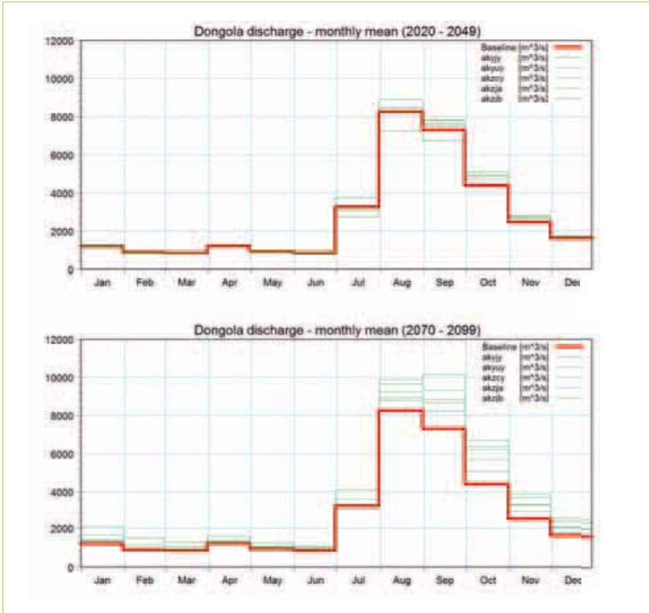
Figure 7.10 Projected changes in the average monthly flows for the Dongola station for the two periods; 2020-2049 & 2070-2099. The solid (red) line shows the baseline levels (1961-1990) & the thin green lines the different RCM ensemble members
