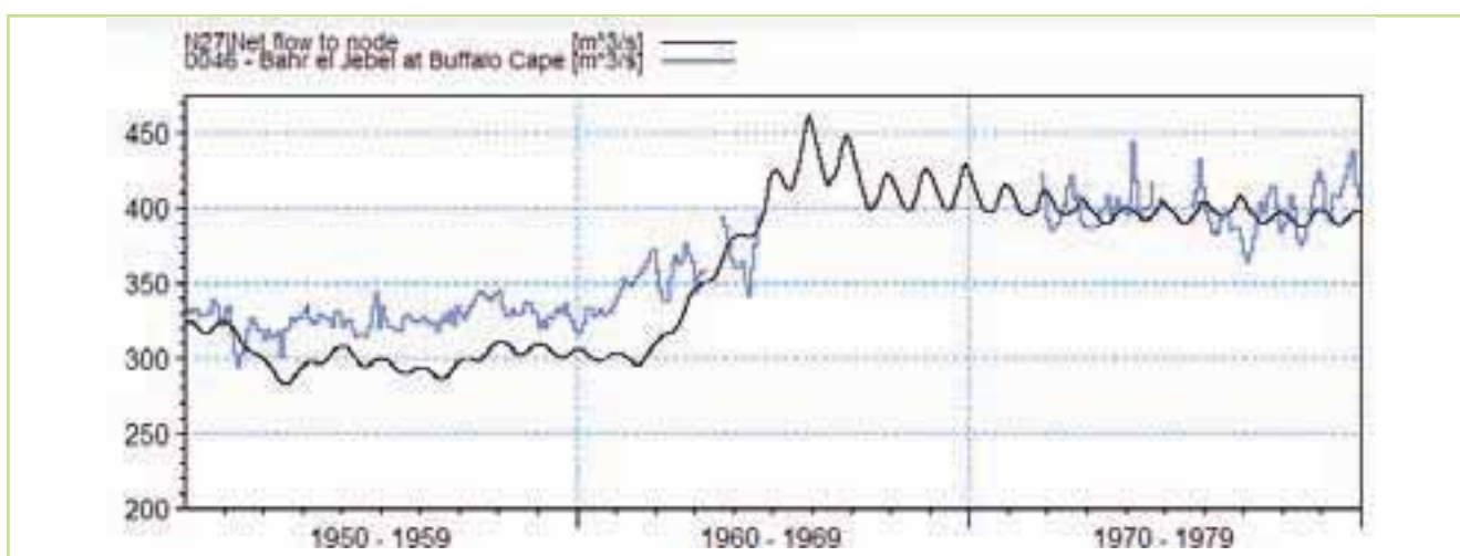
Figure 5.29 Simulated (black line) & observed (blue line) discharge at Buffalo Cape
