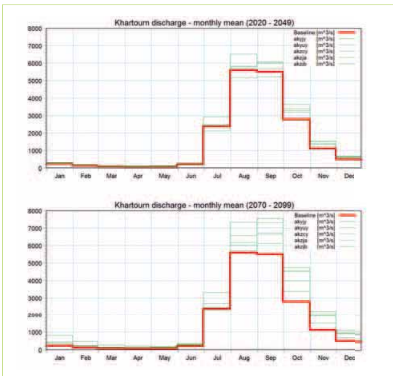
Figure 7.6 Projected changes in the average monthly flows for the Khartoum station for the two periods; 2020-2049 & 2070-2099. The solid (red) line shows the baseline levels (1961-1990) & the thin green lines the different RCM ensemble members
