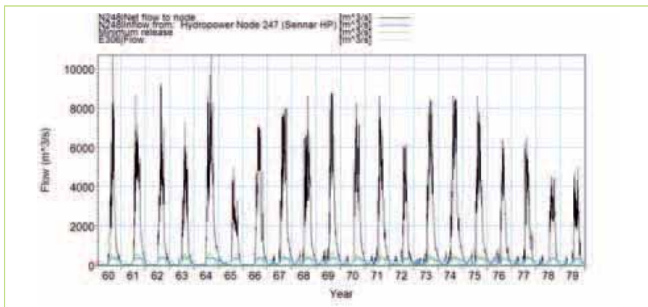
Figure 5.47 Simulated Sennar outflows (“Net flow to node” = total downstream release, minimum release is routed through hydropower and therefore is a component of the hydropower release, E306 = delivery to Gezira-Managil scheme)
