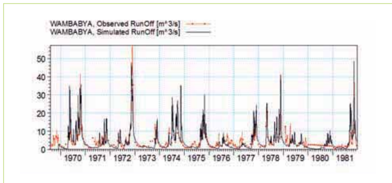
Figure 5.10 An example of a calibration plot from the Wambabya catchment in the Lake Victoria Basin. Comparison of the observed (red) & simulated (black) discharge for the Wambabya catchment, for the period 1970-1981. There is a reasonable agreement between the two hydrographs with the exception of 1980 where the observed data is probably not reliable. It should also be noted that for this particular station the model has difficulties in representing the flow pattern during the dry period
