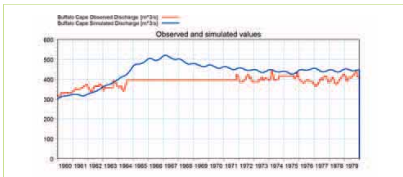
Figure 5.67 Comparison of the observed (red) & simulated (blue) flow hydrographs at the Buffalo Cape station for the period 1960-1980
