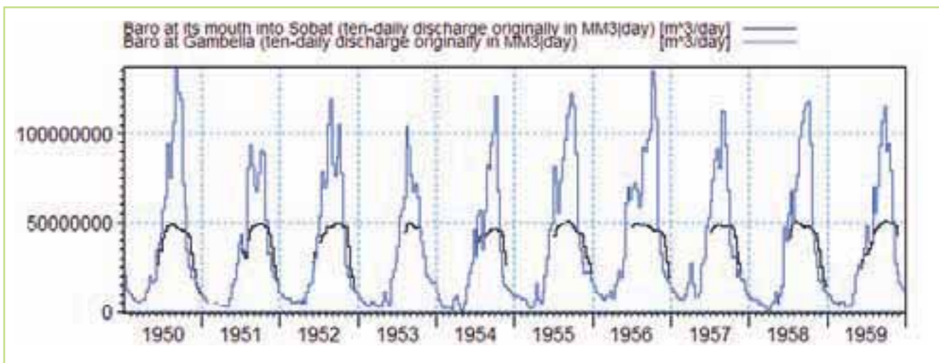
Figure 5.33 Flow record at Gambella & at the outlet to the Baro river
