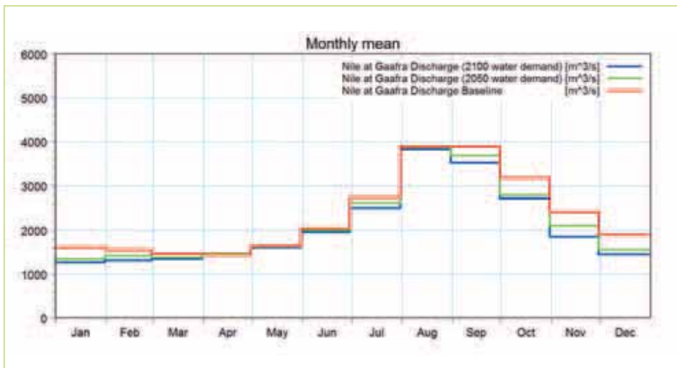
Figure 3. Mean monthly discharges for the Gafra (El-Ga'Afra) gauge for baseline, 2050 & 2100 water demand scenarios
