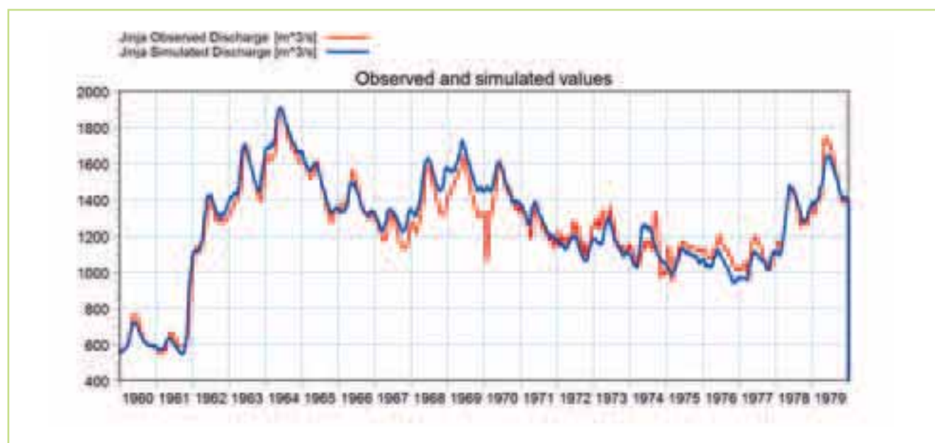
Figure 5.58 Comparison of the observed (red) & simulated (blue) flow hydrographs at the Jinja station for the period 1960-1980
