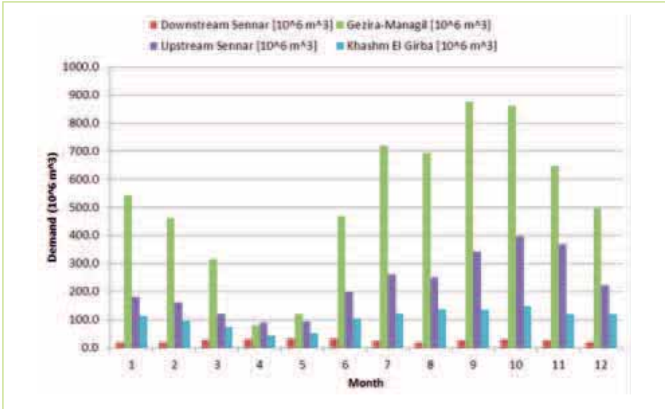
Figure 5.49 Irrigation water demands in Blue Nile & Atbara representation
