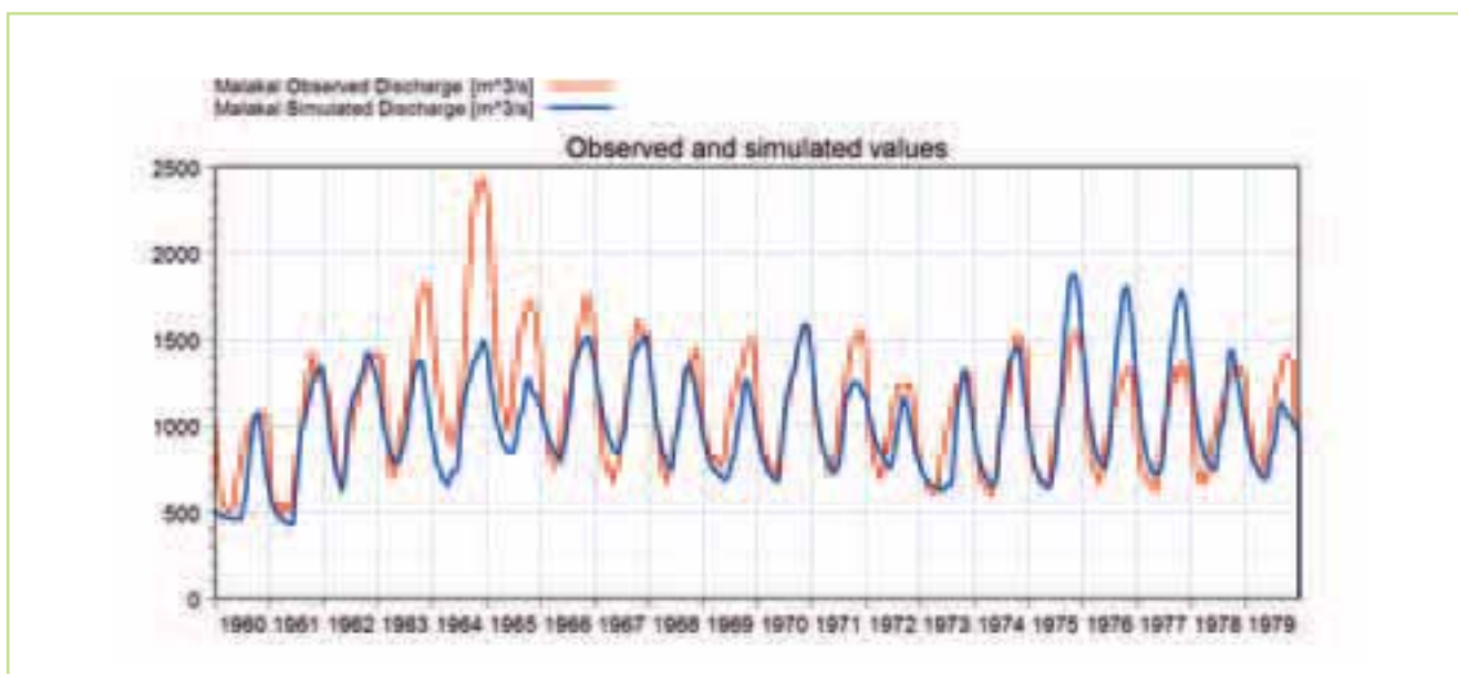
Figure 5.73 Comparison of the observed (red) & simulated (blue) flow hydrographs at the Malakal station for the period 1960-1980
