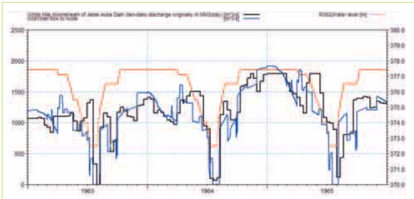
Figure 5.37 Observed outflow from Jebel Aulia (black line), simulated outflow from Jebel Aulia (blue line) & simulated water level at Jebel Aulia (red line)
