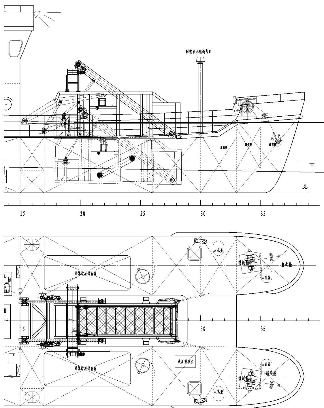
Fig 1. A blueprint of a SGRE fixed on a catamaran.
