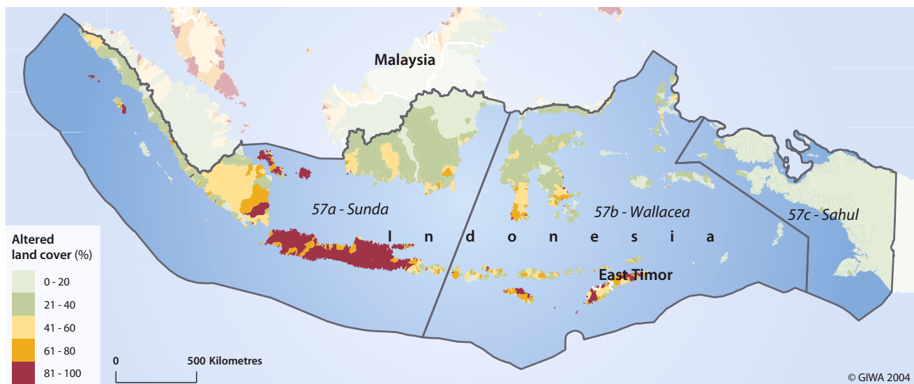
Figure 10 Reefs at risk due to alteration of land cover. (Source: Burke et al. 2002)
