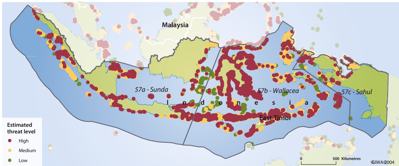
Figure 2 Reefs at risk in the Indonesian Seas region. (Source: Burke et al. 2002)
