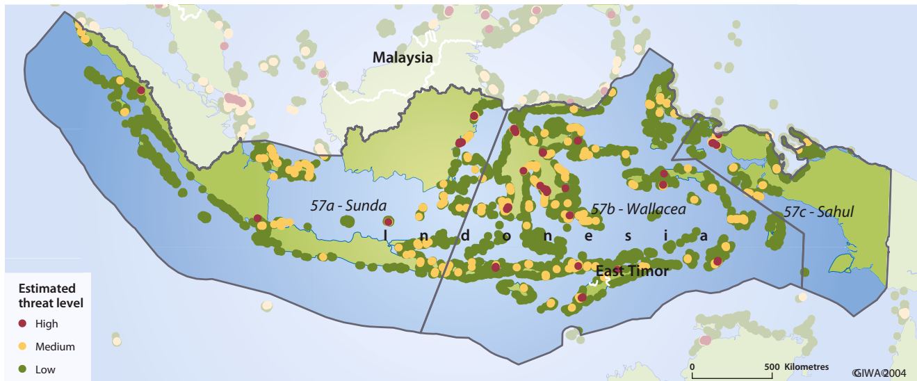
Figure 8 Reefs at risk due to marine pollution. (Source: Burke et al. 2002)
