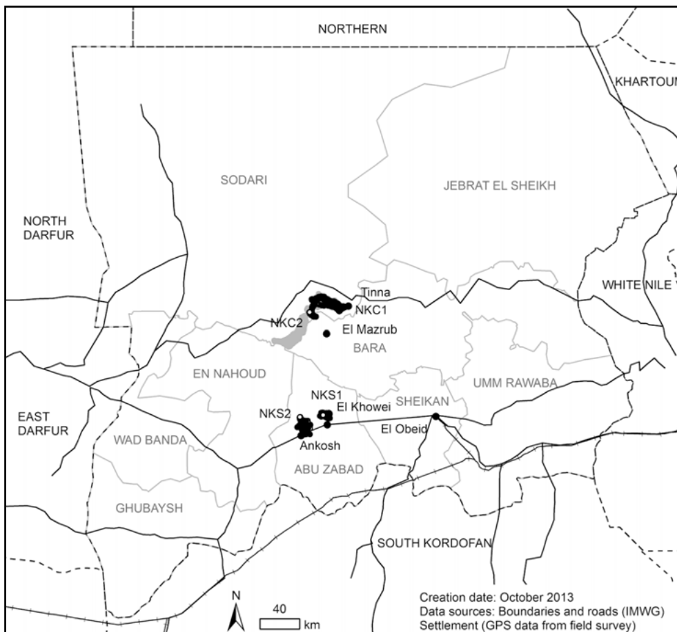
Figure 22. Map of North Kordofan showing the general patterns of the two sheep and two camel herders during the early rains to mid-rainy season
