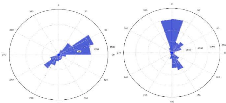
Figure 9. Port-à-Piment and Randel wind direction.
