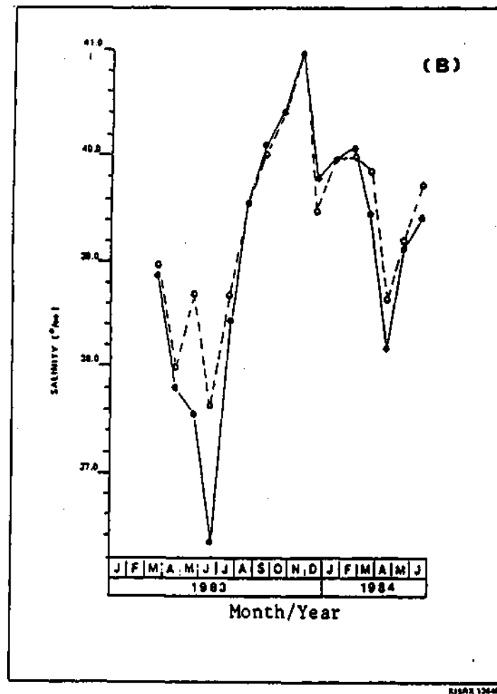
Figure 9. Seasonal changes of (a) seawater temperature, air temperature over the Gulf, and air temperature at the Kuwait International Airport, and (b) surface (—) and 10 m deep (----) seawater salinity (after Literathy et al., 1985).
