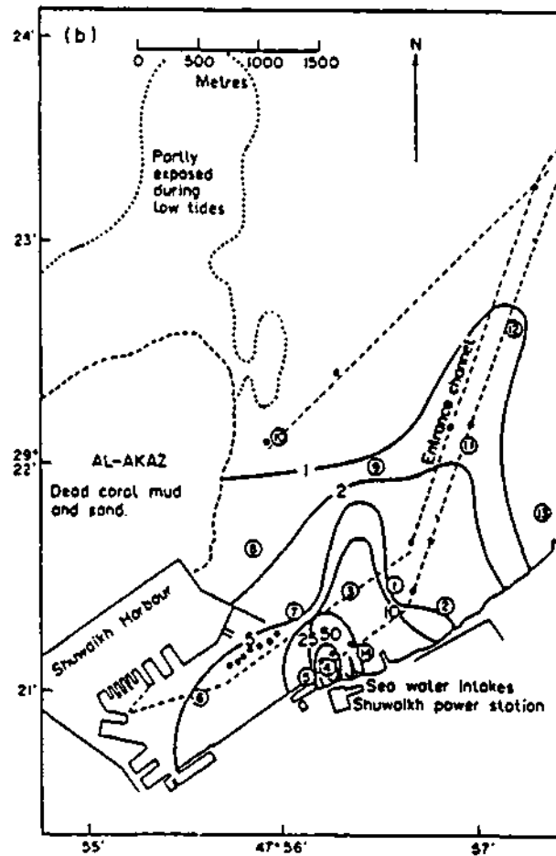
Figure 14. Distribution of halomethanes ( \mu\text{g l}^{-1} ) in seawater off Shuwaikh during the ebb (a) and flood (b) phases of the tide (after Ali and Riley, 1986).
