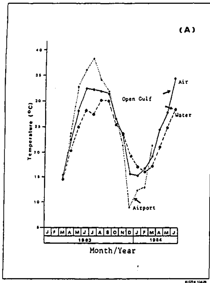
Figure 9. Seasonal changes of (a) seawater temperature, air temperature over the Gulf, and air temperature at the Kuwait International Airport, and (b) surface (—) and 10 m deep (----) seawater salinity (after Literathy et al., 1985).
