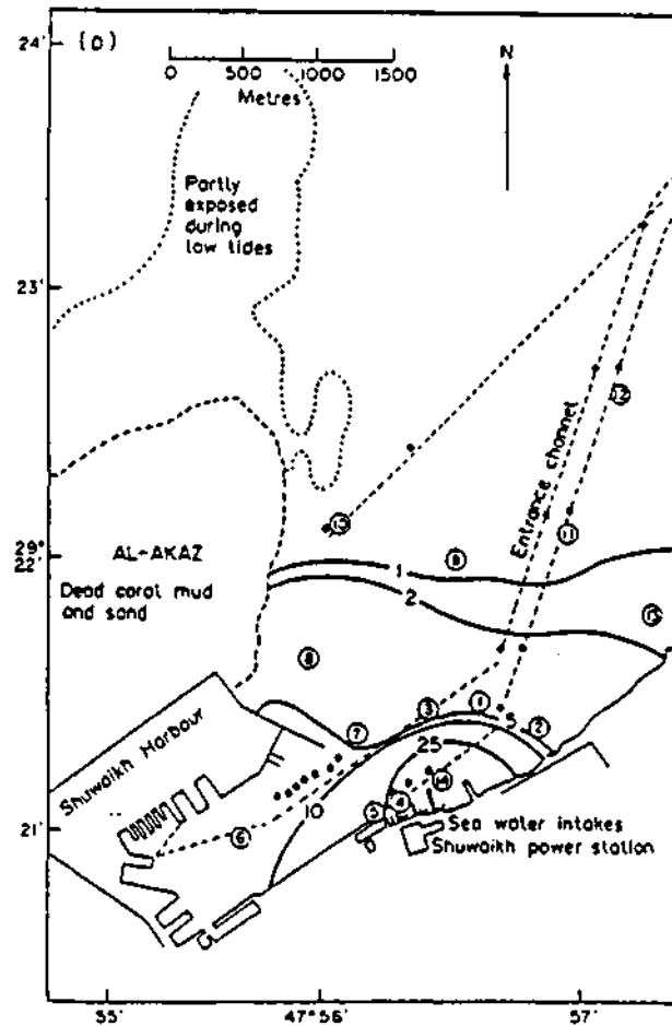
Figure 14. Distribution of halomethanes ( \mu\text{g l}^{-1} ) in seawater off Shuwaikh during the ebb (a) and flood (b) phases of the tide (after Ali and Riley, 1986).
