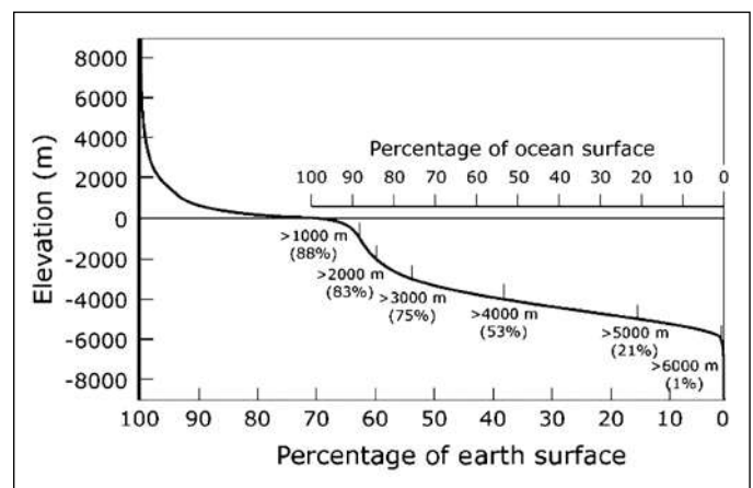
Figure 6.21 Relationship between depth and sea floor area. Flow in ocean bottom boundary layers would need to be taken into account when selecting a site for a \text{CO}_2 lake. Bottom friction and turbulence can enhance the dissolution rate and vertical transport of dissolved \text{CO}_2 and lead to a short lifetime for the lake (Section 6.2.1.6). It has been suggested that \text{CO}_2 lakes would be preferentially sited in relatively restricted depressions or in trenches on sea floor (Ohsumi, 1995).
