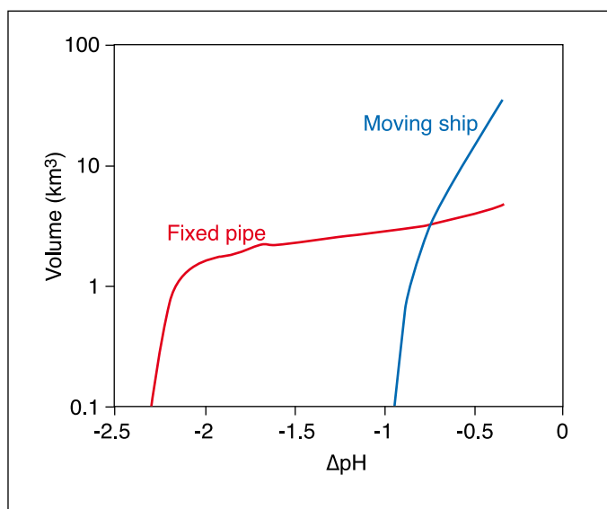
Figure 6.13 Volume of water with a \Delta\text{pH} less than the value shown on the horizontal axis for the simulations shown in Figure 6.12 corresponding to CO 2 releases from a 500 MWe power plant. The fixed pipe simulation produces a region with \Delta\text{pH} < -1 , however, the moving ship disperses the CO 2 more widely, largely avoiding pH changes of this magnitude.
