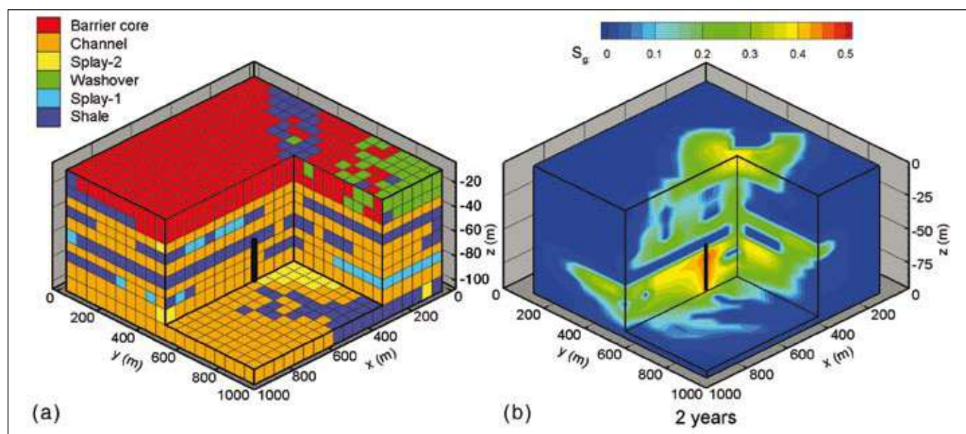
Figure 5.6 Simulated distribution of \text{CO}_2 injected into a heterogeneous formation with low-permeability layers that block upward migration of \text{CO}_2 . (a) Illustration of a heterogeneous formation facies grid model. The location of the injection well is indicated by the vertical line in the lower portion of the grid. (b) The \text{CO}_2 distribution after two years of injection. Note that the simulated distribution of \text{CO}_2 is strongly influenced by the low-permeability layers that block and delay upward movement of \text{CO}_2 (after Doughty and Pruess, 2004).
