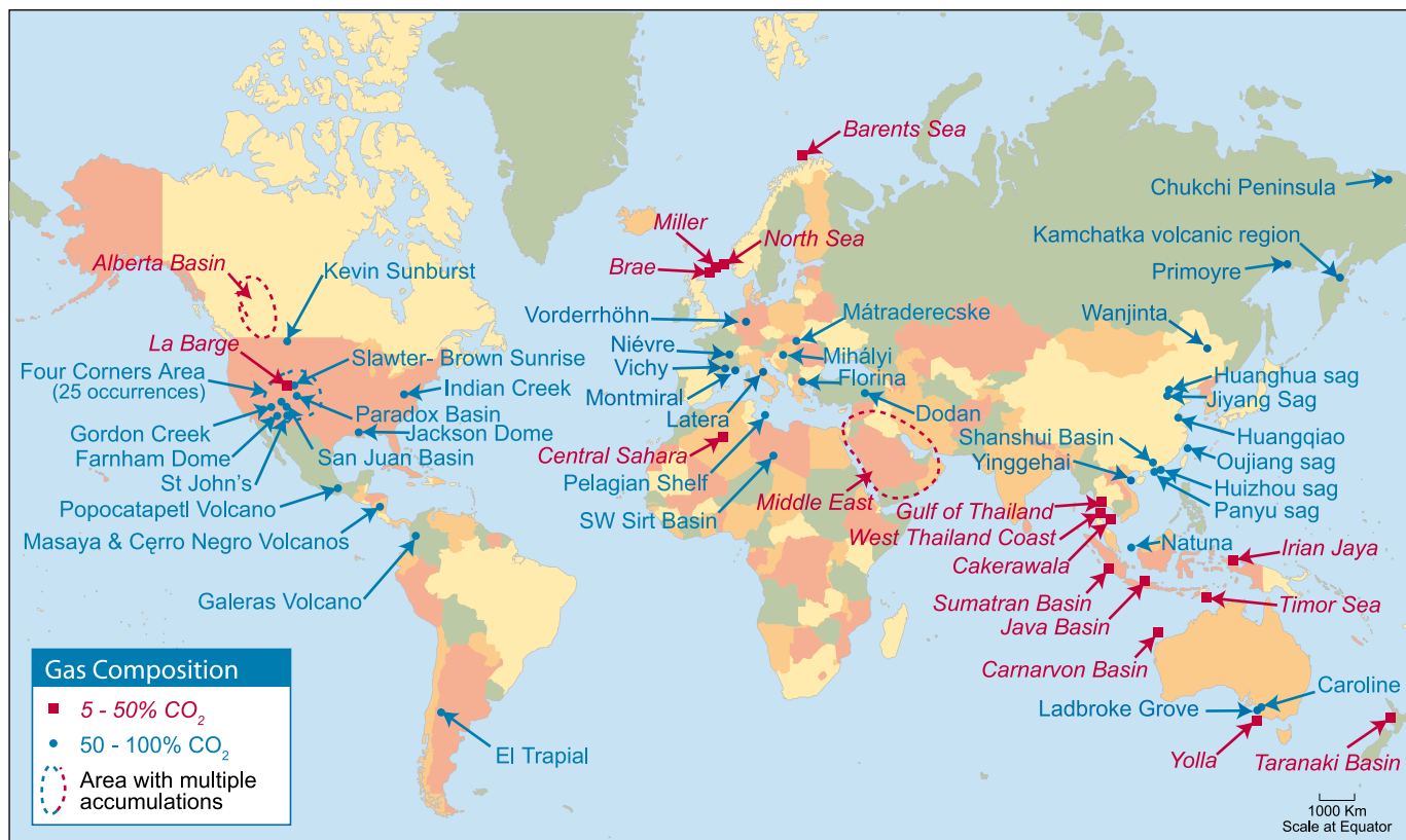
Figure 5.11 Examples of natural accumulations of \text{CO}_2 around the world. Regions containing many occurrences are enclosed by a dashed line. Natural accumulations can be useful as analogues for certain aspects of storage and for assessing the environmental impacts of leakage. Data quality is variable and the apparent absence of accumulations in South America, southern Africa and central and northern Asia is probably more a reflection of lack of data than a lack of \text{CO}_2 accumulations.
