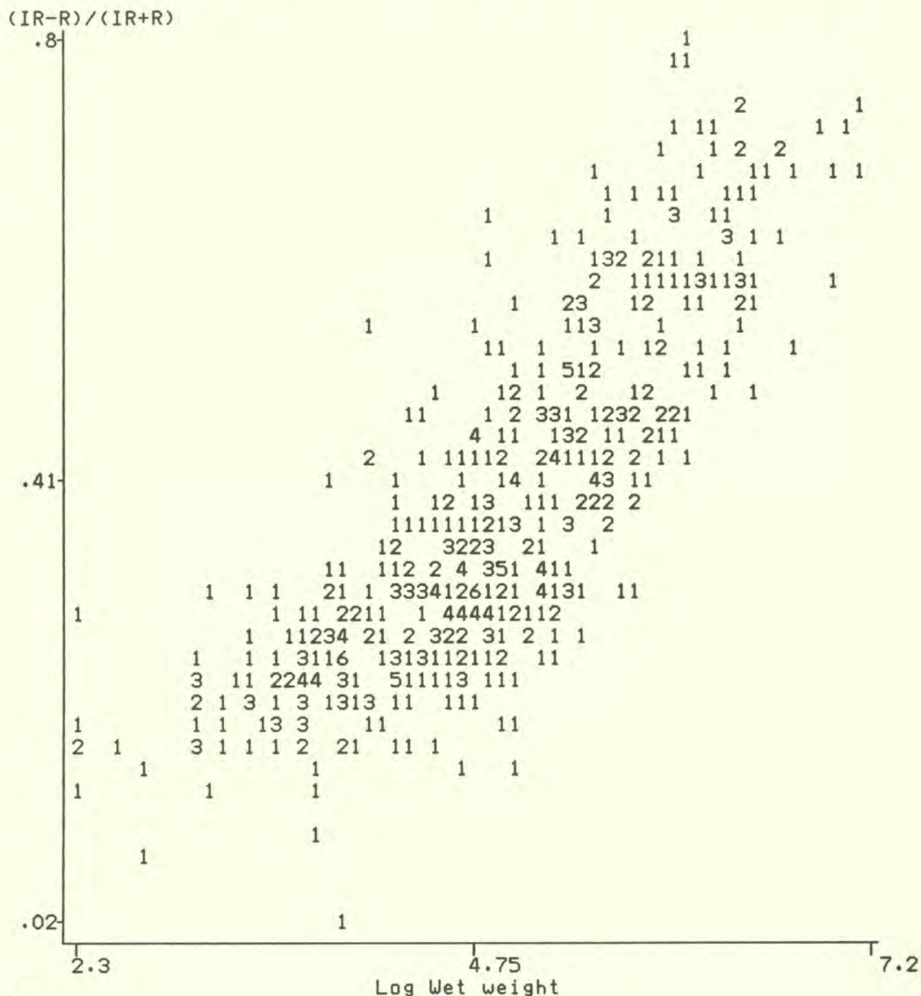
Figure 9: Correlation of (IR-R)/(IR+R) with Log Wet weight for all species.
