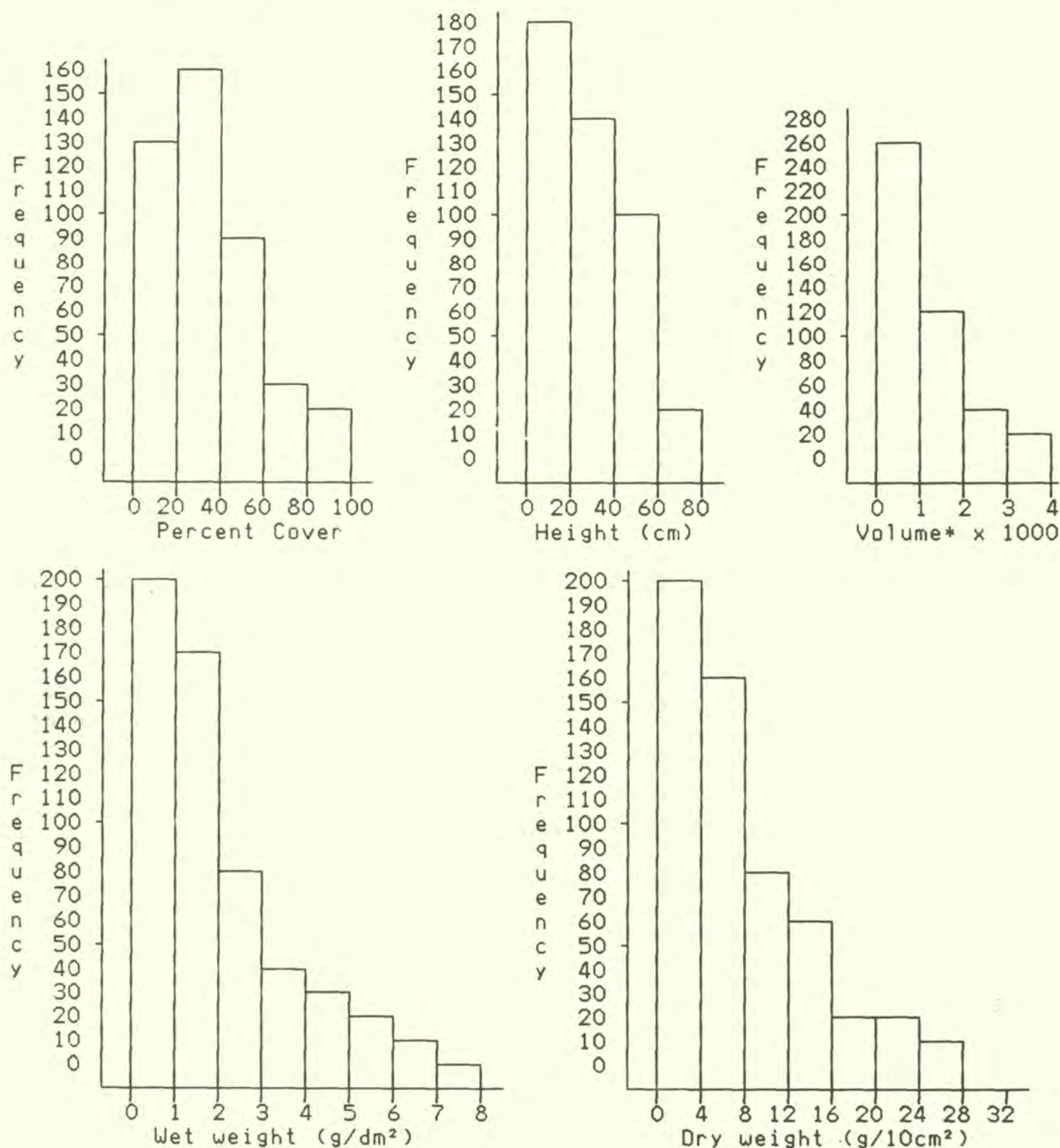
Figure 2: Frequency distributions of parameters measured in the Ferlo at the end of the growing seasons of 1981, 82 and 83.
