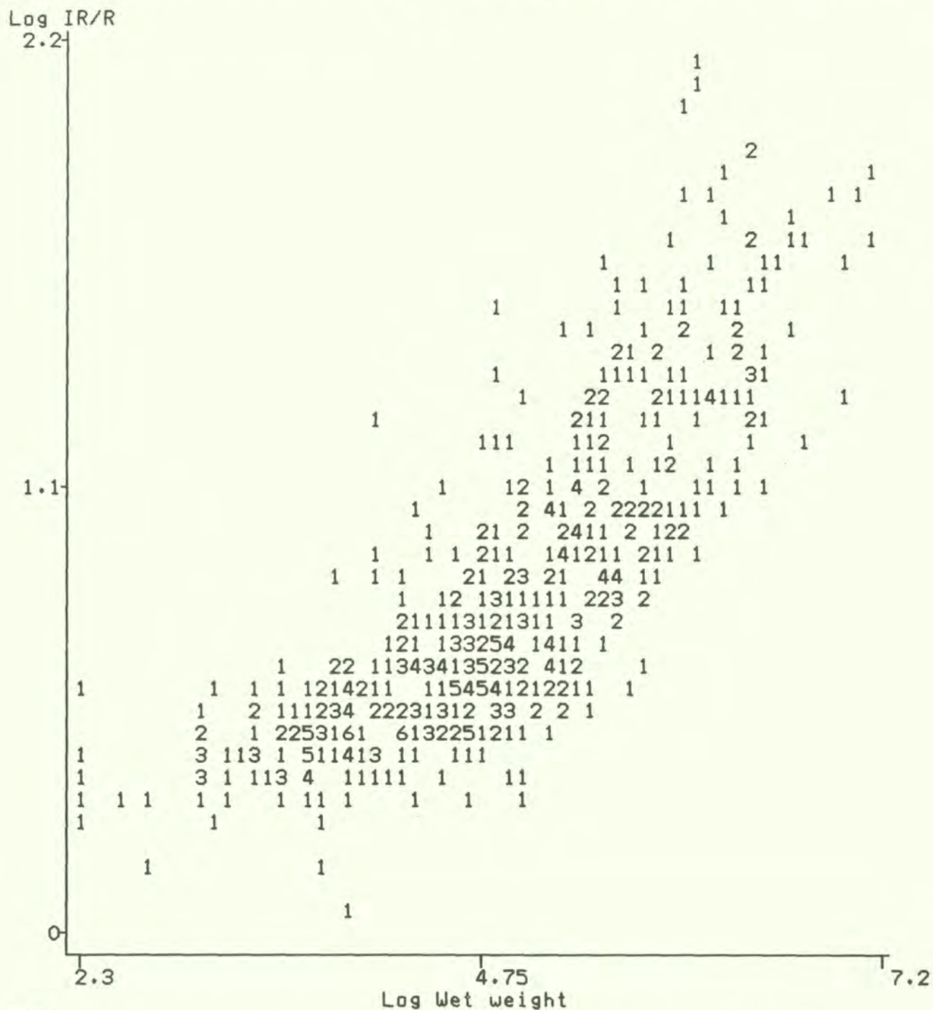
Figure 7: Correlation of \log(\text{IR/R}) and \log(\text{wet wt}) for all species
