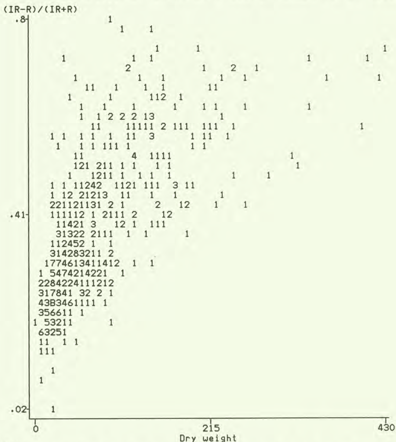
Figure 8: Correlation of (IR-R)/(IR+R) with Dry weight for all species.
