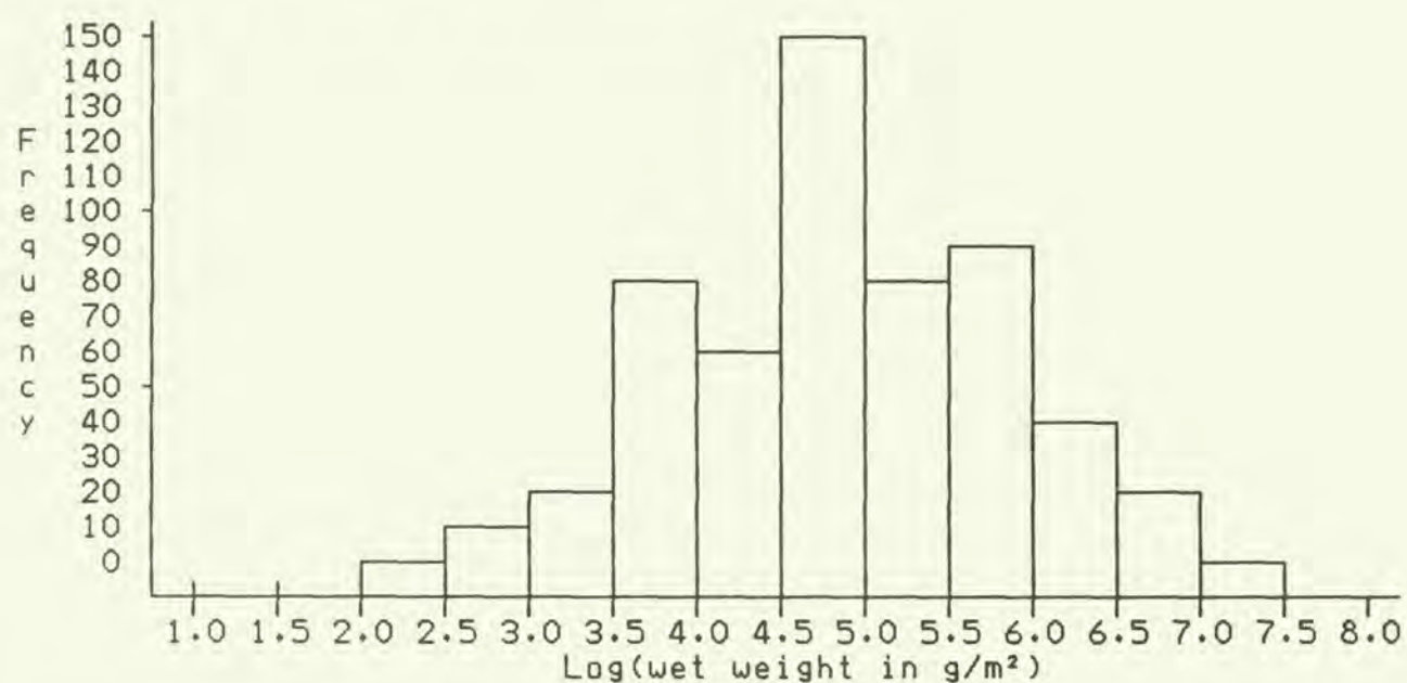
Figure 3: Frequency distributions of wet and dry weight of clipped grass layer plants transformed by logarithm.
