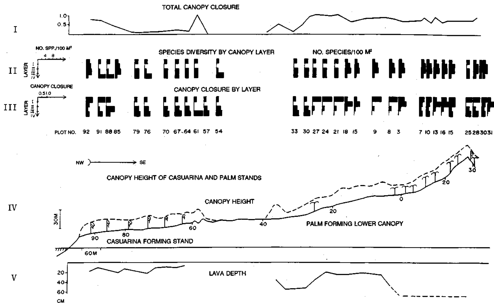
Figure 13. Ecological transect characteristics, Niuafo'ou Island. I. Total canopy closure. II. Species distribution by layers. III. Canopy closure by layers. IV. Hypsometric profile of stand height, abundance of Casuarina in layer I, and palm dominance. V. Depth of lava.
