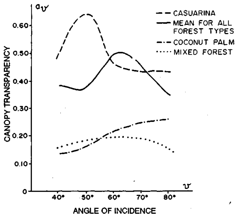
Figure 15. Canopy transparency in the woody layer of forests on Niuafo'ou Island. A. All forests; B. Casuarina forest; C. Palm forest; D. Mixed forest.
