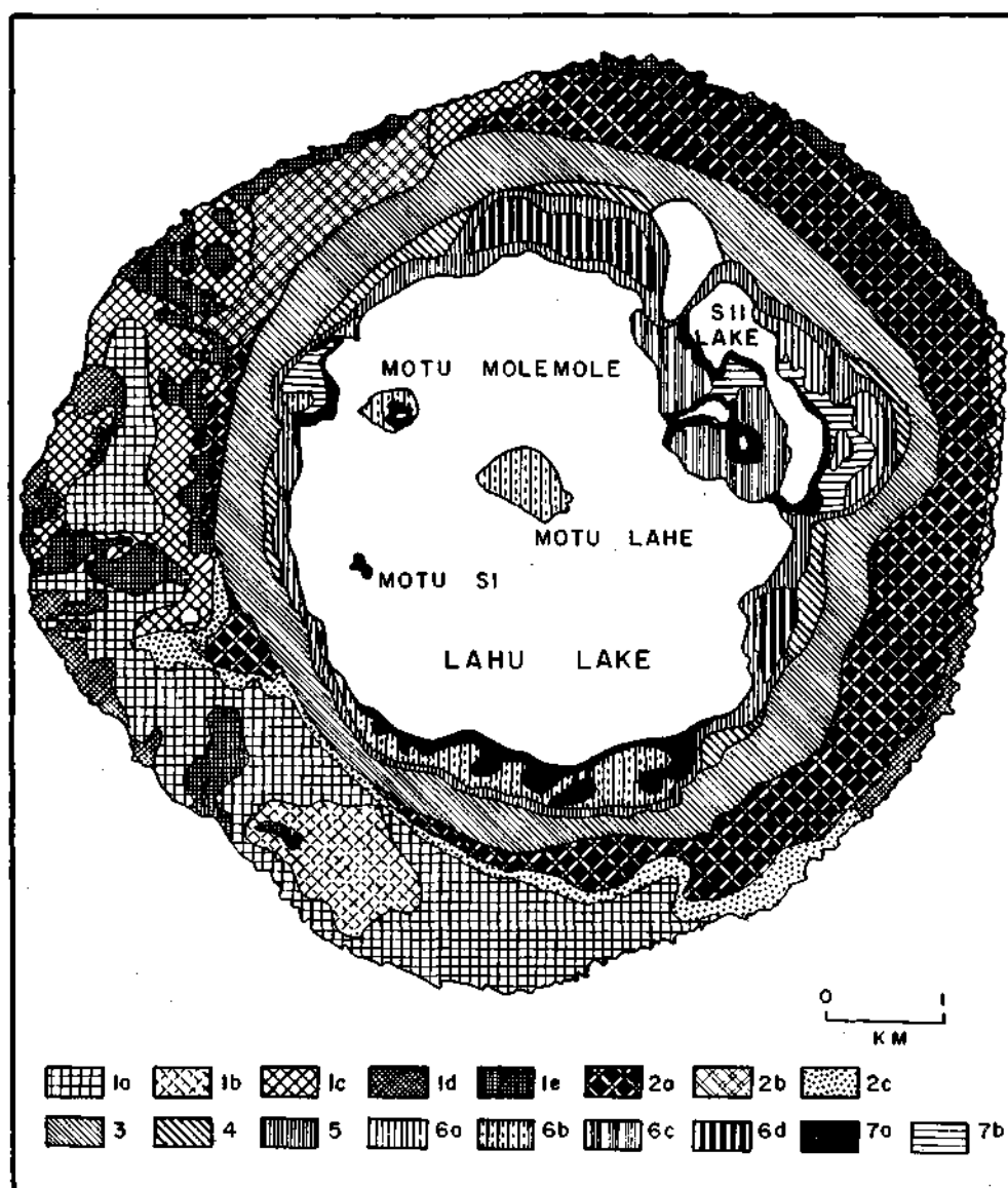
Figure 16. Landscape map of Niuafo'ou Island. Legend. I. External volcano slopes and plains. 1. Ash or lava plain, 2-4° slope; 1a. Lava field with no vegetation; 1b. Ash fields with no vegetation; 1c. Lava field with pioneer vegetation and immature soils in crevices; 1d. Lava field with maritime shrub-herb vegetation, young soils; 1e. Forest "islands". 2. Old lava fields with ash-slaggy soils with developed humus horizons; 2a. Vegetable gardens, plantations, secondary forest and shrub succession in abandoned gardens; 2b. Herb-shrub vegetation; 2c. Coastal shrub vegetation; 3. Strato-volcano mid-level slopes with red andosols, coconut plantations, vegetable gardens, post-garden forest and shrub successions; 4. Upper strato-volcano slopes with polydominant forests on thick ash soils; II. Inner crater slopes and plains. 5. Steep (50-60°) internal crater slopes with oligodominant forests (mainly of Casuarina in the upper layer) on laminated ash soils with old humus horizons; 6. Ash-slaggy hills and plateaus of crater with laminated ash soils; 6a. Undissected hills covered by mature monodominant forest with Casuarina in the upper layer; 6b. Weakly dissected hills covered by young forest of Casuarina ; 6c. Strongly dissected hills covered by Casuarina in open woodlands and pastures; 6d. Plateaus with Casuarina forests; 7a. Lacustrine-ash plain (low level) covered by shrubs; 7b. Lacustrine-ash plains (high level).
