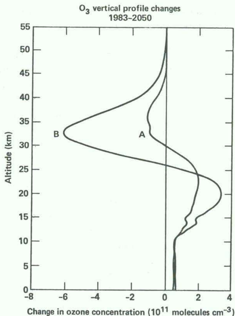
Figure 4.3 (b) 1-D model calculation of change in ozone concentrations (1983-2050) with altitude based on cases (A) and (B) in Figure 4.1
