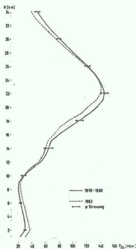
Figure 5 Mean ozone profiles MOHp for 1983 and for 1970-1980
