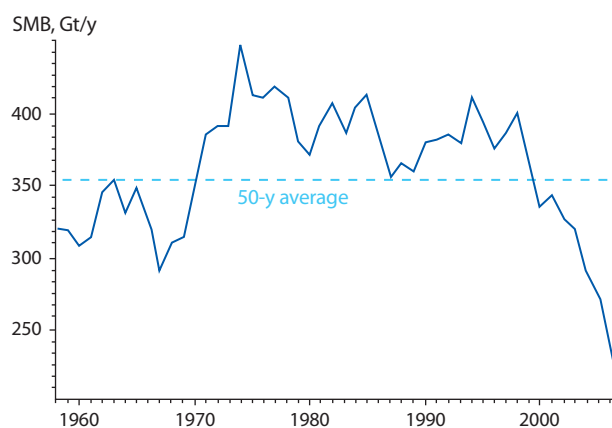
Figure 8.13. Mean SMB of the three reconstructions (MAR, PMM5, Hanna) shown in Figure 8.9. The data have been smoothed over a running 5-year period to reduce interannual variation. Source: Jonathan Bamber, University of Bristol.
