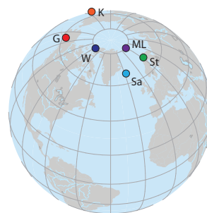
Figure 7.10. Cumulative area-averaged mass balance for six Arctic glaciers: White Glacier (Axel Heiberg Island), Gulkana Glacier (Alaska), Storglaciären (Sweden), Midre Lovénbreen (Svalbard), Satujökull (Hofsjökull, Iceland), and Kozelsky (Kamchatka) over the period of record. All records show a negative cumulative balance (net thinning) over the period of record and more rapid thinning after about 1990 (although the precise timing of this varies between regions). Source: AMAP.
