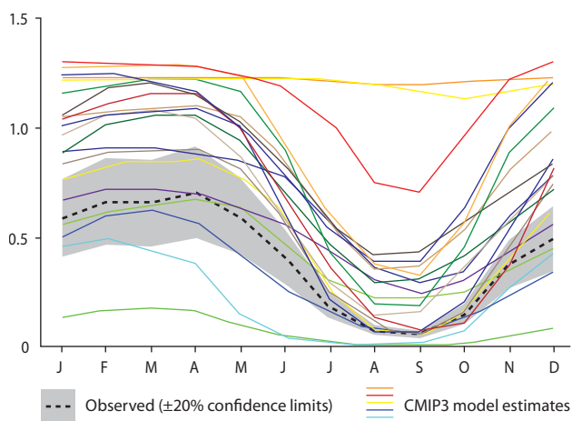
Figure 3.7. Seasonal cycle of sea ice in the Barents Sea according to various CMIP3 models. Note that most models show too much sea ice coverage. Source: modified version of figure 3 from Overland and Wang (2007).
