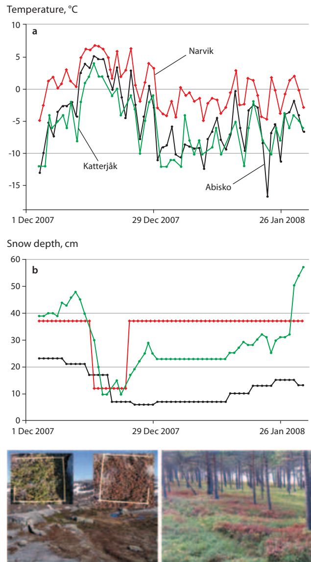
Figure 4.21. A mid-winter warming event in December 2007 and its impact on vegetation over 1400 km 2 in sub-Arctic Norway and Sweden. Air temperatures (a) increased at three sites along a transect from Narvik, Norway, to Abisko, Sweden, (68° N) for a few days in December and snow melted (b) before returning. The few snow-free days resulted in the death of some dwarf shrubs in open, alpine habitats (photo left) and coastal pine forests (photo right). Snow remaining in depressions protected vegetation (left insert); whereas unprotected vegetation died (right insert). Source: Bokhorst et al. (2009).
