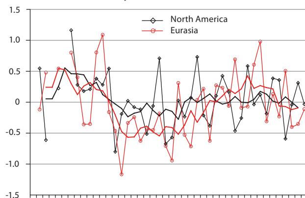
Arctic autumn SCD anomaly (relative to 1988-2007)
