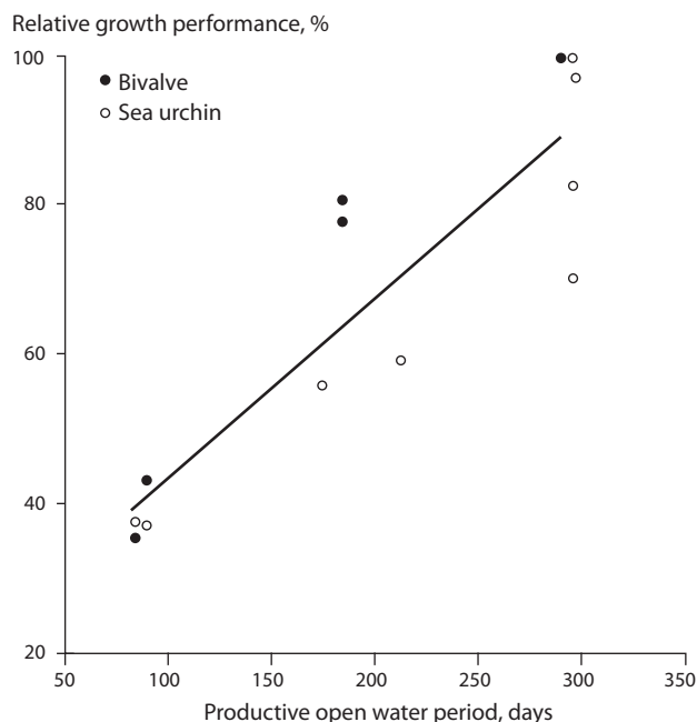
Figure 9.33. Growth performance of the bivalve Clinocardium ciliatum estimated as maximum annual shell growth plotted against the productive open-water period. Data for the sea urchin Strongylocentrotus droebachiensis recalculated from Blicher et al. (2007) are included. Linear regression for the combined dataset of both species: G_{\max} = 0.24 \times [\text{POWP}] + 19.4 , p < 0.01 , R^2 = 0.78 . Source: Sejr et al. (2009).
