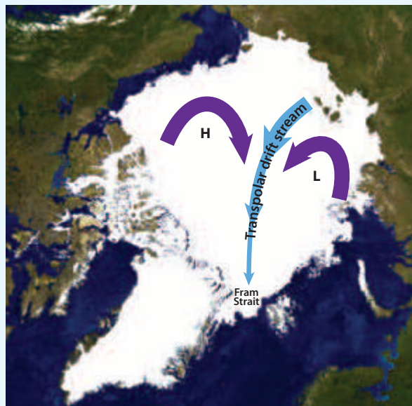
Figure 9.26. Schematic illustration of the Polar Express phenomenon.
