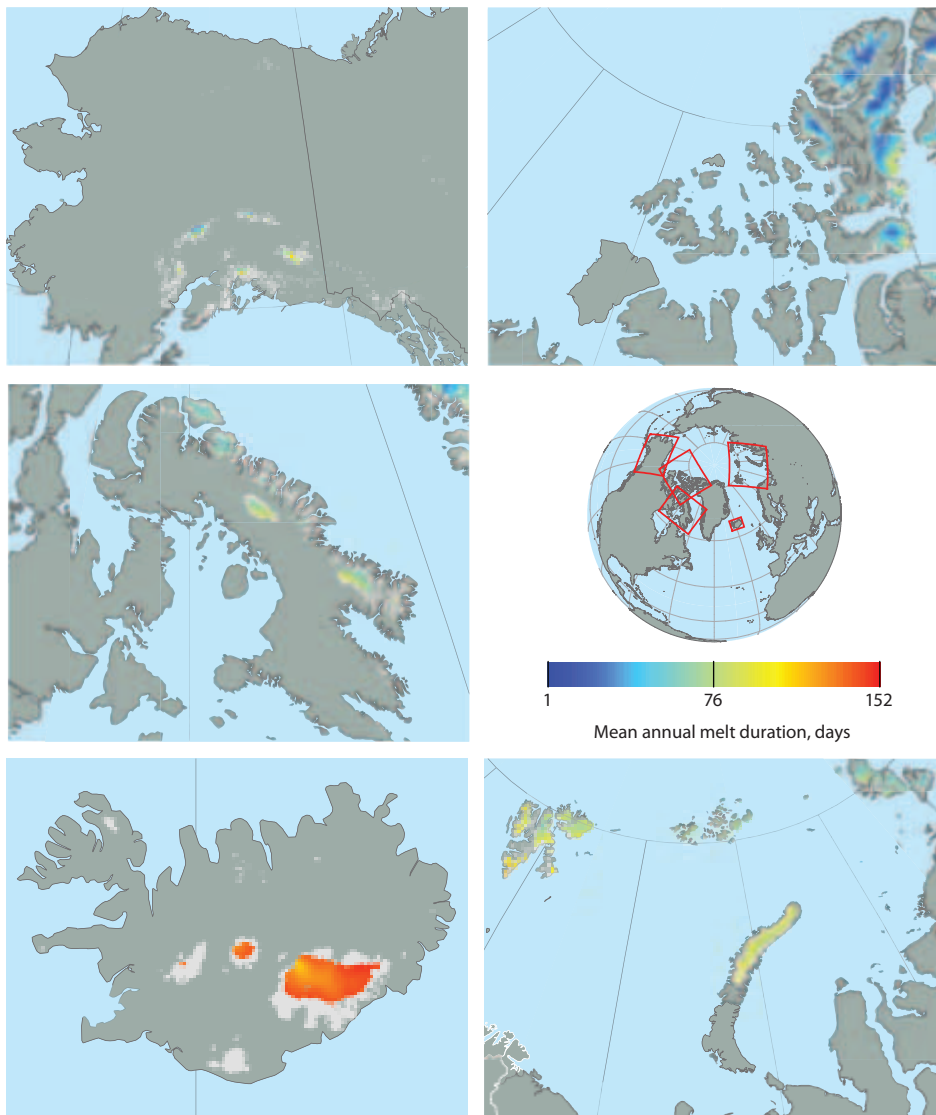
Figure 7.13. Mean annual melt duration on larger Arctic ice masses for the period 1999 to 2008 based on QuikSCAT scatterometer data. Source: Gabriel Wolken, Alaska Division of Geological and Geophysical Surveys.
