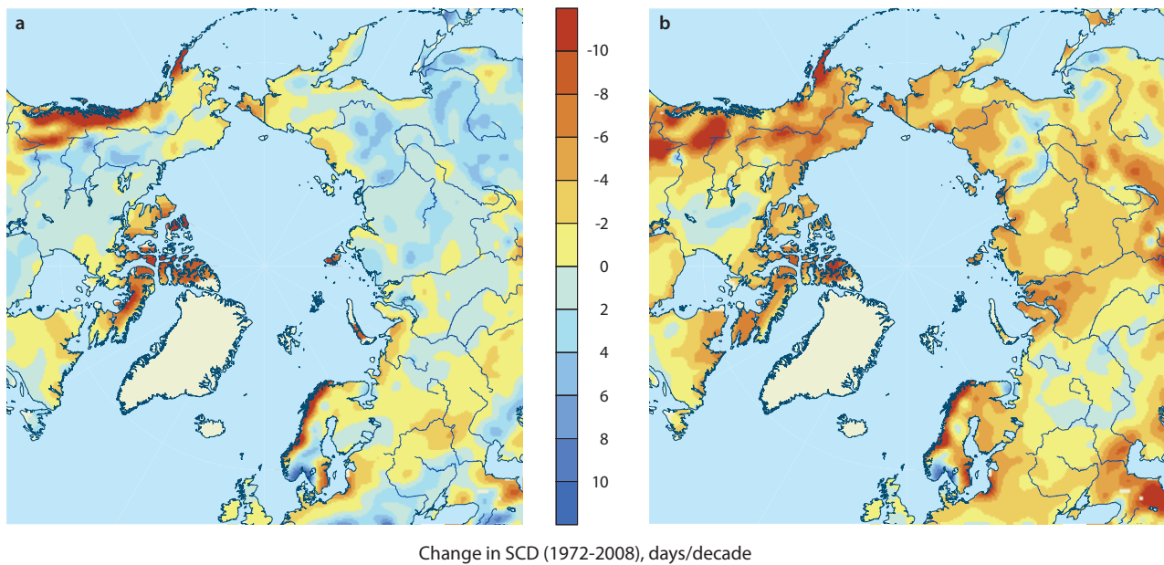
Figure 4.11. Trend in snow-cover duration for (a) autumn (snow-cover onset period) and (b) spring (snow-cover melt period) over the 1972/73 to 2008/09 snow seasons from the NOAA weekly dataset maintained at Rutgers University by Dr. D. Robinson. Trends were computed using the least squares method. Source: updated from UNEP (2007) by R. Brown, Climate Research Division, Environment Canada, 21 September 2009.
