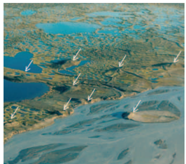
Figure 5.22. Pingos (indicated by arrows) in ice-wedge polygon terrain on a terrace covered with thaw lakes on Bylot Island, Canada. The eroded pingos along the riverbank and on the island are collapsing. Photo: Michel Allard.
