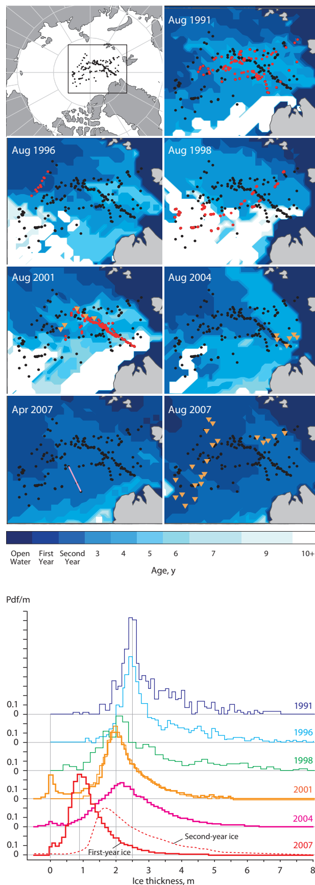
Figure 9.14. Late summer sea-ice age (above) and thickness (below) in the region of the North Pole between 1991 and 2007. Thickness was obtained by means of ground-based (thin lines, •) and airborne (thick lines, ▼) electromagnetic induction sounding. In 2007, first-year ice prevailed in August, but second-year ice was still present in April 2007. The latter distribution was seasonally adjusted to be comparable with summer conditions. Source: Haas et al. (2008).
