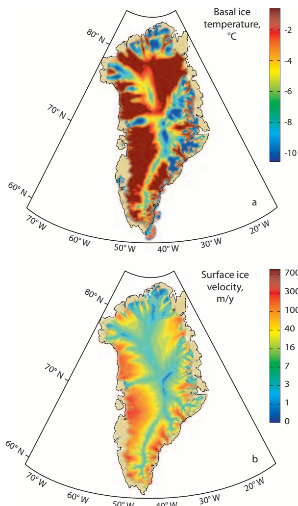
Figure 8.25. Model reconstructions of the present-day Greenland Ice Sheet (a) basal ice temperatures below the pressure-melting point, and (b) surface ice velocity. Source: Unpublished results, based on the Greenland Ice Sheet model described by Marshall and Cuffey (2000).
