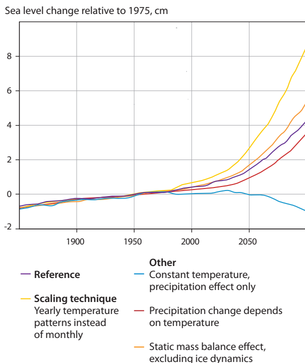
Figure 8.31. Modeled sea level rise from Greenland Ice Sheet retreat, 1860 to 2100, driven by modeled high-resolution ( 1.125^\circ ) temperature and precipitation patterns over Greenland, with temporal climate perturbations from the Hadley Centre AOGCM. The different lines denote different treatments of climate. Source: Huybrechts et al. (2004).
