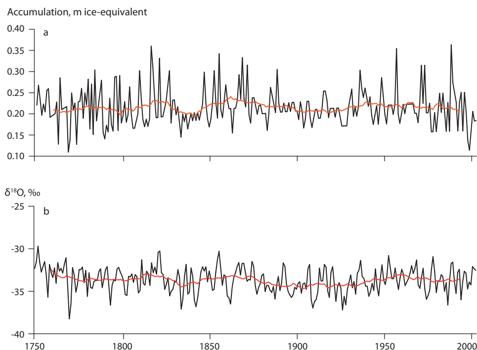
Figure 8.14. Results from a shallow ice core drilled at NEEM (77.5° N, 51° W) in 2007. The black curves represent annual values of accumulation (a) and stable water isotopes δ 18 O (b) while the red curves represent 20-year sliding mean values for the period 1750 to 2003. The accumulation rates are determined from detailed δ 18 O identification of annual layers based on 2.5 cm samples and a measured density record. Source: courtesy of the NEEM project.
