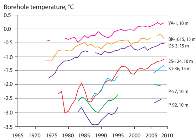
Figure 5.36. Time series of ground temperatures at 10 and 15 m depth at different locations within the Vorkuta research region. All the boreholes numbered above have the following landscape description: ZS-124 – peatland with ice wedge polygons; KT-36 flat surface of an alluvial-marine terrace; P-92 – gently sloping surface of an alluvial-lacustrine plain; P-57 – flat surface of an alluvial-lacustrine plain; BK-1615 – catchment of a glacial-marine plain; DS-3 – ice wedge polygons on a glacial-marine plain; YA-1 – within a water track on an erosional plain. Source: Romanovsky et al. (2010a).
