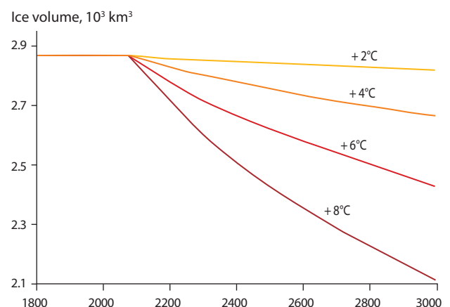
Figure 8.26. Modeled Greenland Ice Sheet volume response to different climate warming scenarios. Warming scenarios are introduced as a linear temperature perturbation from 2000 to 2100, with warming held constant at that level (2, 4, 6, or 8 °C) from 2100 to 3000. Source: Unpublished model results from Shawn Marshall, University of Calgary. For illustrative purposes only; not intended as a forecast for the ice sheet.
