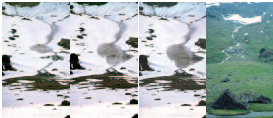
Figure 4.25. Images based on a rare recording of a slush torrent in June 1996 from sub-Arctic Sweden. The first three images show the result of increased saturation of the snowpack and then release of a large amount of water. The fourth image shows the valley in spring with a fan formed by such short-lived events over millennia. Photo: Gude and Scherer (1995).
