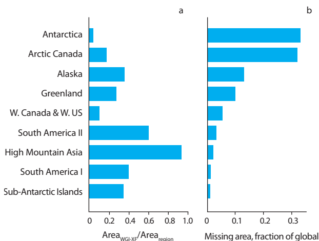
Figure 7.32. (a) Ratio between the area of Extended World Glacier Inventory (WGI-XF) glaciers (Cogley, 2009b), A_{WGI-XF} , and regional glacier area, A_{region} , for the nine glacierized regions that have incomplete glacier inventories. (b) Missing area in WGI-XF as a fraction of missing global glacierized area. While 'a' shows the degree of completeness of each regional inventory, 'b' indicates how much the different regions contribute to the global missing area. South America I refers to Bolivia, Ecuador, and Peru, while South America II refers to Argentina and Chile. Source: after Radić and Hock (2010).
