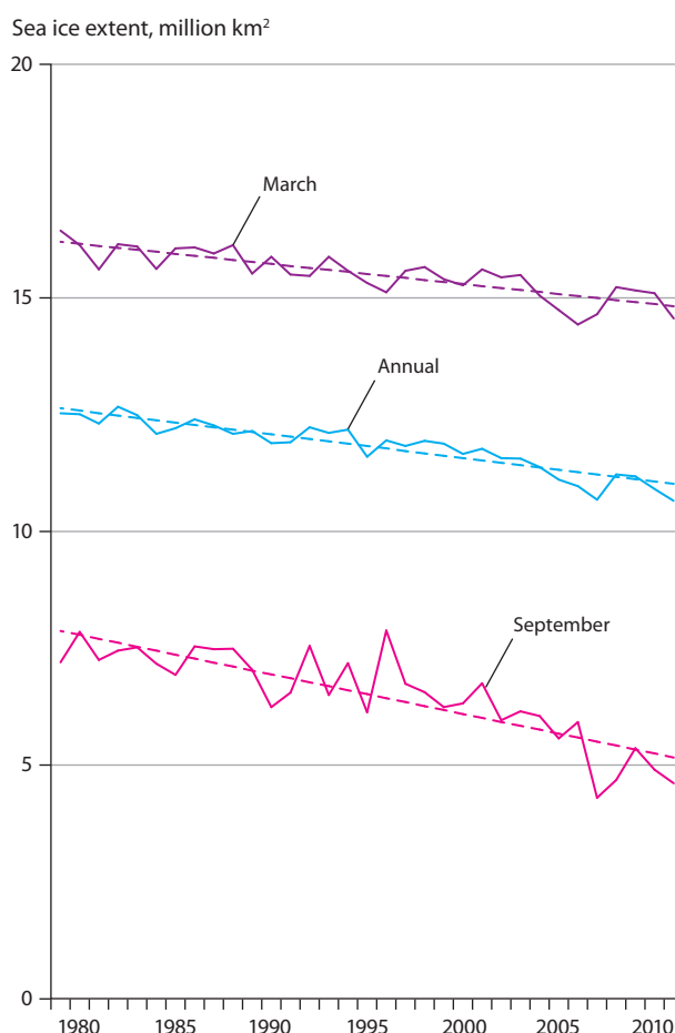
Figure 9.9. Average sea-ice extent in the Arctic in March, September, and annually for 1979 to 2011, including trend lines, from passive microwave satellite data. Source: updated from Fetterer et al. (2011).
