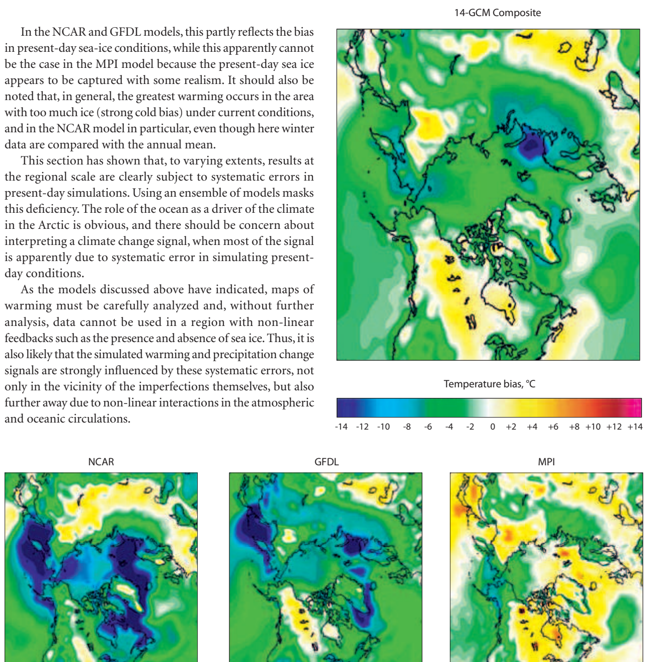
Figure 8.23. Ensemble mean temperature (based on 14 models) and three individual model temperature biases for winter (1958–2000). Source: Walsh et al. (2008).
