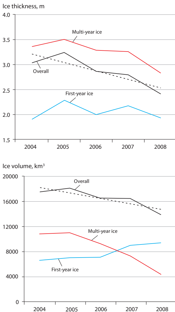
Figure 9.7. Decline in winter Arctic first-year (FYI) and multi-year (MYI) sea-ice thickness and volume between 2004 and 2008 derived from ICESat observations (Kwok et al., 2009). Overall thickness is the mean MYI and FYI thickness weighted by their areal coverage; overall volume is the sum of MYI and FYI volume.
