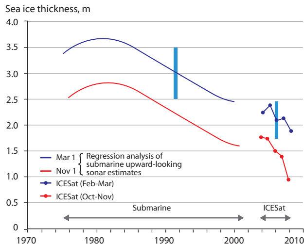
Figure 9.12. Interannual changes in winter and summer sea-ice thickness from Rothrock et al. (2008) and Kwok et al. (2009) centered on the ICESat campaigns. Blue error bars show residuals in the regression and quality of ICESat data (Kwok and Rothrock, 2009).
