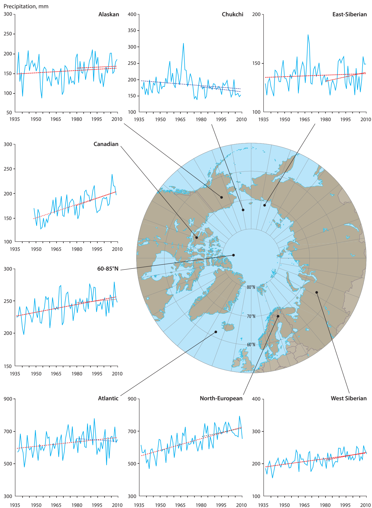
Figure 4.3. Long-term variability of total precipitation during the cold season (October to May when mean monthly temperature is below -2^{\circ}\text{C} ) for inland stations in different sectors of the Arctic (see Appendix 4.1 for sector definitions) together with their long-term (1936–2009) and short-term (1980–2009) linear trends; red line denotes positive trend and dark blue line negative trend. Precipitation amounts were calculated using a method of optimal averaging (Frolov, 2010). Results for Canada used the adjusted and homogenized precipitation dataset of Mekis and Hogg (1999) updated to 2008.
