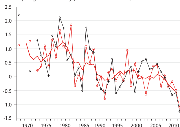
Figure 4.9. Time series of standardized snow-cover duration anomalies for the North American and Eurasian Arctic (relative to a 1988 to 2007 reference period) from the NOAA record for the (a) first half (autumn) and (b) second half (spring) of the snow season. Solid lines denote the five-year moving average. Source: Derksen et al. (2009).
