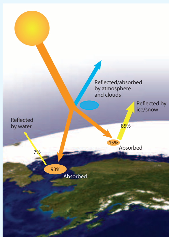
Figure 9.19. A simulated view from space of Arctic sea ice in August. The view shows the north coast of Alaska, an area of open water where the ice has melted, and the main ice pack.
