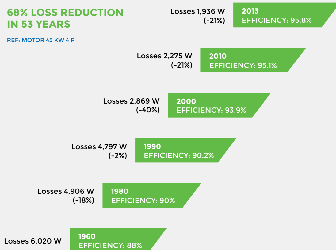
Figure 11: Induction motor energy efficiency improvements over the years— Example of 45 kW, 4-pole designs 19
