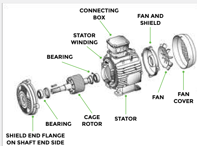
Figure 26: Assembly diagramme of an induction motor 84
