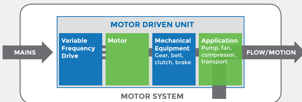
Figure 16: Motor-driven unit 39
