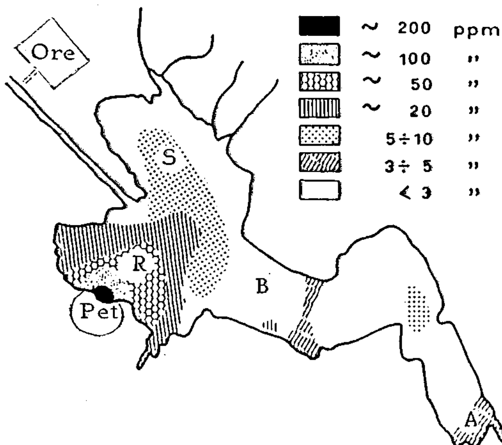
Figure 36. Mercury concentration in the surficial sediments of the S. Gilla Lagoon (Cagliari). A: entrance from the Gulf of Cagliari; Pet: petrochemical industry; Ore: ore processing industry; B, S, R: different zones in the lagoon (Porcu and Masala, 1983, modified).
