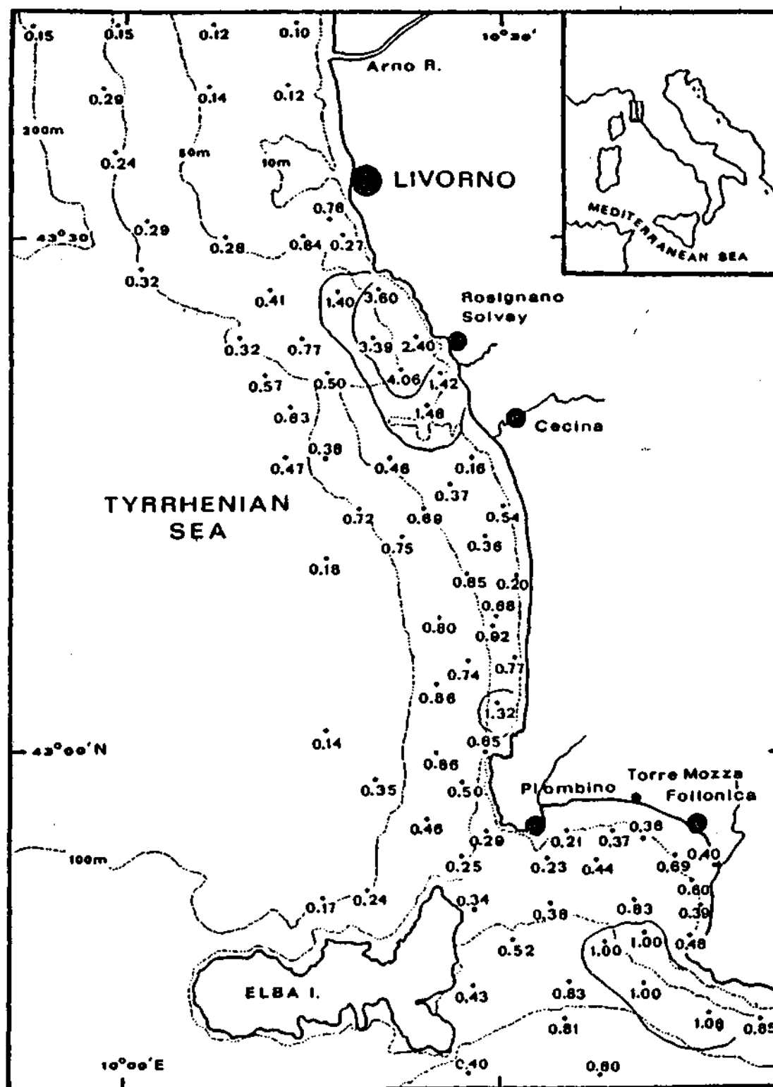
Figure 24. Distribution of mercury (mg Hg-T/kg DW) in surficial sediments from the western Italian coastline from the Arno to Follonica. (Baldi and Bargagli, 1984).
