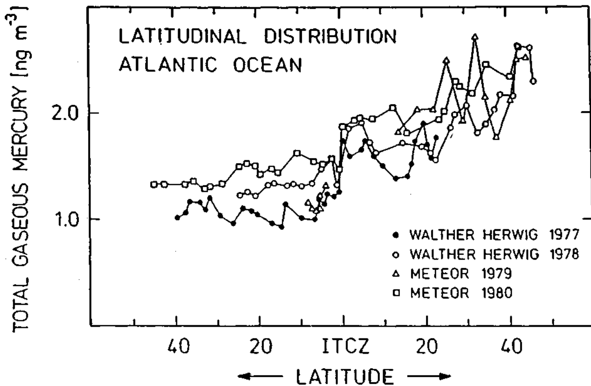
Figure 2. Latitudinal distribution of total "Gaseous Mercury" in surface air over the Atlantic (Slemr et al. , 1985). The midpoint presents the position of the Intertropical Convergence Zone (ITCZ). The Northern Hemisphere is to the right.
