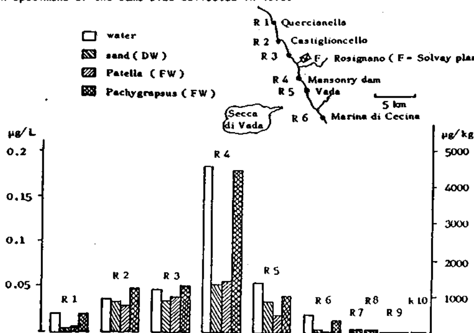
Figure 32. Mercury concentrations in sea water, sediments, Patella sp. and Pachygrapsus from the outfall area of the Solvay chlor-alkali plant in 1973 before the installation of a mercury waste treatment and in Patella and Pachygrapsus from several other Mediterranean sites as controls (R 7: Fiumicino, R 8: Montecarlo, R 9: S. Stefano, R 10: Talamone) (Bernhard and Renzoni, 1977).
