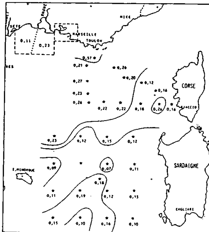
Figure 6. Mercury levels in sediments (mg/kg DM) in the Western Mediterranean (Arnoux et al. 1981).
