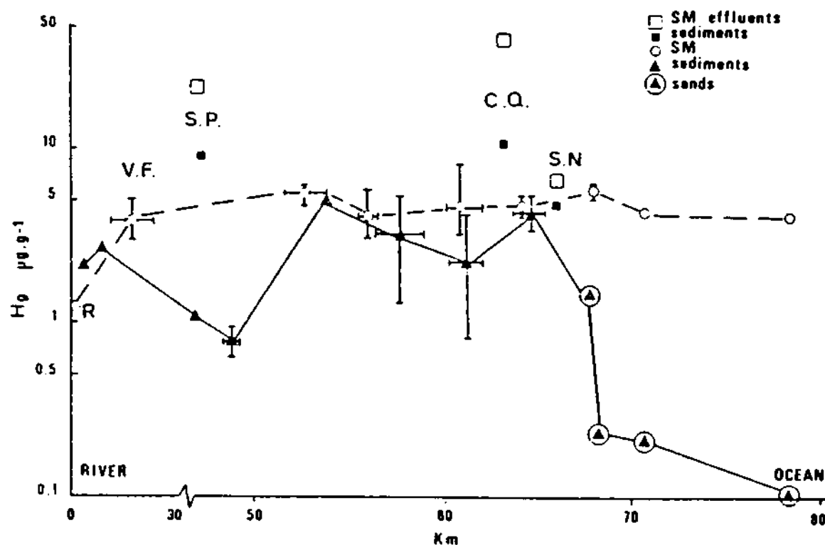
Figure 47. Longitudinal evolution of particulate mercury in the Tagus estuary
