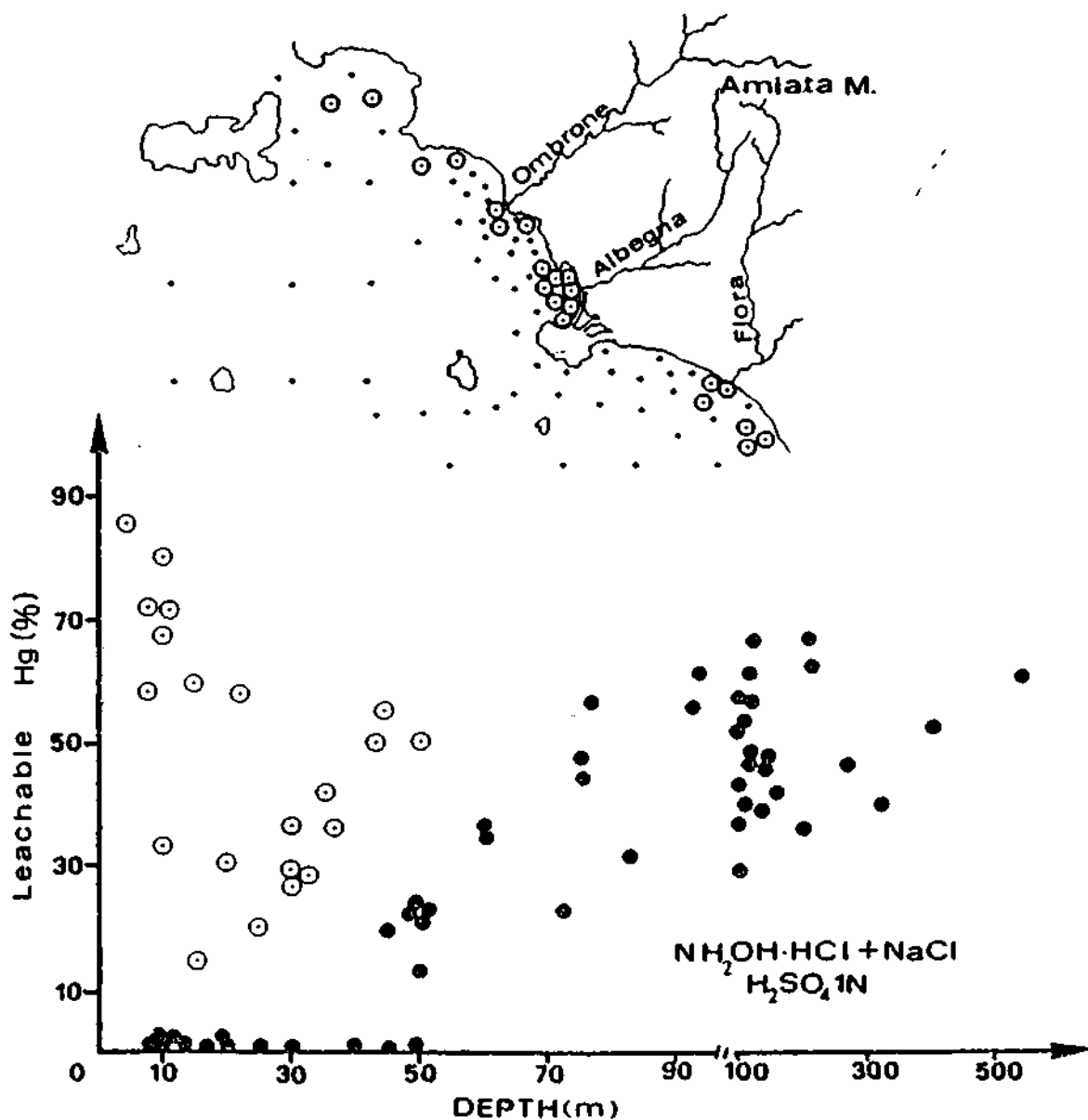
Figure 26. Percentage of acid-leachable (weakly bound) mercury in sediments affected by the Hg anomaly of the Mt. Amiata region (Baldi, 1986). The leaching solution used was \text{NH}_2\text{OH}\cdot\text{HCl} + \text{NaCl} in 1 \text{ NH}_2\text{SO}_4 .
