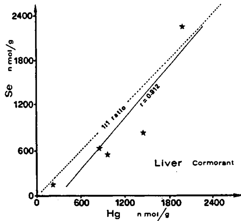
Figure 42. Relationship between selenium and mercury molar concentrations in brain and liver of marine birds. (Cottiglia et al. , 1984).
