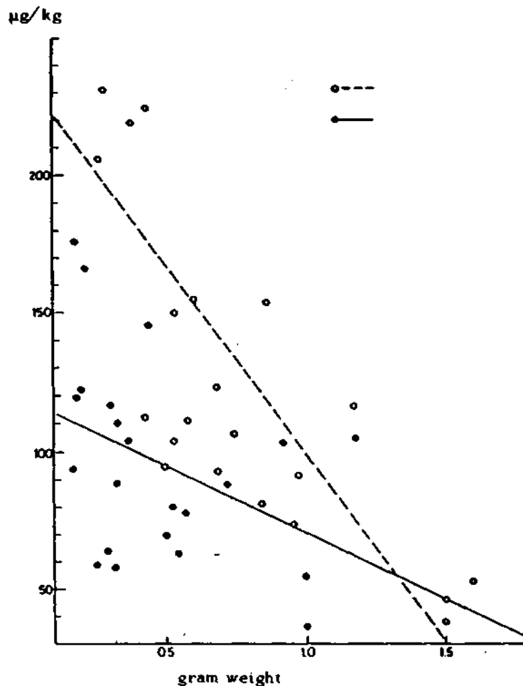
Figure 20. Relationship between methyl mercury and dry weight in oyster (open circle, dashed line) and mussels (full circle, continuous line) (Najdek and Bazulic, 1986).
