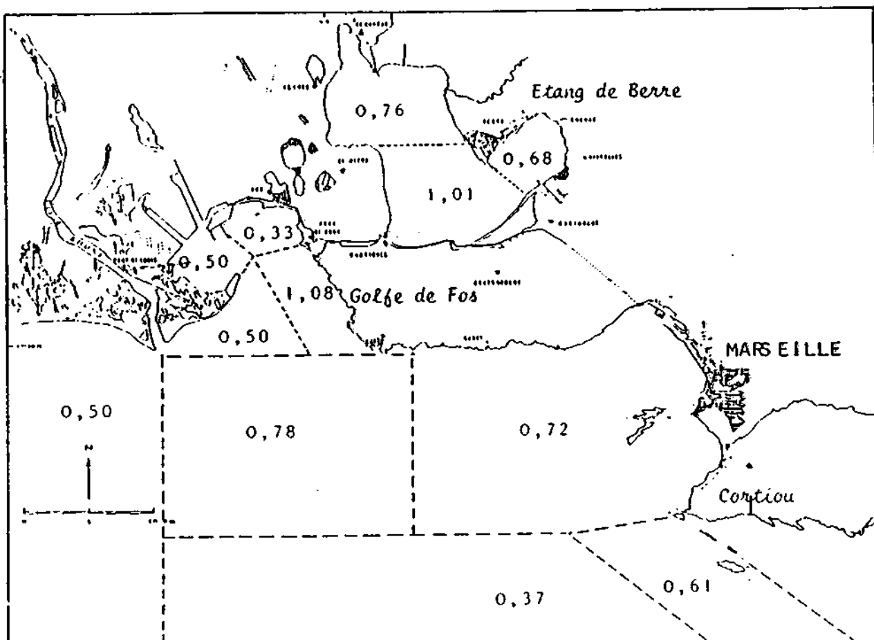
Figure 4. Mean mercury concentrations (mg/kg DW) in sediments near Marseilles (Arnoux et al. 1983).
