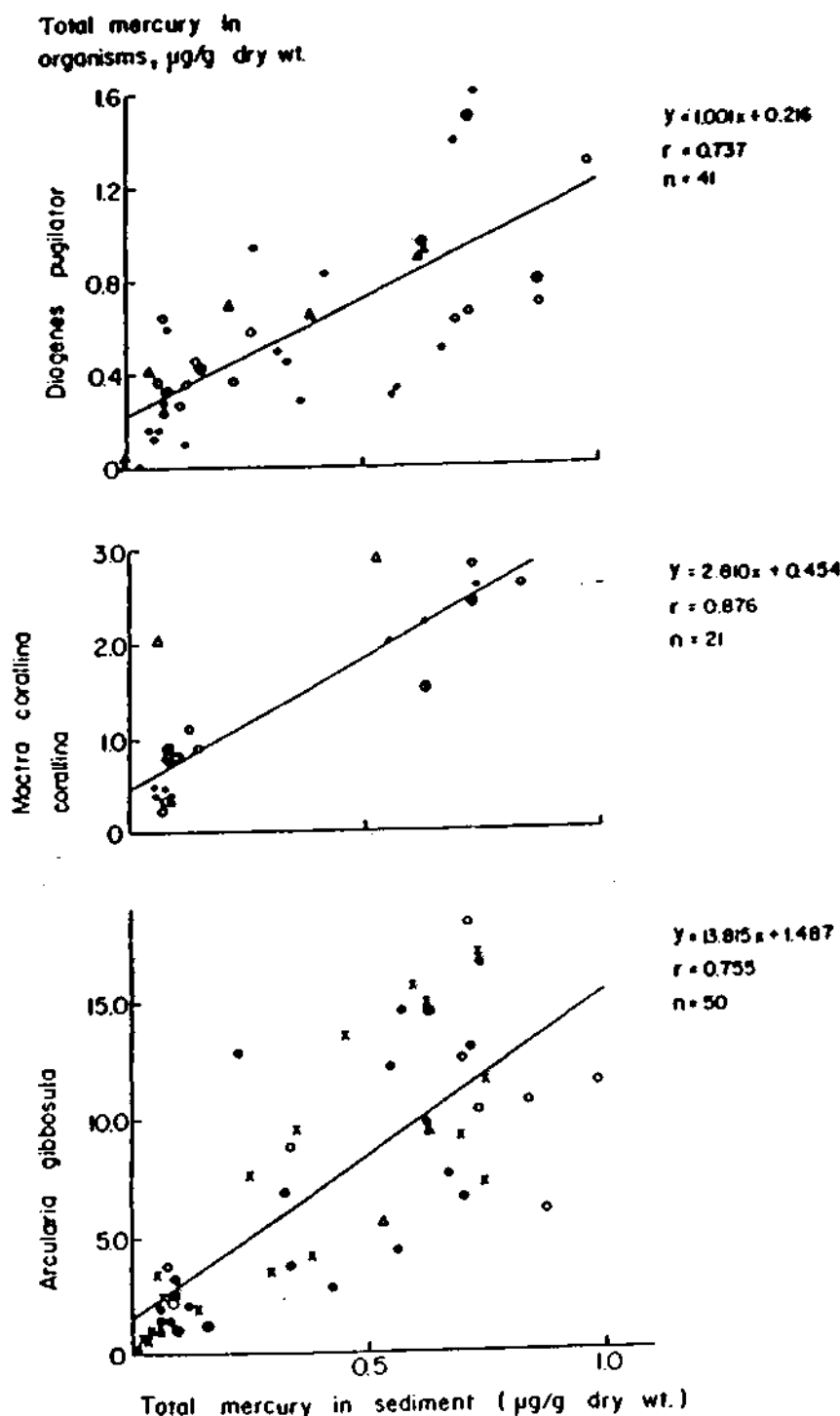
Figure 40. Relationship between mercury concentrations in three benthic organisms and surficial sediments from the coast of Israel (Hornung, 1986).
