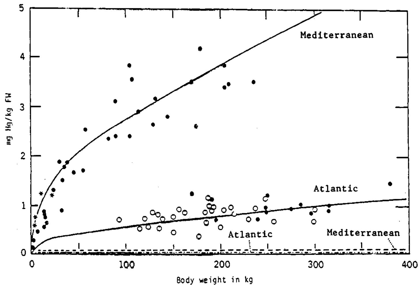
Figure 52. Total mercury concentrations in Thunnus thynnus from the Strait of Gibraltar (○), Tyrrhenian Sea (●) and Spanish coast (*). The continuous lines show total Hg concentrations calculated by a model; intermittent lines show inorganic Hg concentration calculated by a model (Bernhard, 1985).
