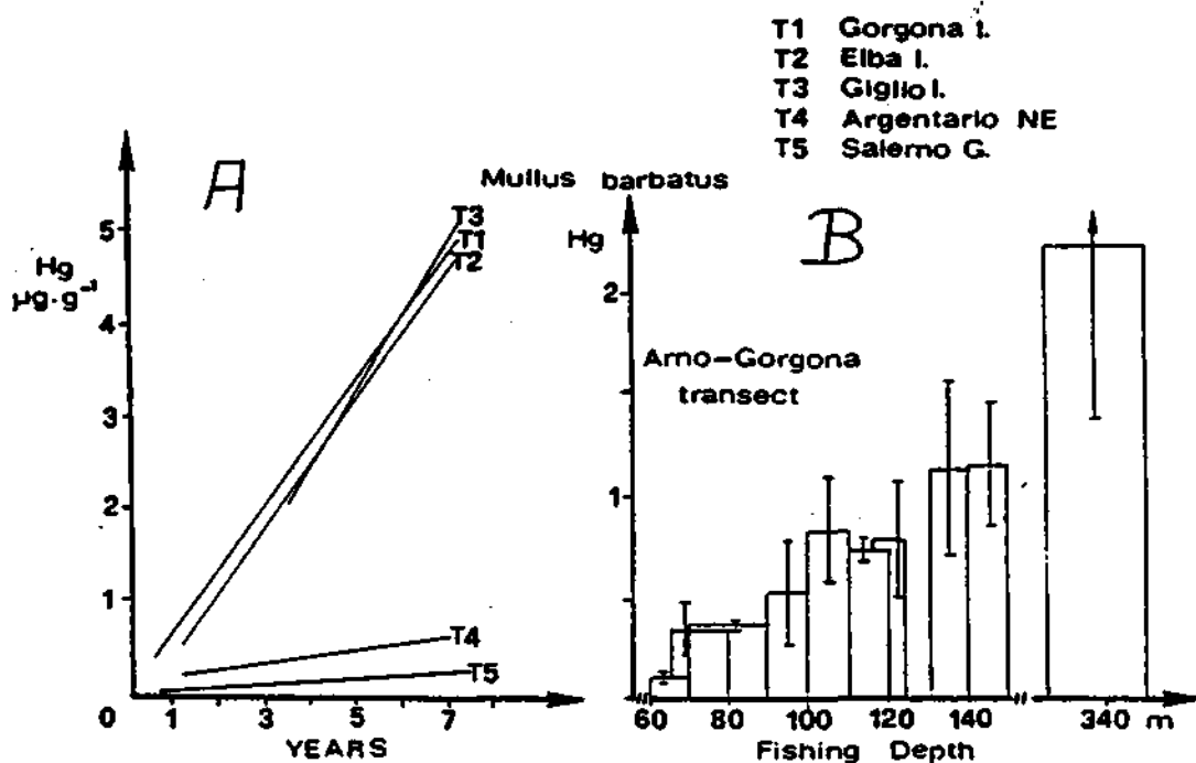
Figure 27. (A): Mercury concentrations versus age (years) correlations in Mullus barbatus from different locations of the western Italian coast and (B): mercury concentrations in specimens of the same size versus fishing depth along a transect offshore of the river Arno (B). (Baldi, 1986).
