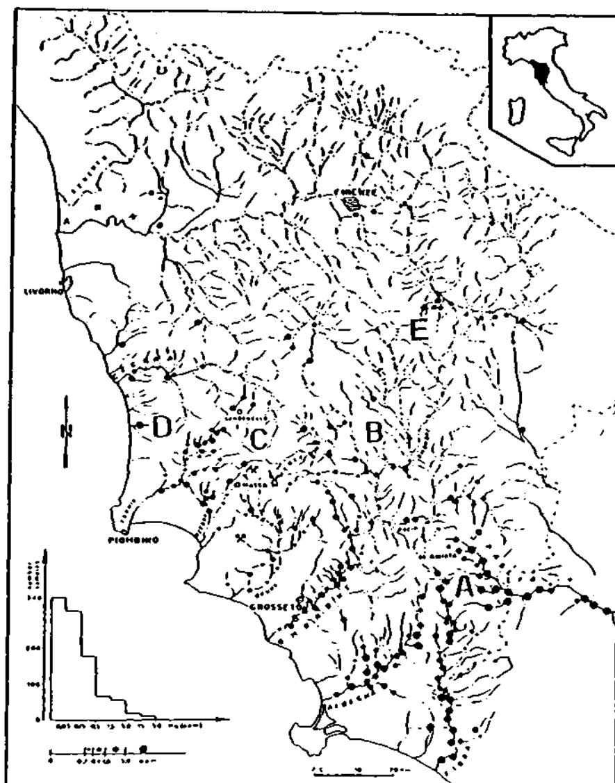
Figure 23. Distribution of mercury in river sediments around the mercury anomaly of Mt. Amiata (Tuscany) (Dall'Aglia, 1974).
