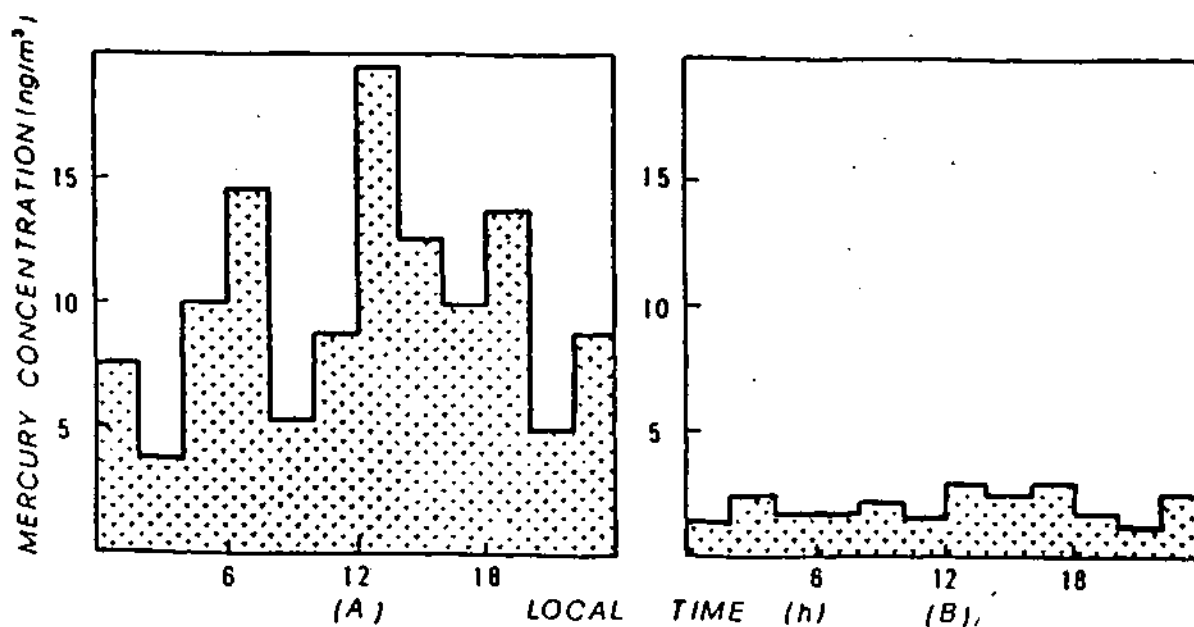
Figure 1. Diurnal variation of mercury concentrations in an urban (A) and a rural (B) area (Ferrara et al. 1982).
