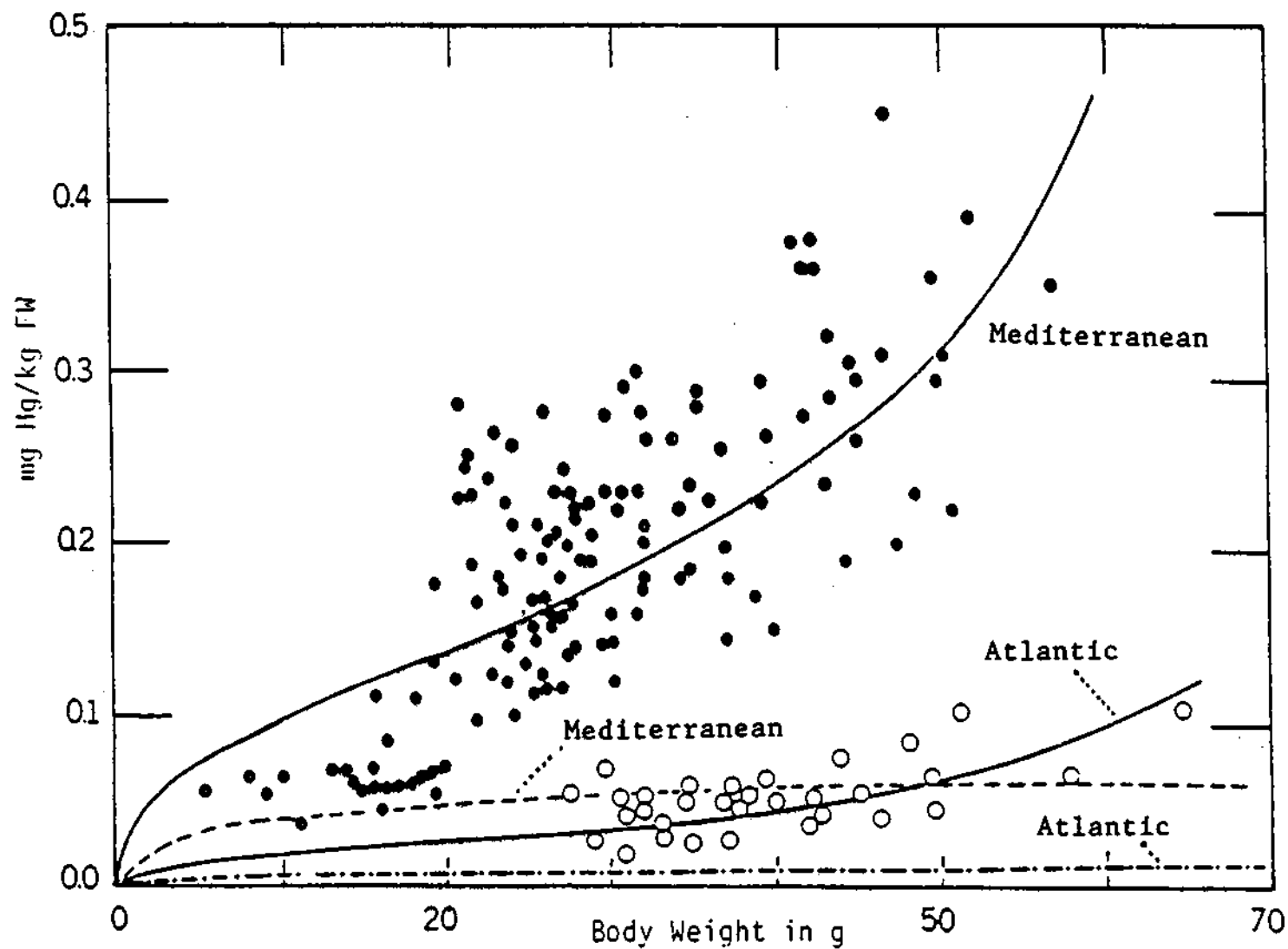
Figure 53. Total mercury concentrations in Sardinia pilchardus from the Strait of Gibraltar (○) and Tyrrhenian Sea (●). The continuous lines show total Hg concentrations calculated by a model; intermittent lines show inorganic Hg concentration calculated by a model (Bernhard, 1985).
