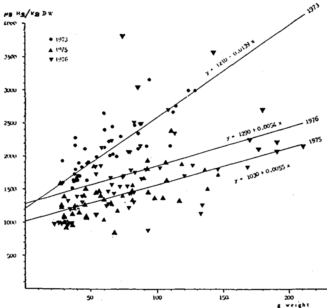
Figure 33. Mercury concentration versus weight in Scorpaena porcus from the banks of Vada before (1973) and after (1975 and 1976) waste treatment began in the Solvay chlor-alkali plant (Renzone, 1977).
