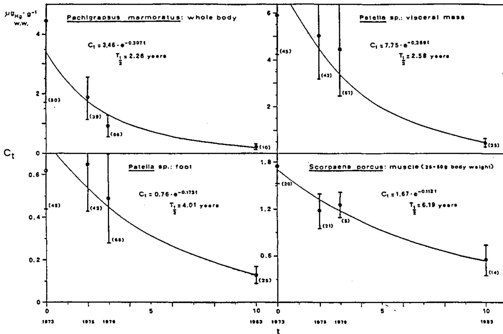
Figure 35. Recovery trends estimated from different "bioindicators" in Solvay outfall area (Bacchi et al. 1986). C_t represents the Hg concentration in the indicator organisms according to a one compartment model, and T_{1/2} biological half-time of mercury in organisms.
