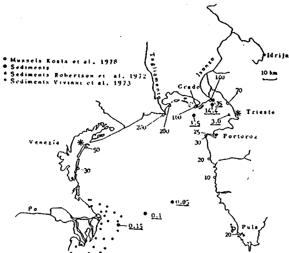
Figure 30. Mercury concentrations ( \mu\text{g Hg-T/kg DW} ) in sediments of the River Isonzo (Soca and in marine sediments (underlined values) and in Mytilus ( \mu\text{g Hg-T/kg FW} ) from the Gulf of Trieste. Sediment levels in the Po Delta: 0.4 (0.07 to 0.97) mg Hg-T/kg DW. Data from Kosta et al. 1978; Robertson et al. 1972; Viviani et al. 1973).
