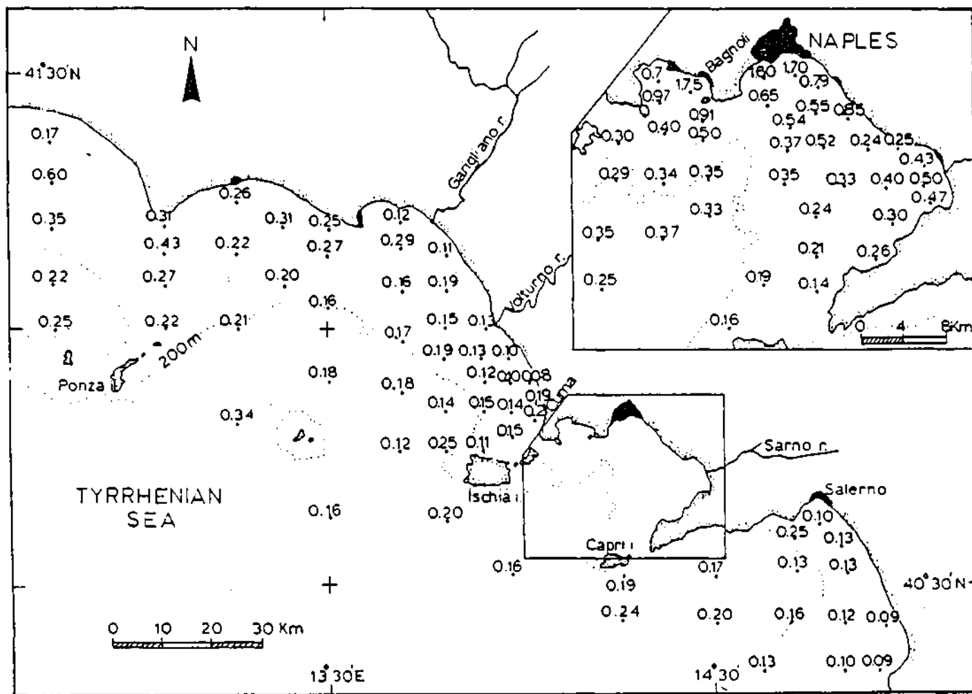
Figure 7. Mercury concentrations (mg/kg DW) in the top 3 cm of sediments in the Gulf of Naples (Baldi et al. 1983)
