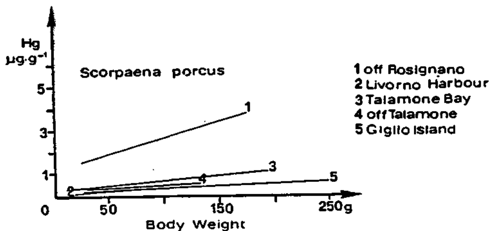
Figure 28. Mercury concentrations (mg Hg-T/kg FW) in Scorpaena porcus from the western Italian coast (Baldi, 1986) versus body weight (g).
