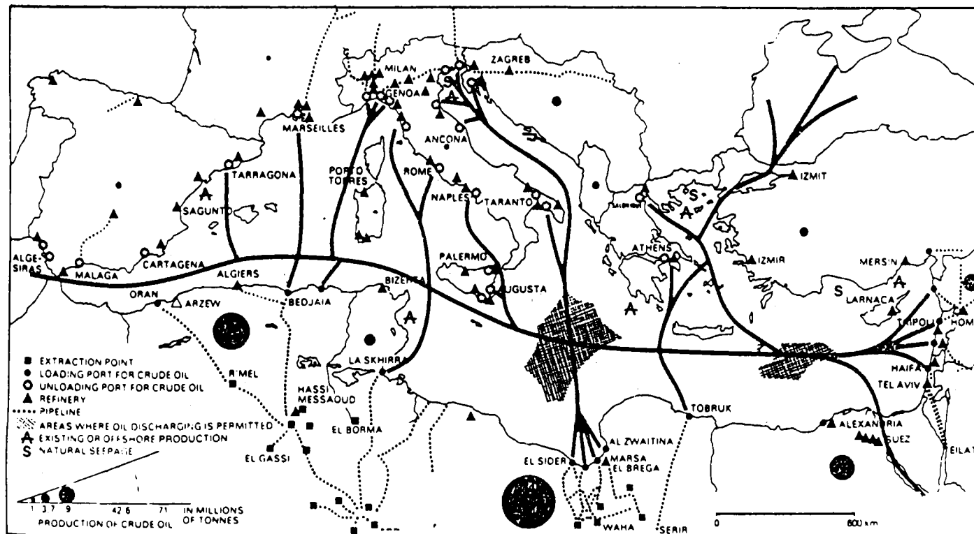
Figure 3. Production and transport of oil in the Mediterranean Sea. (From Le Lourd 1977).
