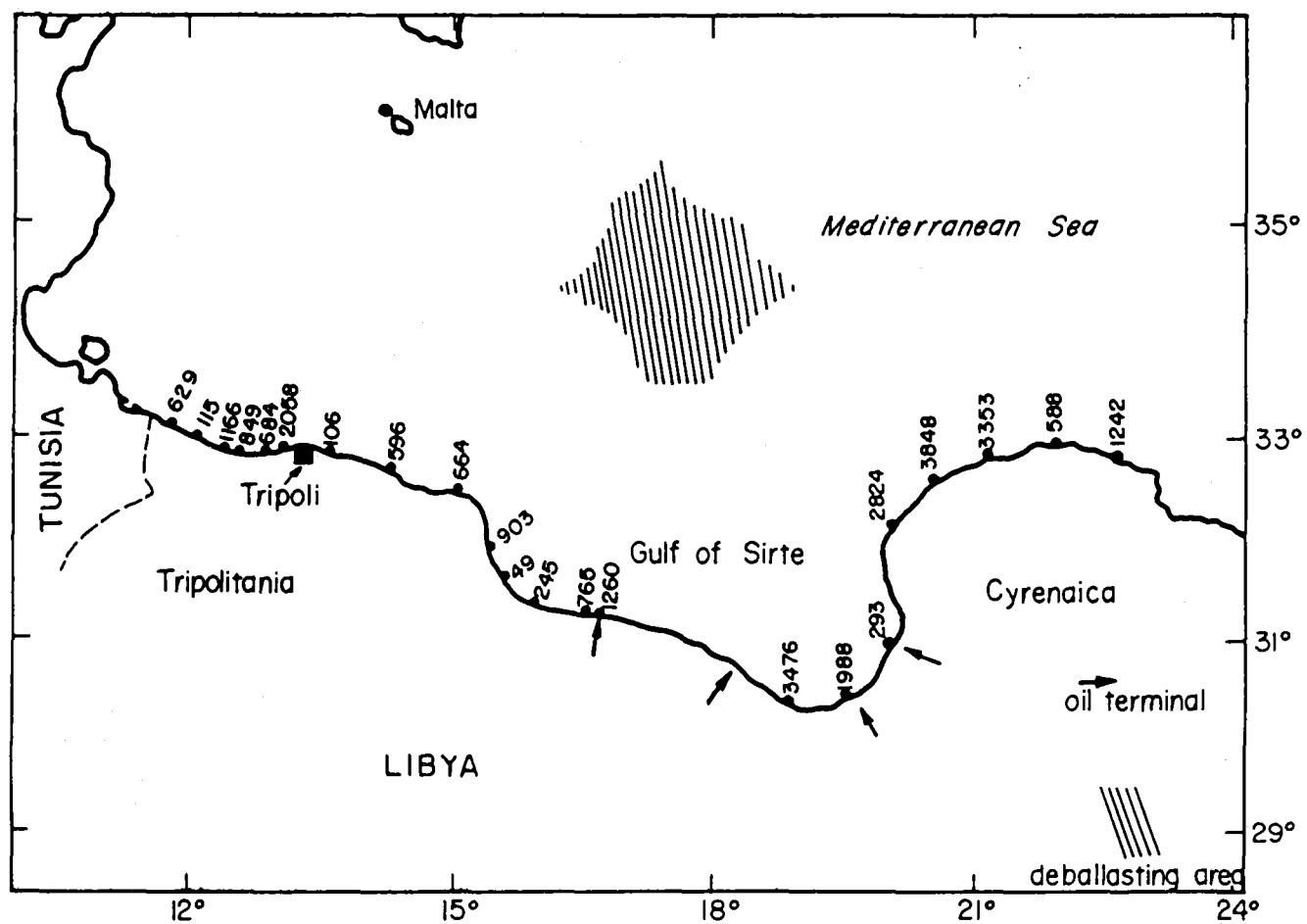
Figure 5. Quantitative distribution of tar in g/m on the Libyan coast in 1980/81. (From El-Ghirani, 1981).
