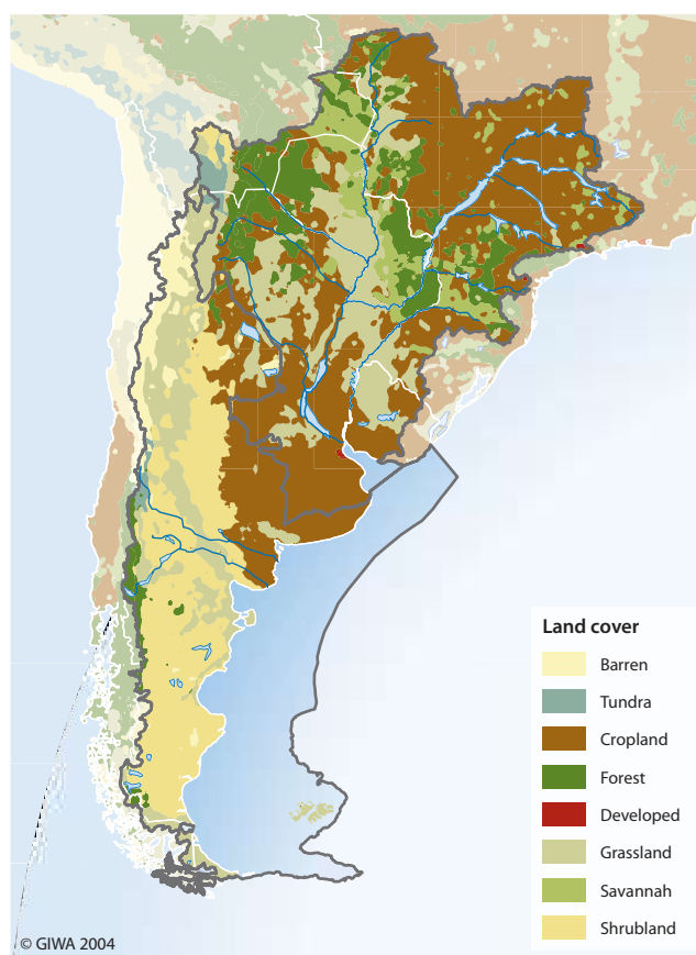
Figure 6 Land cover. (Source: Data from Loveland et al. 2000)
