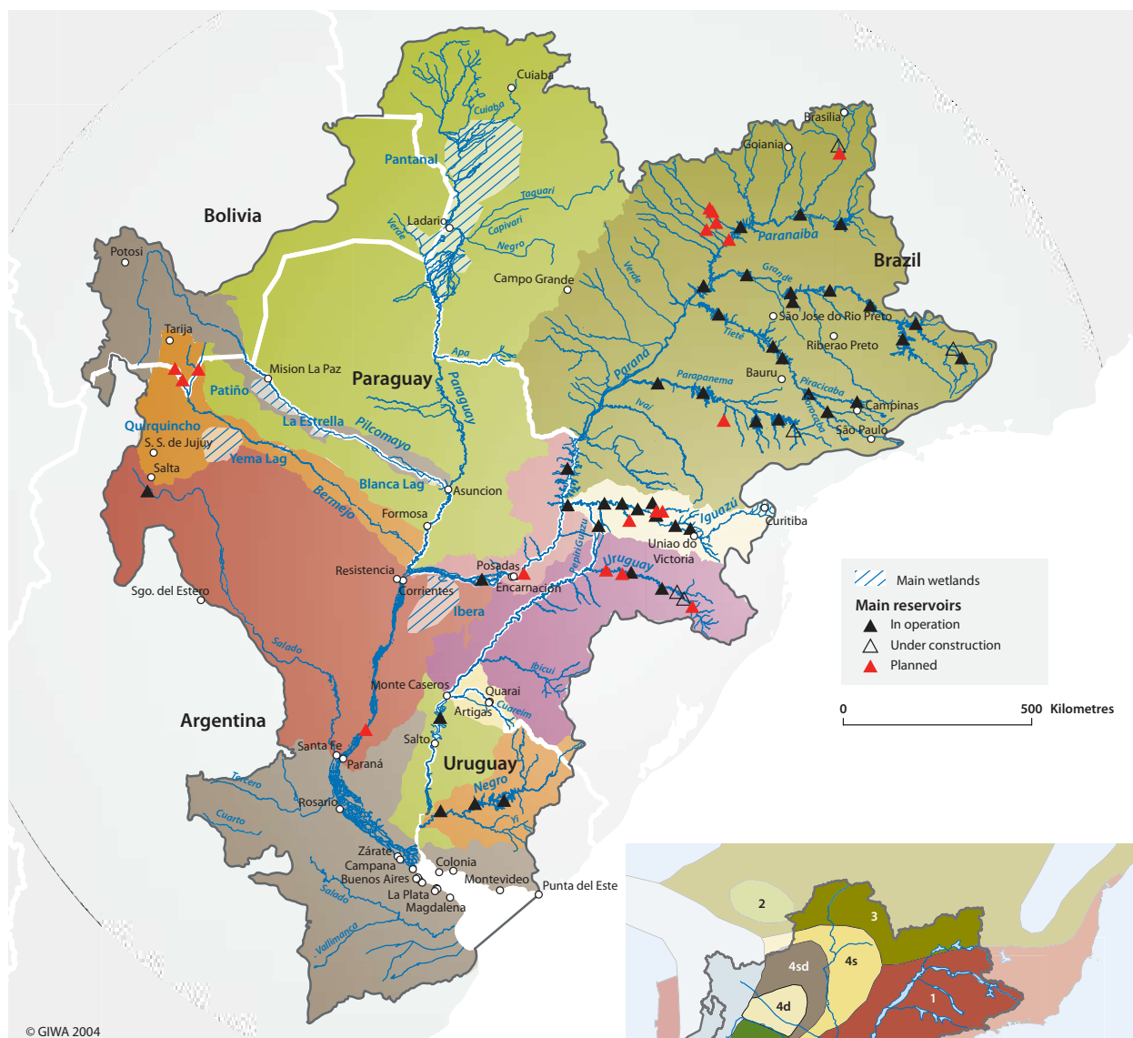
Figure 3 The drainage basins of the tributaries comprising La Plata River Basin. (Source: ANEEL 2000)
