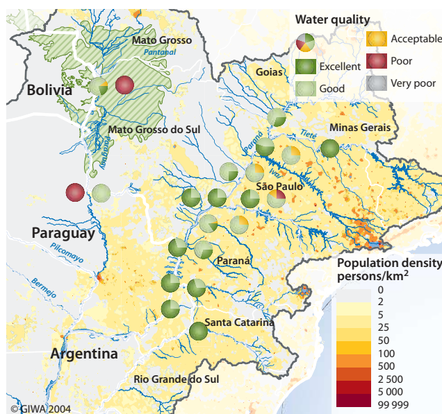
Figure 14 Water quality in the Brazilian area of La Plata River Basin. (Source: ANEEL 2001)
