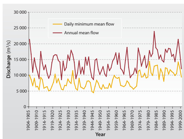
Figure 13 Daily minimum mean and annual mean flow of Paraná River at Tunel (Paraná-Santa Fe, Argentina). (Source: SSRH 2000)
