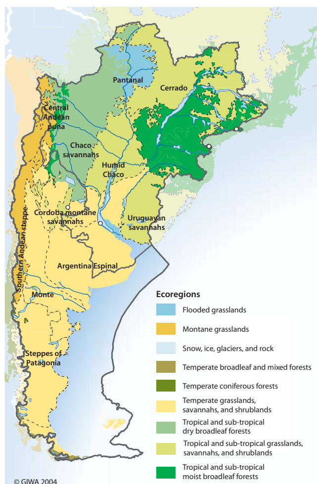
Figure 5 Ecoregions. (Source: Olson et al. 2001)
