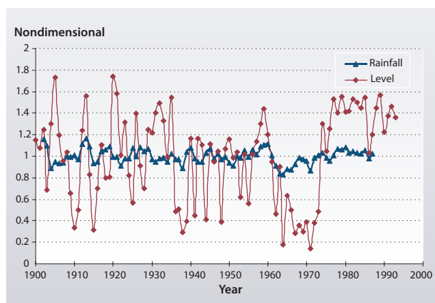
Figure 12 Variation in annual water level at Ladário (Upper Paraguay) and rainfall (3 year moving average) at Cuiabá (Paraguay River). (Source: Tucci & Clarke 1998)
