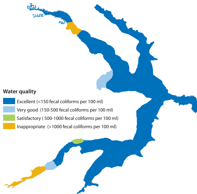
Figure 17 Water quality for leisure use in Paranoa Lake, Brasilia (Brazil). (Source: CAESB 2002)
