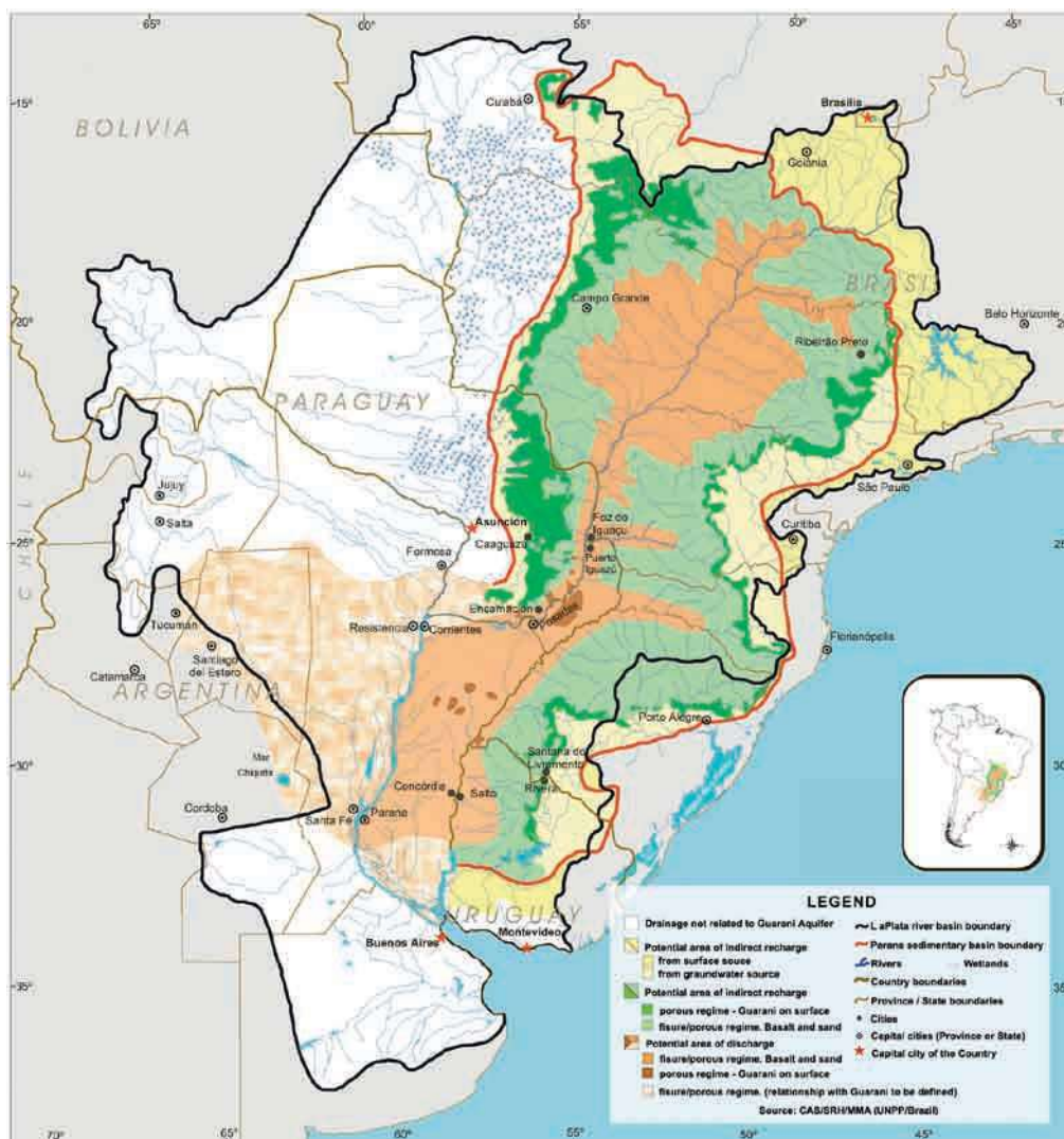
Figure 8 Guaraní Aquifer. (Source: CAS/SRH/MMA (UNPP/Brazil))
