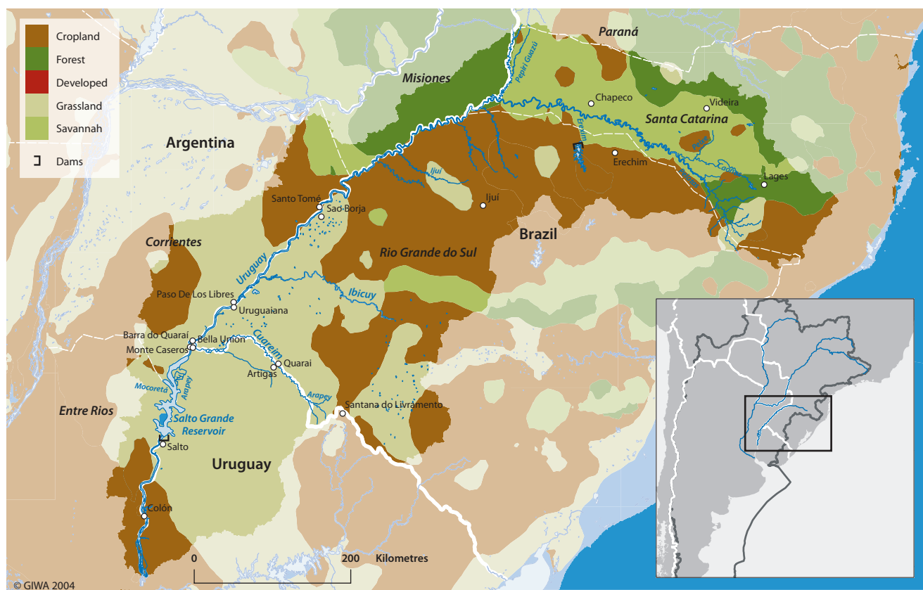
Figure 29 Uruguay River Basin. (Source: Loveland et al. 2000)
