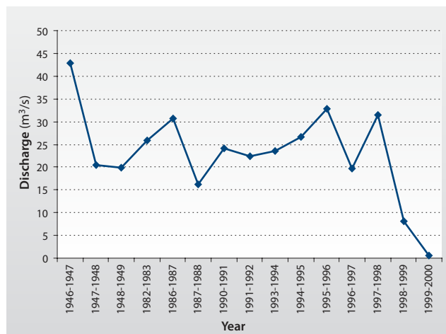
Figure 22 Annual discharge at Puente Camino Buen Pasto gauging site. Senguerr River near Colhué Huapi Lake. (Source: SSRH-EVARSA 2000)
