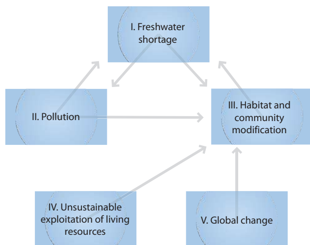
Figure 28 Links between the GIWA concerns.
