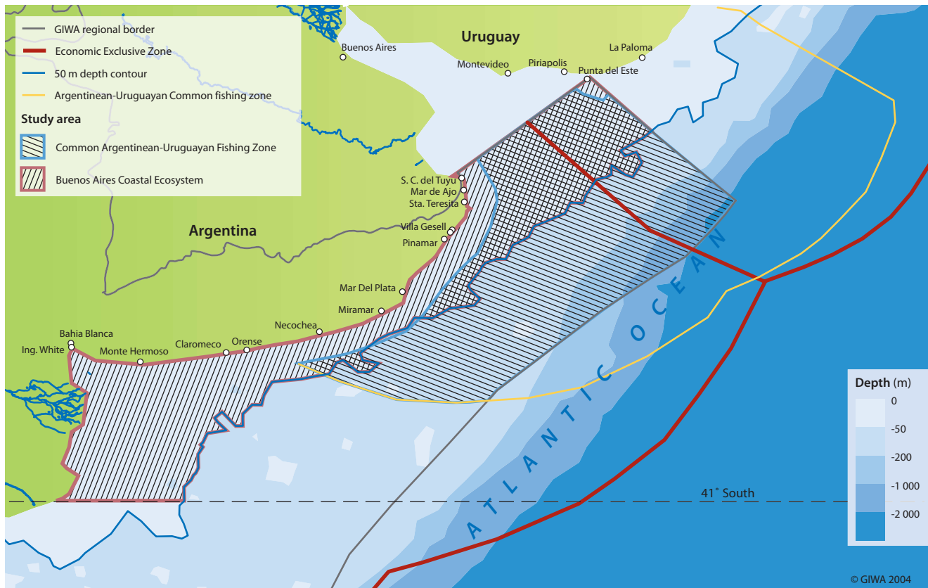
Figure 32 Buenos Aires Coastal Ecosystem and Argentinean-Uruguayan Fishing Zone and their relative location in South Atlantic Drainage System.
