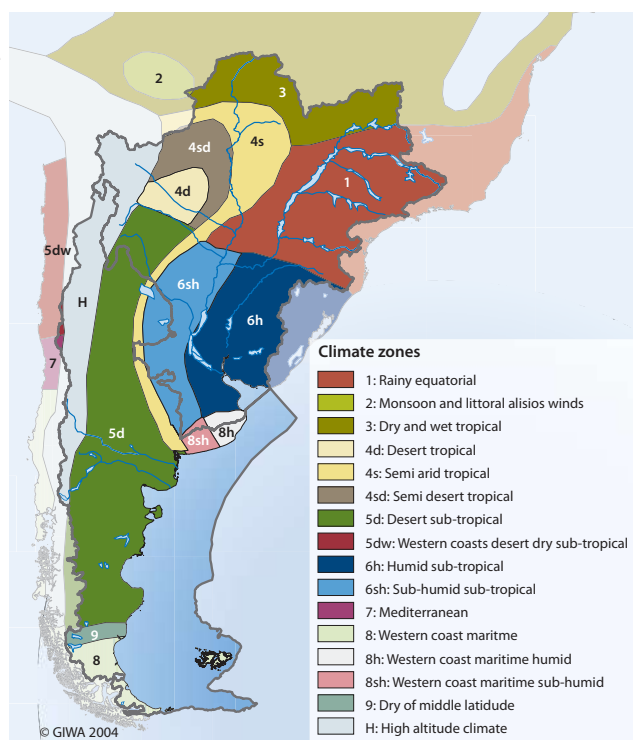
Figure 4 Climate zones. (Source: CIAT 1998, Strahler & Strahler 1989)
