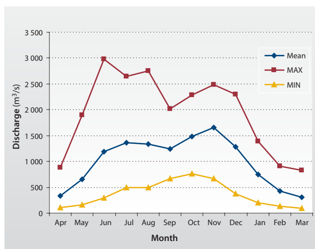
Figure 23 Discharge at Paso Córdoba gauge (province of Río Negro) before operation of Cerros Colorados System (1978). (Source: SSRH-EVARSA 2000)
