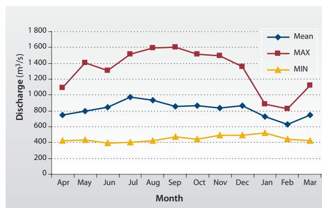
Figure 24 Discharges at Paso Córdoba gauge (province of Río Negro) after operation of Cerros Colorados System (1978). (Source: SSRH-EVARSA 2000)
