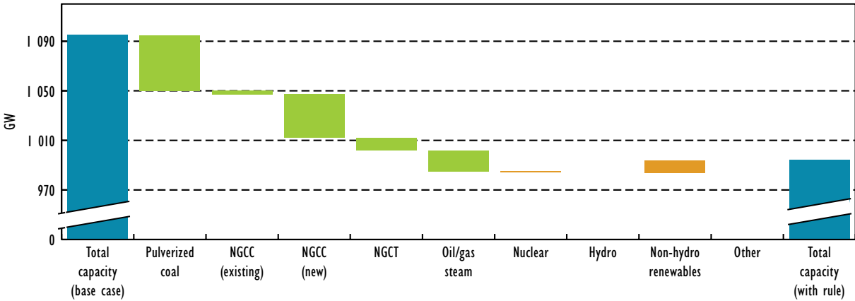
Figure 4.3.4 Change in US electricity generation capacity in 2030, by technology, from base case (GW)
