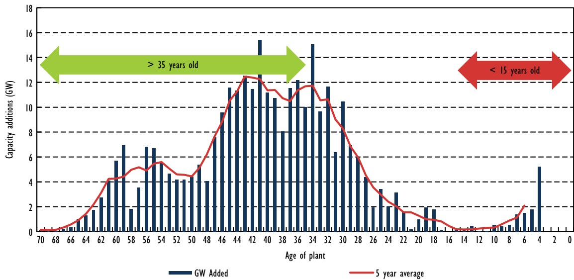
Figure 1.3 Age of current (2014) capacity of coal-fired power plants in the United States
