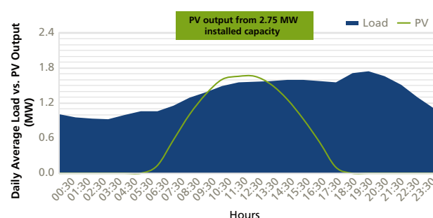
Figure 5: Daily average load vs. possible PV output (Puerto Leguizamo)
