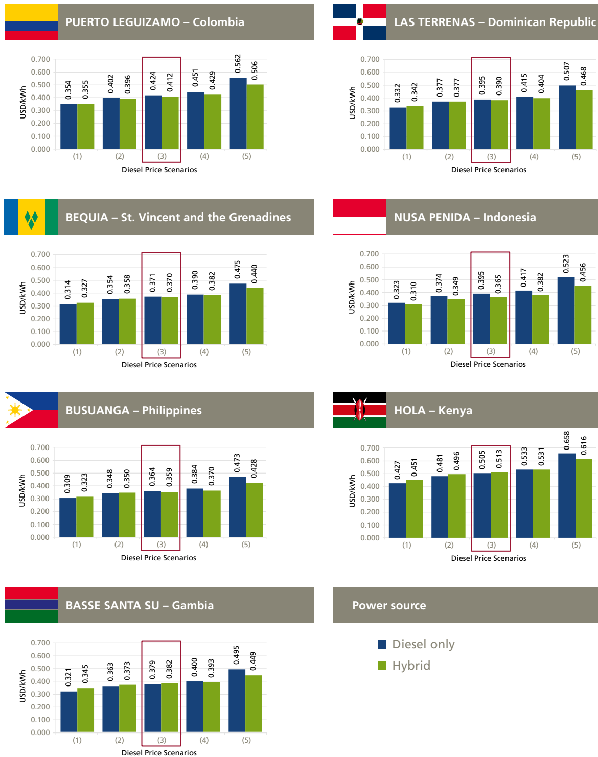
Figure 41: LCOEs for different diesel price scenarios
