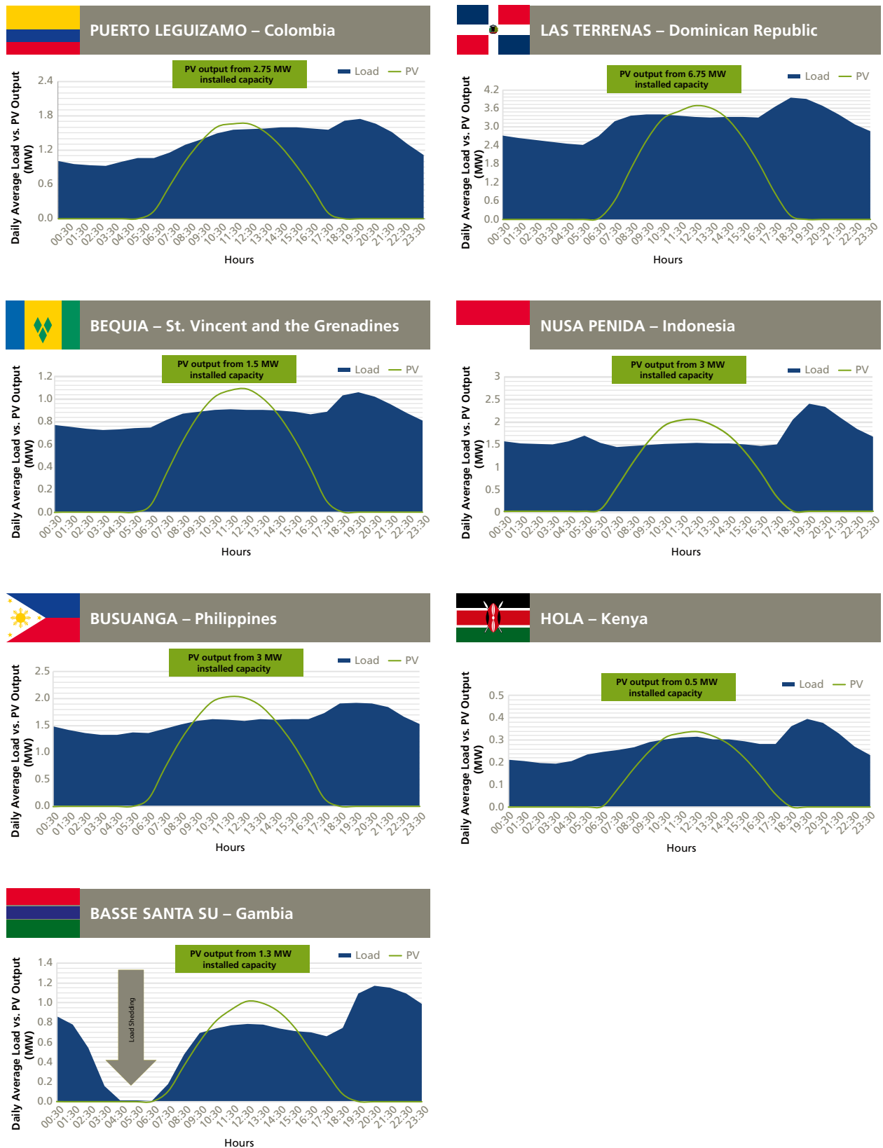
Figure 23: Daily average load vs. possible PV output
