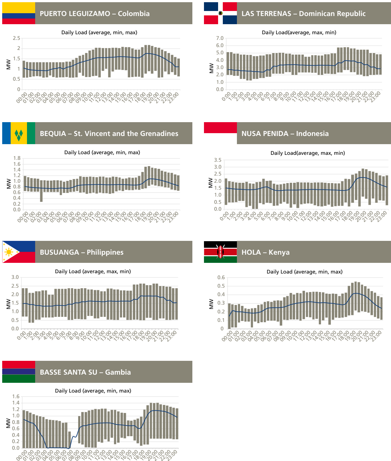
Figure 19: Load profiles (daily average, min, max)
