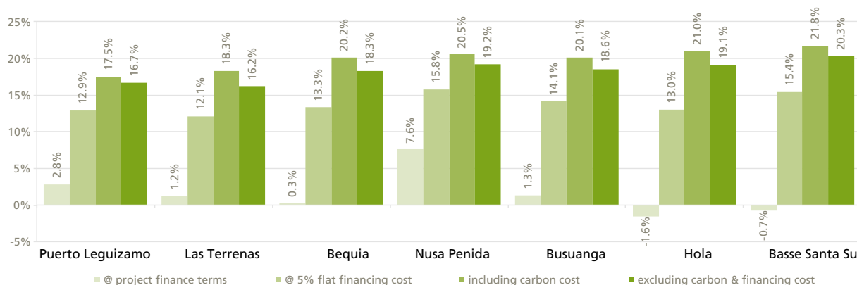
Figure 35: Relative cost advantage of hybridisation
