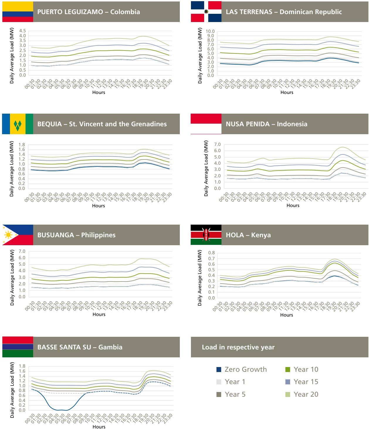
Figure 26: Load profiles for growth scenario
