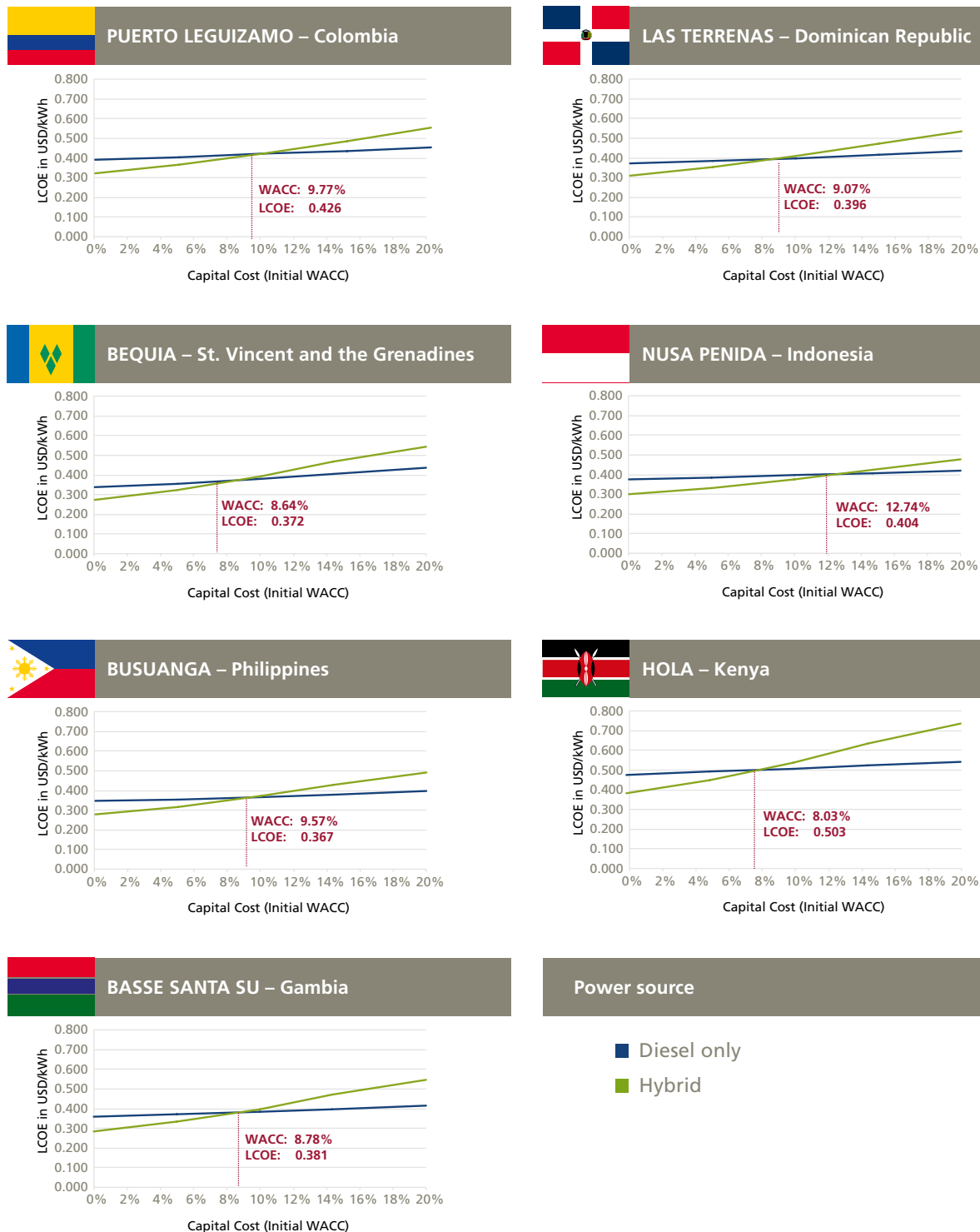
Figure 46: LCOE as a function of financing costs (break-even WACC)
