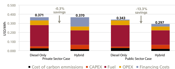
Figure 10: LCOE breakdown for private vs. public financing costs (Las Terrenas)
