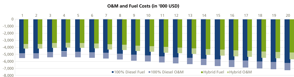
Figure 29: Operating costs of diesel and hybrid (in USD '000)
