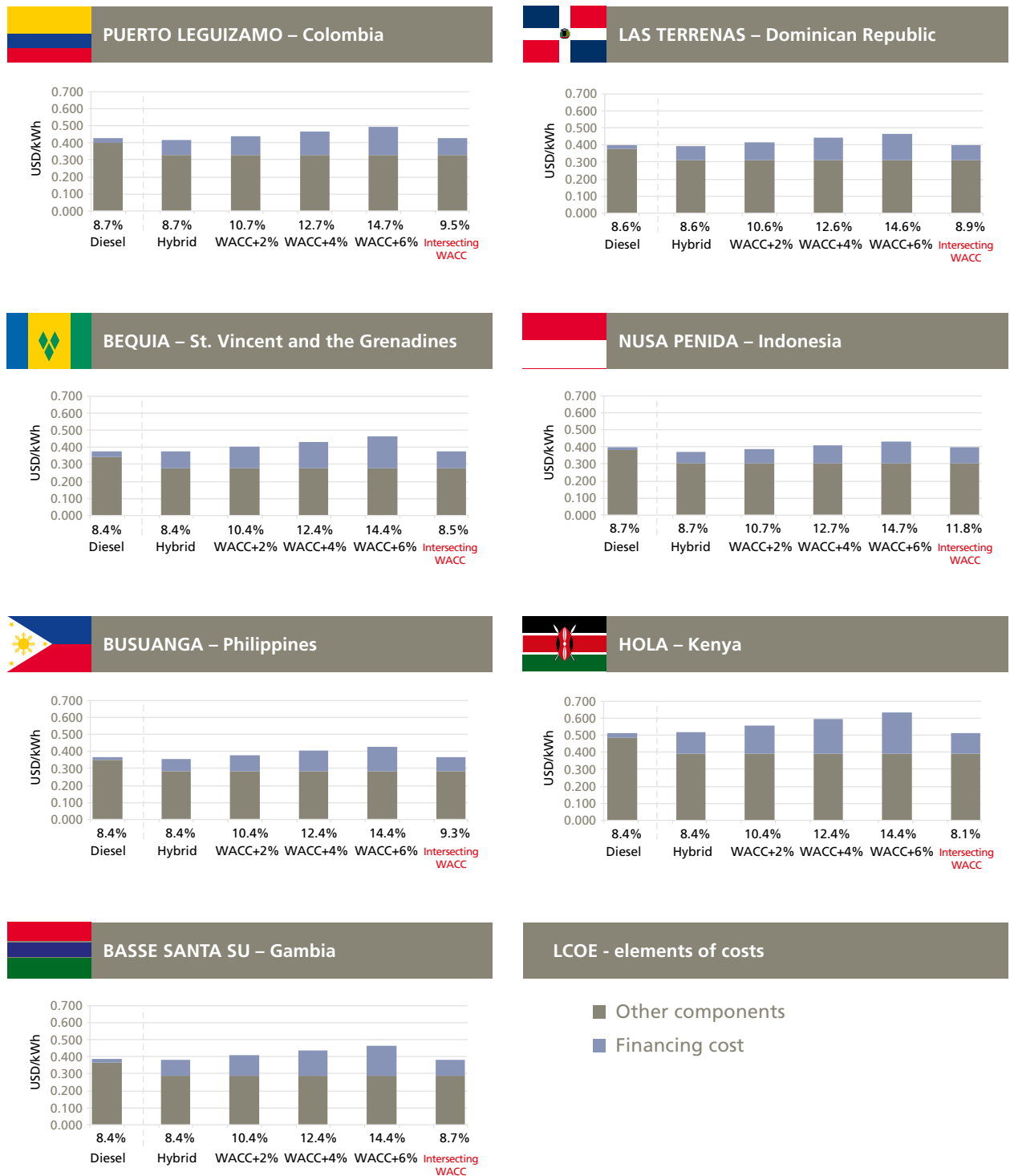
Figure 48: Impact of different risk margins on LCOE
