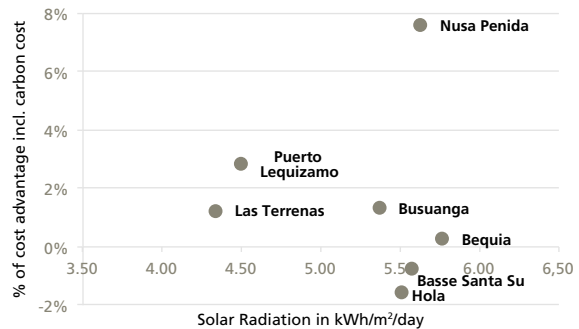
Figure 37: Relation of solar radiation and LCOE
