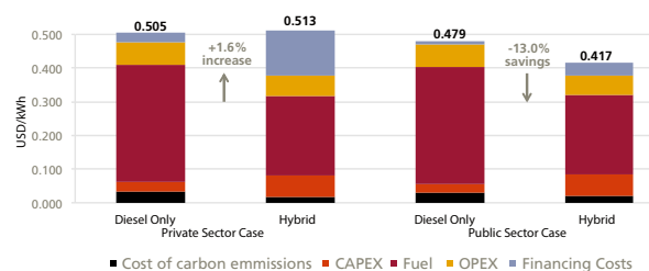
Figure 16: LCOE breakdown for private vs. public financing costs (Hola)
