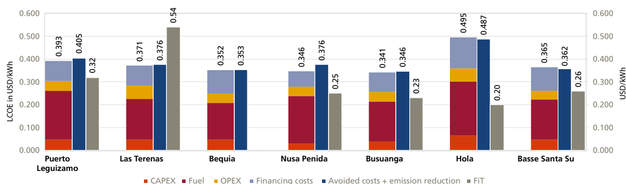
Figure 53: LCOE for hybrid systems excluding cost of carbon under no-growth scenario
