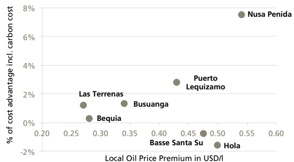
Figure 38: Relation of local diesel price and LCOE
