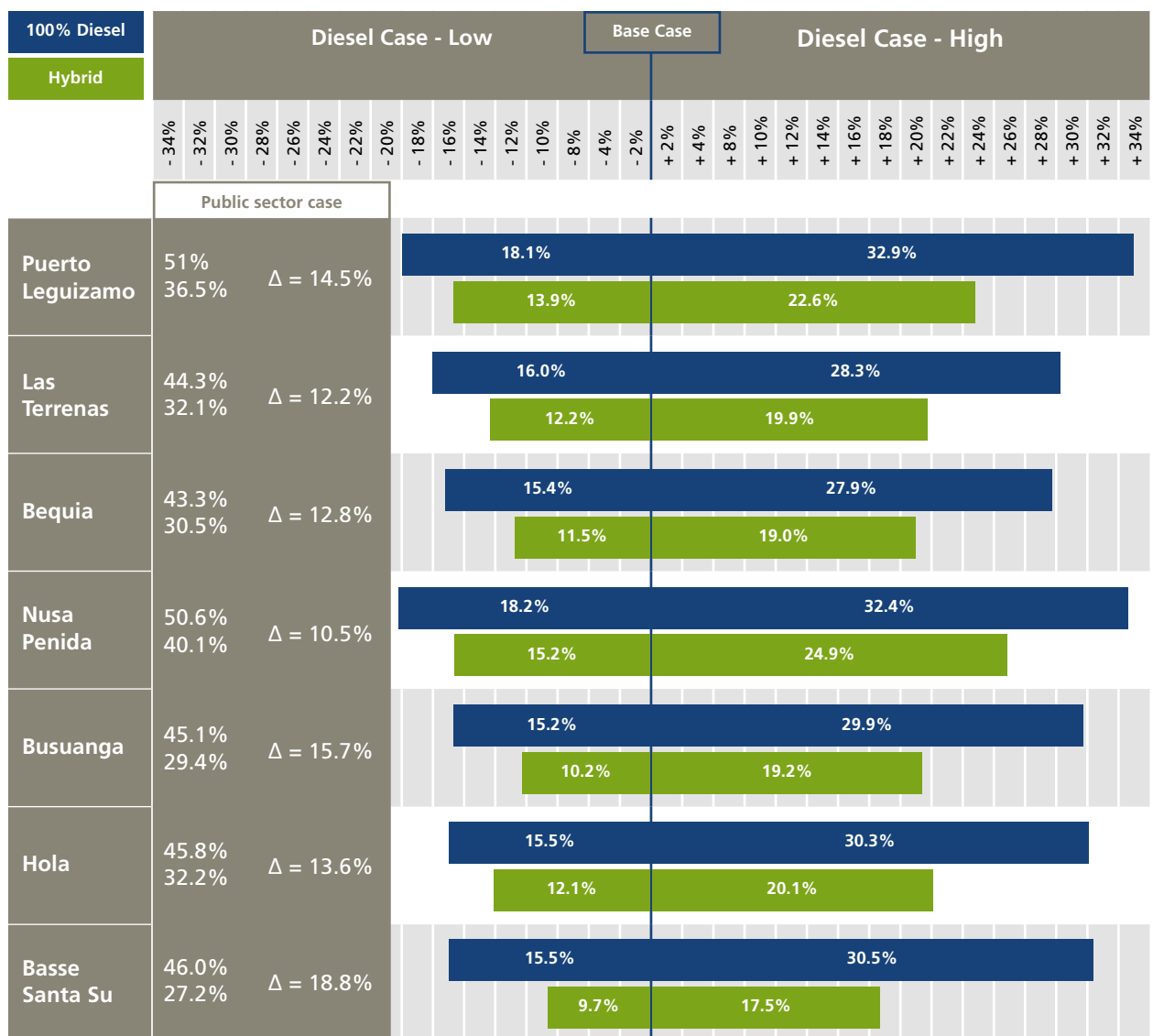
Figure 43: Volatility of LCOEs for different diesel price scenarios
