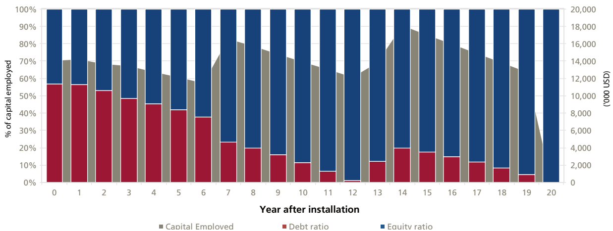
Figure 62: Debt repayment; growth case (in USD '000, Nusa Penida)
