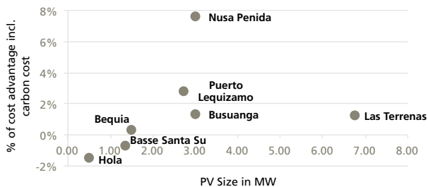
Figure 36: Relation of PV size and LCOE
