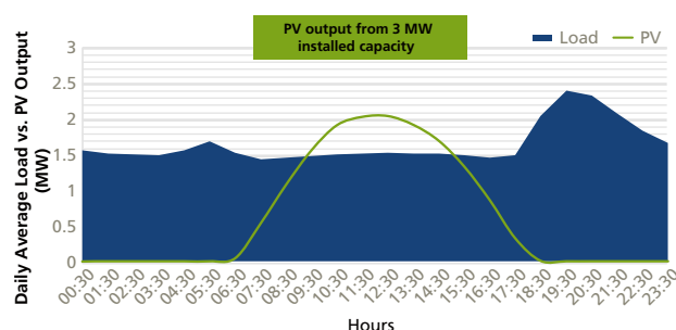
Figure 11: Daily average load vs. possible PV output (Nusa Penida)
