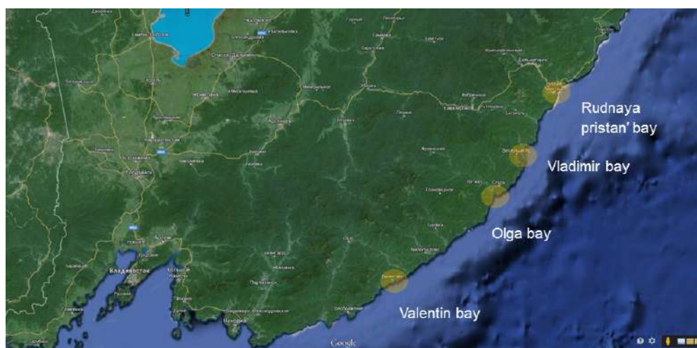
Figure 31. Marine litter concentration area in eastern coastal water area.
