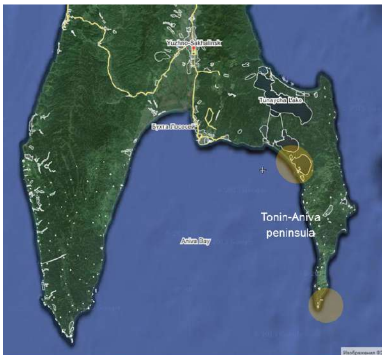
Figure 35. Marine litter concentration area in the Aniva gulf coastal water area.
