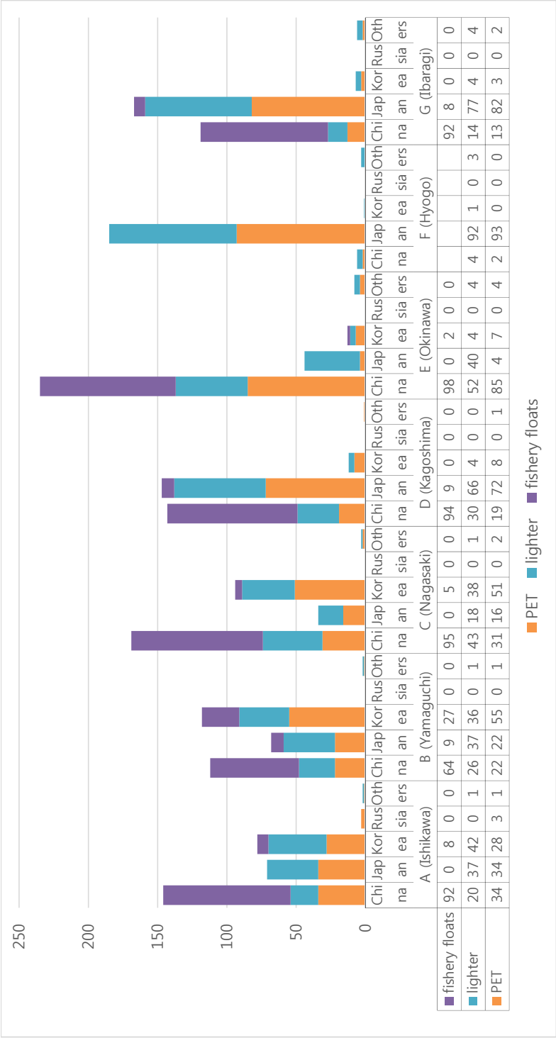
Figure 11. Cumulative ratios of foreign-originated floating marine litters collected at surveyed beaches of Japan.
