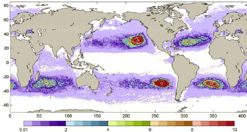
Figure 1. Convergent zones for surface tracers (Dohan and Maximenko, 2010).
