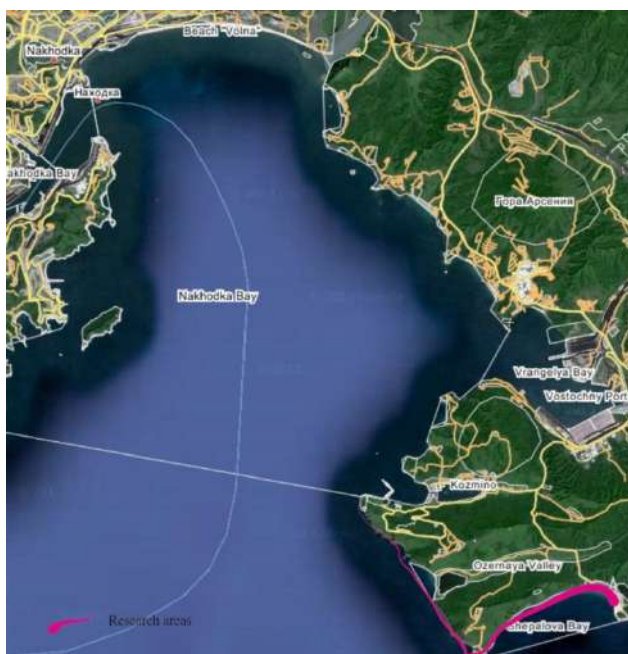
Figure 41. Research areas in the south part of the Primorsky region.
