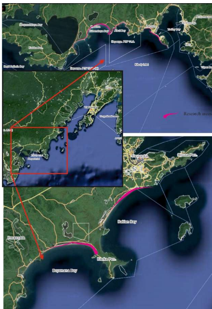
Figure 40. Research areas in the south-west part of Primorsky region.
