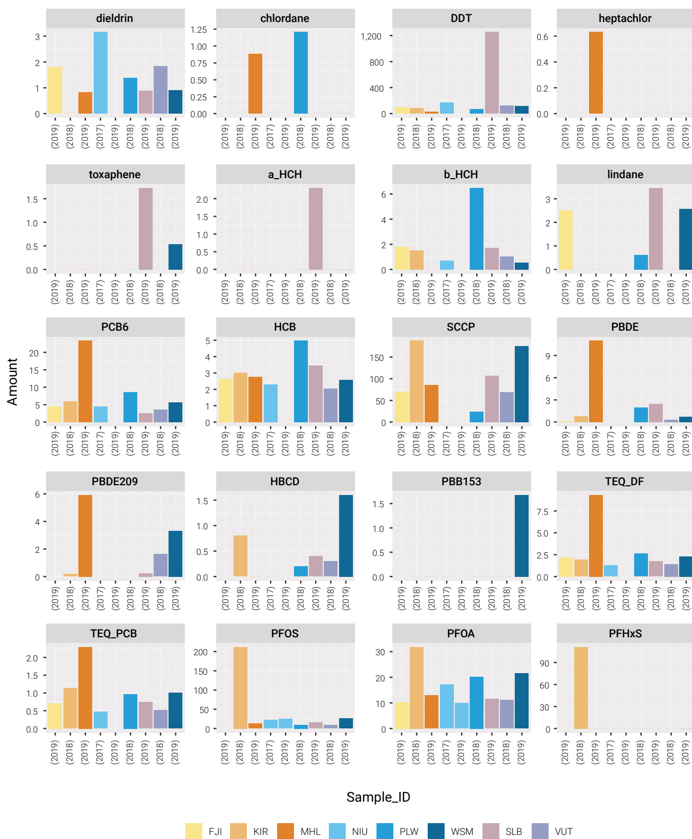
Figure 33: Human milk: Scaled barplots by POPs with concentrations by country (pg TEQ/g lipid for the dl-POPs, pg/g f.w. for PFAS; all other in ng/g lipid)
