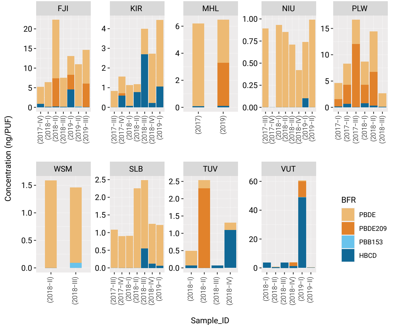
Figure 15: PAS/PUF: Stacked bar graphs for brominated POPs by country and sample (n=49)
