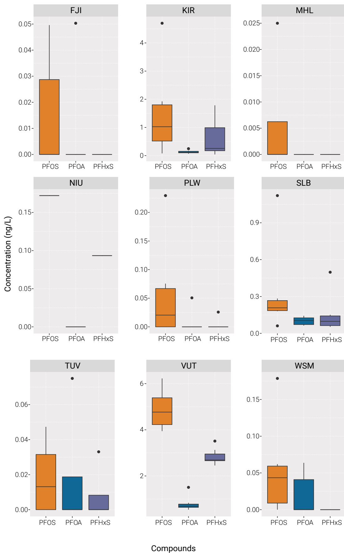
Figure 31: Water: Amounts according PFOS, PFOA, PFHxS by country and year (ng/L)
