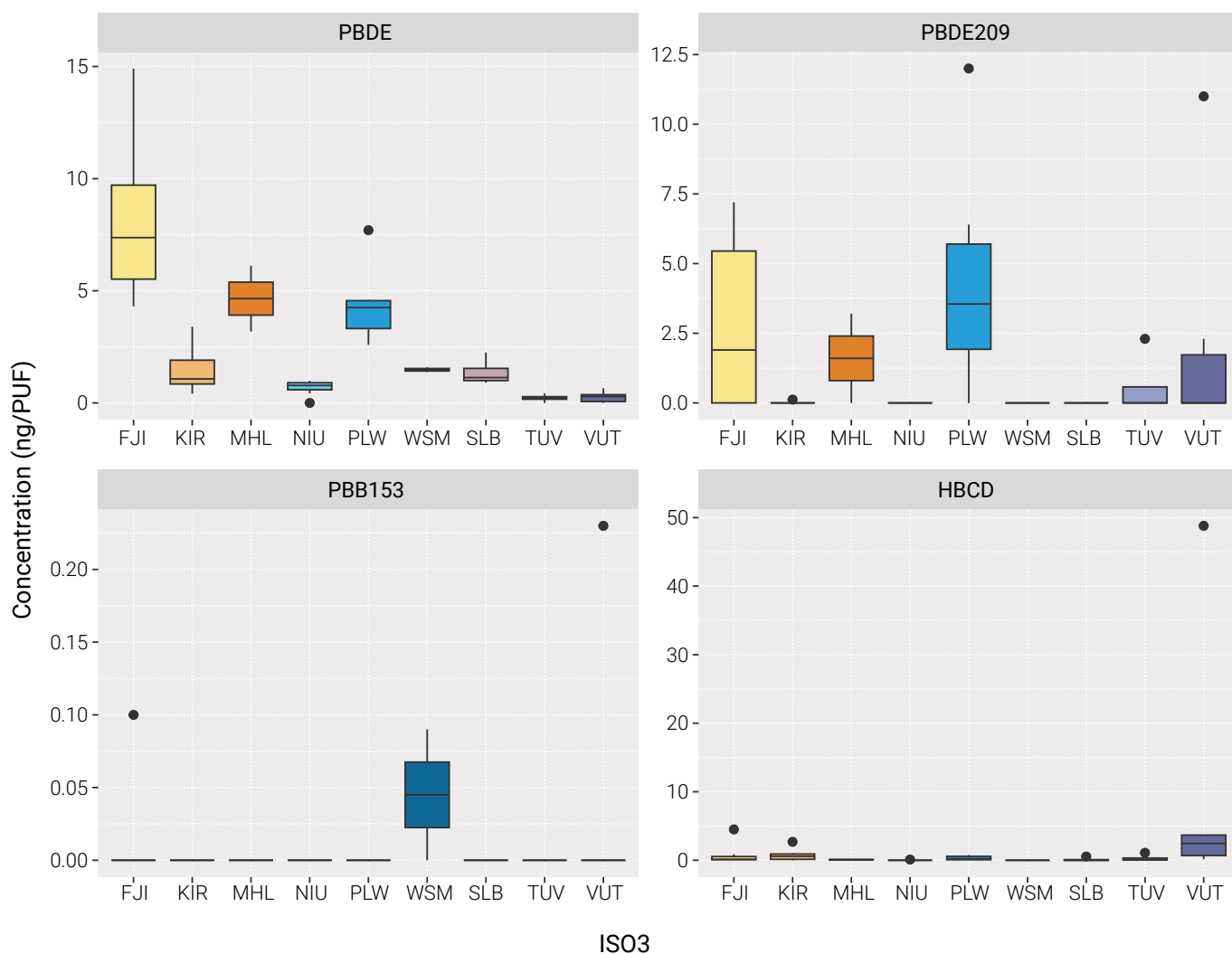
Figure 20: PAS/PUF: Scaled boxplots for country by brominated POPs (n=49)
