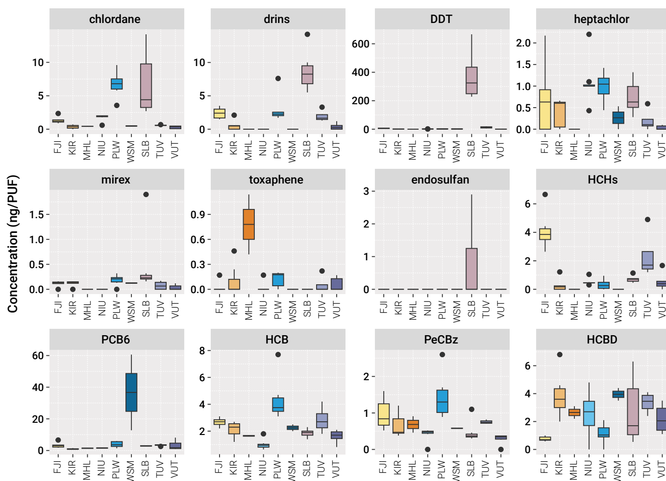
Figure 8: PAS/PUF: Scaled boxplots for country by chlorinated POP (n=49)
