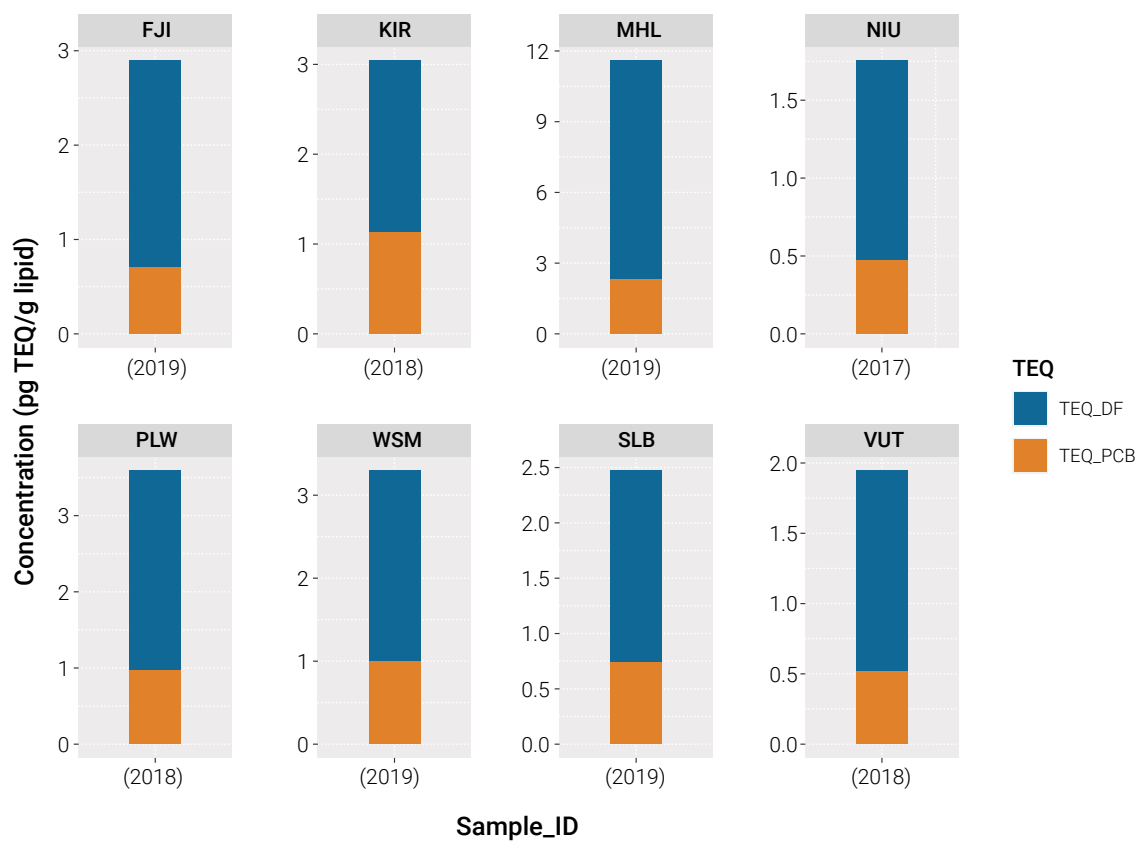
Figure 35: Human milk: Stacked bars for dl-POPs (pg TEQ/g lipid)
