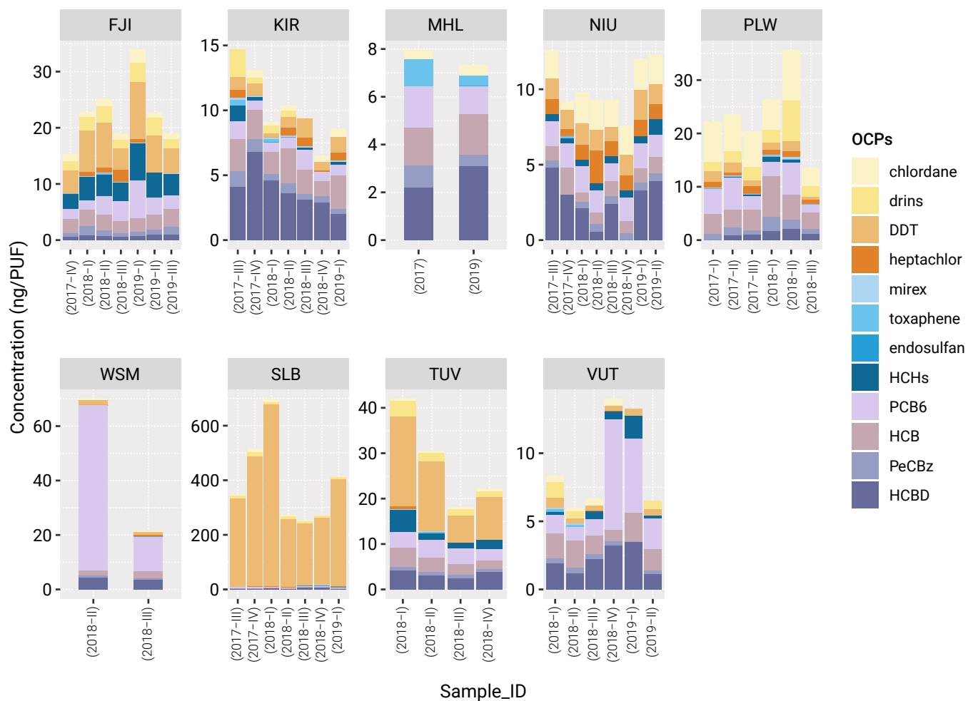
Figure 4: PAS/PUF: Stacked bar graphs for chlorinated POPs by country and sample (n=49)
