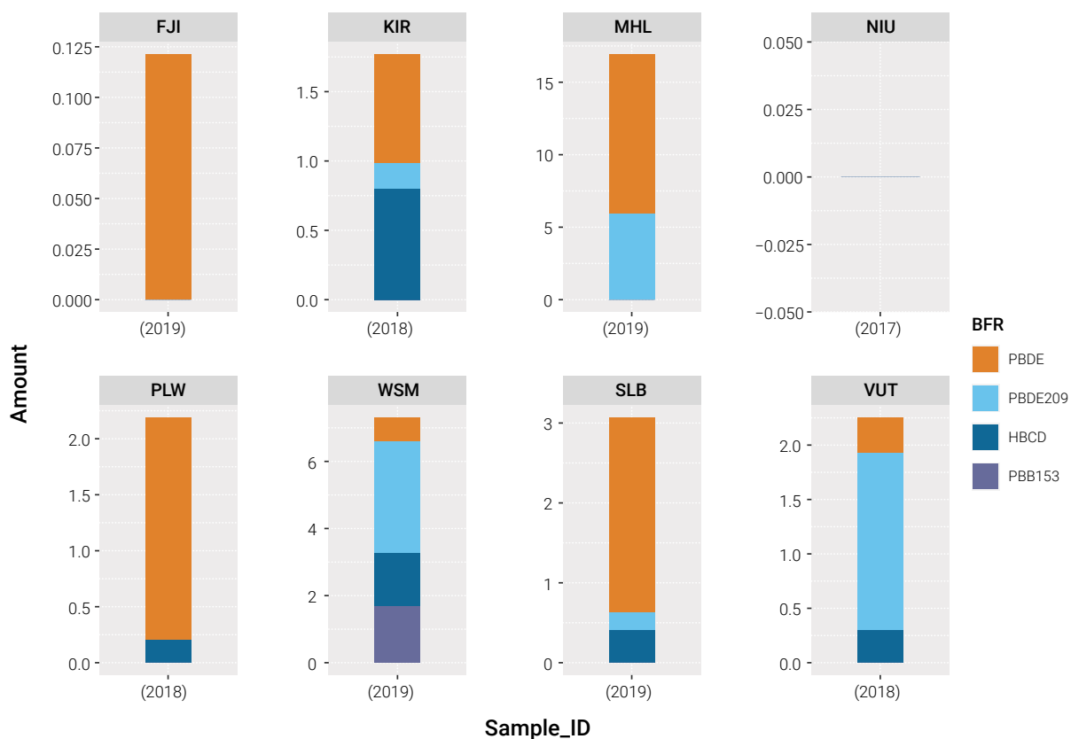
Figure 36: Human milk: Stacked bars for brominated POPs by country (ng/g lipid)
