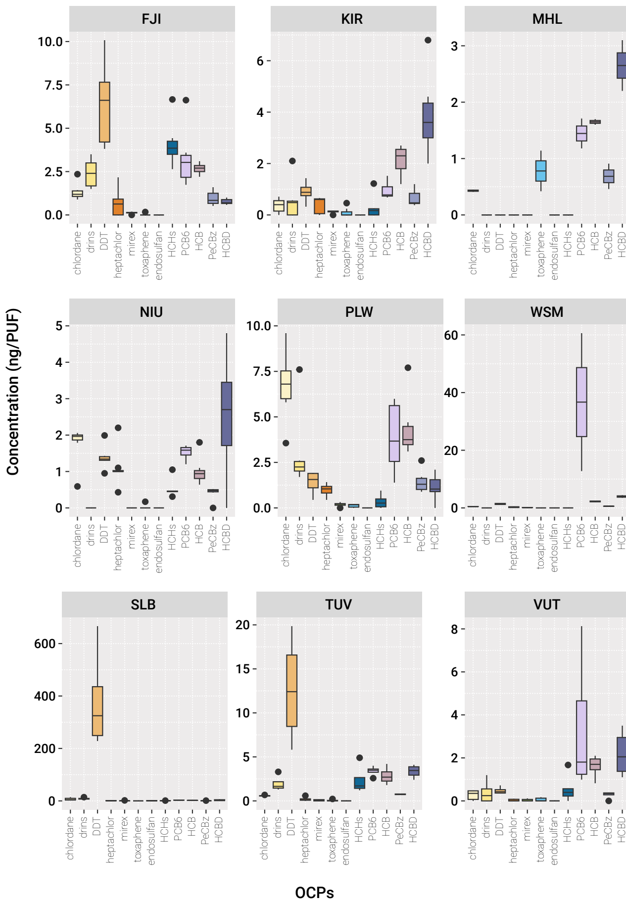
Figure 7: PAS/PUF: Scaled boxplots for sums of chlorinated POPs by country(n=49)
