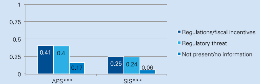
Figure 4. Differences in scheme APS/SIS by policy driver
