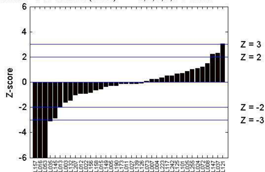
Ranked Overview - Air extract (TOL) 1,2,3,7,8-PnCDF Ranked Z score - Air extract (TOL) 1,2,3,7,8-PnCDF
