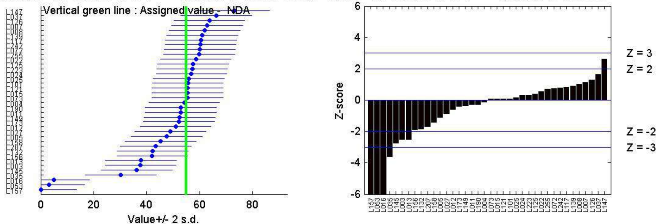
Ranked Overview - Air extract (TOL) 1,2,3,6,7,8-HxCDD Ranked Z score - Air extract (TOL) 1,2,3,6,7,8-HxCDD
