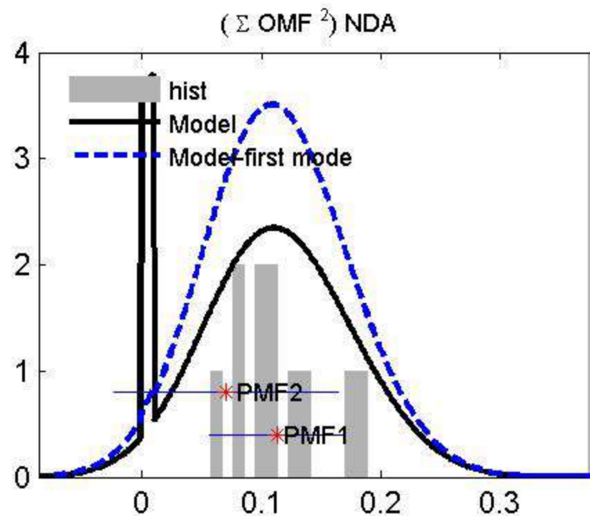
Kilt plot(overlap matrix) Human milk BDE 99
