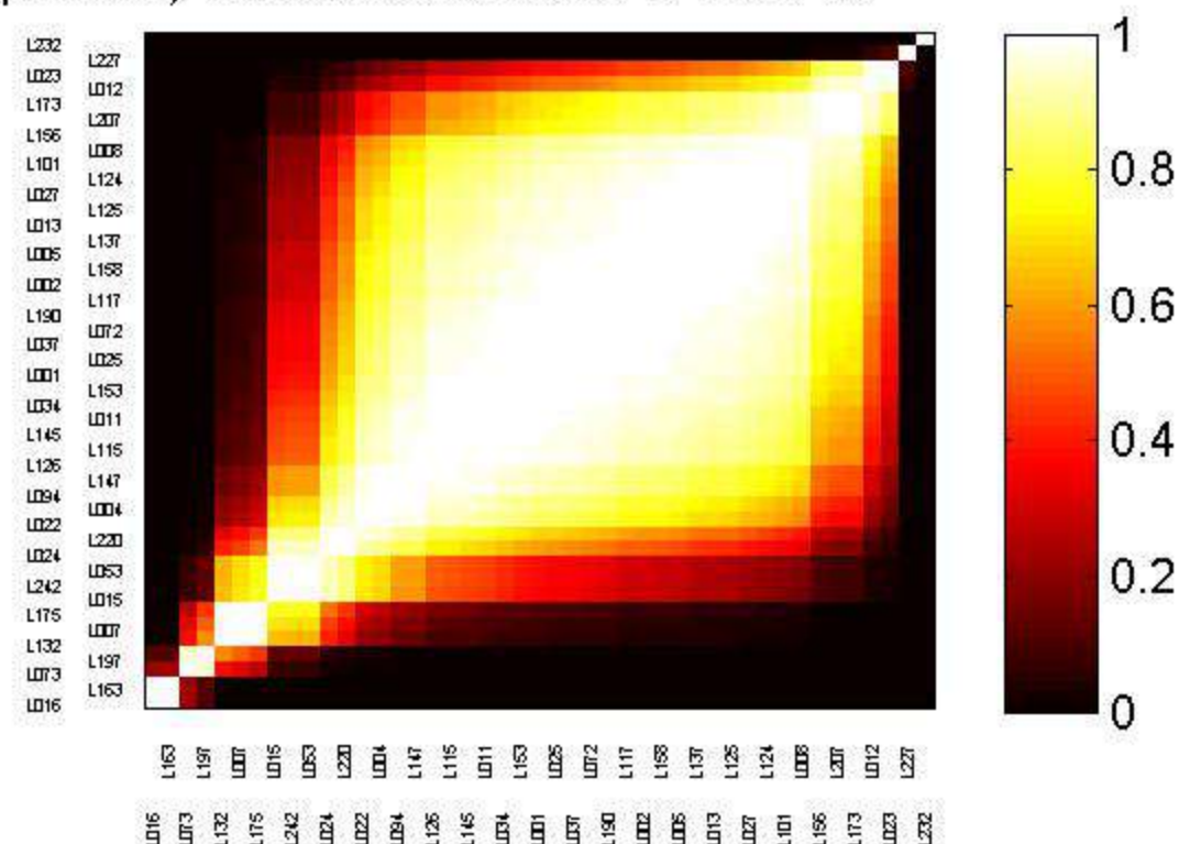
( \Sigma OMF 2 ) NDA Kilt plot(overlap matrix) Test solutions K and L PCB 157
