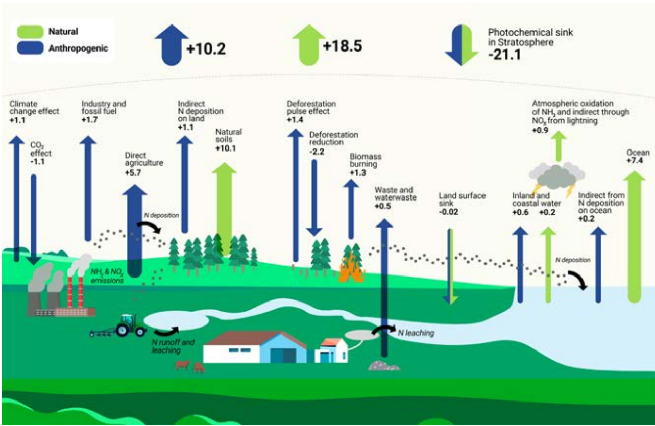
Figure 2.3 Nitrous oxide sources and sinks, megatonnes of nitrous oxide per year. Values shown are the mean for 2010–2019. Source: Adapted from Tian et al. 2024.
