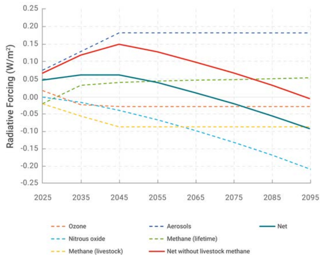
Figure 4.1 Estimated radiative forcing as a function of time by component (dashed) and for the net (solid) under the technical reductions and societal change scenario relative to the reference scenario, 2025–2095, watts per square metre
