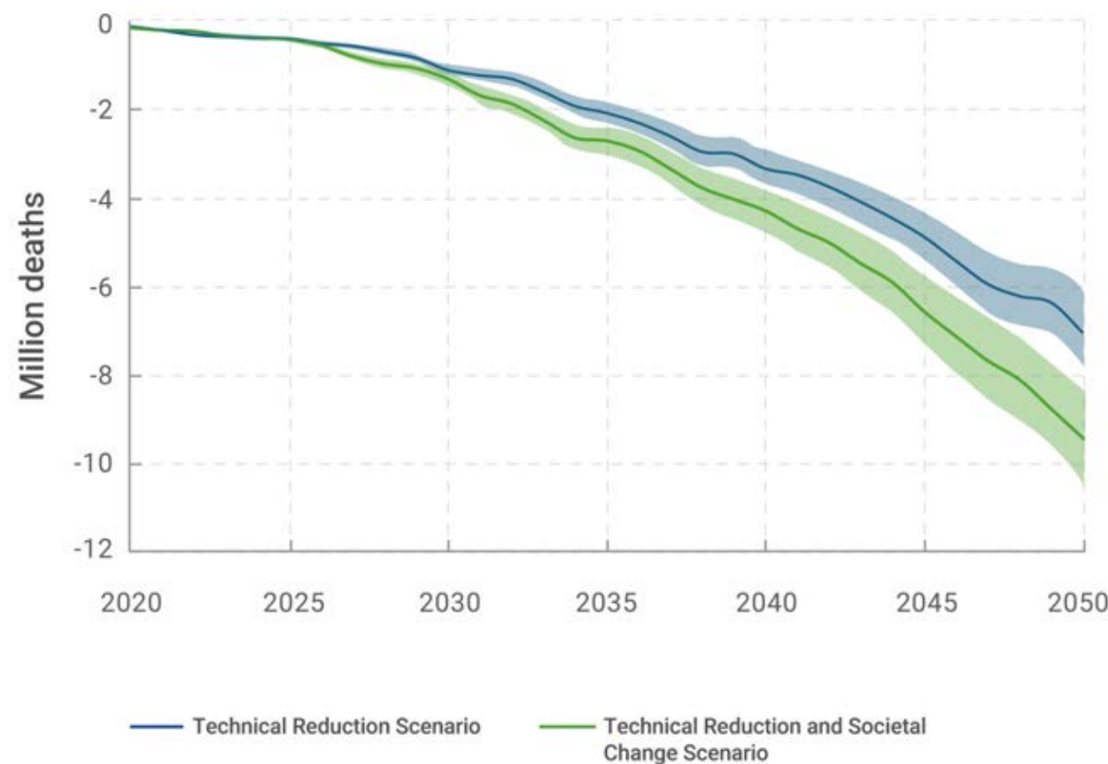
Figure 4.5 Cumulative avoided fine particulate matter-attributable premature deaths under the indicated scenarios relative to the reference scenario based on the GISS model, 2020–2050, million deaths. Note: Uncertainties are based on uncertainties in the exposure-response function.
