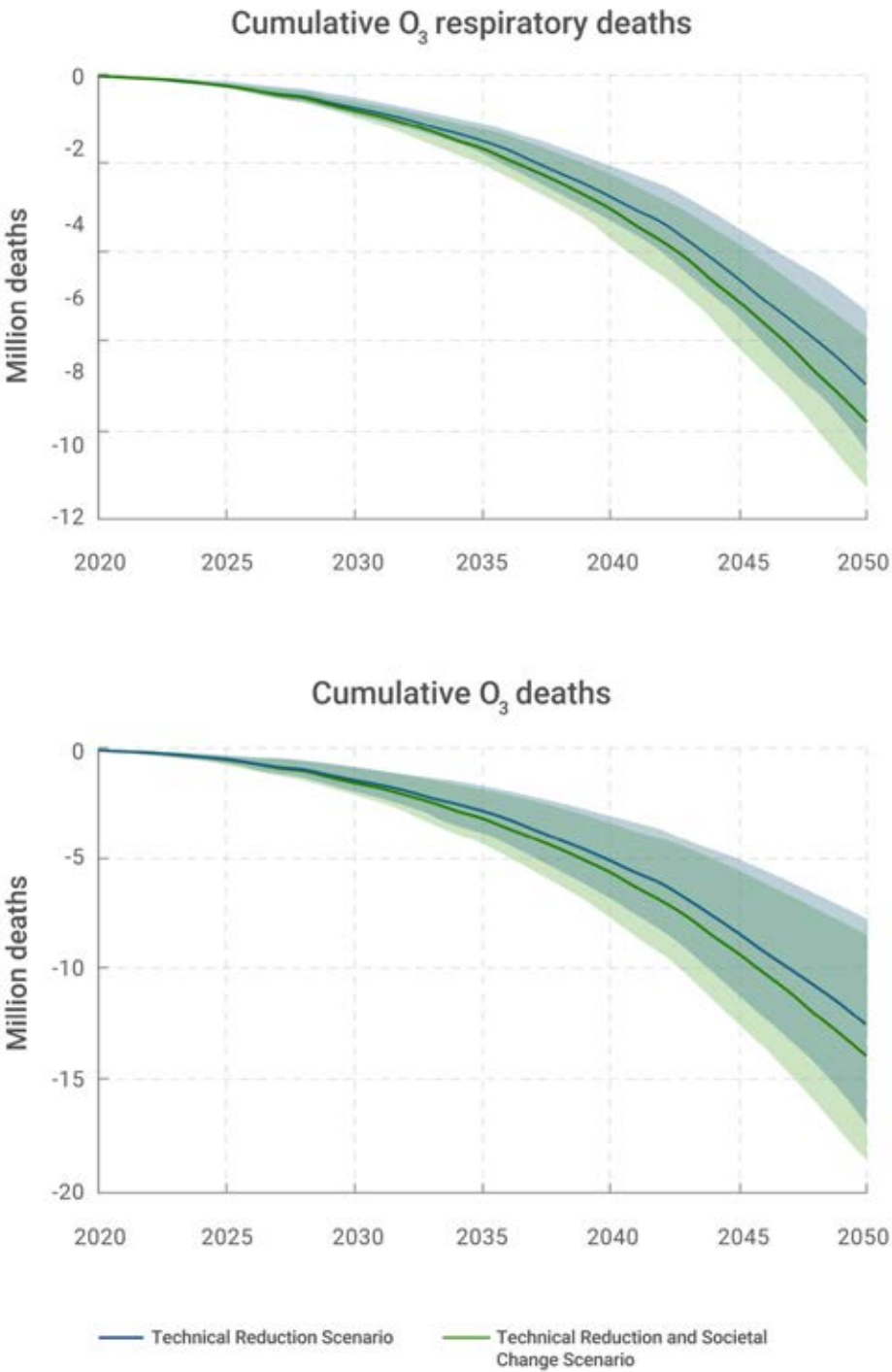
Figure 4.7 Cumulative avoided ozone-attributable premature deaths under the indicated scenarios relative to the reference scenario for (top) respiratory diseases only and (bottom) including the less certain impacts on cardiovascular diseases and diabetes along with respiratory diseases. Note: Uncertainties are based on uncertainties in the exposure-response function.
