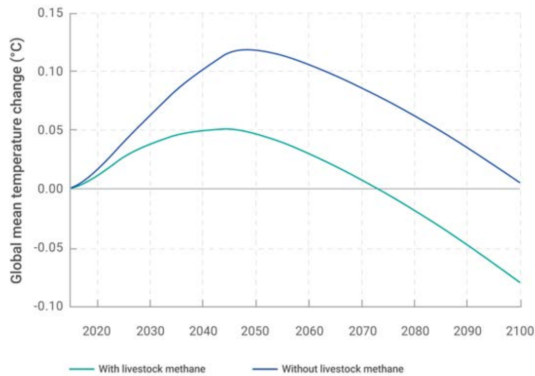
Figure 4.3 Global mean temperature response to the technical reductions and societal change scenario relative to the reference scenario, 2015–2100, degrees Celsius
