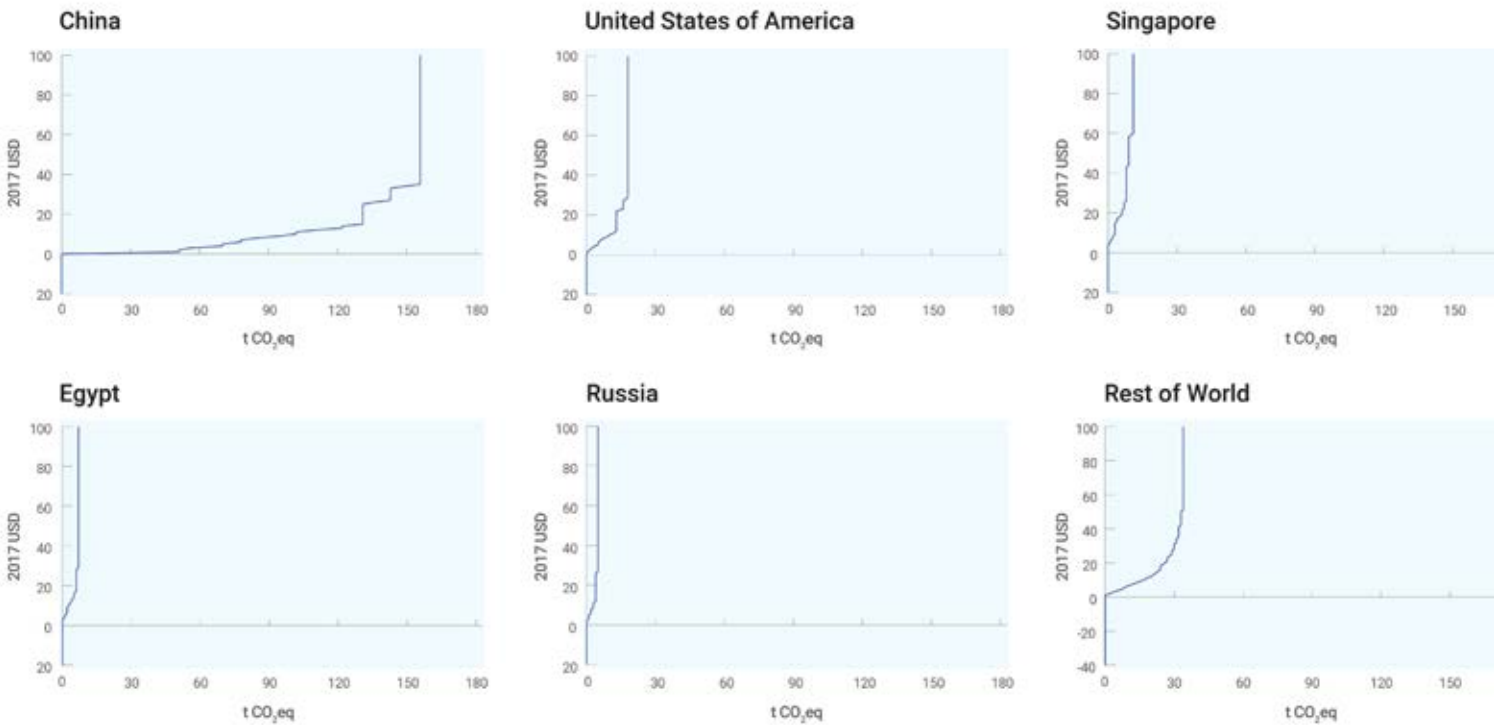
Figure 5.1 Marginal abatement cost curves for projected 2030 nitrous oxide emissions from adipic and nitric acid facilities for the top emitters and the rest of the world Note: The horizontal axis shows the potential for emission abatement in metric tonnes of carbon dioxide equivalent, using 298 as the global warming potential for nitrous oxide relative to carbon dioxide instead of the 273 used in this Assessment. These potentials reflect each country’s current emissions, for example, large in China and small in Russia. The vertical axis shows costs in 2017 dollars for each increment of additional abatement. Source: US EPA 2019
