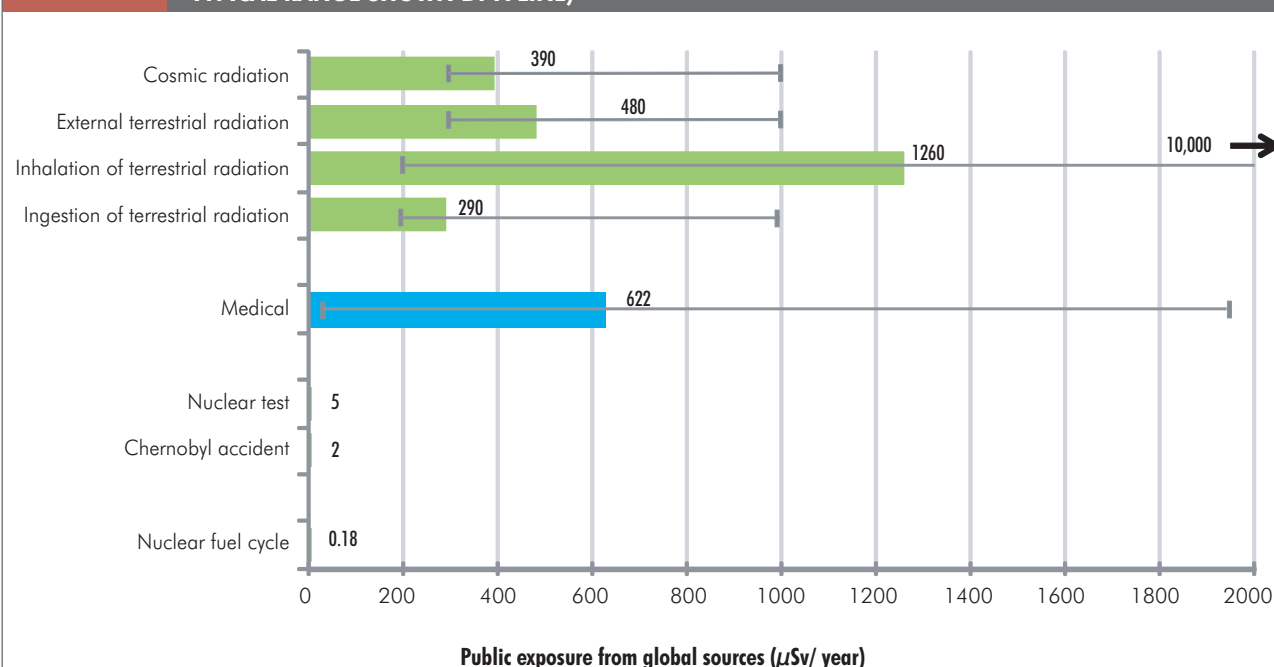
FIGURE 5 PUBLIC EXPOSURE TO RADIATION FROM GLOBAL SOURCES (AVERAGE SHOWN BY A BAR, AND TYPICAL RANGE SHOWN BY A LINE)
