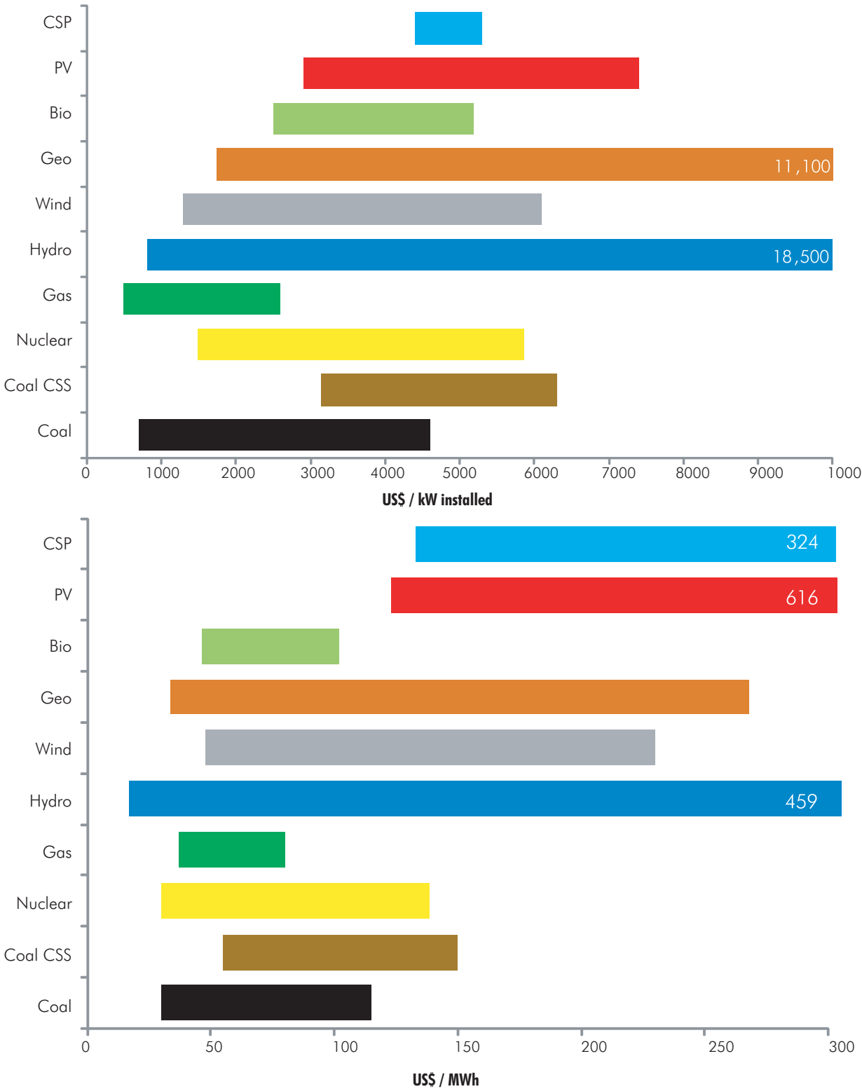
FIGURE 3 INVESTMENT COST RANGES PER KW INSTALLED (UPPER PANEL) AND LEVELIZED COSTS OF ELECTRICITY GENERATION (LCOE) IN US$/MWH OF DIFFERENT GENERATING OPTIONS FOR DISCOUNT RATES BETWEEN 5% AND 10% (LOWER)
