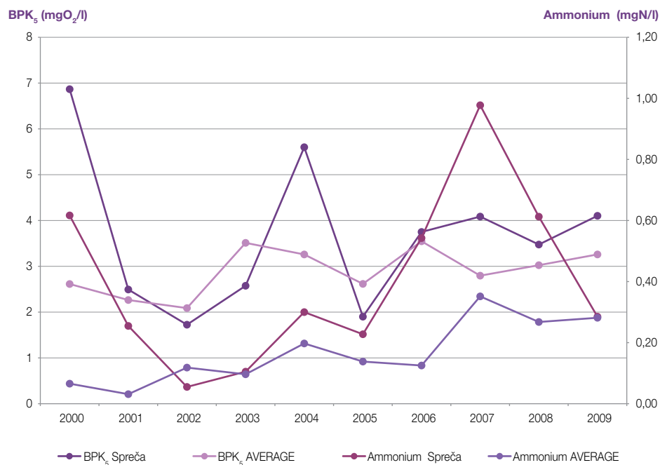
Figure 82: Ammonium and \text{BOD}_5 at the mouth of the Spreča River flowing into the Bosna River, as well as average ammonium values and \text{BOD}_5 in the rivers of BiH (Source: Results of monitoring of surface waters carried out by Water Agencies in BiH)
