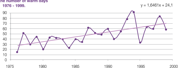
Trends in the number of warm days 1976 - 1999.
