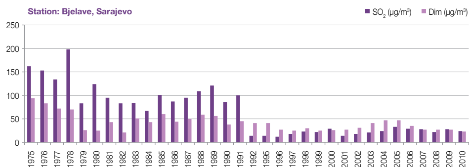
Figure 105: Average annual concentrations of \text{SO}_2 and smoke in Sarajevo in the period 1975-2010 (Source: FHMI BiH, 2011)
