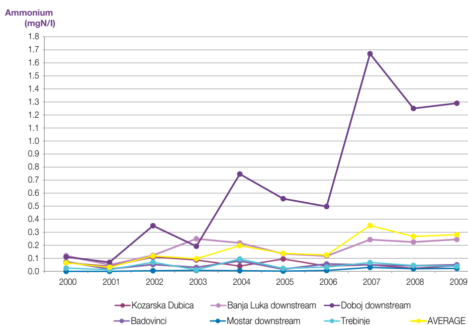
Figure 81: Average values of ammonium ( \text{mg NH}_4^+-\text{N/l} ) in the rivers of BiH – separately (Source: Results of monitoring of surface waters carried out by Water Agencies in BiH)
