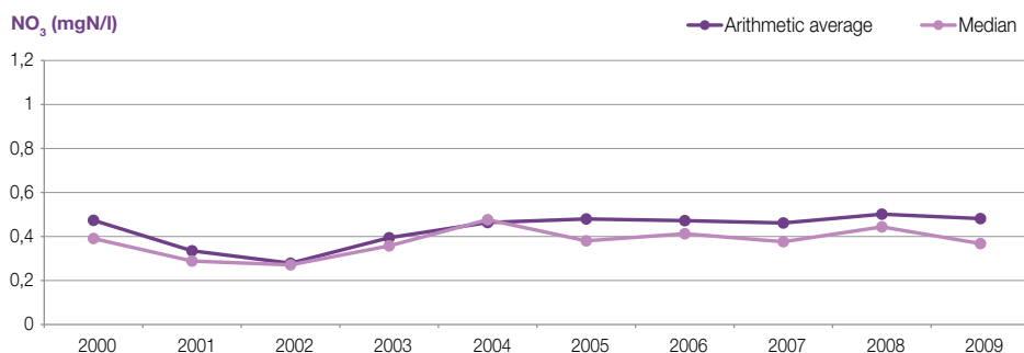
Figure 83: Value of nitrates ( \text{mgNO}_3\text{--N/l} ) in the rivers of BiH (Source: Results of monitoring of surface waters carried out by Water Agencies in BiH)
