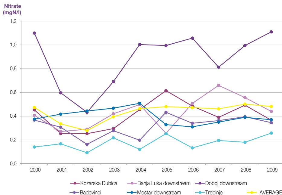
Figure 84: Average values of nitrates ( \text{mgNO}_3\text{--N/l} ) in the rivers of BiH – separately (Source: Results of monitoring of surface waters carried out by Water Agencies in BiH)
