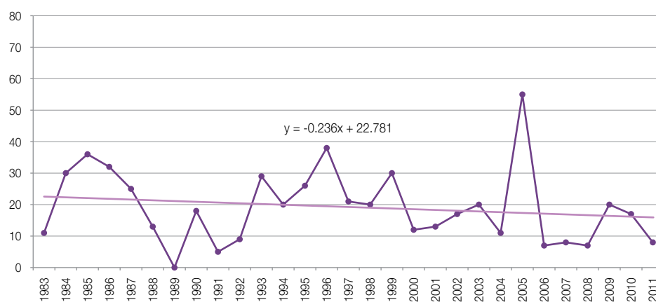
Figure 128: Annual number of days with snow cover of 10 cm and more in Banja Luka in the period 1983-2011 (Source: RHMS RS)
