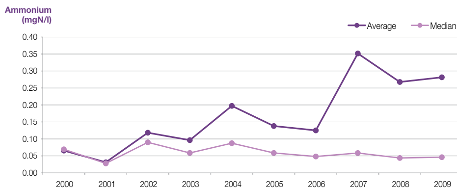
Figure 80: Values of ammonium ( \text{mg NH}_4^+-\text{N/l} ) in the rivers of BiH (Source: Results of monitoring of surface waters carried out by Water Agencies in BiH)
