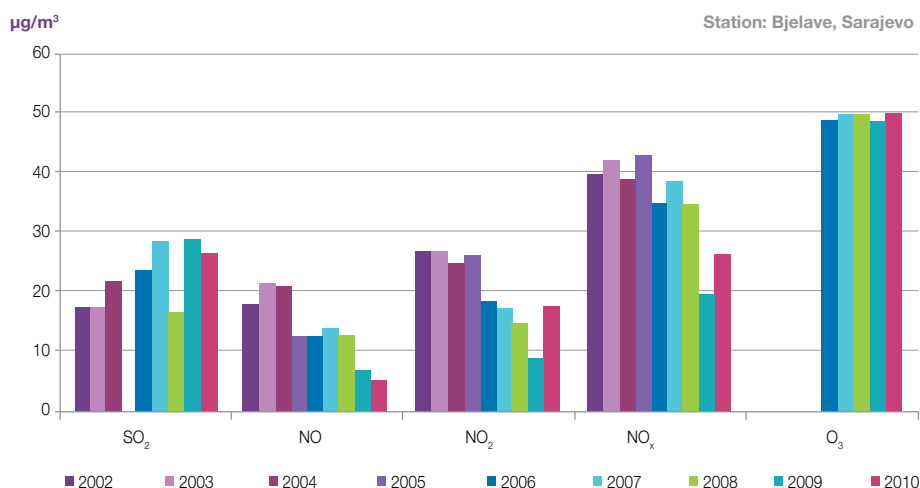
Figure 106: Average annual concentrations of \text{SO}_2 , NO, \text{NO}_2 , \text{NO}_x , \text{O}_3 in Sarajevo (1-hour values) in the period 2002-2010 (Source: FHMI BiH, 2010)
