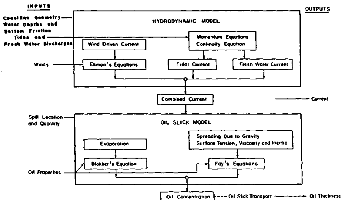
Fig. 5. General formulation of the mathematical model of an oil slick
