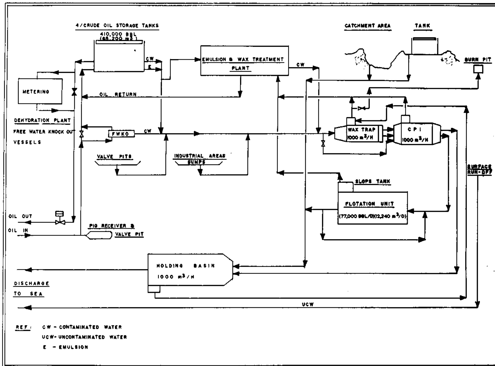
Fig. 9. A typical wastewater treatment system of a crude oil terminal in Malaysia.
