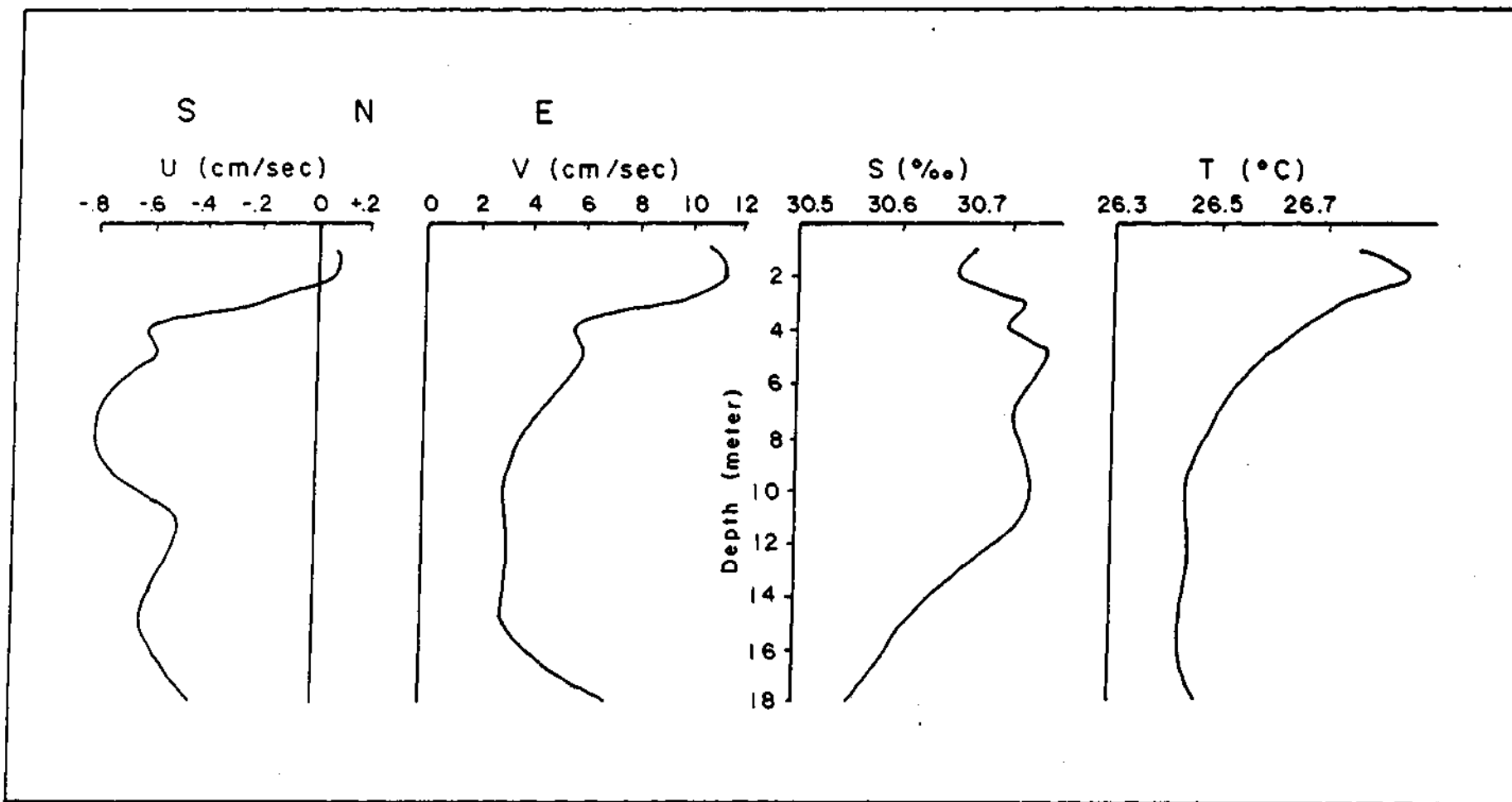
Fig. 3. The variations of some physical properties of sea water offshore of Ban Laem averaged per tidal cycle in a vertical direction.
