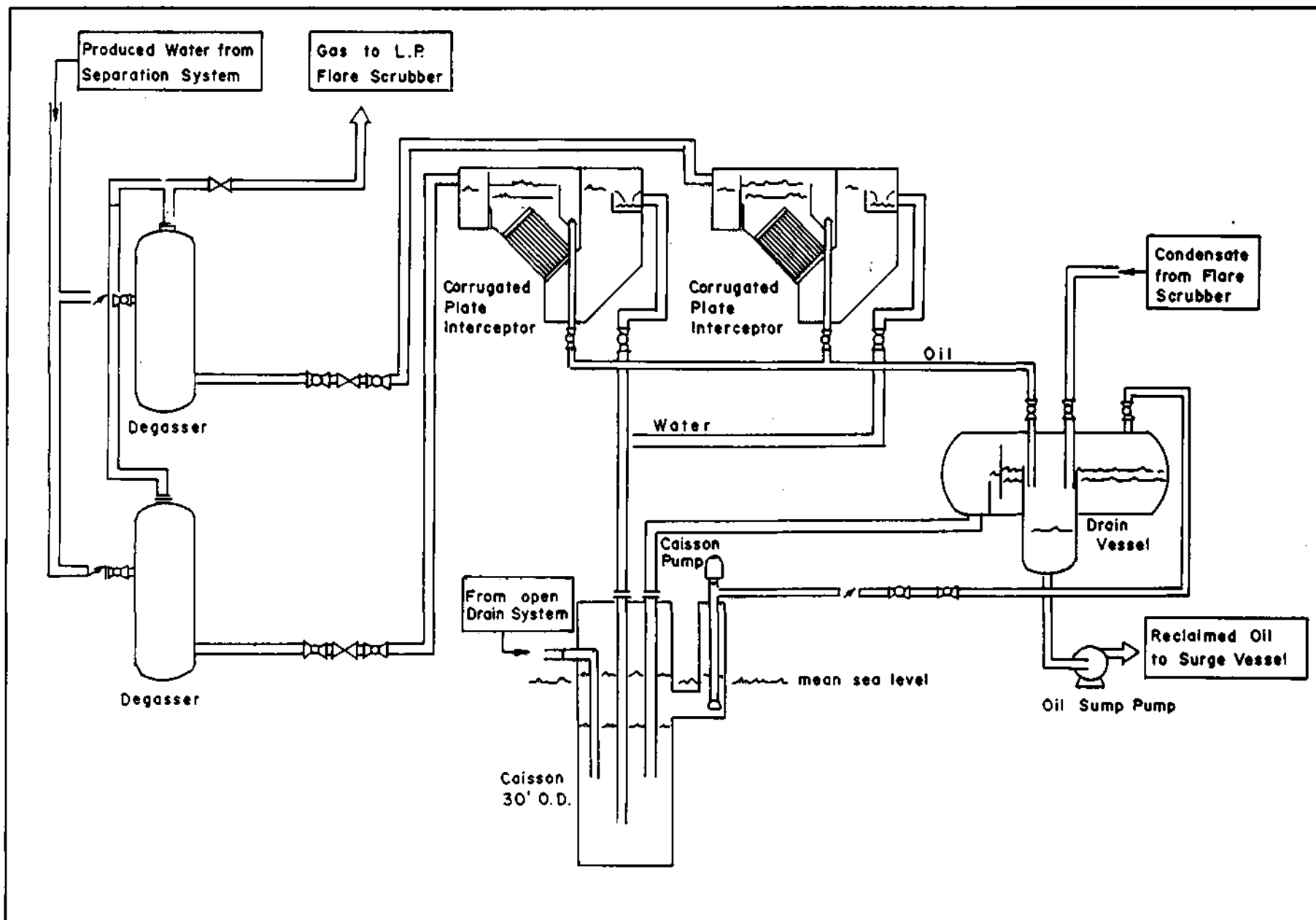
Fig. 8. A typical wastewater treatment system of an offshore production platform in Malaysia.
