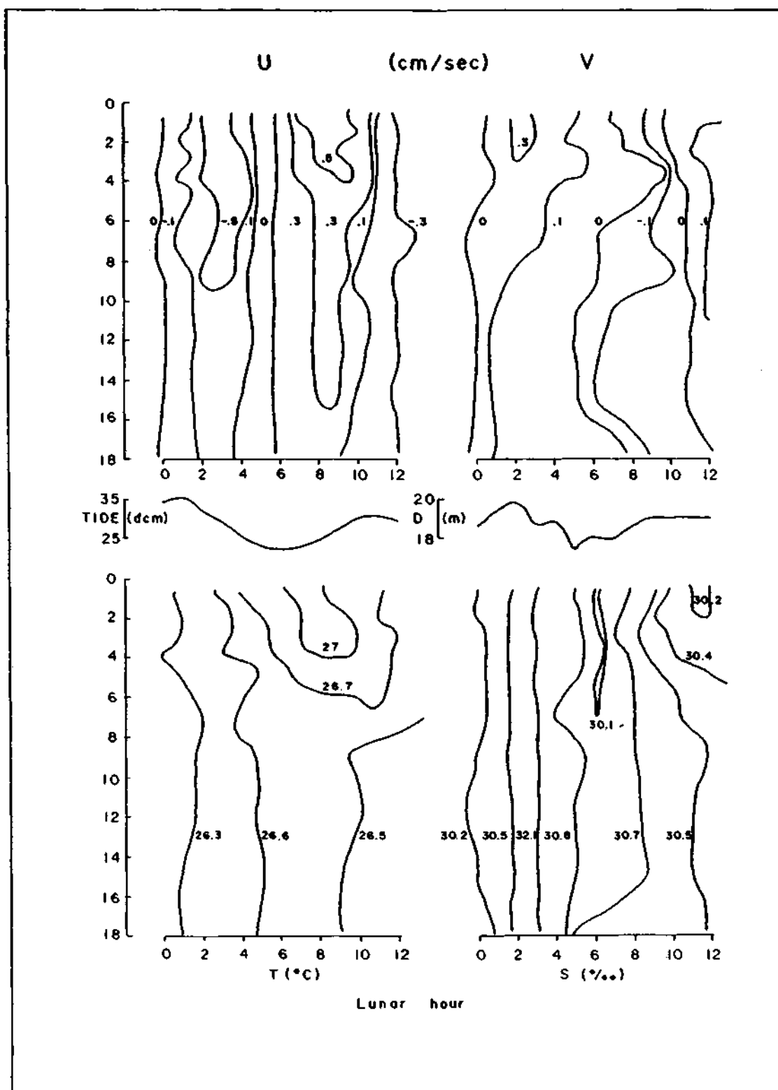
Fig. 2. The variations of some physical properties of seawater offshore of Ban Laem from lunar hour 0 to 12 at various depths (from Siripong and Tamiyavanich 1984).
