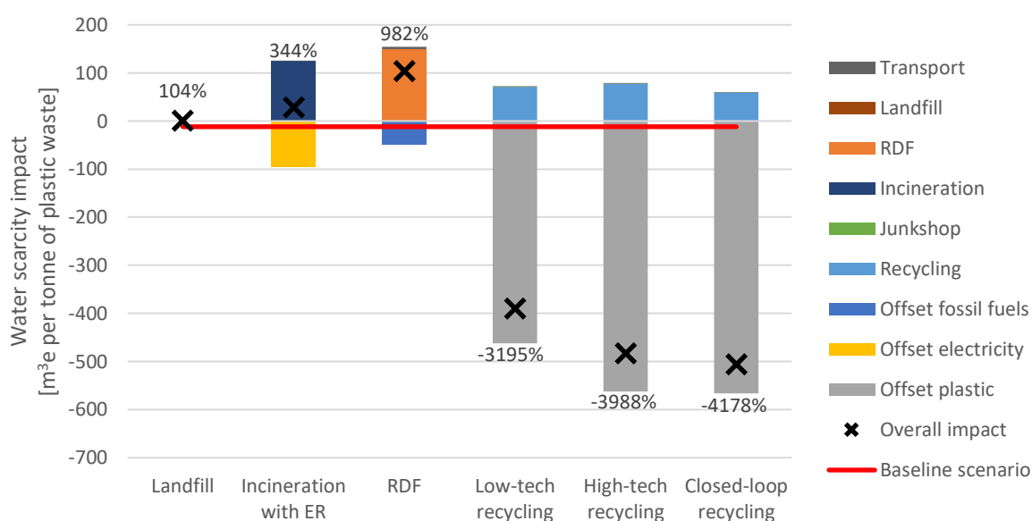
Figure 8: Water scarcity impacts, broken down by life cycle stage, for plastic waste management options in Pakistan. Crosses represent the net impacts each option, with percentages reflecting the difference in impact relative to the Pakistan baseline scenario for each option.
