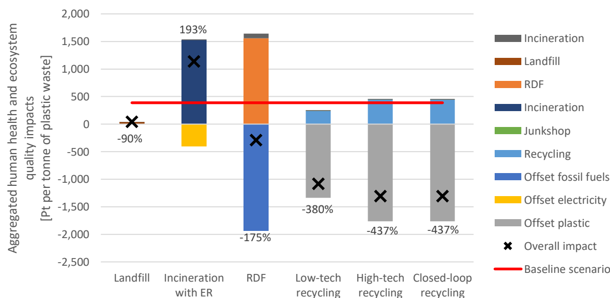
Figure 14: Aggregated life cycle human health and ecosystem quality impacts, broken down by life cycle stage, for plastic waste management options in Pakistan. Scenario investigating the “worst case” scenario for polymers (PET recycling, offsetting HDPE virgin polymer).
