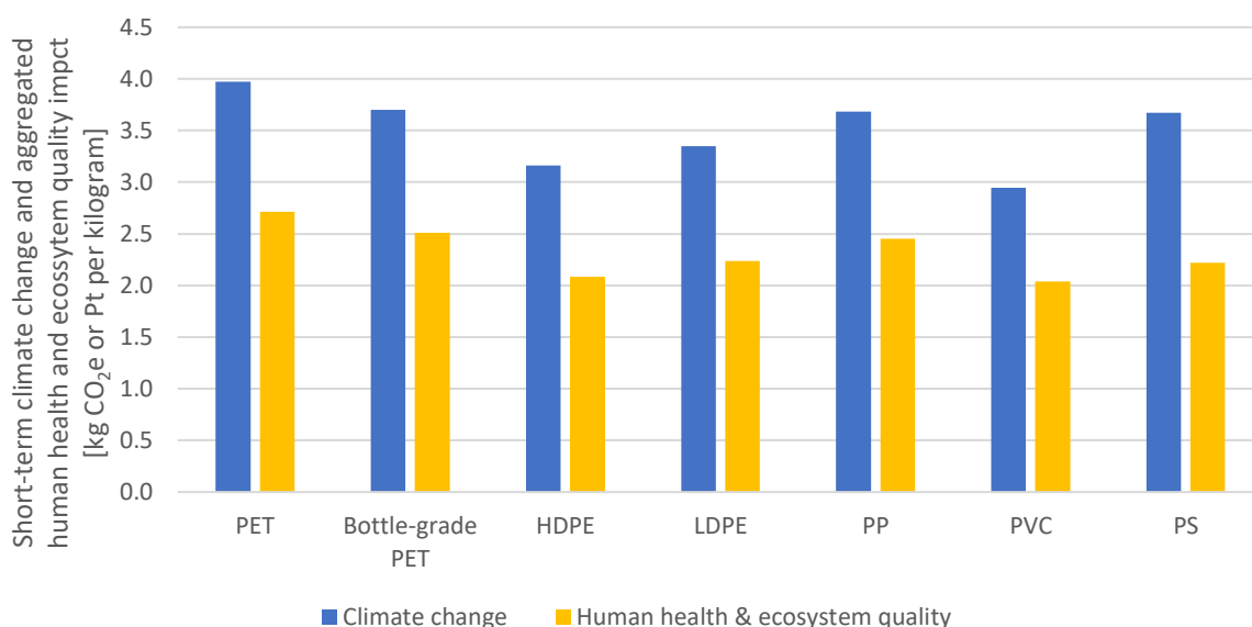
Figure 12: Short-term climate change and aggregated human health & ecosystem quality impacts of various virgin plastic polymers 31
