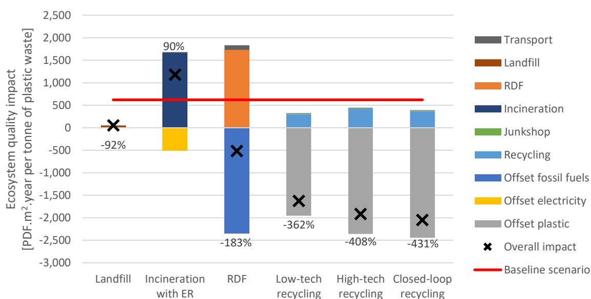
Figure 10: Ecosystem quality impacts, broken down by life cycle stage, for plastic waste management options in Pakistan. Crosses represent the net impacts each option, with percentages reflecting the difference in impact relative to the Pakistan baseline scenario for each option.
