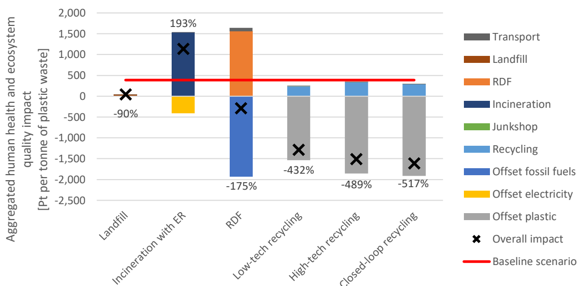
Figure 5: Aggregated life cycle human health and ecosystem quality impacts, broken down by life cycle stage, for plastic waste management options in Pakistan. Crosses represent the net aggregated result of each option, with percentages reflecting the difference in impact relative to the Pakistan baseline scenario for each option.
