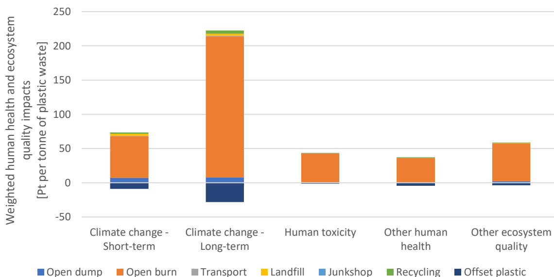
Figure 4: Aggregated life cycle human health and ecosystem quality impacts of current Pakistani plastic waste management, broken down by life cycle stage, disposal type and damage category 20
