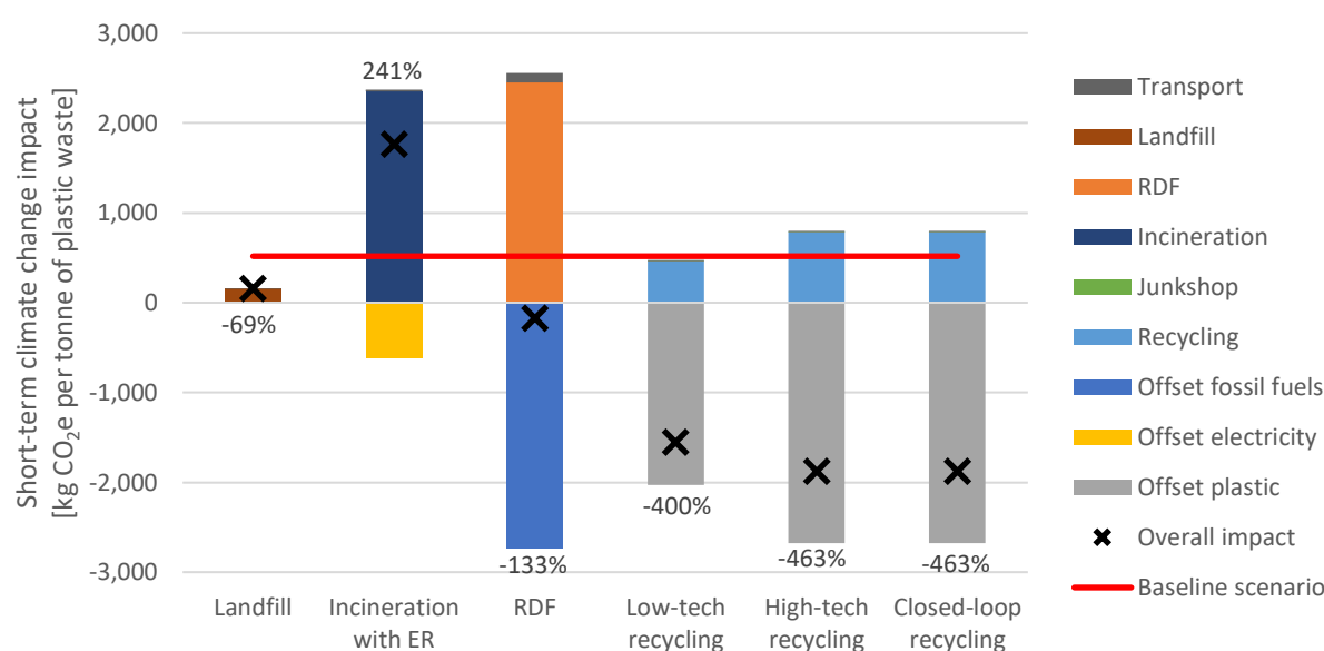
Figure 13: Short-term climate change impacts, broken down by life cycle stage, for plastic waste management options in Pakistan. Scenario investigating the “worst case” scenario for polymers (PET recycling, offsetting HDPE virgin polymer).
