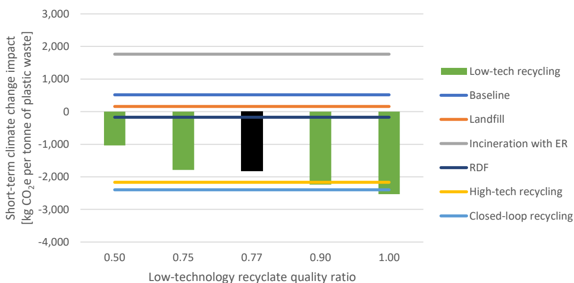
Figure 19: Short-term climate change impacts for scenario investigating varying the quality ratio of recycle from low-technology mechanical recycling. Black column is default low-technology mechanical recycling scenario (quality ratio of 0.77).
