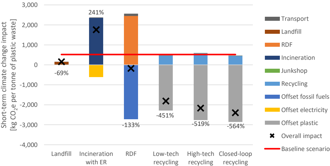
Figure 6: Short-term climate change impacts, broken down by life cycle stage, for plastic waste management options in Pakistan. Crosses represent the net impacts each option, with percentages reflecting the difference in impact relative to the Pakistan baseline scenario for each option.
