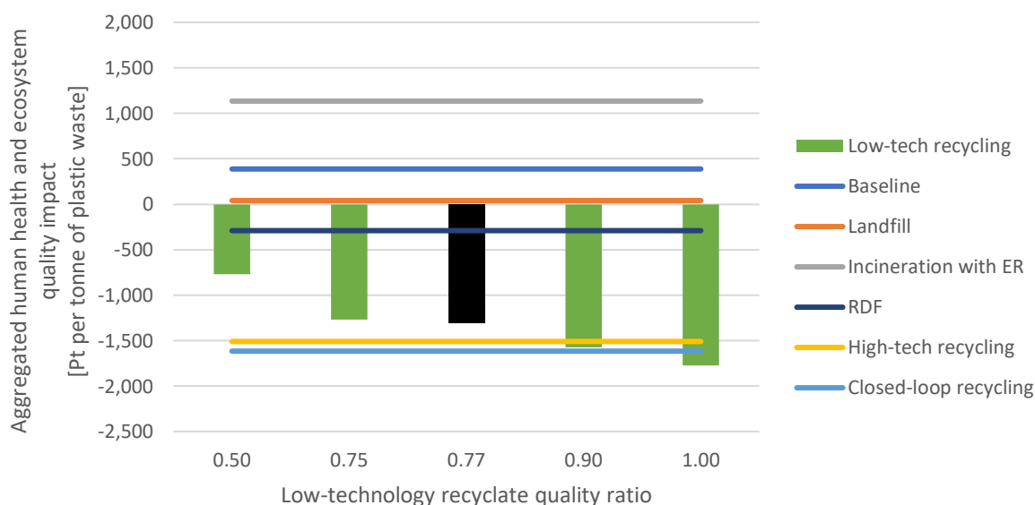
Figure 20: Aggregated human health and ecosystem quality impacts for scenario investigating varying the quality ratio of recycle from low-technology mechanical recycling. Black column is default low-technology mechanical recycling scenario (quality ratio of 0.77).
