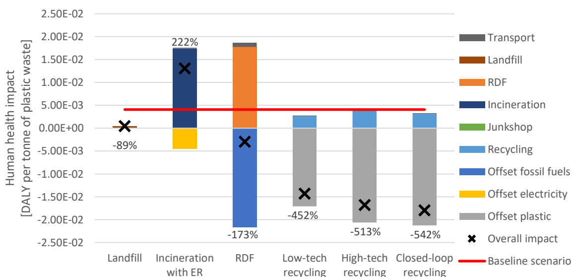
Figure 9: Human health impacts, broken down by life cycle stage, for plastic waste management options in Pakistan. Crosses represent the net impacts each option, with percentages reflecting the difference in impact relative to the Pakistan baseline scenario for each option.
