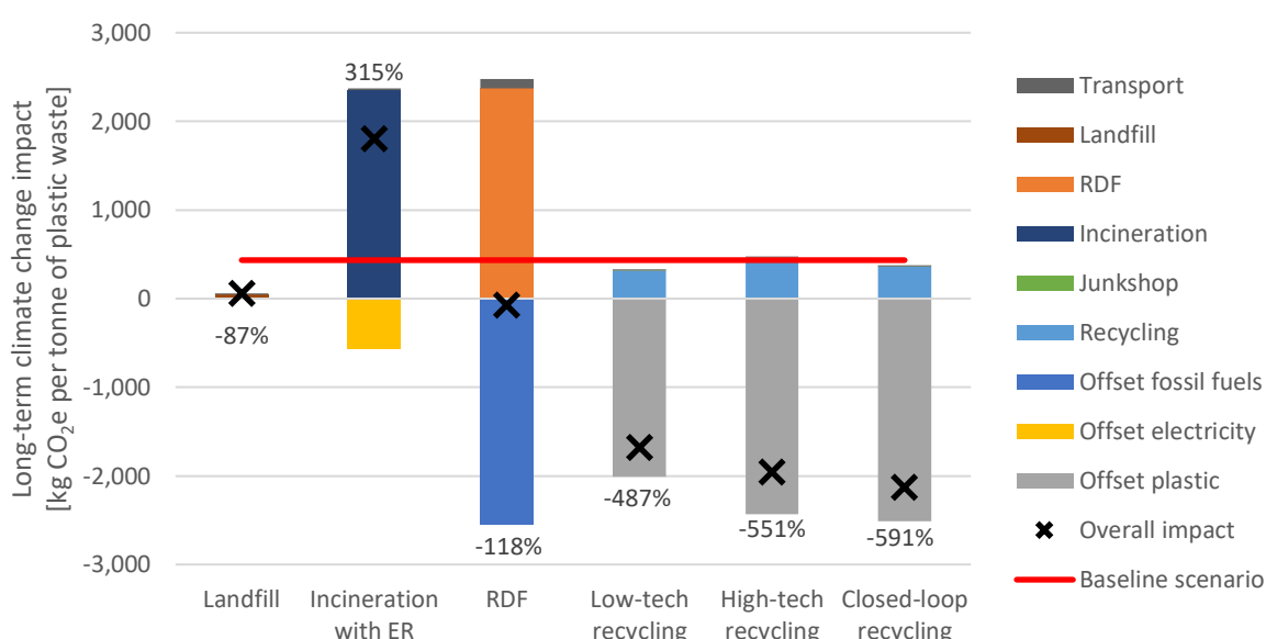
Figure 7: Long-term climate change impacts, broken down by life cycle stage, for plastic waste management options in Pakistan. Crosses represent the net impacts each option, with percentages reflecting the difference in impact relative to the Pakistan baseline scenario for each option.
