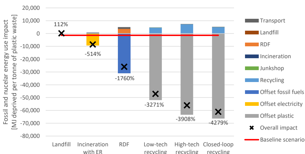
Figure 11: Fossil and nuclear energy use impacts, broken down by life cycle stage, for plastic waste management options in Pakistan. Crosses represent the net impacts each option, with percentages reflecting the difference in impact relative to the Pakistan baseline scenario for each option.
