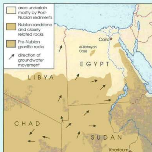
Part of the sub-Saharan fossil aquifer; arrows show the direction of water movement.
