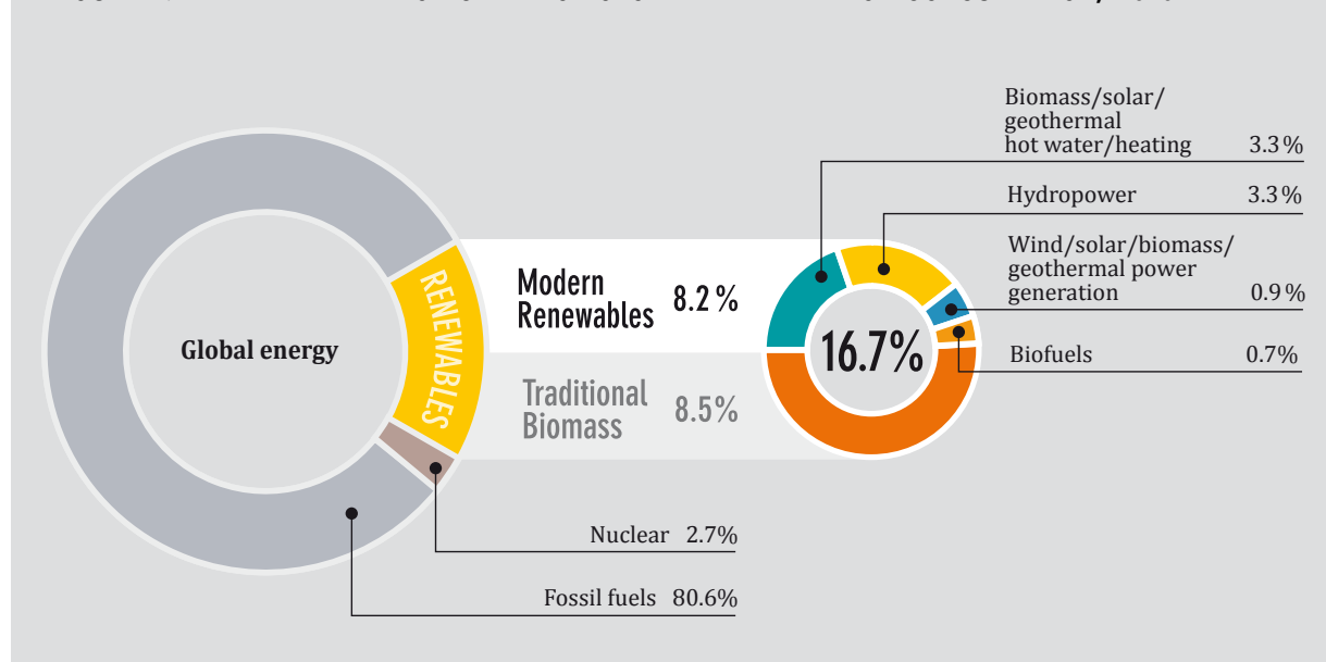
FIGURE 1. RENEWABLE ENERGY SHARE OF GLOBAL FINAL ENERGY CONSUMPTION, 2010
