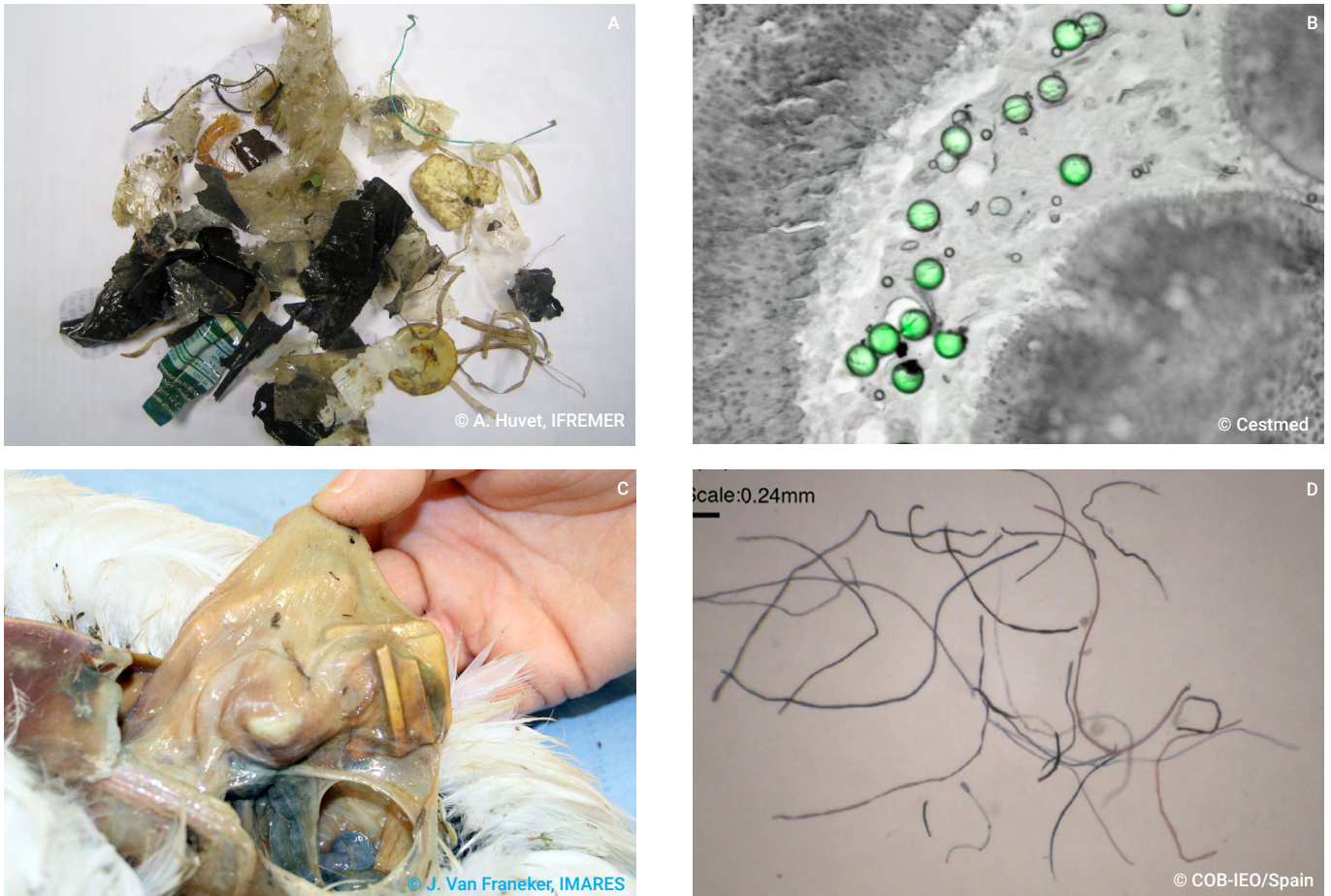
Figure 1: Marine litter ingested by Mediterranean marine organisms.
