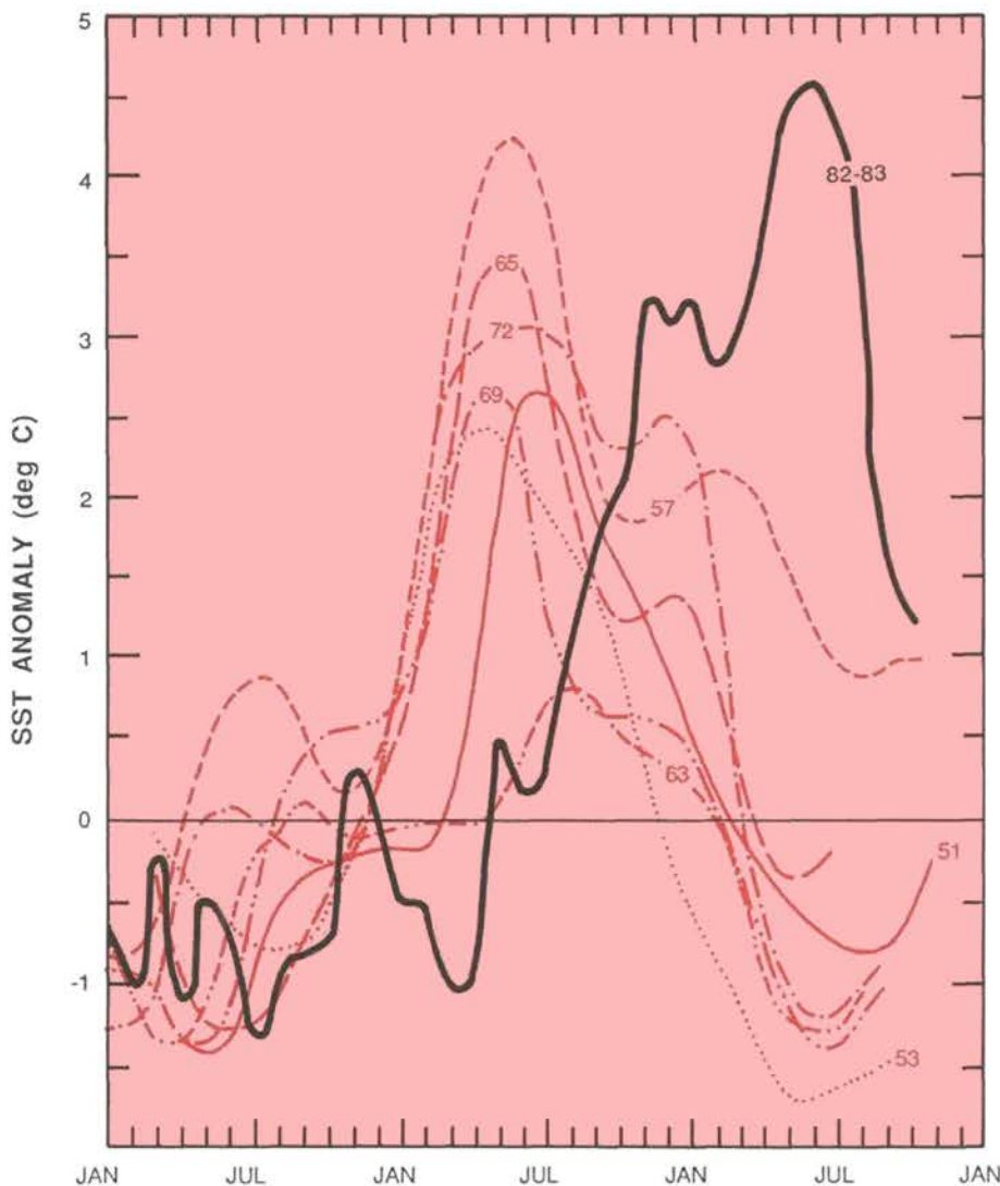
Fig. 1.8 SST anomaly time series for the eight most significant warm episodes between 1950 and 1983. (adapted from Rasmusson and Carpenter, 1982.)
