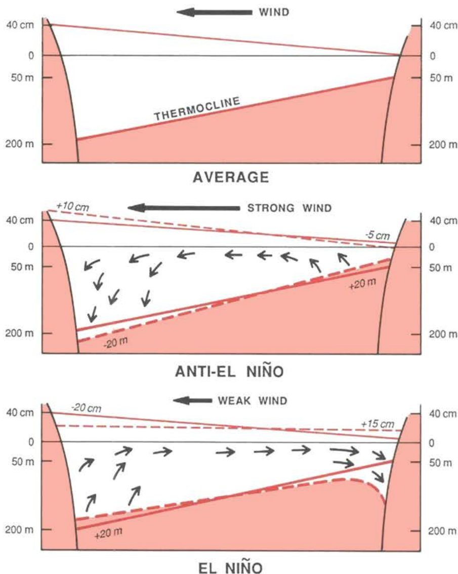
Fig. 1.4 The response of the thermal structure of the equatorial Pacific to changing winds. TOP: Under normal easterly trade wind conditions sea level rises to the west and the thermocline deepens. CENTER: This situation is amplified during strong trade winds. BOTTOM: When the winds relax, water sloshes east, which leads to a rise in sea level and a deepening of the thermocline along South America. In the western Pacific, sea level drops and the thermocline rises. (Adapted from K. Wyrtki, 1982.)
