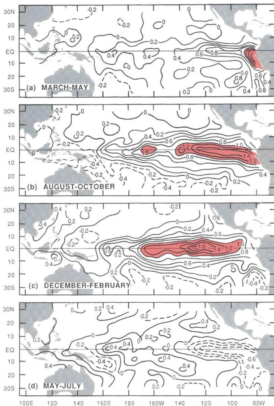
Fig. 1.9 SST anomalies during a typical ENSO event for (a) March, April, and May after onset, (b) the following August, September, and October, (c) the following December, January, and February, and (d) May, June and July, more than a year after the onset. (From Philander, 1983.)
