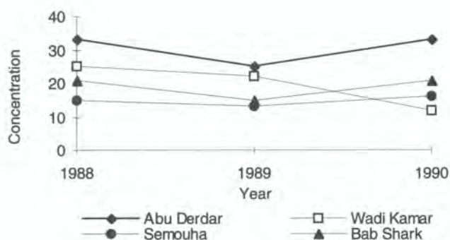
Figure 5.1 Annual mean smoke concentrations in Alexandria ( \mu\text{g m}^{-3} )
