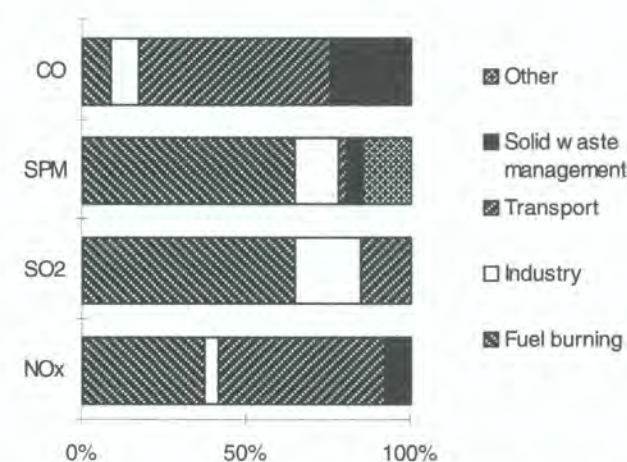
Figure 22.8 Sources of emissions for 1989 in Taipei
