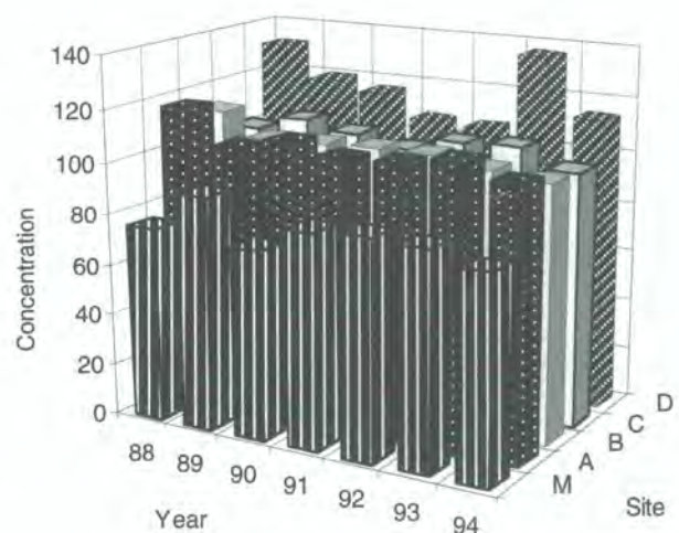
Figure 20.1 \text{PM}_{10} trends at five sites in Santiago, 1988–1994 ( \mu\text{g m}^{-3} )
