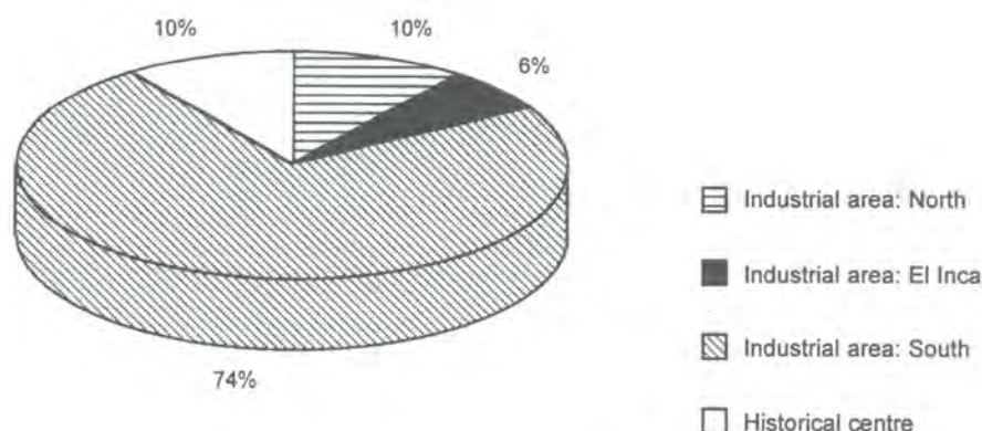
Figure 19.8 Estimated industrial emissions from different areas in Quito (1989)
