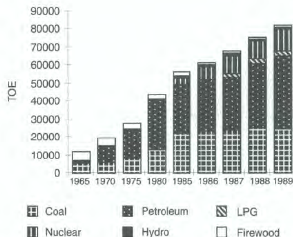
Figure 18.2 Trends in primary energy consumption by fuel type
