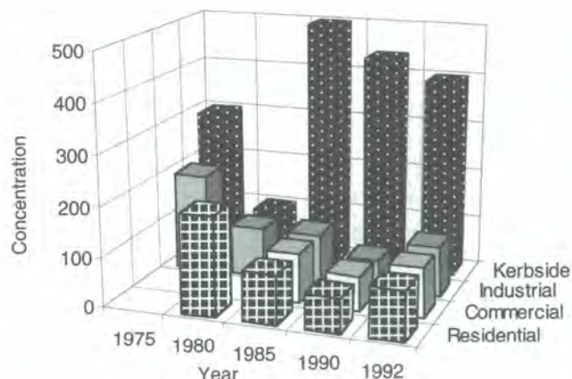
Figure 9.2 St Petersburg annual mean dust concentrations, 1975–1992 (µg m -3 )
