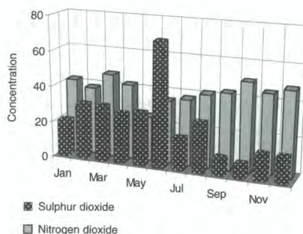
Figure 10.3 \text{SO}_2 and \text{NO}_2 concentrations in 1990 at an industrial site (Kwun Tong) ( \mu\text{g m}^{-3} )
