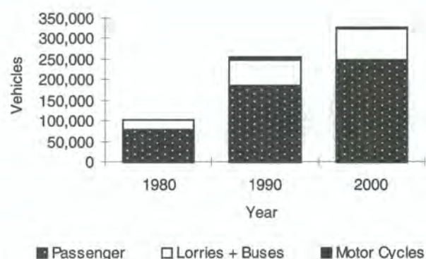
Figure 5.2 Vehicle numbers in 1980, 1990 and 2000 (projected) in Alexandria
