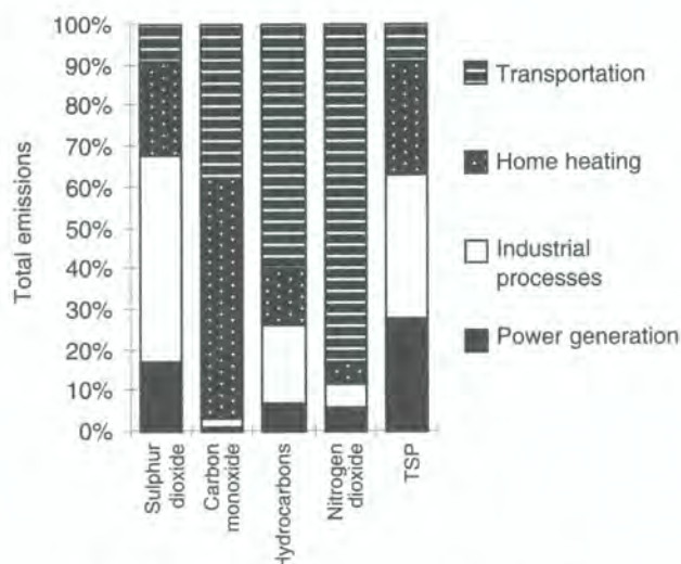
Figure 18.7 Relative emissions source contributions, Korea 1989
