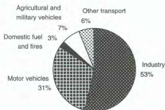
Figure 9.6 Emission sources for the Russian Federation in 1989
