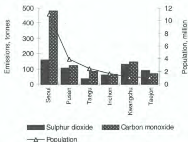
Figure 18.6 Emissions of \text{SO}_2 and CO in Korean cities, 1989
