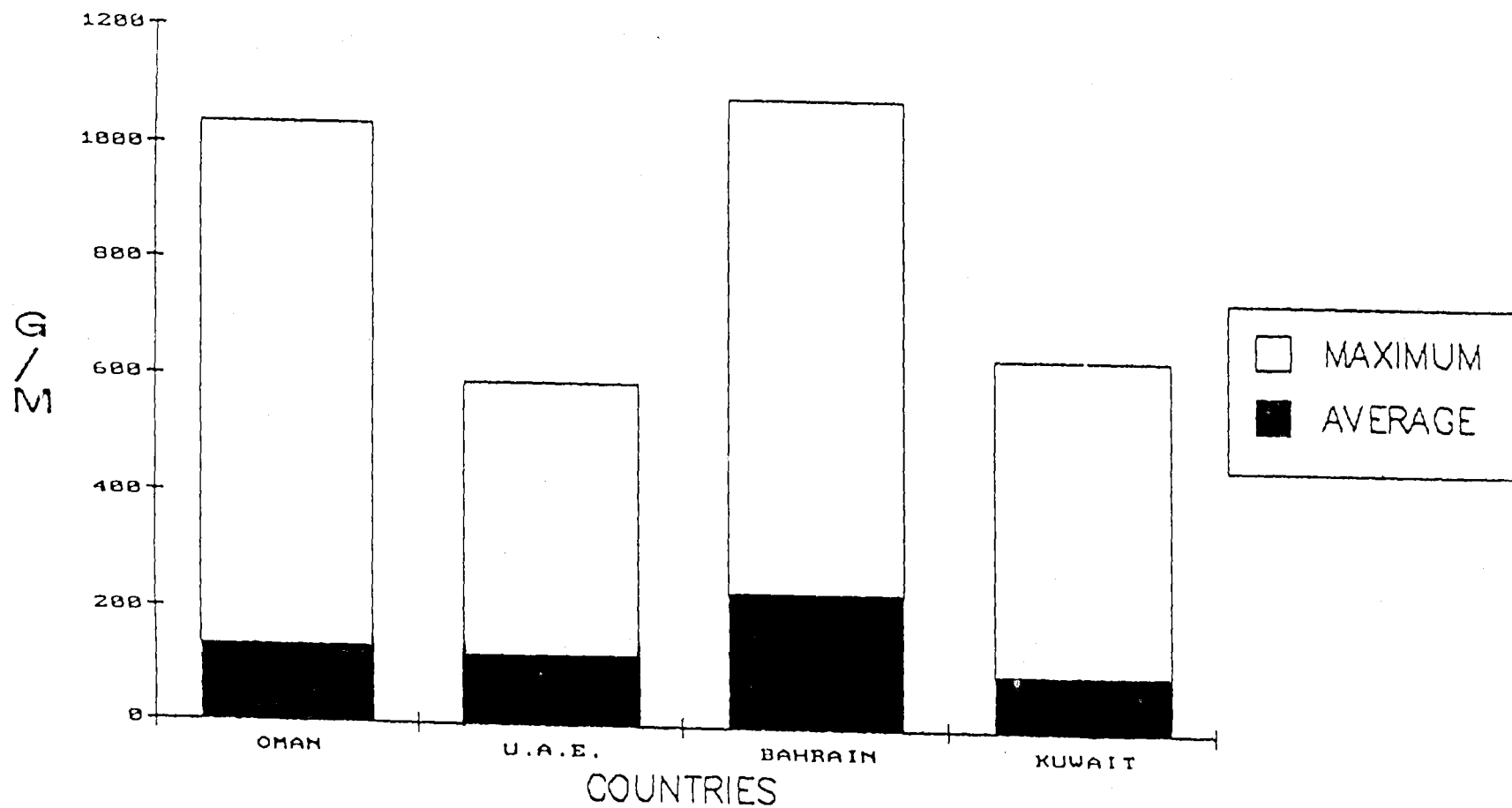
Figure 7. Monthly dust fallout (g/m²) in the North Western part of the region (ROPME, 1987)
