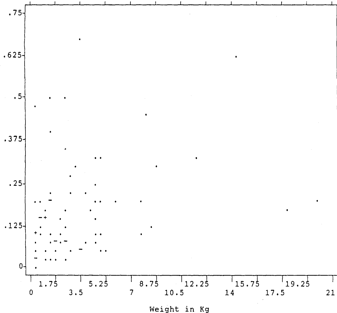
Figure 6. Total mercury in muscle of groupers according to weight (ROPME/IAEA, 1988)
