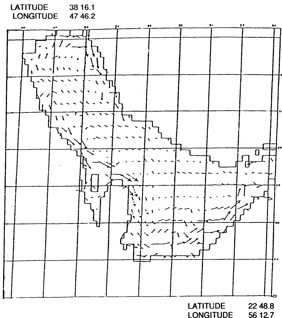
Figure 4. Surface current component due to wind stress using a 5 m/s wind from northwest (Galt et al., 1984)
