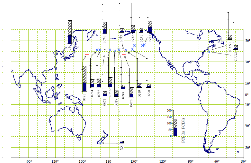
Figure 3-47. Dioxins levels (pg/g wet) in squid livers collected in various places along circumpolar front in north Pacific and central NOWPAP area (Hashimoto 1999).
