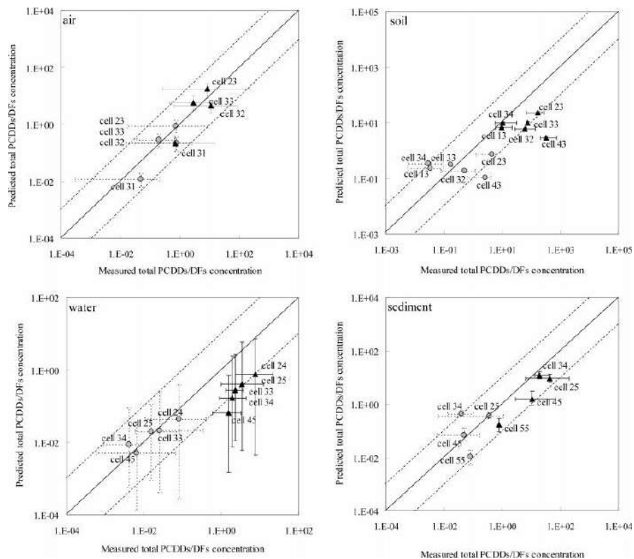
Figure 3-78. Comparisons between predicted total PCDD/Fs concentrations and those measured in each medium. The measured concentration is the averaged value of the measurements in each cell. Data are mean and the range. Triangles mark the mass-
