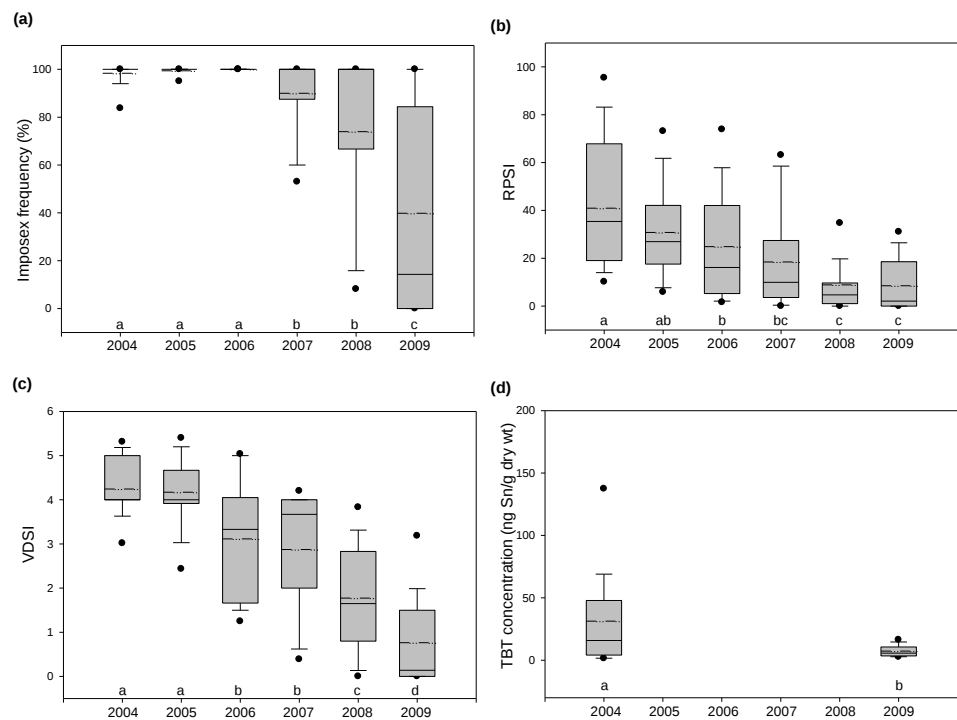
Figure 3-66. Temporal trends of (a) imposex frequency, (b) Relative Penis Size Index (RPSI), (c) Vas Deference Sequence Index (VDSI), and (d) gastropod ( Thais clavigera )
