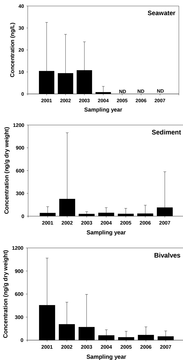
Figure 3-36. Temporal trends of TBT in seawater, sediment and bivalves (mussels or oysters) collected from Korean coastal waters (Choi et al., 2010; 2011).
