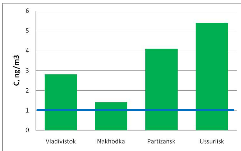
Figure 3-4. Benzo(a)pyrene concentration ( C , \text{ng/m}^3 ) in the air of industrial cities of Primorsky krai in 2010 (Report...2012). MPC of benzo(a)pyrene in Russia is 1 \text{ ng/m}^3 .
