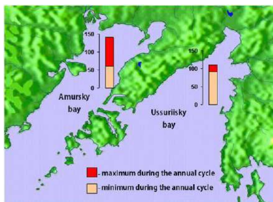
Figure 3-61. GST activity in the liver of flounder Liopsetta pinnifasciata from Amursky and Ussuriysky bays (Lukyanova,Ireykina,2012)
