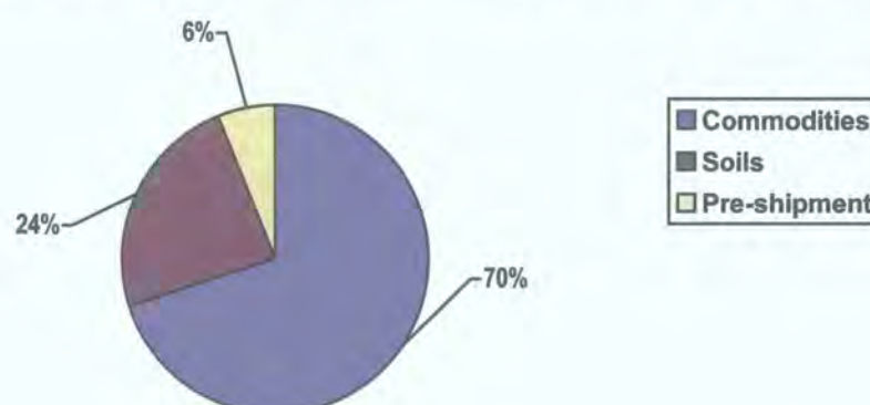
Fig. 9.1. Global QPS use by general category as found by survey (TEAP 2006a).
