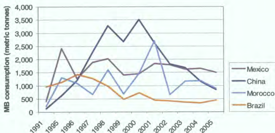
Figure 3.15. Trends in MB consumption in four Article 5 Parties that have consumed the largest volume of MB (>1400 tonnes per annum), 1991 – 2005.
