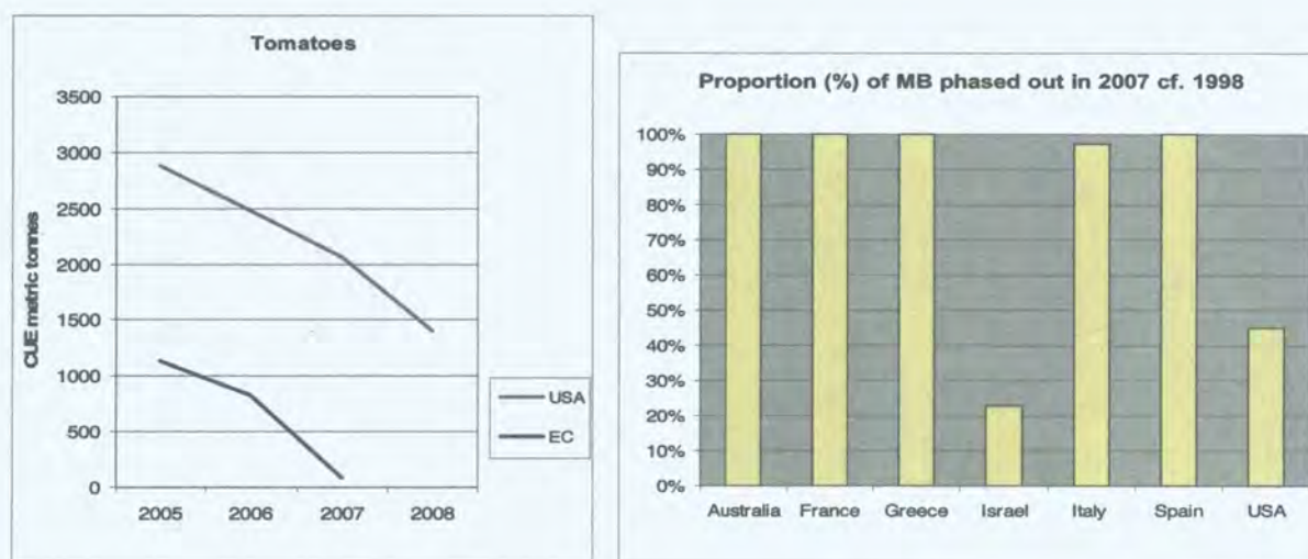
Figure 3.20. Left: Tomato CUE tonnes authorised by the MOP, 2005-2008. Right: Percentage of MB phased-out in tomato, 2007 c.f. 1998.
