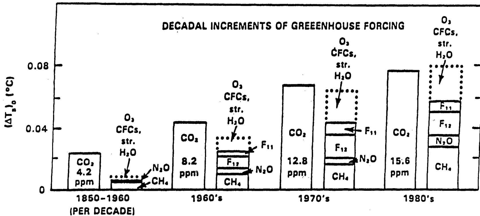
Figure 2. Decadal additions to global-mean greenhouse forcing of the climate system. (\Delta T_s)_0 is the computed temperature change at equilibrium ( t \rightarrow \infty ) for the estimated decadal increases in trace gas abundances, with no climate feedbacks included. (WMO, 1985).
