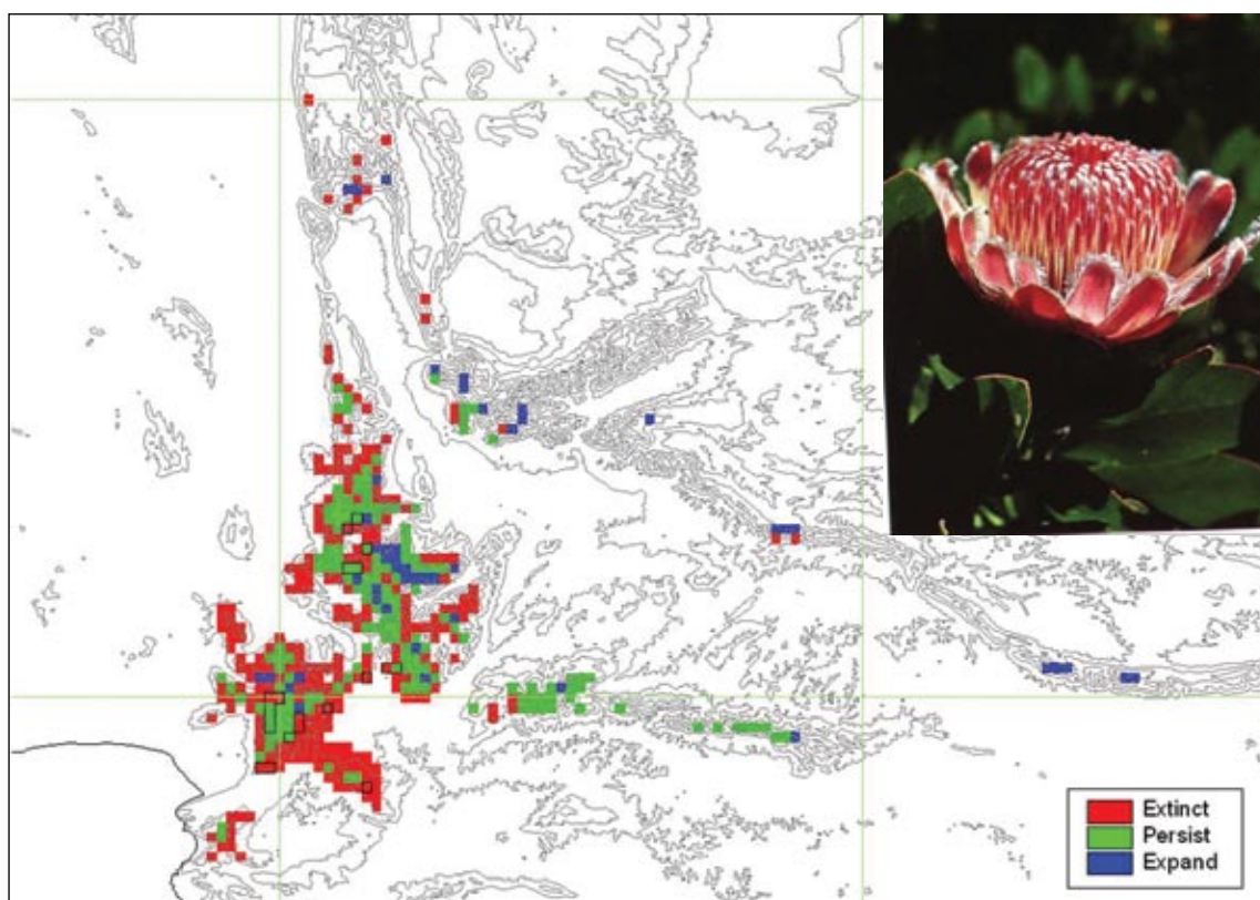
FIGURE 1. Shifting and shrinking ranges of the Protea laetiflora flower in Cape Floral Region Protected Areas (South Africa). The areas where this iconic plant will persist are displayed in green, while in many areas it will become extinct (red). (Hannah, 2005).
