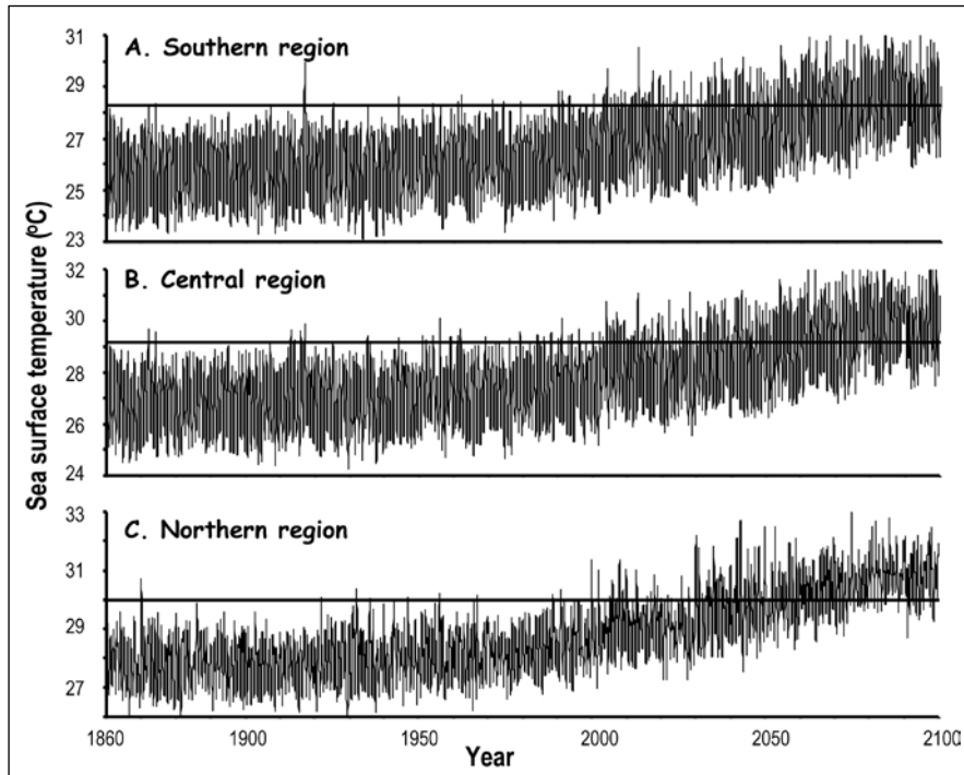
FIGURE 2. Sea surface temperature trends in the Great Barrier Reef region generated by the global coupled atmosphere-ocean-ice model (ECHAM4/OPYC3) forced by greenhouse warming that conforms to the IPCC scenario IS92a. Horizontal lines indicate the thermal thresholds of corals at each site. (Hoegh-Guldberg, 1999)
