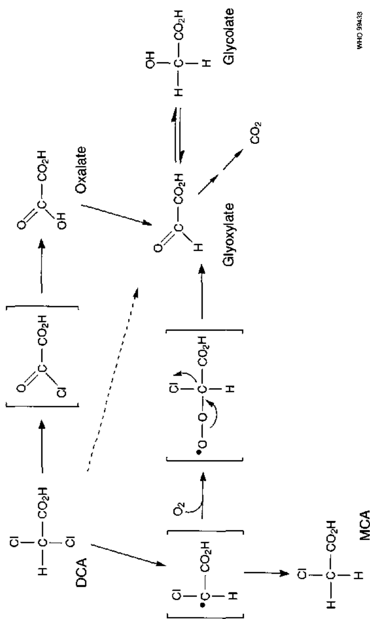
Fig. 3. Metabolic scheme for the metabolism of DCA (adapted from Larson & Bull, 1982).
