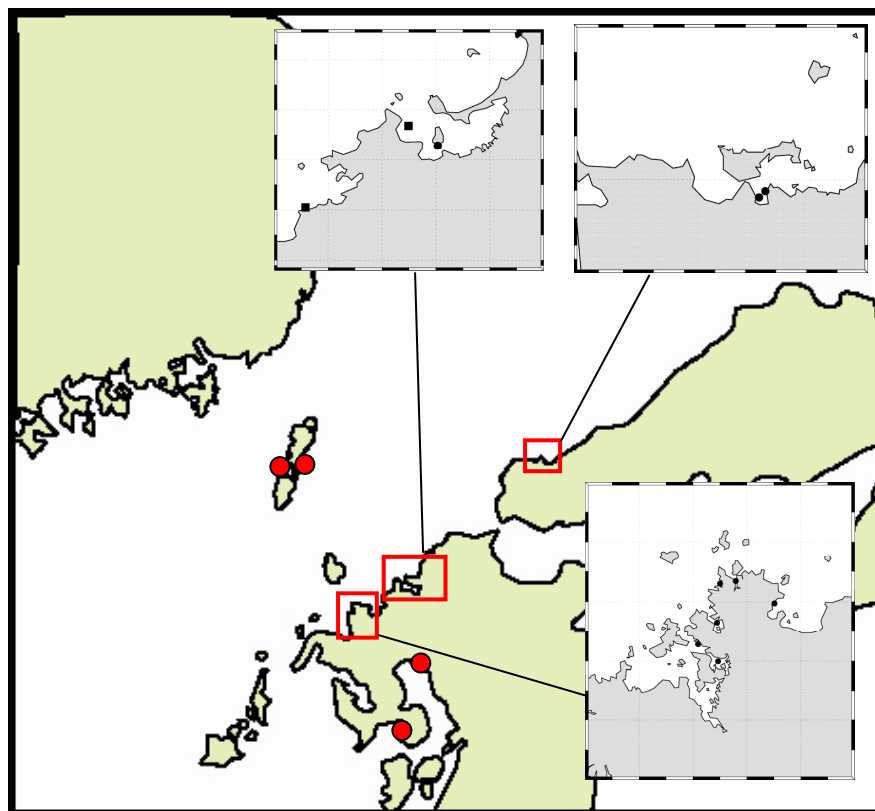
Figure 2.3 Location of shellfish poisoning and toxin-producing plankton monitoring sites in Japan
