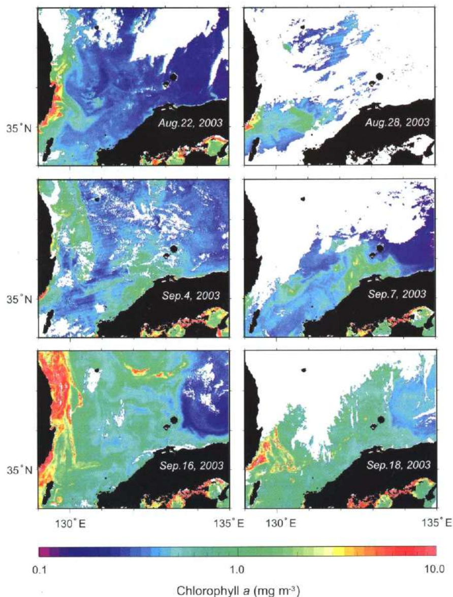
Figure 3.11 Movement of C. polykrikoides blooms along the coast of the Chugoku Region in Sea Area A
