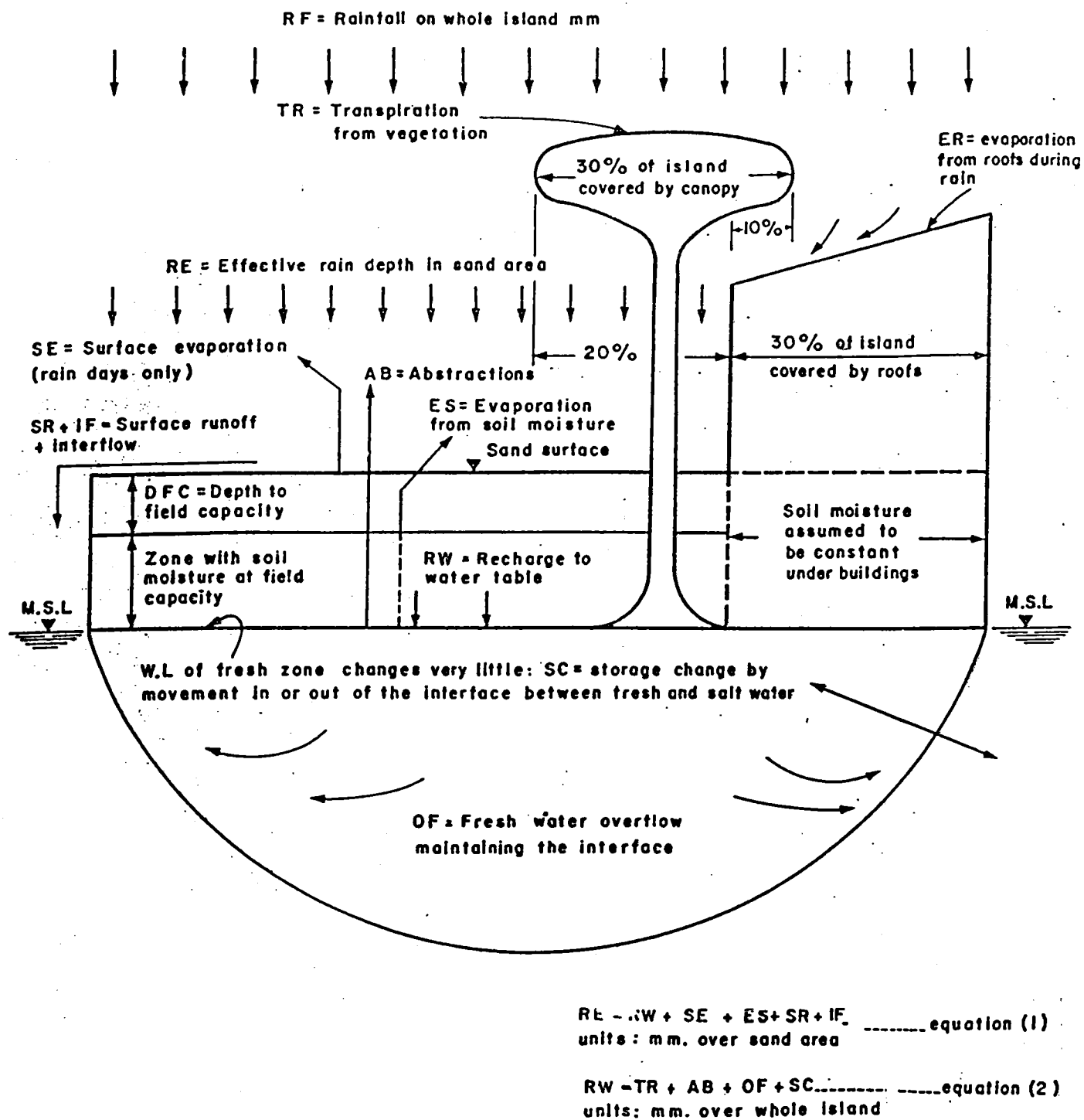
Figure 16. Malé hydrological cycle (Binnie &amp; Partners, 1983)
