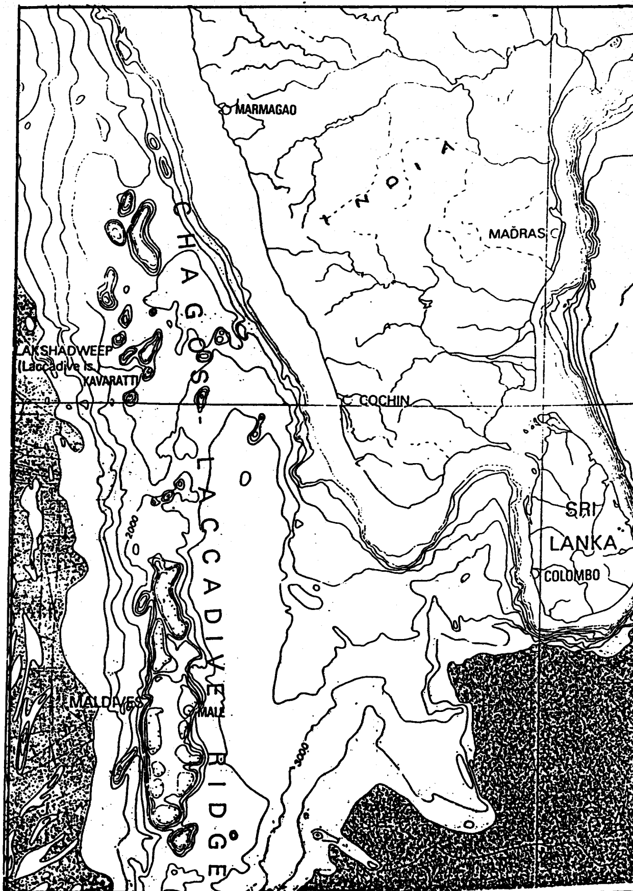
Figure 3. Generalized bathymetry of the Maldives Ridge
