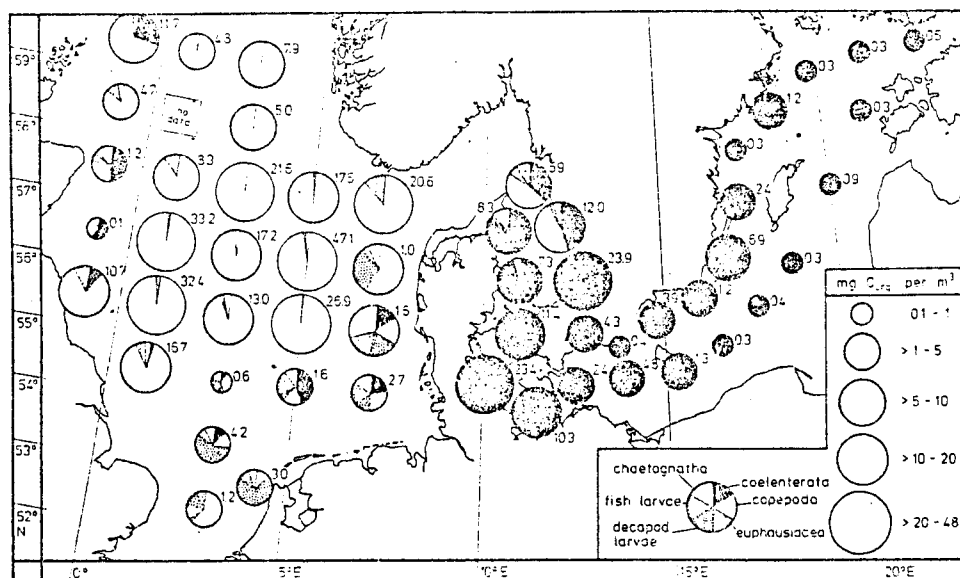
Figure I. Total biomass and composition of zooplankton > 500 µm in North Sea and Baltic Sea, 01/08 - 15/09/1978 (Möller, 1980 a)
