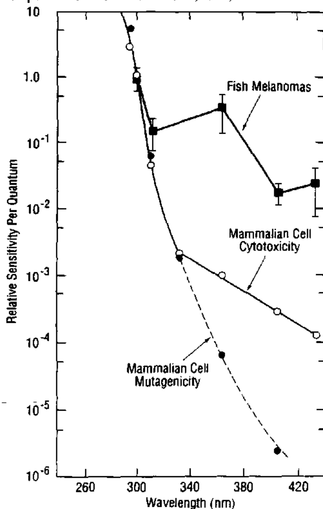
Figure 7.3 Estimated action spectrum for induction by UV and visible light of melanocytic tumours in hybrid fish of the genus Xiphophorus compare with published action spectra for mammalian cell mutagenicity and cytotoxicity. o, cytotoxicity; ●, mutagenicity; ■, induction of melanocytic tumours (Reprinted with permission from Setlow et al., 1993).
