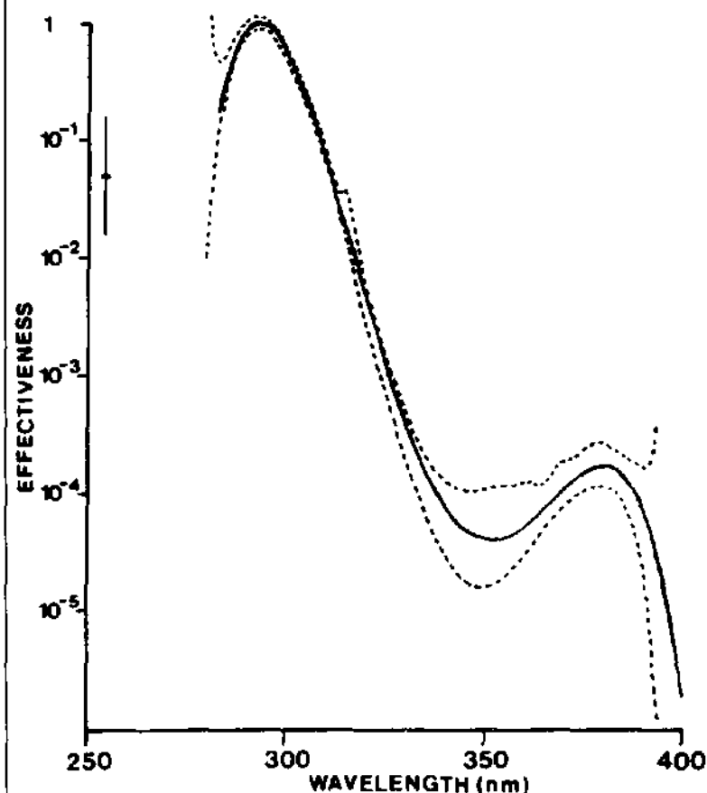
Figure 7.2 Estimated action spectrum (called the SCUP action spectrum) for induction by UV of SCC in the skin of albino hairless mice (Skh-hr 1). The dashed lines (--) show the upper and lower limits for 5 nm displacements of the action spectrum that do not increase the \chi^2 for fit of the spectrum to the data by more than 1.0 (Reprinted with permission from de Gruijl et al., 1993).
