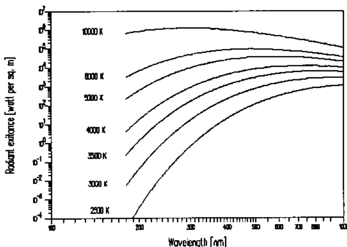
Figure 3.2 Spectral emissions of black body radiators at different temperatures (McKinlay et al., 1988)
