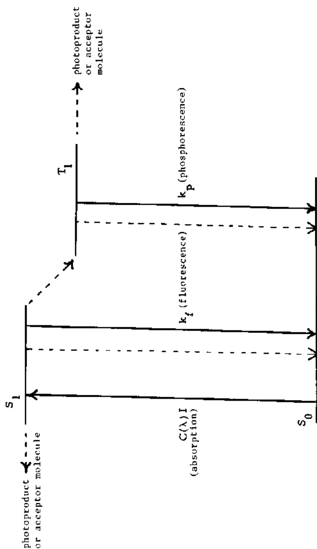
Figure 5.1 Three-level electronic energy level diagram. Dashed lines represent non-radiative transitions while solid lines correspond to radiative transitions
