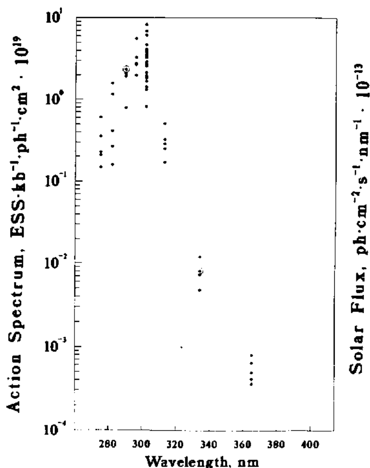
Figure 8.1 Action spectrum for the formation of pyrimidine dimers in human skin on exposure to UV between 275 nm and 366 nm as measured by the formation of micrococcus luteus endonuclease sensitive sites (ESS). Each point (•) represents one subject, circled points indicate two subjects with identical dimer yields. ph=photon, kb=kilobase. (Reprinted in modified form with permission from Freeman et al., 1989).
