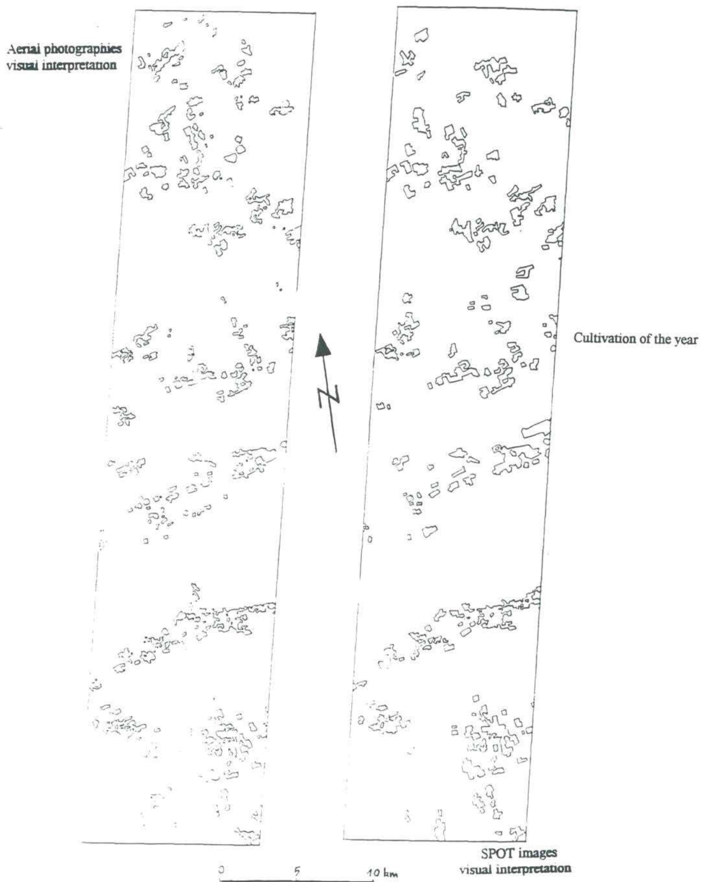
FIGURE 5: NARA - COMPARATIVE INTERPRETATION OF AERIAL PHOTOGRAPHS AND SPOT IMAGE IN THE THEME: LAND CULTIVATION OF THE YEAR IN 1987.
