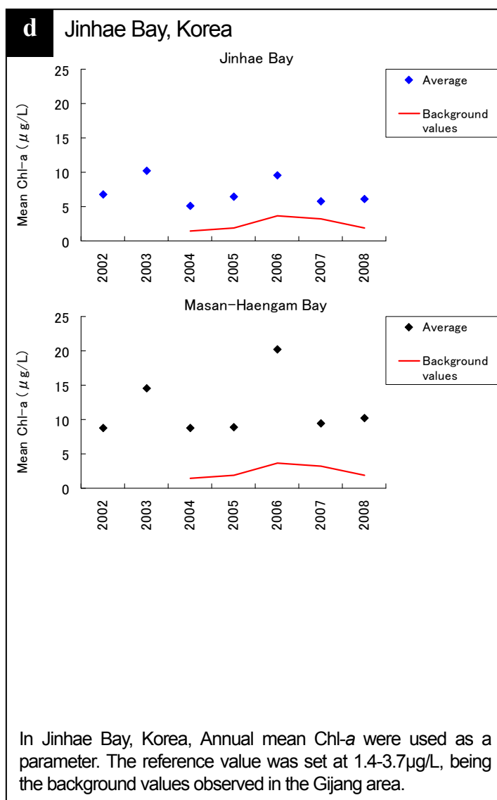
Fig. 3.7 Annual mean Chl- a in selected sea areas in the NOWPAP region
