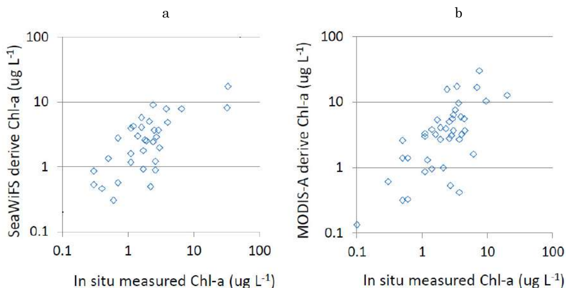
Fig. 4 Comparison of in situ and satellite derived Chl- a in Toyama Bay
