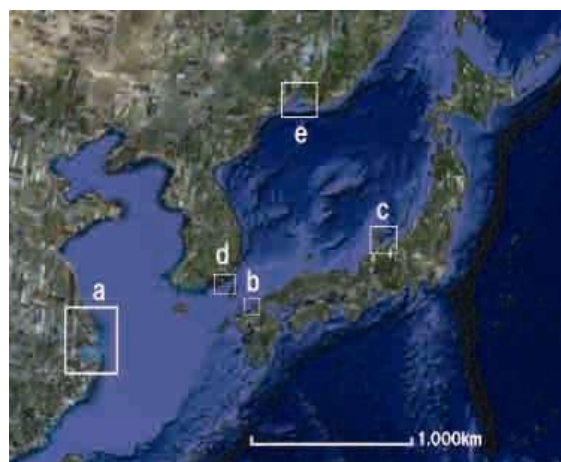
Fig. 3.4 DIP concentration in selected sea areas in the NOWPAP region
