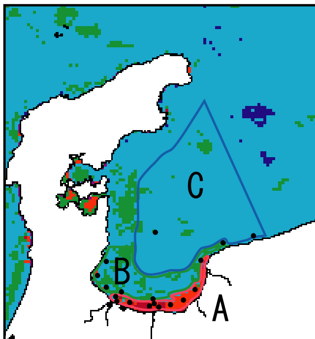
Fig. 2.10 Sub-areas determined from the preliminary eutrophication assessment by satellite derived Chl- a data in Toyama Bay, Japan (See Annex C): (A) coastal area, (B) intermediate area and (C) offshore area.
