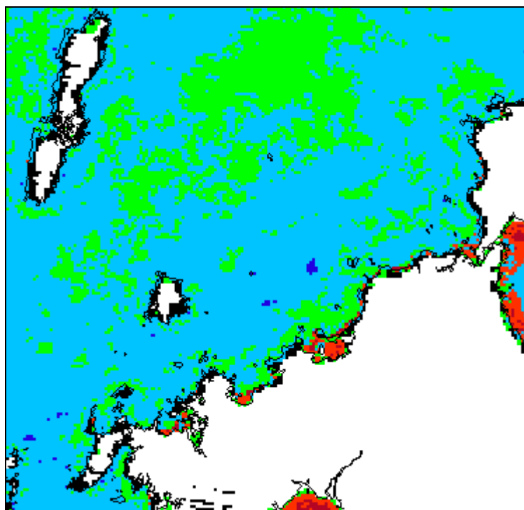
Fig. 3 Preliminary eutrophication assessment by satellite derived Chl- a data in the Northwest Kyushu sea area, Japan
