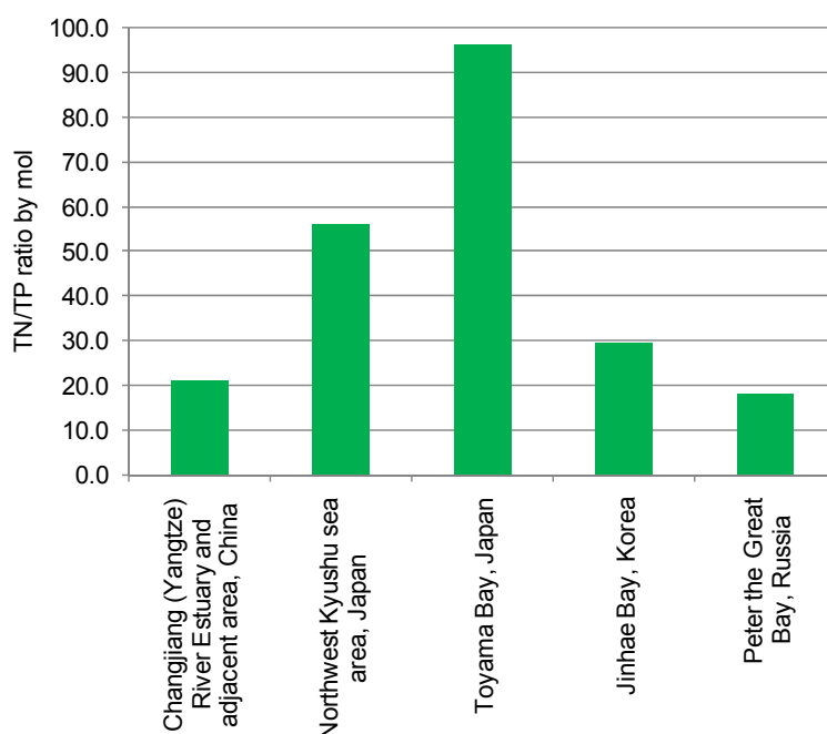
Fig. 3.11 Ratios of TN/TP loadings in the selected sea areas in the NOWPAP region. The value of Changjiang (Yangtze) River Estuary and its adjacent area is for 2010. The values of the Northwest Kyushu sea area and Toyama Bay are for 2007. The value of Jinhae Bay is an average between 1995 and 1996. The value of the Peter the Great Bay is an average between 2001 and 2008.
